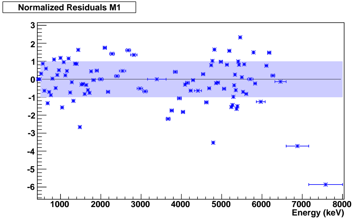
Figure C.13: Fit of the simulated spectrum components to the Multiplicity 1 (M1) spectrum for crystal configuration F. The fit was performed simultaneously on the M1, M1, and M2Tot spectra.
