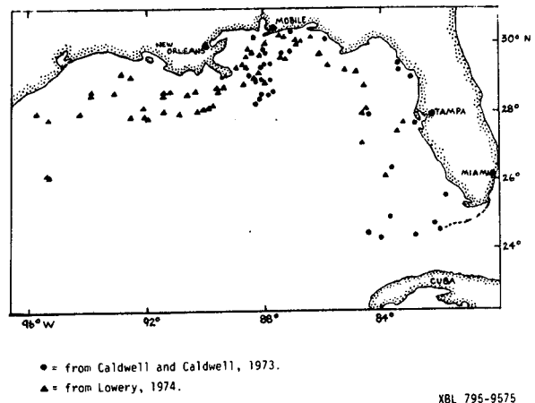
Fig. 2 Sightings of the spotted dolphin, Stenella plagiodon , in the Gulf of Mexico.
