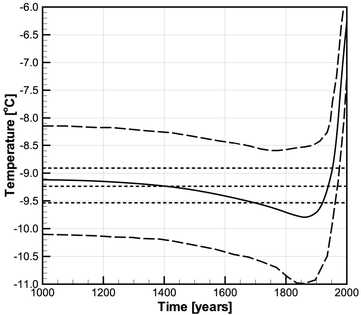
Figure 4. Estimated ground surface temperature history (solid line) with 95% error band; estimated long-term average (dash-dotted) line with 95% uncertainty band.
