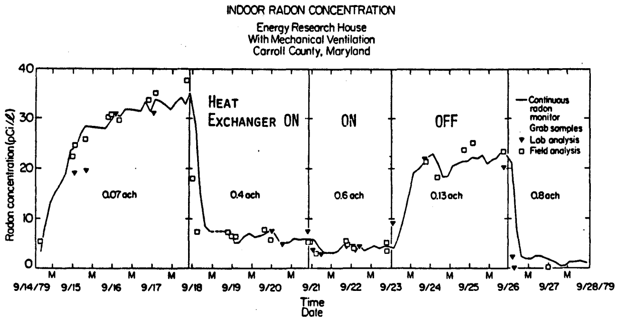
Figure 2. Indoor Radon concentrations at various air-exchange rates. In terms of risk of lung cancer, the vertical scale corresponds to "cigarettes per day" on days that the windows are closed.
