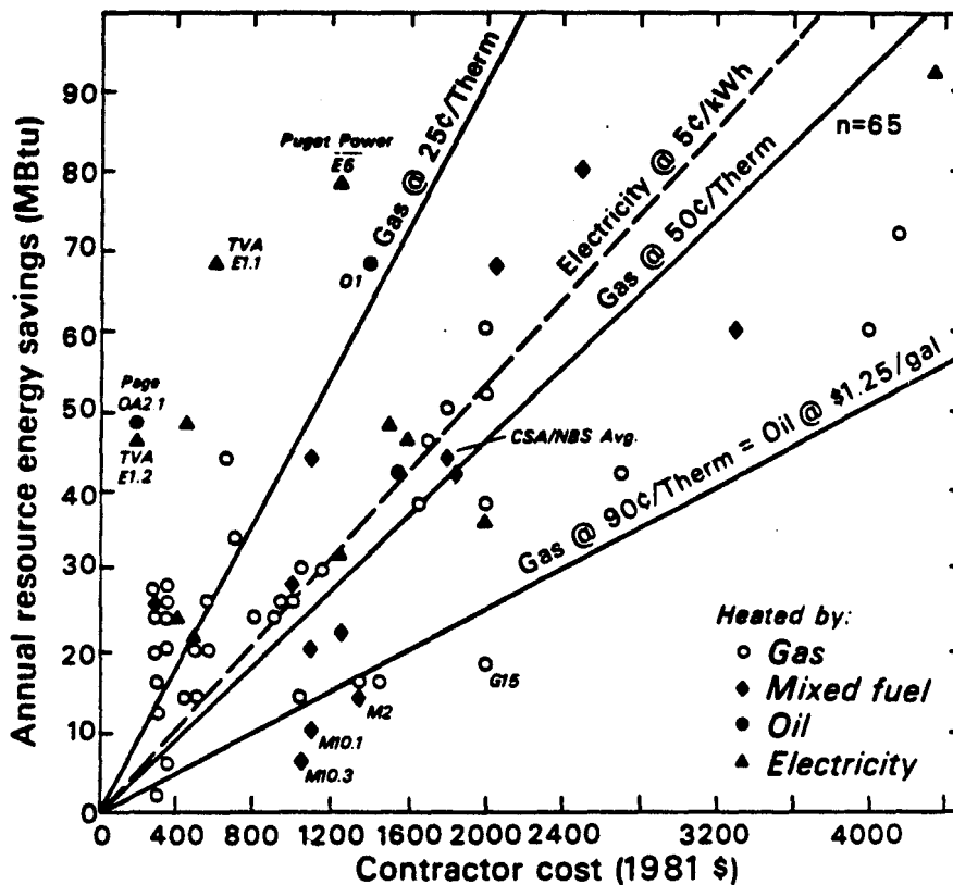
Figure 14. Scatter plot of Annual resource energy savings vs. Contractor cost for the residential building retrofit projects contained in the BECA-B data base. Cost-effectiveness boundary lines are drawn for reference.
