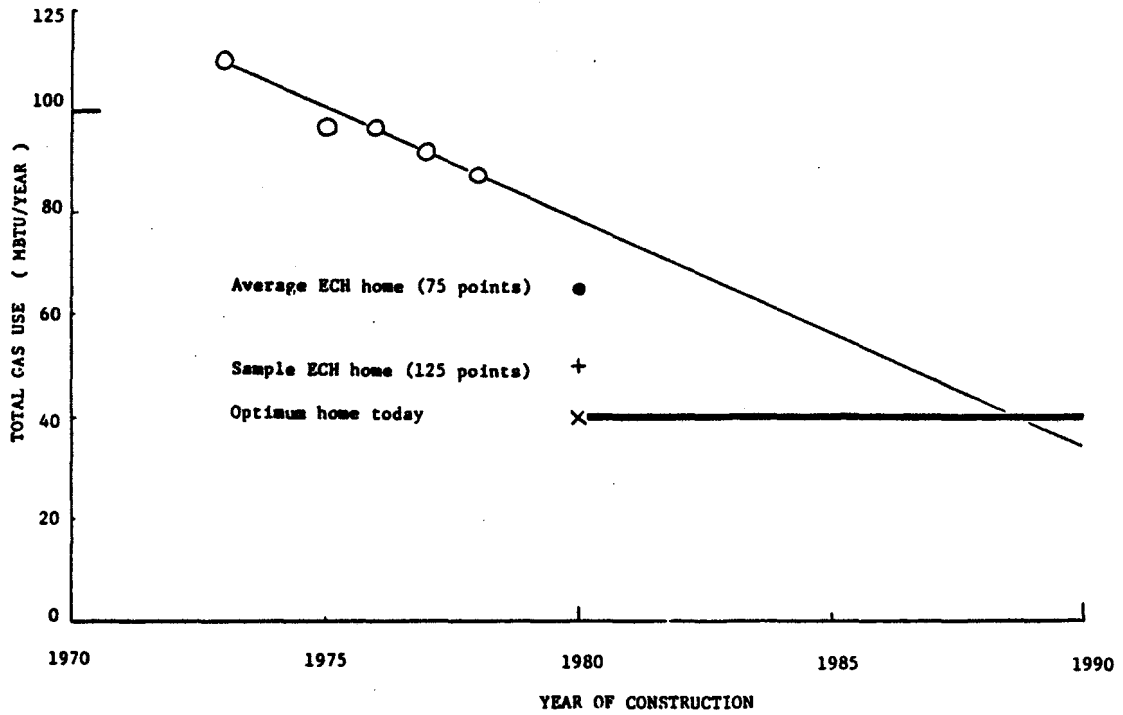
Figure 20. Time trend for total gas use in new homes located within Pacific Gas & Electric Company's service area. Points representing an average ECH home and an optimum home are plotted for reference.
