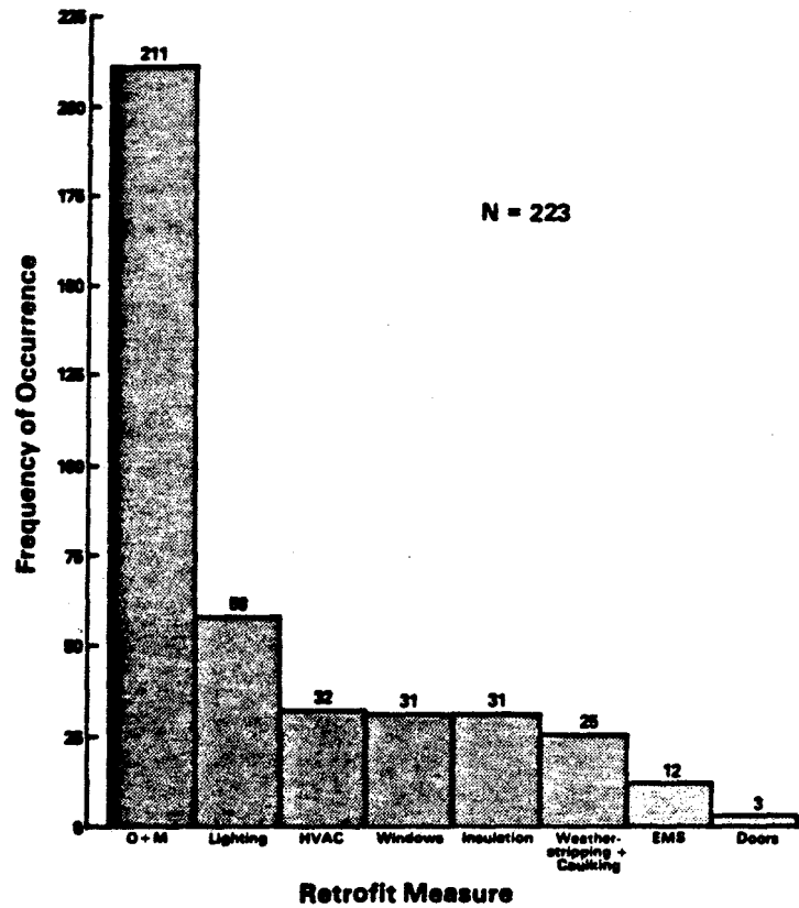
Figure 11. Histogram of installed measures for commercial building retrofits contained in BECA-C data base.
