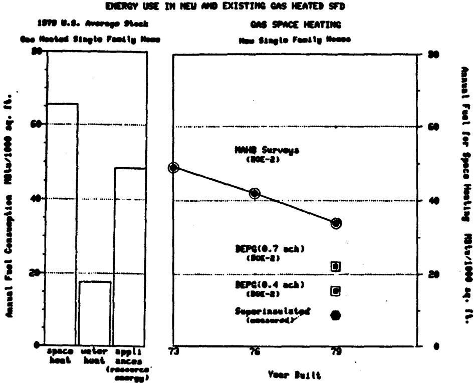
Figure 8. Time trend in annual fuel for space heating in new U.S. single-family homes.
