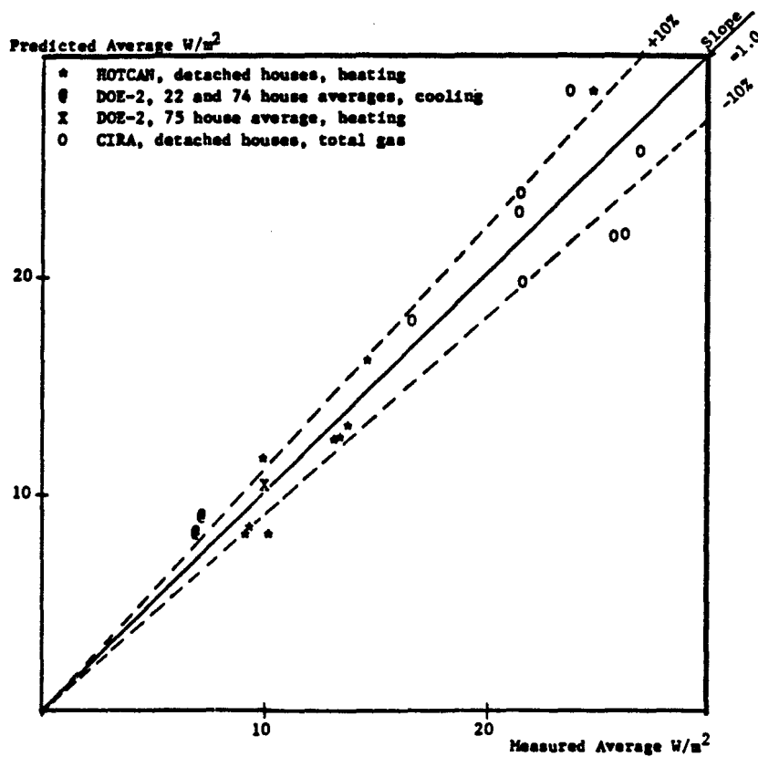
Figure 18. Predicted energy use vs. Measured site energy use, averaged over monitoring period (3 months to 1 year), for residential buildings contained in the BECA-V data base.
