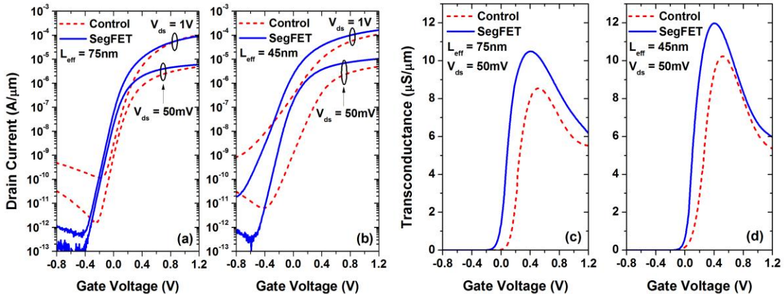
Fig. 2.6. Measured transfer characteristics for a SegFET and a control device for electrical channel lengths of (a) 75 nm and (b) 45 nm; measured linear transconductance for (c) L_{\text{eff}} = 75 nm and (d) 45 nm. Data is normalized to the device layout width.
