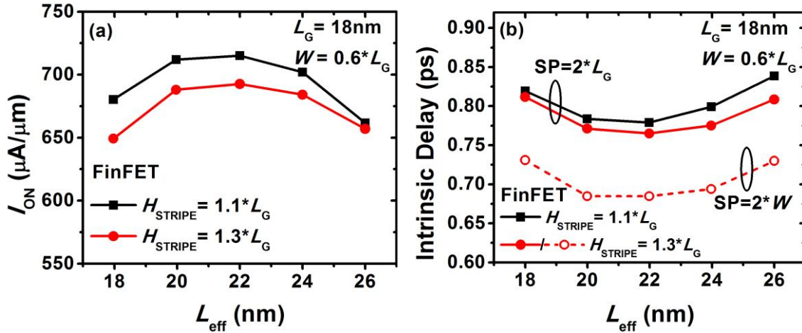
Fig. 3.8. FinFET bulk MOSFET design optimization. (a) I_{ON} vs. L_{\text{eff}} , for I_{\text{OFF}} = 7\text{ nA}/\mu\text{m} , (b) Delay vs. L_{\text{eff}} . L_G = 18\text{nm} , W = 0.6 \cdot L_G , t_{\text{ox}} = 9\text{Å} , X_{\text{J,SD}} = 1.2 \cdot H_{\text{STRIPE}} , t_{\text{Si}} = H_{\text{STRIPE}} , V_{\text{DD}} = 0.7\text{V} . Solid lines are for SP = 2 \cdot L_G ; dashed line is for SP = 2 \cdot W .
