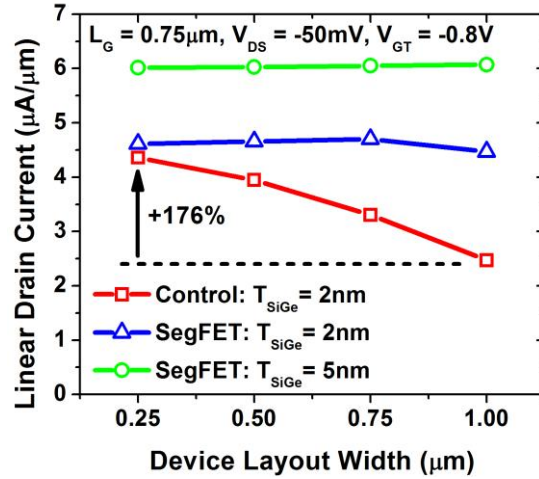
Fig 5.12. I_{D,LIN} of the planar control and various SegFET devices for different layout widths. Current is per \mu\text{m} layout width. L_G = 0.75 \mu\text{m} .
