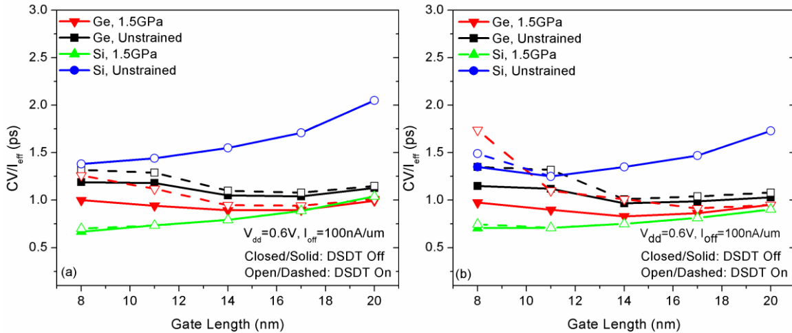
Fig. 6.9: Intrinsic delay as a function of gate length, for (a) \langle 110 \rangle / \{ 100 \} and (b) \langle 110 \rangle / \{ 110 \} channel orientations with and without DSDT.
