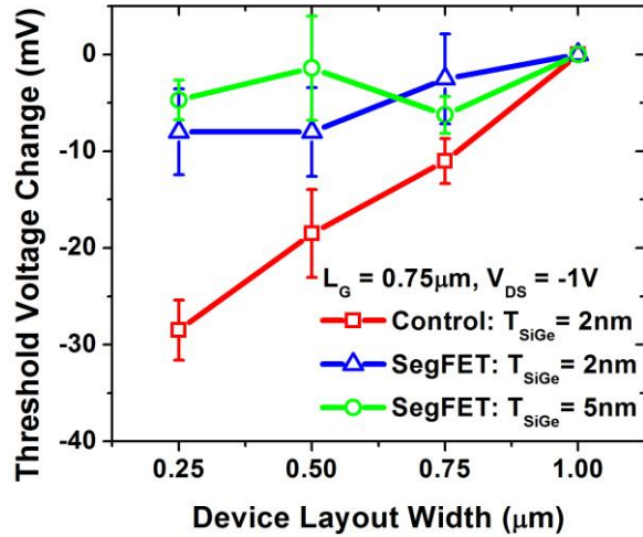
Fig 5.11. \Delta V_{T,SAT} for control and SegFET devices, for different layout widths. The error bars indicate +/- one standard deviation in \Delta V_{T,SAT} . L_G = 0.75 \mu\text{m} .
