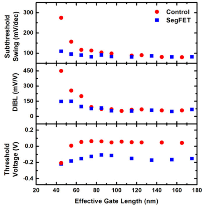
Fig. 2.10. Average (over 6 die) measured subthreshold swing, drain-induced barrier lowering (DIBL), and V_{\text{TH, SAT}} as a function of L_{\text{eff}} . SegFETs show improved scalability compared to the control devices.
