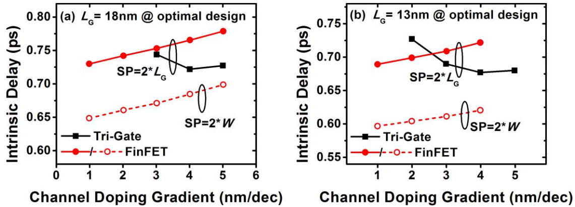
Fig. 3.9. Impact of retrograde channel doping gradient on the performance of tri-gate bulk and FinFET bulk MOSFETs. For the tri-gate design, W = 1 \cdot L_G , H_{\text{STRIPE}} = 0.8 \cdot L_G ; for the FinFET design, W = 0.6 \cdot L_G , H_{\text{STRIPE}} = 1.3 \cdot L_G . (a) L_G = 18\text{nm} , t_{\text{ox}} = 9\text{Å} , t_{\text{Si}} = H_{\text{STRIPE}} , V_{\text{DD}} = 0.7\text{V} , (b) L_G = 13\text{nm} , t_{\text{ox}} = 8\text{Å} , t_{\text{Si}} = H_{\text{STRIPE}} , V_{\text{DD}} = 0.6\text{V} . Solid lines are for SP = 2 \cdot L_G ; dashed line is for SP = 2 \cdot W .
