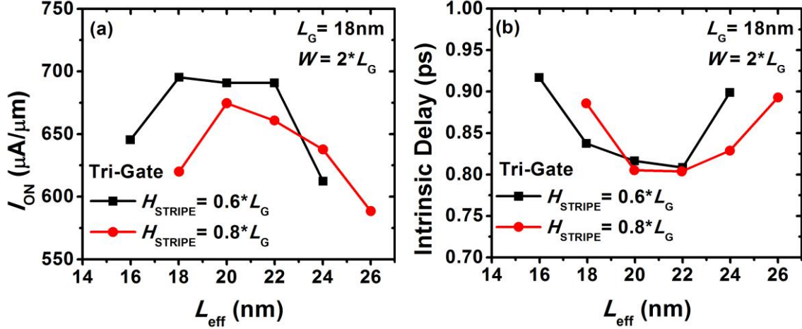
Fig. 3.7. Tri-gate bulk MOSFET design optimization for channel stripe width W = 2 \cdot L_G . (a) I_{ON} vs. L_{eff} , for I_{OFF} = 7 \text{ nA}/\mu\text{m} , (b) Delay vs. L_{eff} . L_G = 18\text{nm} , t_{ox} = 9\text{\AA} , X_{J,SD} = 1.2 \cdot H_{STRIPE} , t_{Si} = H_{STRIPE} , V_{DD} = 0.7\text{V} .
