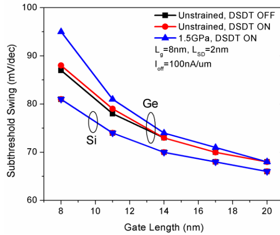
Fig. 6.5: S as a function of gate length, with and without DSDT, for MOSFETs with \langle 110 \rangle / \{ 100 \} channel orientation.
