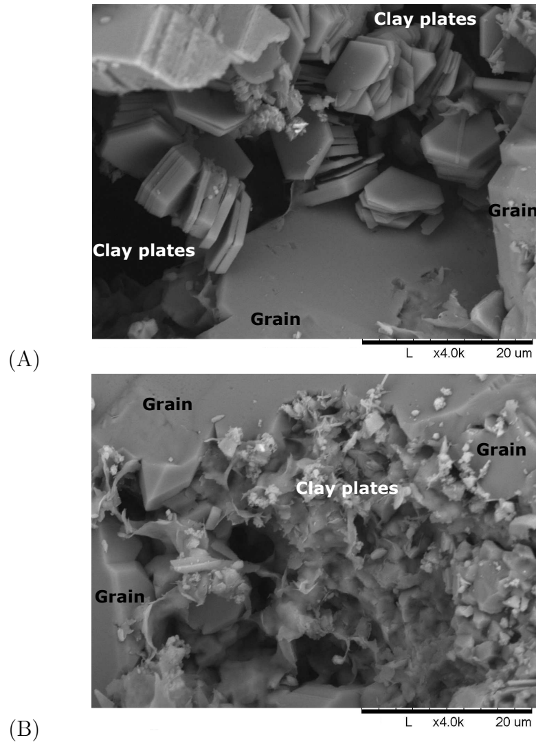
FIGURE 7. SEM 4000 \times magnification images show different types of clay plates contribute to the microporosity of the sample: kaolinite (A) and montmorillonite (B).
