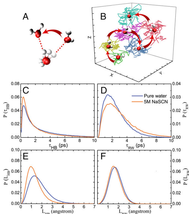
Fig. 4. Two possible “hopping” mechanisms. The schematic picture of the hydrogen bond switching (A) and the collective water dynamics (B). The distributions of hopping time ( Middle row ) and length ( Bottom row ) of water molecule are presented for pure water (blue) and 5 M NaSCN solutions (orange) in the hydrogen bond switching (C and E) and collective dynamics (D and F) picture, respectively.
