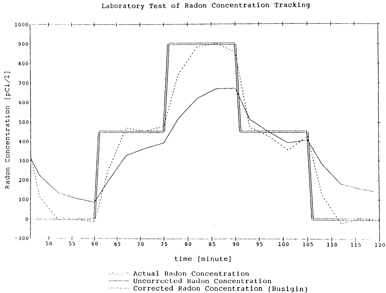
Figure 7. Comparison between actual time-varying radon concentration and the concentration predicted using continuous-radon-monitor data with and without data correction using the Busigin (1979) method. In actual practice, radon concentrations are determined by averaging the predictions during each measurement period, excluding the first few predictions which are affected by purging the scintillation cell of the previous sample.
