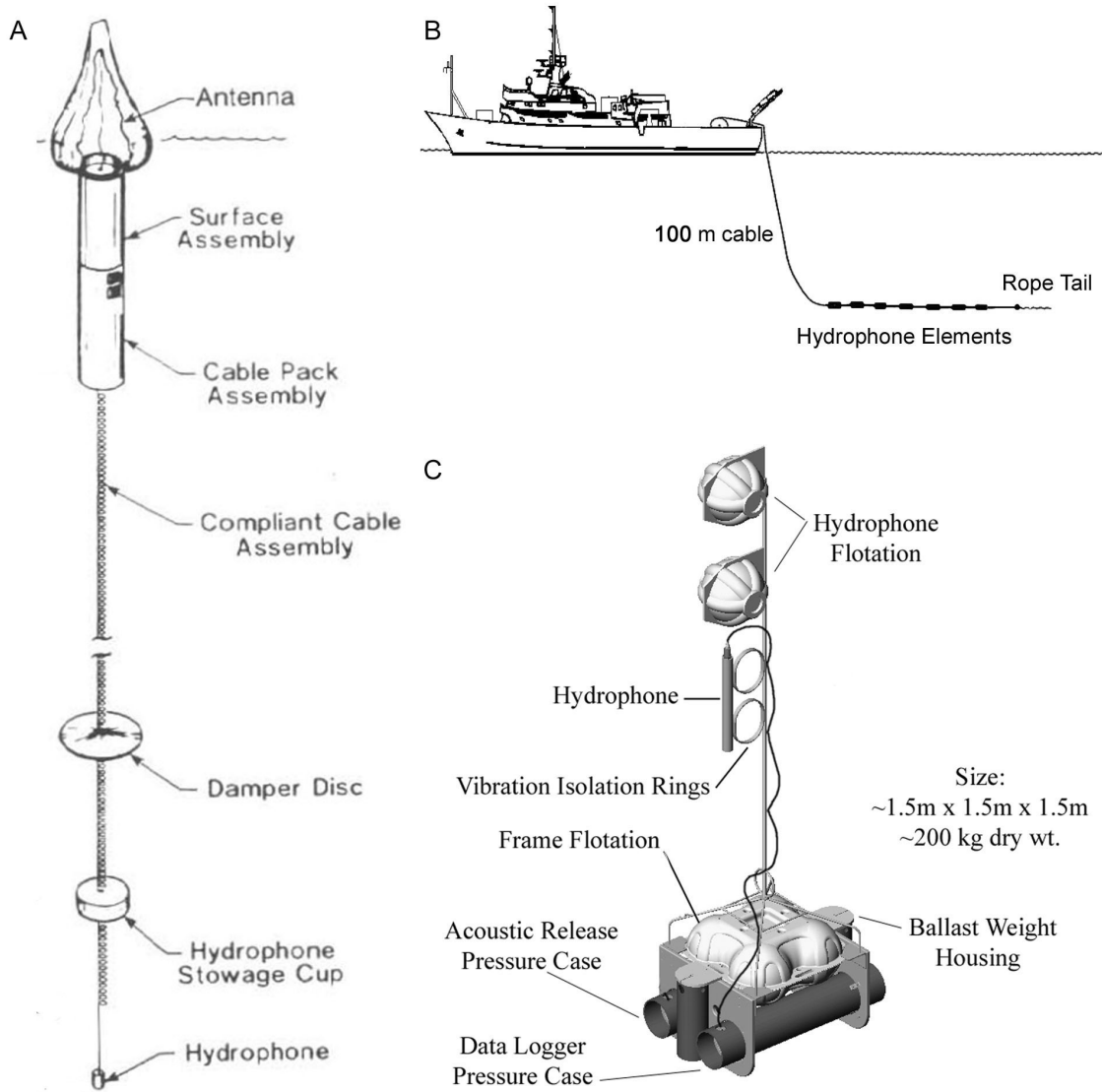
Figure 1. Acoustic instruments used for detecting cetaceans in the CalCOFI study area. A) SSQ 57 type sonobuoy. B) Towed hydrophone array. C) HARP (High-frequency Acoustic Recording Package).
