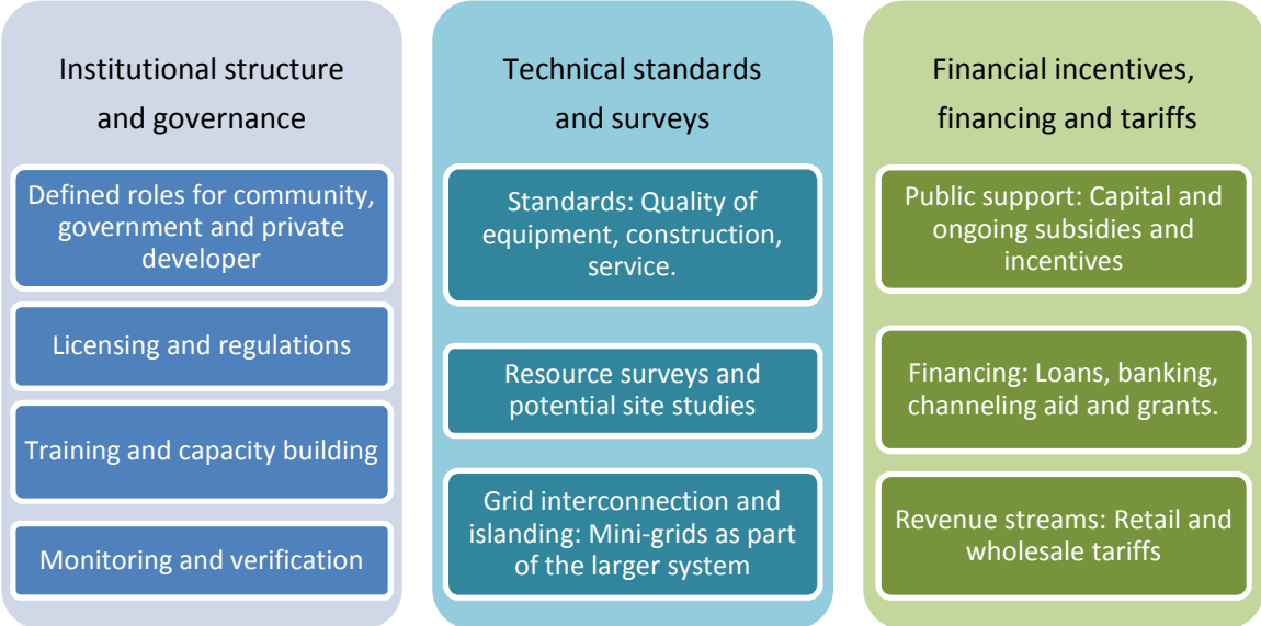
Figure 3: Categories of renewable energy-based mini-grids policy framework
