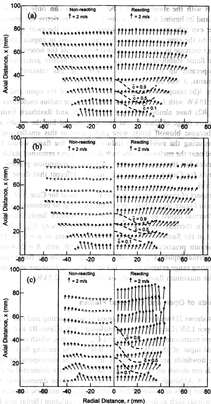
FIGURE 4 2D rector plots obtained in non-reacting and reacting flows at S_g = 0.05 , U_\infty = 3.0 \text{ m/s} , and \phi = 0.80 for (a) Case A; (b) Case B1; and (c) Case B2.
