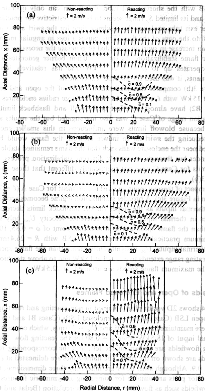
FIGURE 4 2D vector plots obtained in non-reacting and reacting flows at S_g = 0.05 , U_\infty = 3.0 \text{ m/s} , and \phi = 0.80 for (a) Case A; (b) Case B1; and (c) Case B2.
