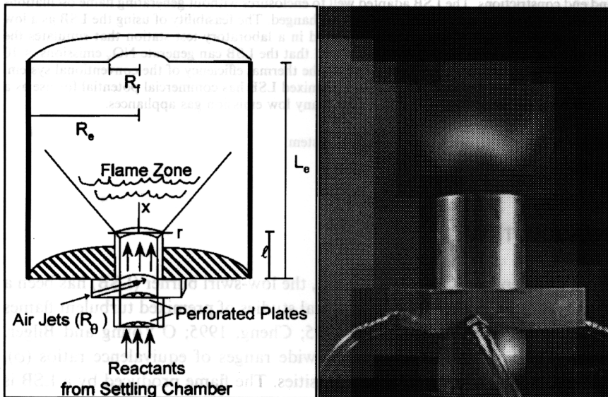
FIGURE 1 Schematic of the Low Swirl Burner and its operation.
