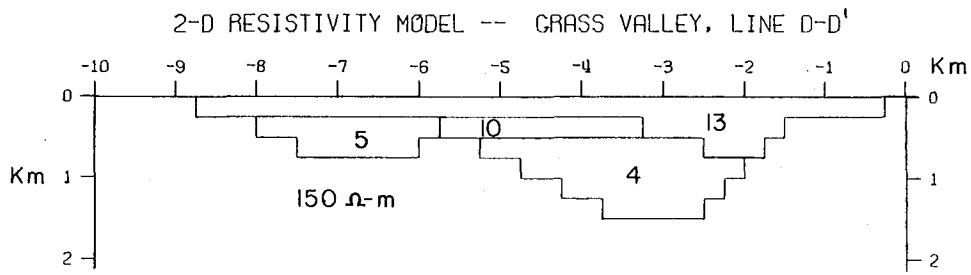
Figure III-20. Dipole-dipole apparent resistivity pseudo-section for 1 km dipoles along Line D-D': field data, model generated data, and two-dimensional resistivity model.
