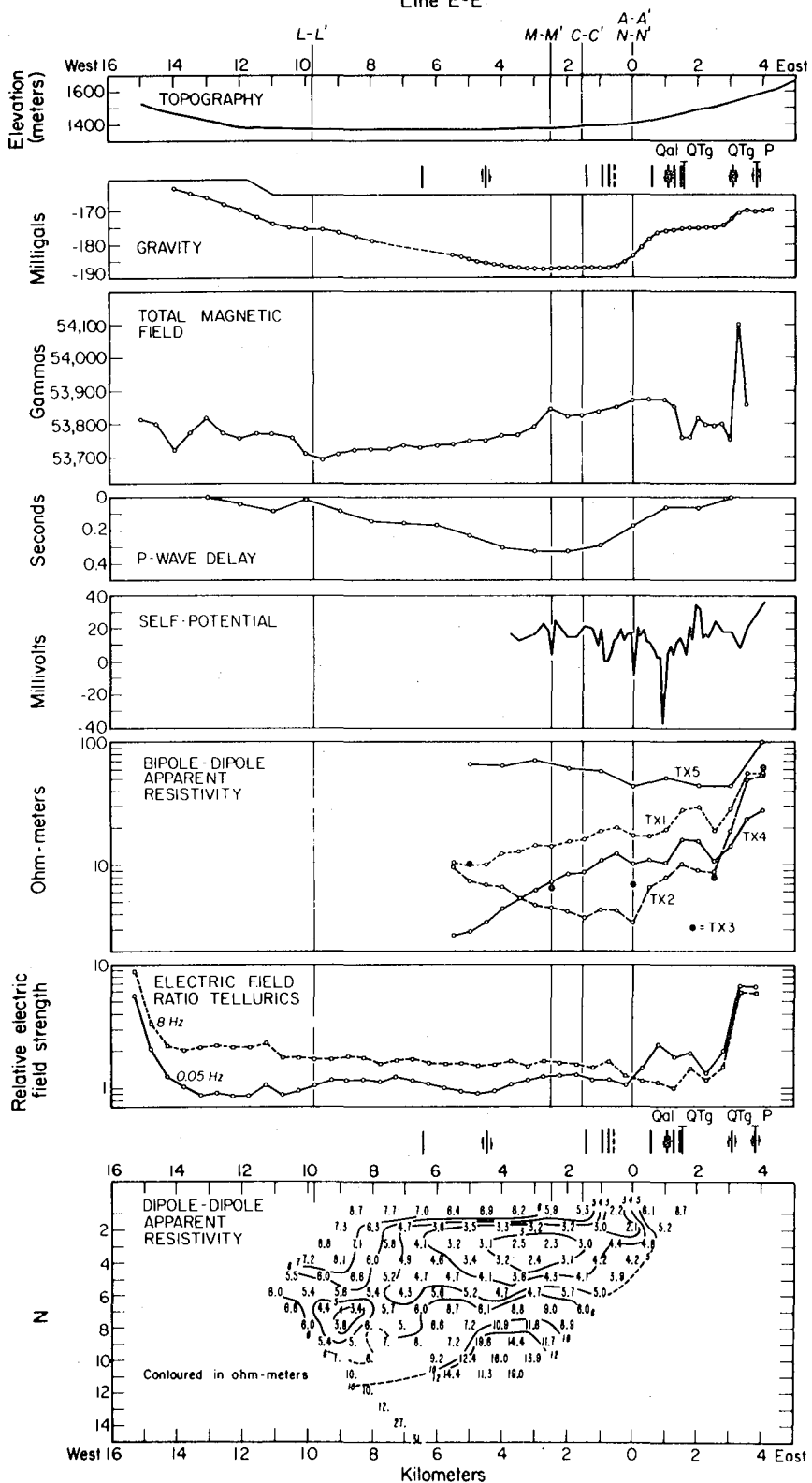
Figure 111-A5. Geophysical data profile composite for Line E-E'.
