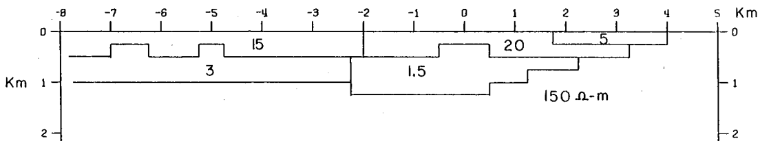
Figure III-19. Dipole-dipole apparent resistivity pseudo-section for 1 km dipoles along Line B-B': field data, model generated data, and two-dimensional resistivity model.
