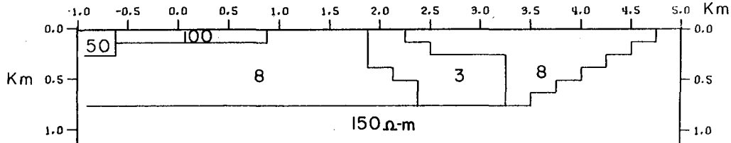
2-D RESISTIVITY MODEL -- GRASS VALLEY, LINE H-H'
