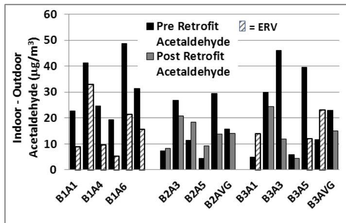
Figure 10: Acetaldehyde concentrations
