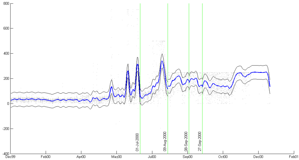
Figure 6: The ISO prices during 2000 (blue dots) with Gaussian processes from different runs separated by change points (green lines).
