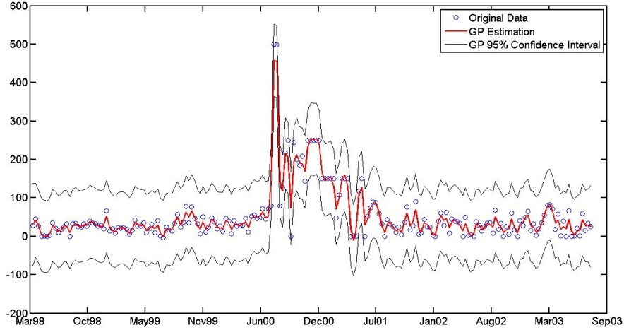
Figure 2: Gaussian Process
