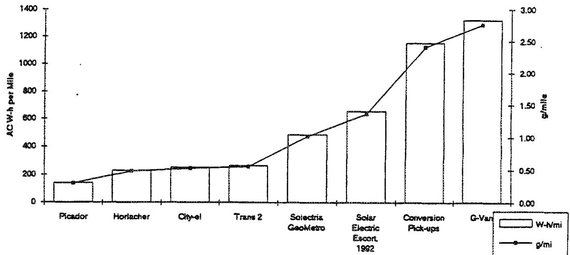
Energy Use and Emissions for EV's
