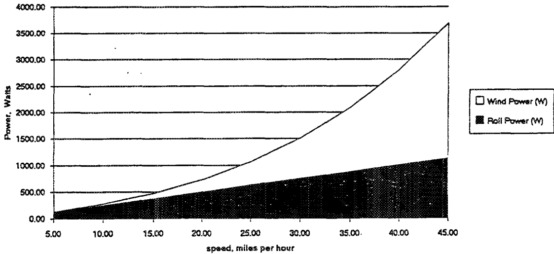
Rolling Resistance Plus Wind Resistance vs Speed, for City-el (Cd*A = 0.475, F-roll = 50 N)
