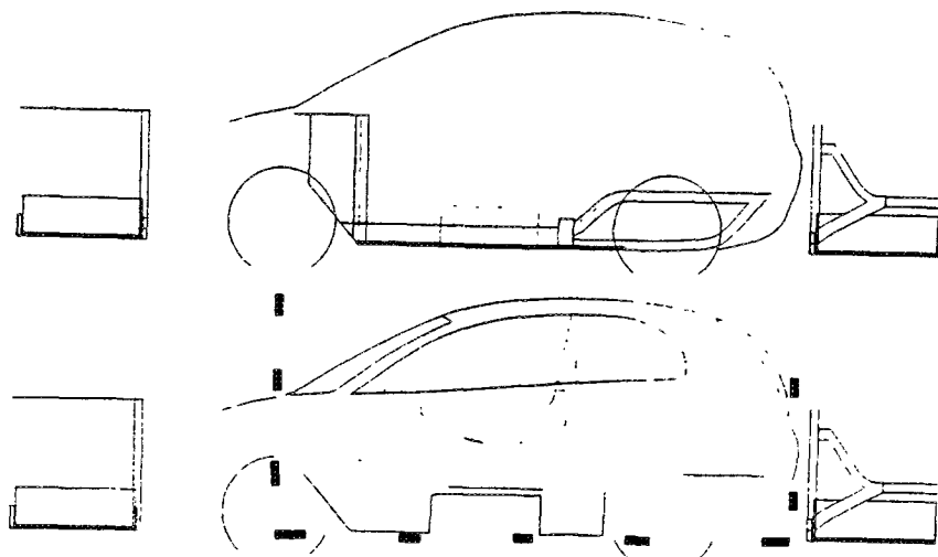
Figure 6: Drawings developed to evaluate driver and passenger ergonomics
