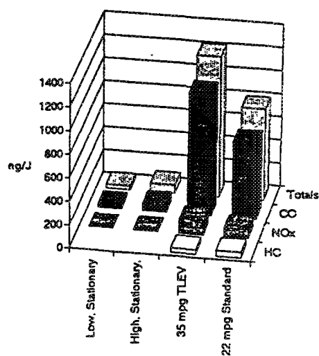
Emissions permitted, stationary vs. Mobile Sources
