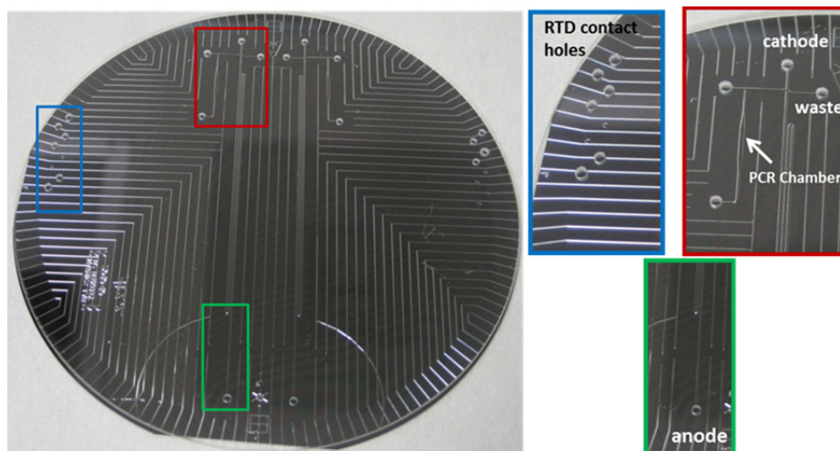
Figure 85. Top view of the etched glass wafer.
