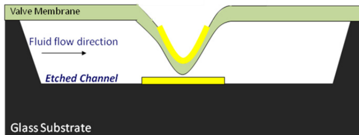
Cross Section: Actuated Valve
