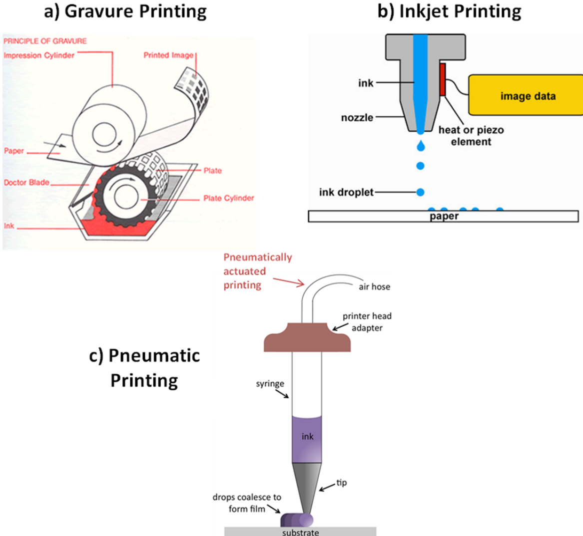
Figure 1. The principle behind a) gravure [3], b) inkjet [4], and c) pneumatic [5] printing methods.
