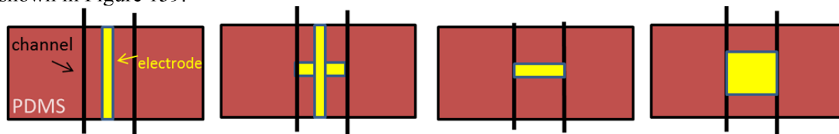
Figure 159. Different print configurations for electrode2 that can potentially enhance the functioning of valves.
