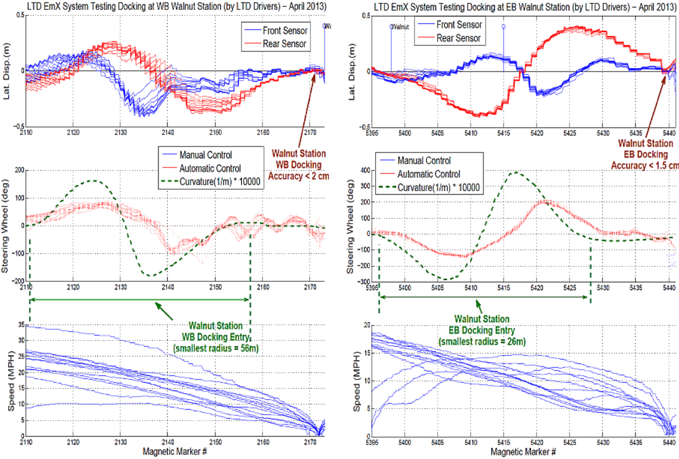
Figure 5-19 Precision docking performance at EmX track—Walnut Station (WB & EB)
