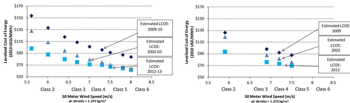
Figure ES-2. LCOE for wind energy over time in the United States (left) and Denmark (right)
