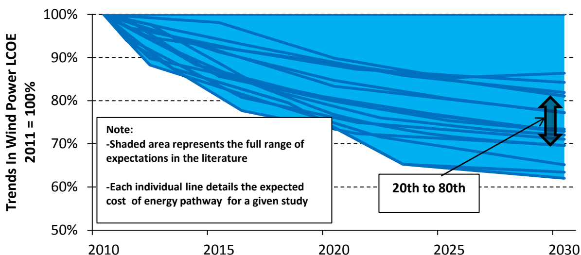
Figure 11. Estimated range of wind LCOE projections across 18 scenarios
