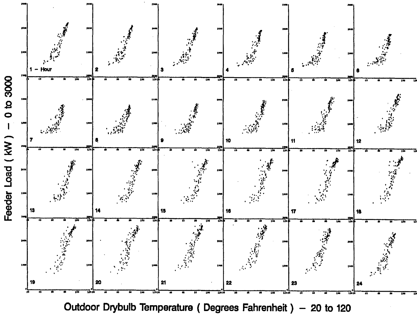
Figure A-34. Scatterplots of Feeder 12 Hourly Load vs. Drybulb Temperature for Standard Summer Days
