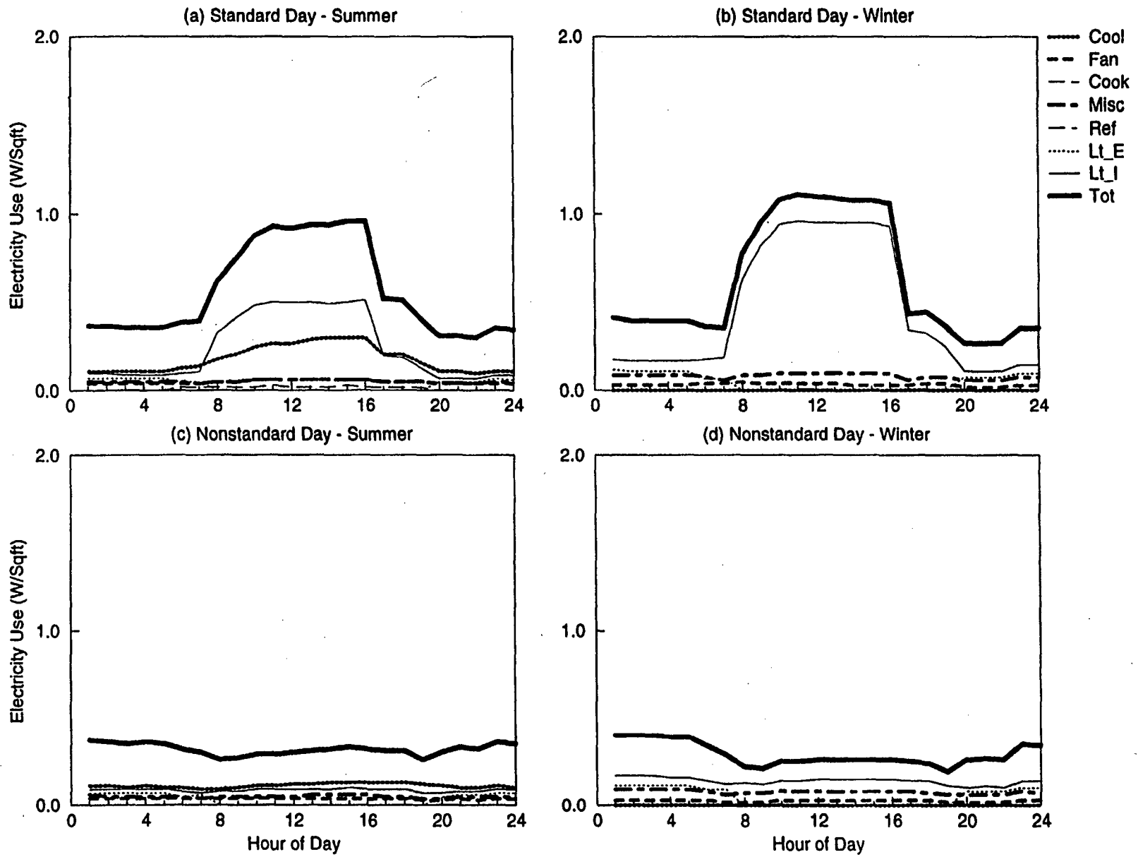
Figure C-43. EDA Reconciled End-use Load Shapes for Large Vehicle Maintenance (Split DX) (Feeder 15)
