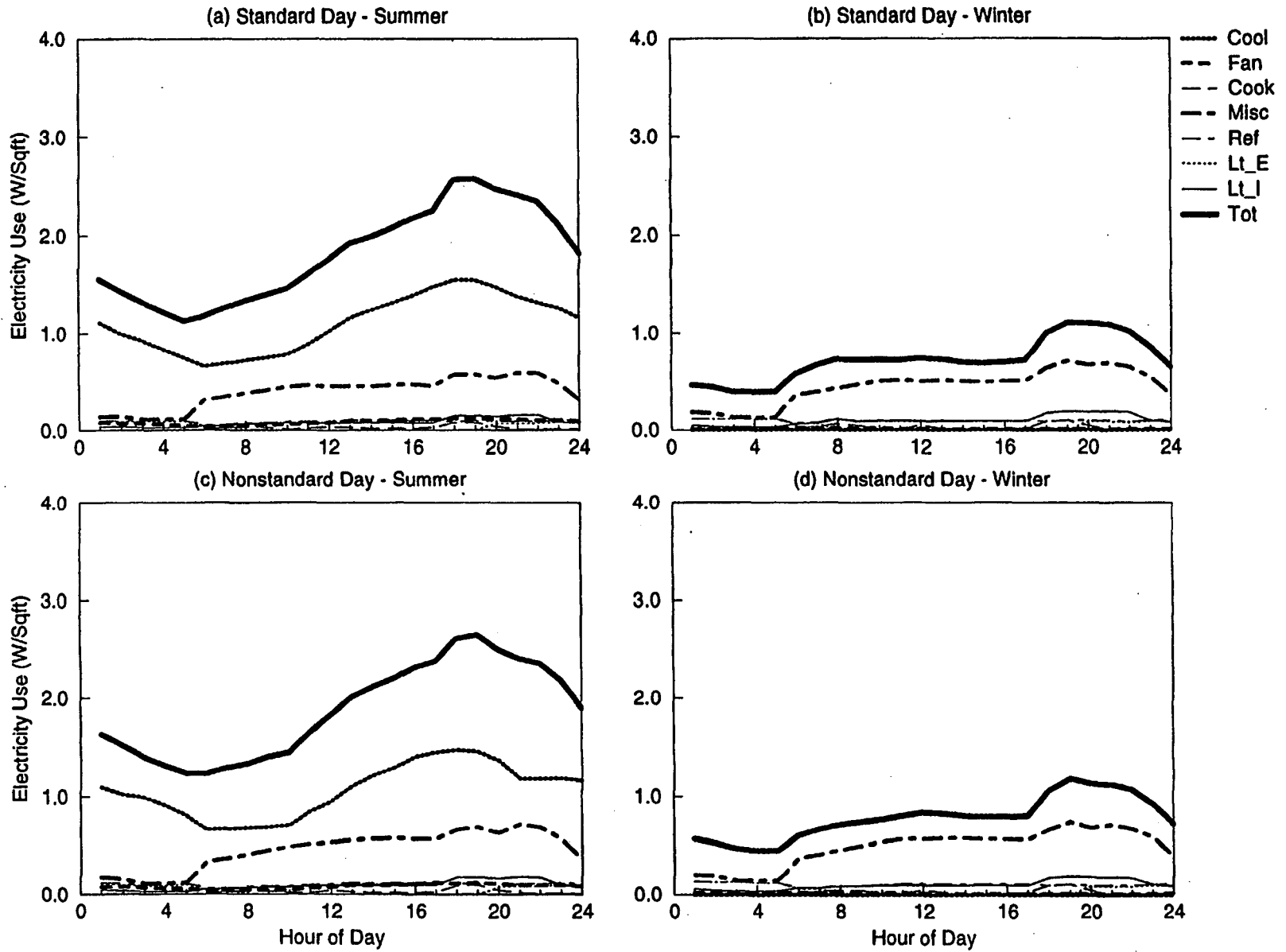
Figure C-50. EDA Reconciled End-use Load Shapes for Detached Residential (Feeder 5)
