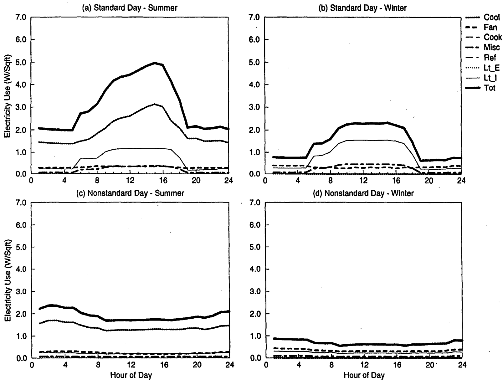
Figure C-27. EDA Reconciled End-use Load Shapes for Small Administration (Old w/ Split DX) (Weighted 2,10)
