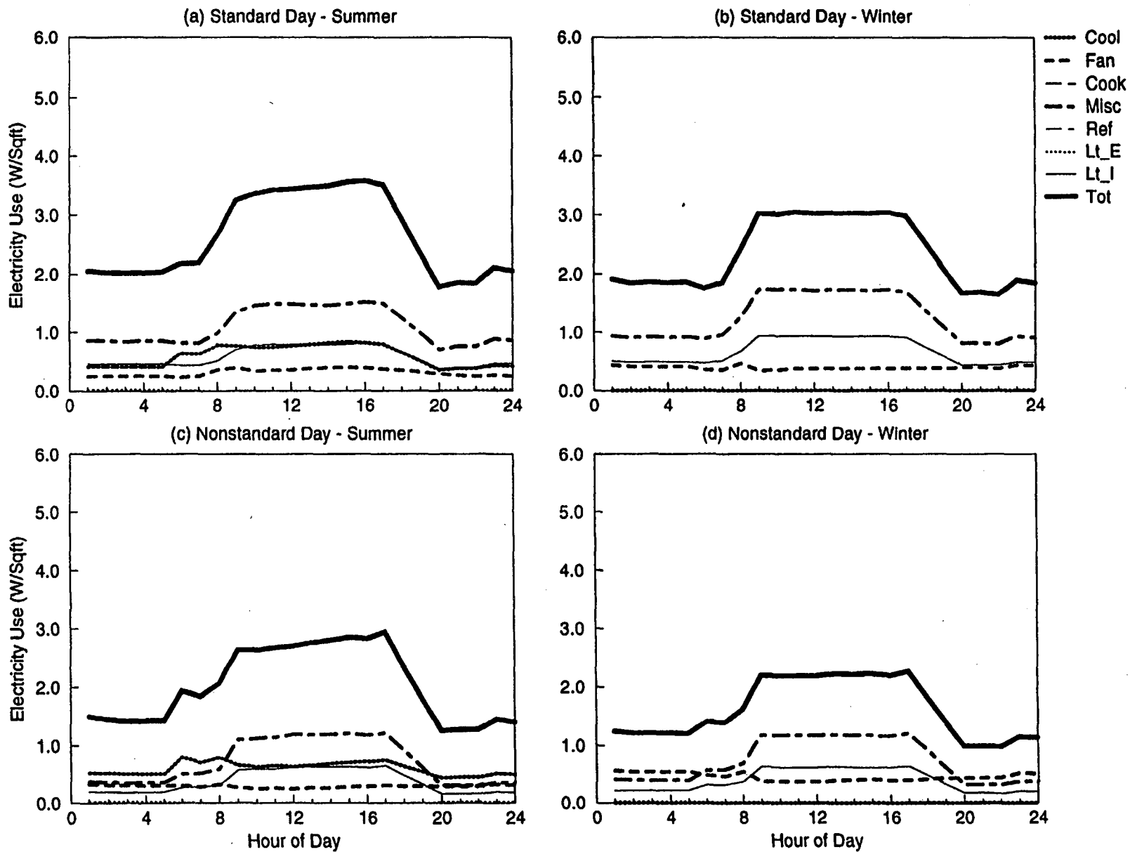
Figure C-23. EDA Reconciled End-use Load Shapes for Large Administration (Weighted 2,5)
