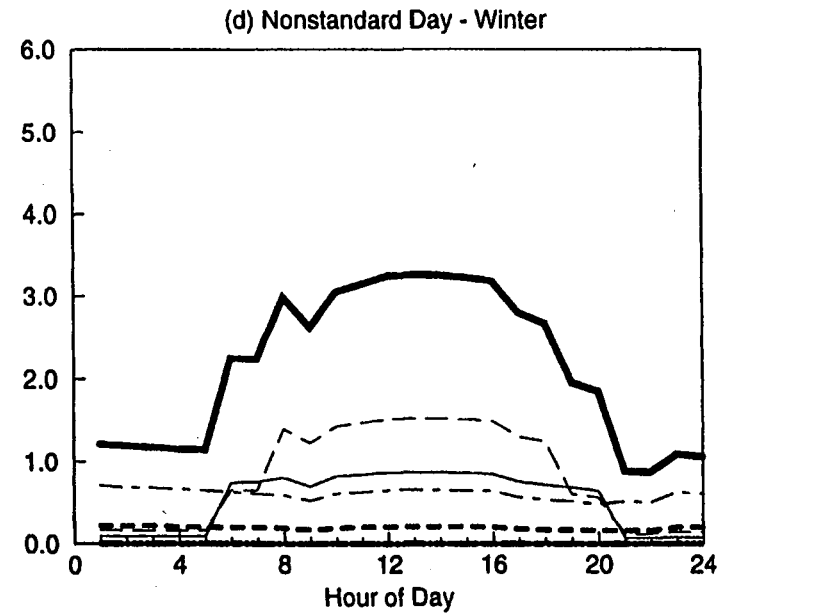
Figure C-16. EDA Reconciled End-use Load Shapes for Dining Hall (Feeder 10)
