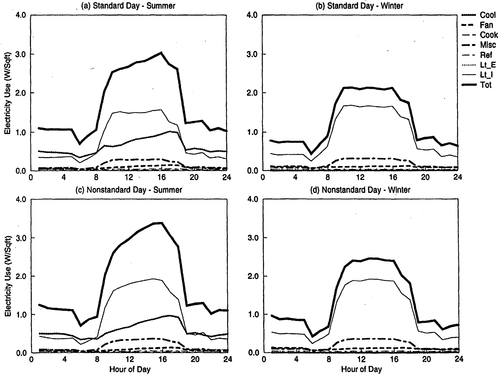
Figure C-67. EDA Reconciled End-use Load Shapes for Miscellaneous (Feeder 5)
