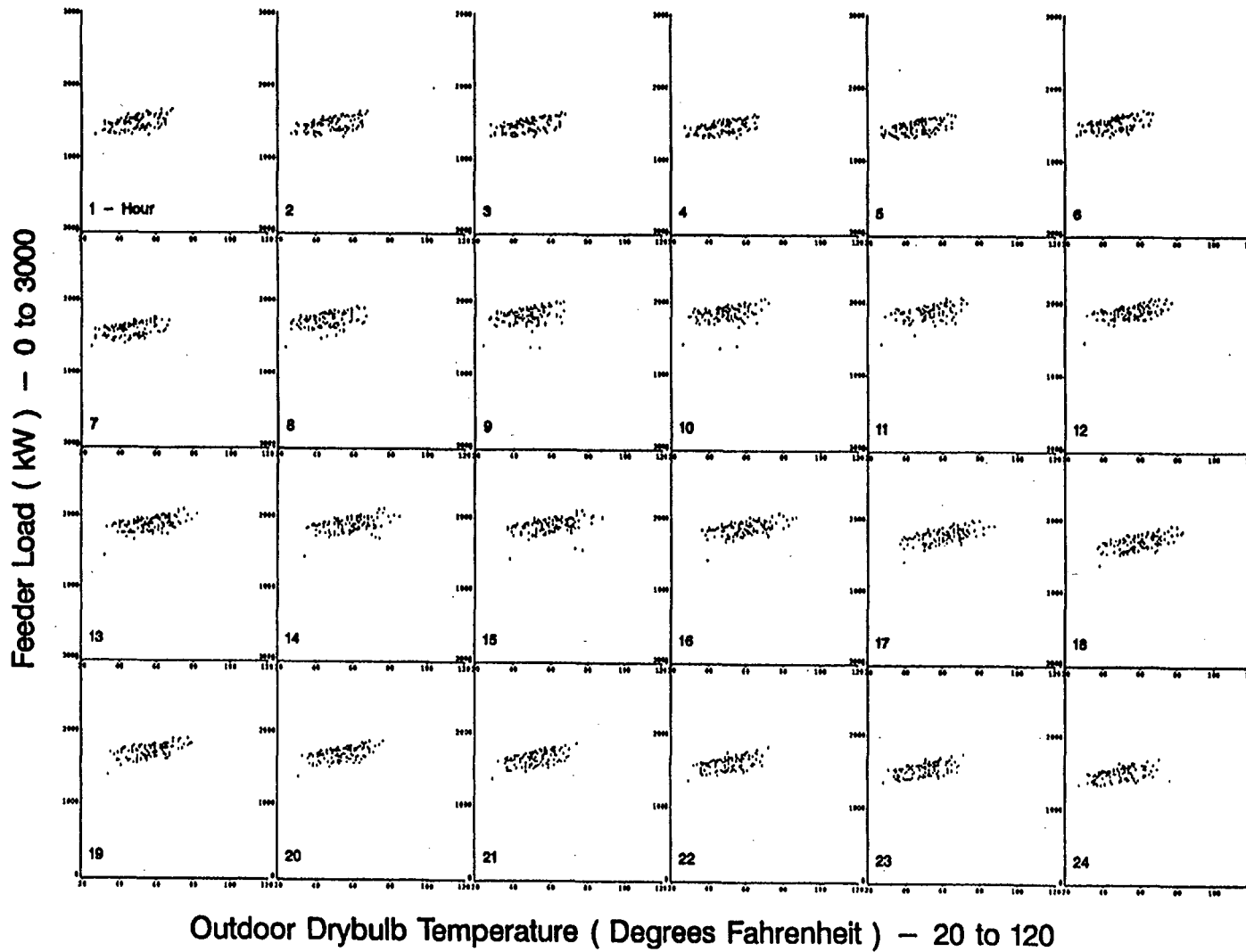
Figure A-22. Scatterplots of Feeder 9 Hourly Load vs. Drybulb Temperature for Standard Winter Days
