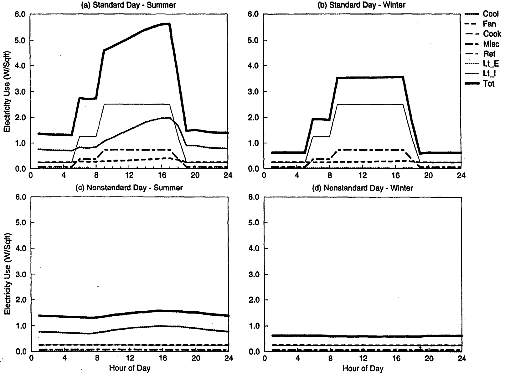
Figure B-10. DOE-2 Simulated End-use Load Shapes for Small Administration (New w/ Split DX)
