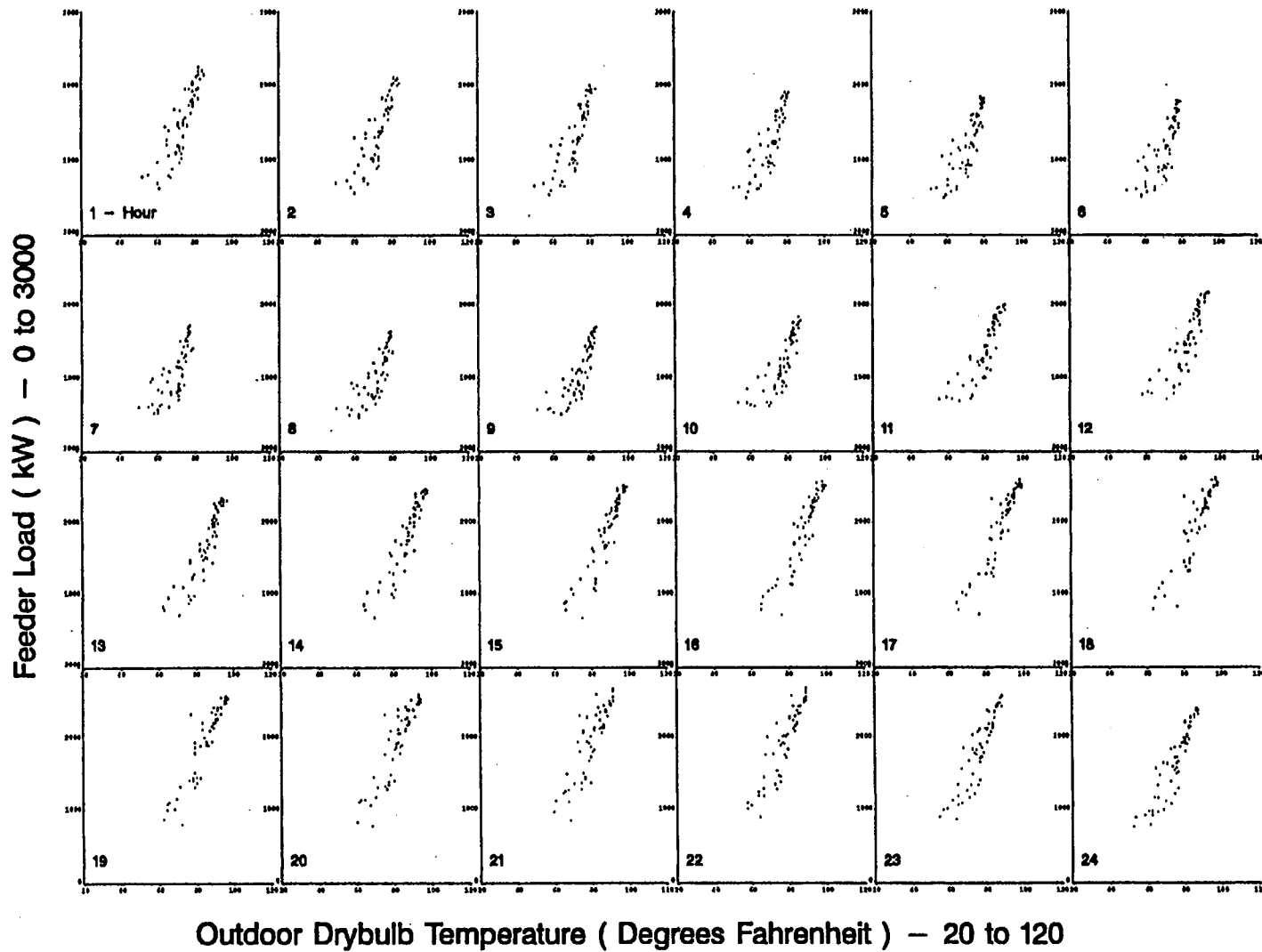
Figure A-35. Scatterplots of Feeder 12 Hourly Load vs. Drybulb Temperature for non-Standard Summer Days
