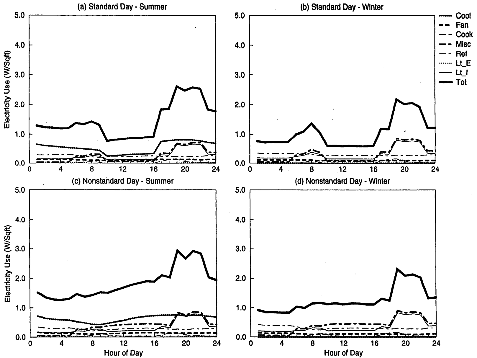
Figure C-9. EDA Reconciled End-use Load Shapes for Modular Barrack (Feeder 5)
