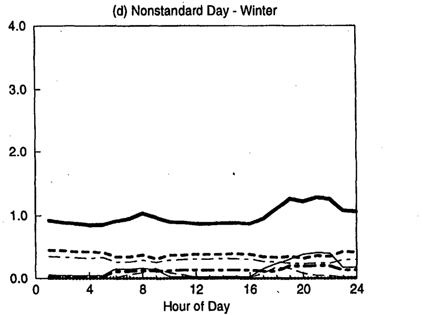
Figure C-7. EDA Reconciled End-use Load Shapes for Rolling Pin Barrack (Weighted 3,10)
