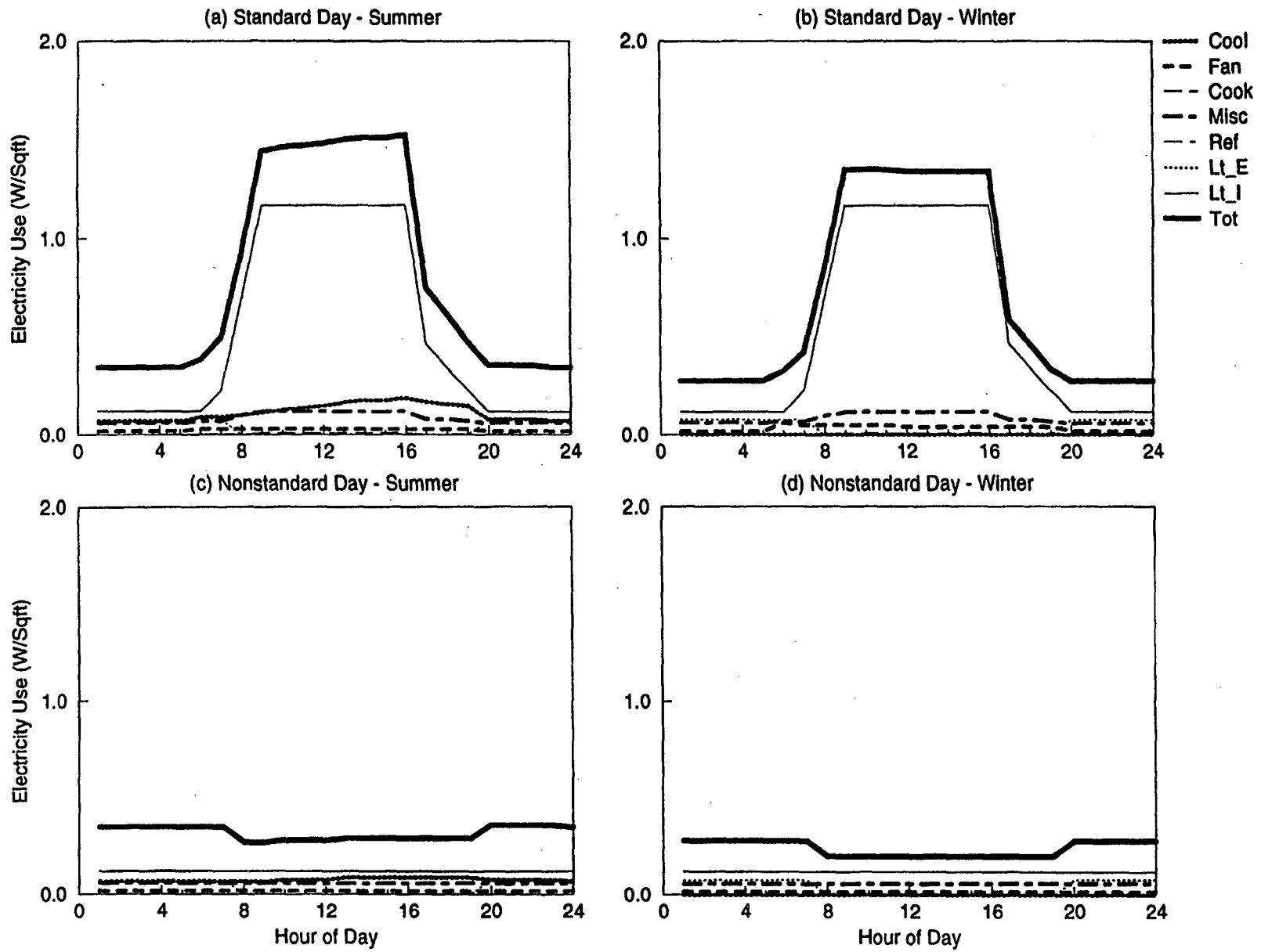
Figure B-13. DOE-2 Simulated End-use Load Shapes for Large Vehicle Maintenance (Split DX)
