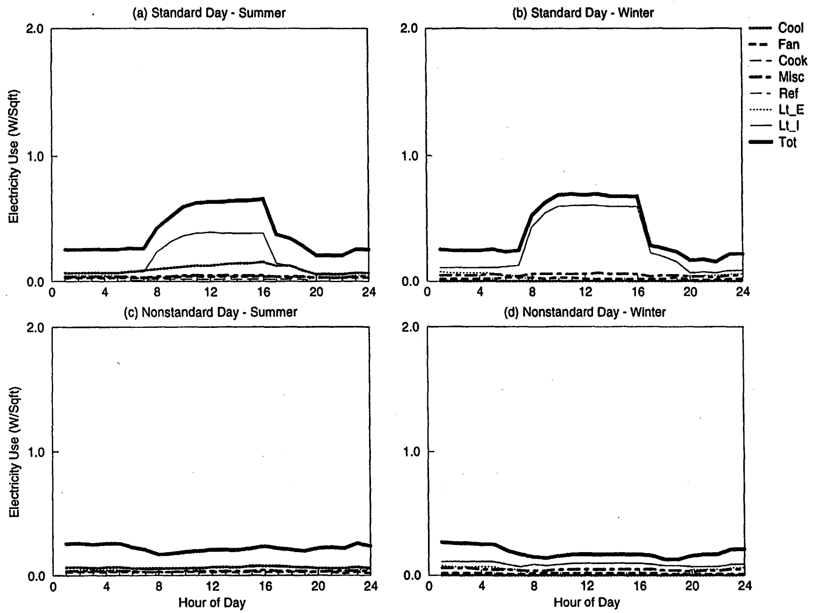
Figure C-41. EDA Reconciled End-use Load Shapes for Large Vehicle Maintenance (Split DX) (Feeder 3)
