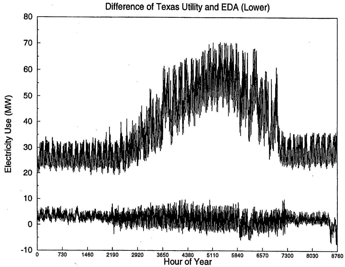
Figure 4-1. EDA Annual Hourly Electricity Use (Upper) Difference of Texas Utility and EDA (Lower)
