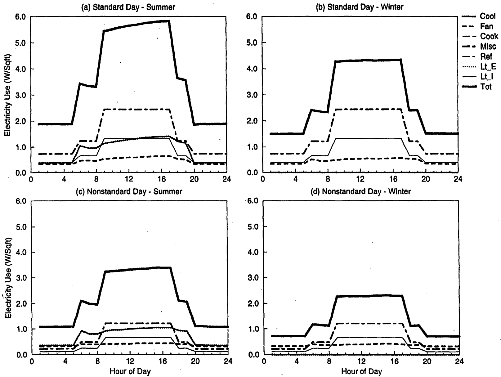
Figure B-7. DOE-2 Simulated End-use Load Shapes for Large Administration
