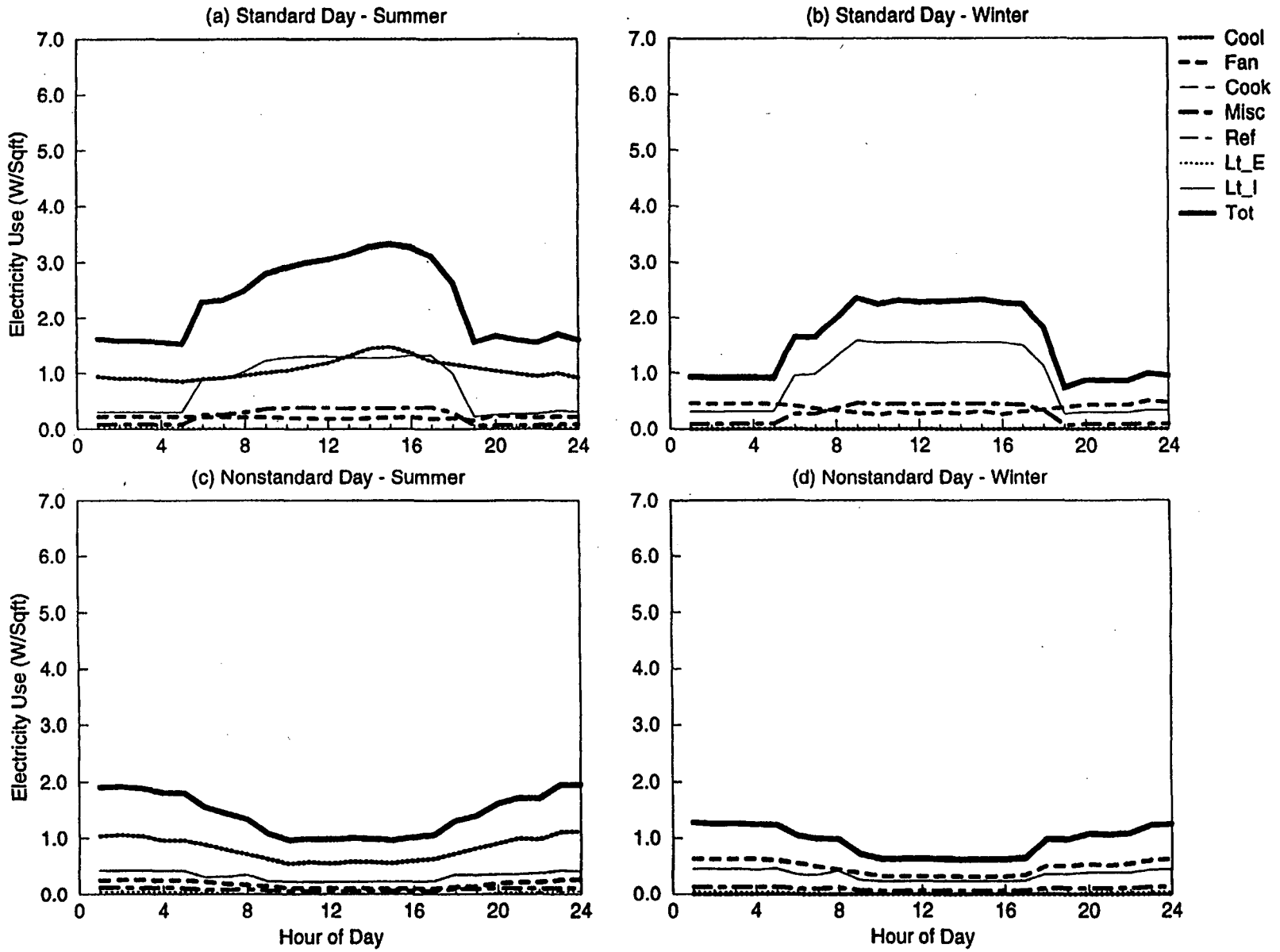
Figure C-24. EDA Reconciled End-use Load Shapes for Small Administration (Old w/ Split DX) (Feeder 2)
