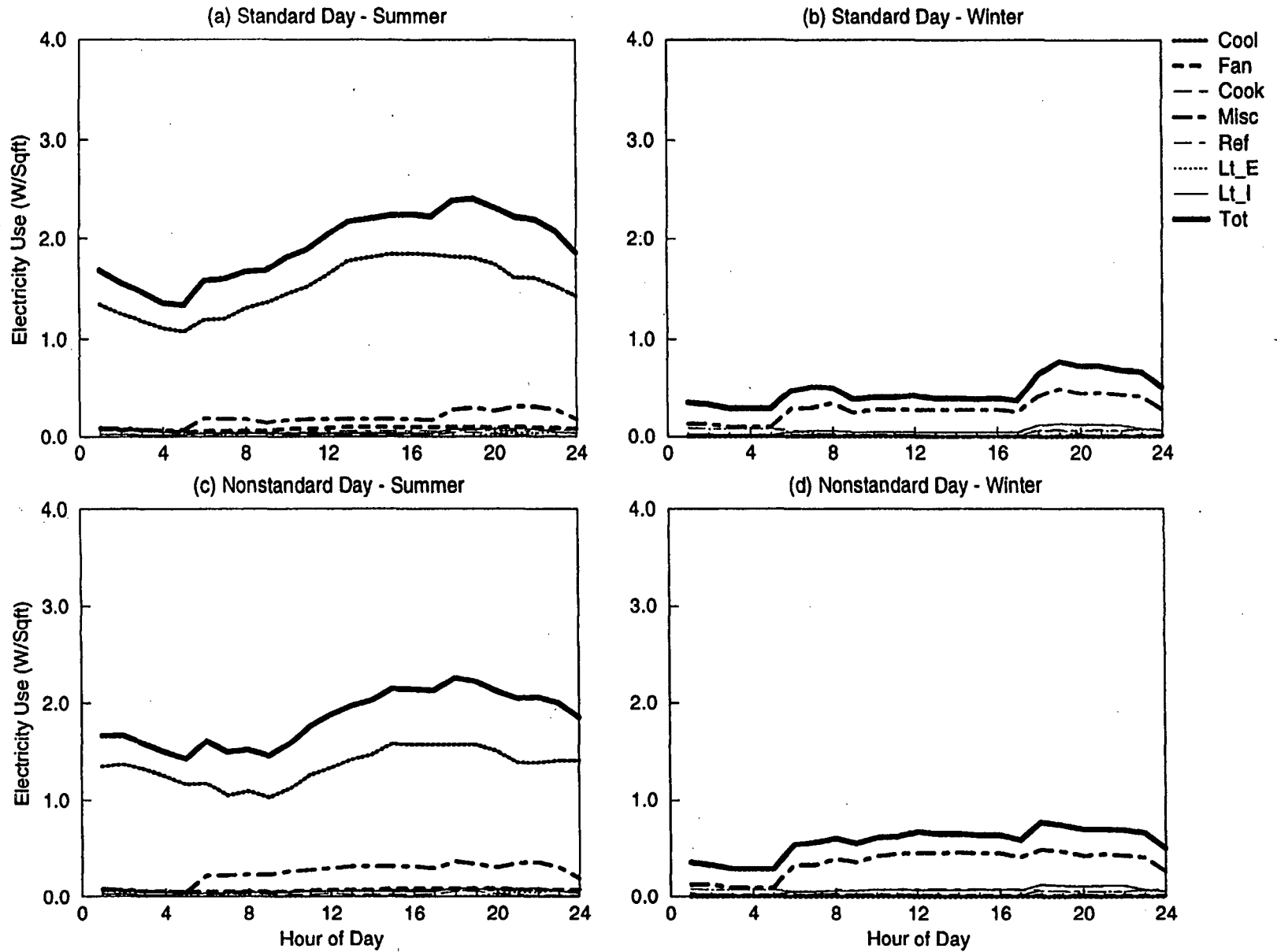
Figure C-59. EDA Reconciled End-use Load Shapes for Four-Plex Residential (Feeder 3)
