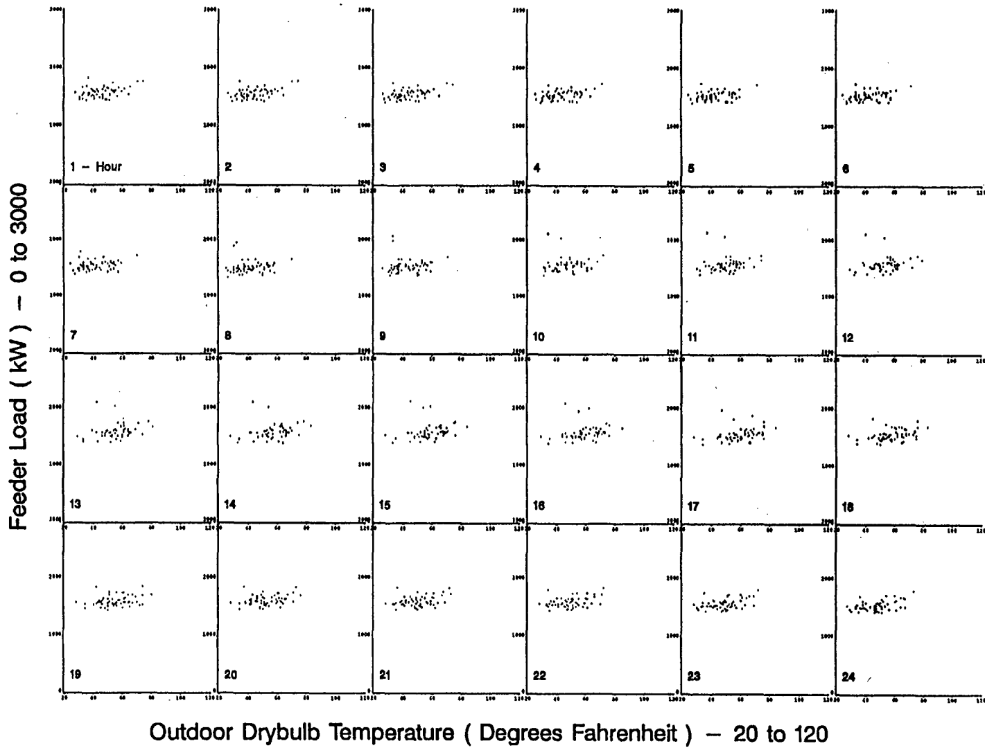
Figure A-3. Scatterplots of Feeder 2 Hourly Load vs. Drybulb Temperature for non-Standard Winter Days
