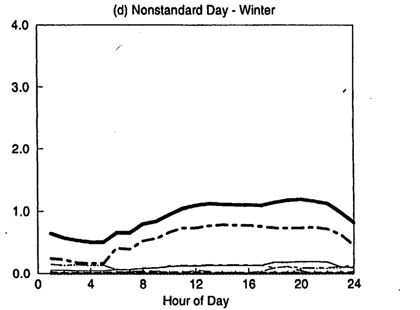
Figure C-60. EDA Reconciled End-use Load Shapes for Four-Plex Residential (Feeder 12)
