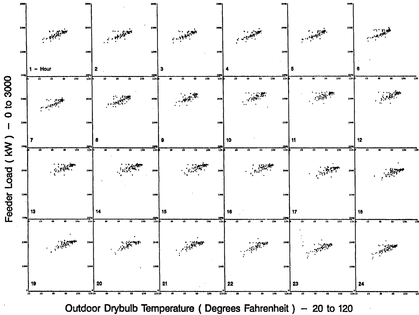
Figure A-24. Scatterplots of Feeder 9 Hourly Load vs. Drybulb Temperature for Standard Summer Days
