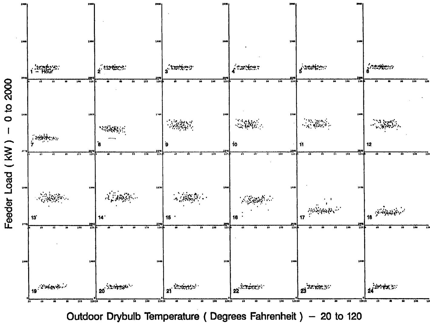
Figure A-52. Scatterplots of Feeder W6 Hourly Load vs. Drybulb Temperature for Standard Winter Days
