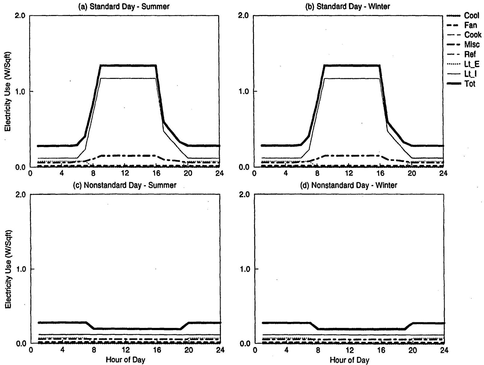
Figure B-21. DOE-2 Simulated End-use Load Shapes for Warehouse (No AC)
