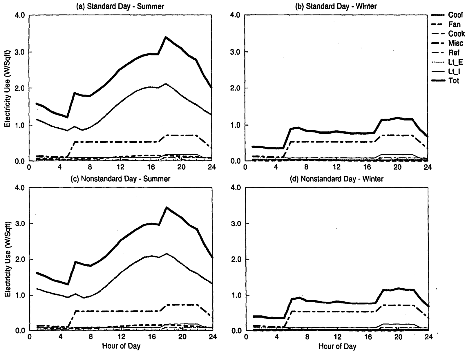
Figure B-17. DOE-2 Simulated End-use Load Shapes for Detached Residential
