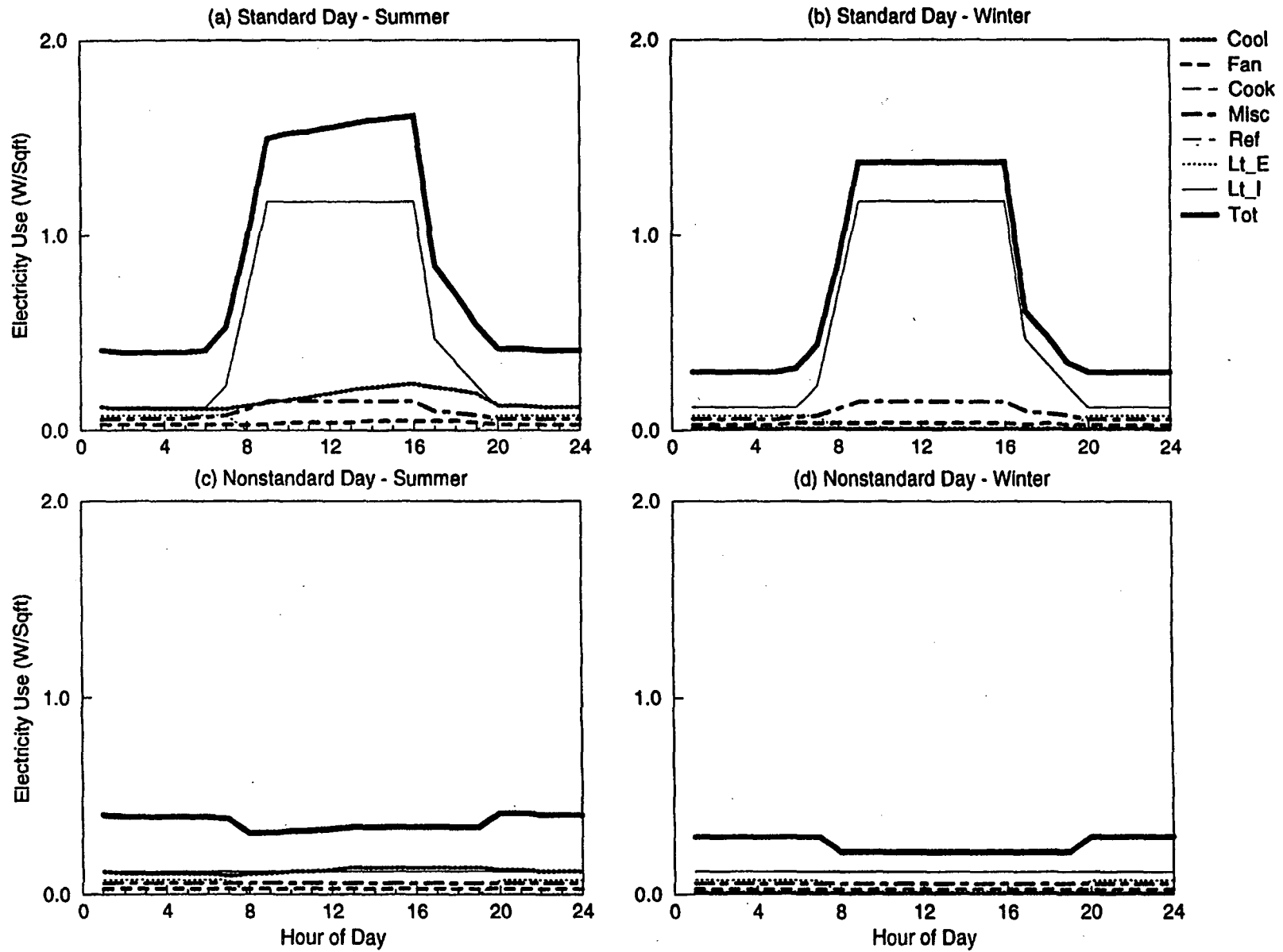
Figure B-22. DOE-2 Simulated End-use Load Shapes for Warehouse (Split DX)
