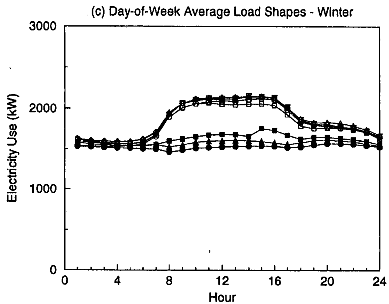
Figure 3-3. Feeder 2 Data
