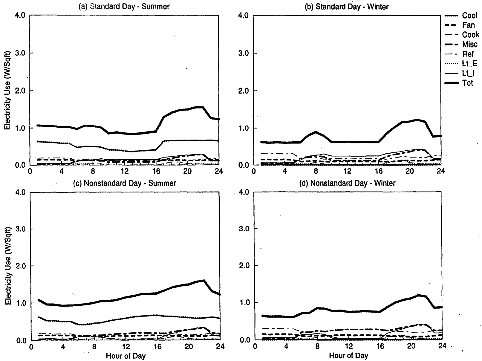
Figure C-1. EDA Reconciled End-use Load Shapes for Hammerhead Barrack (Feeder 3)
