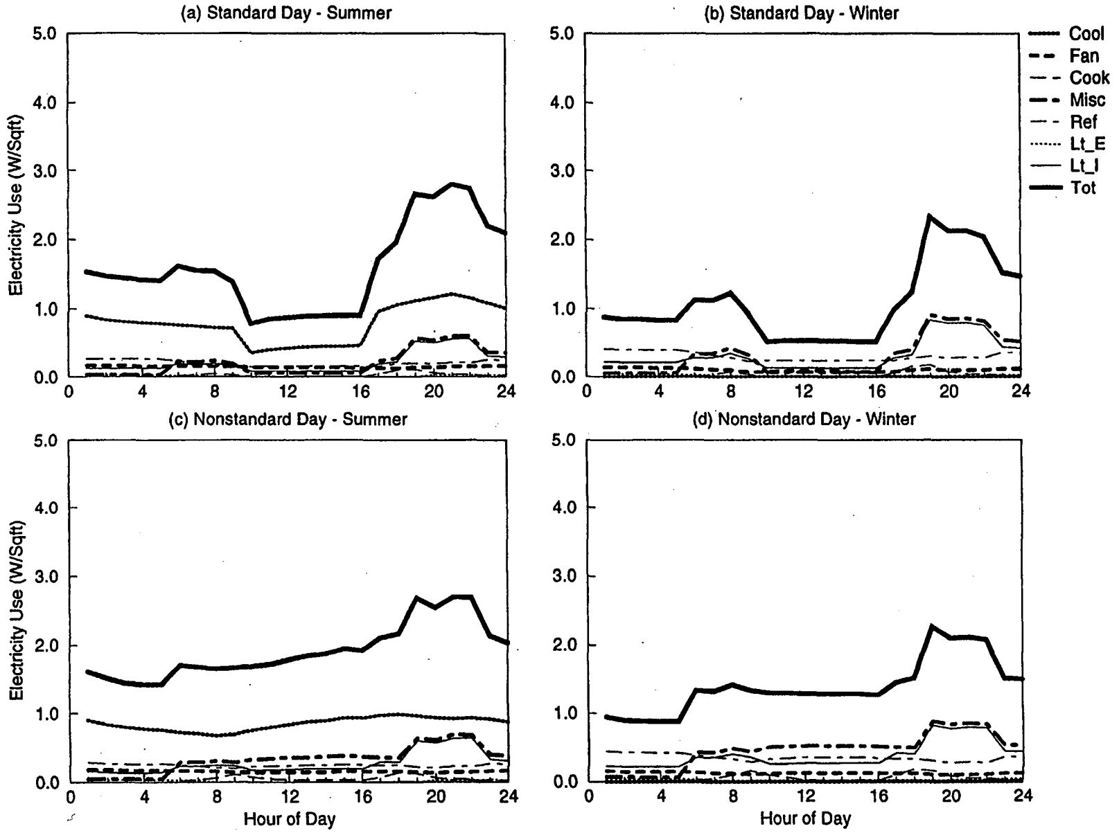
Figure C-12. EDA Reconciled End-use Load Shapes for Modular Barrack (Weighted 2,5,15)
