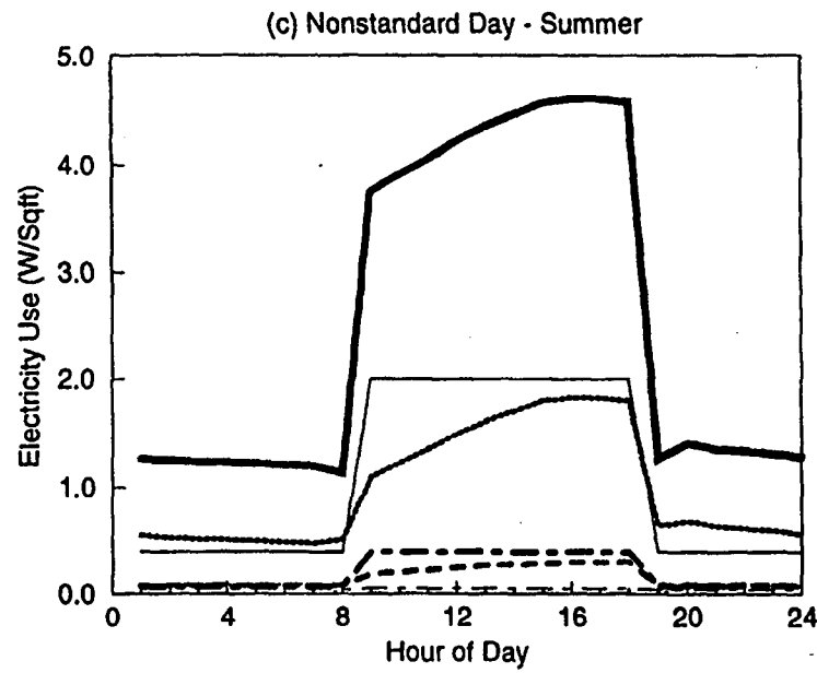
Figure B-29. DOE-2 Simulated End-use Load Shapes for Small Retail
