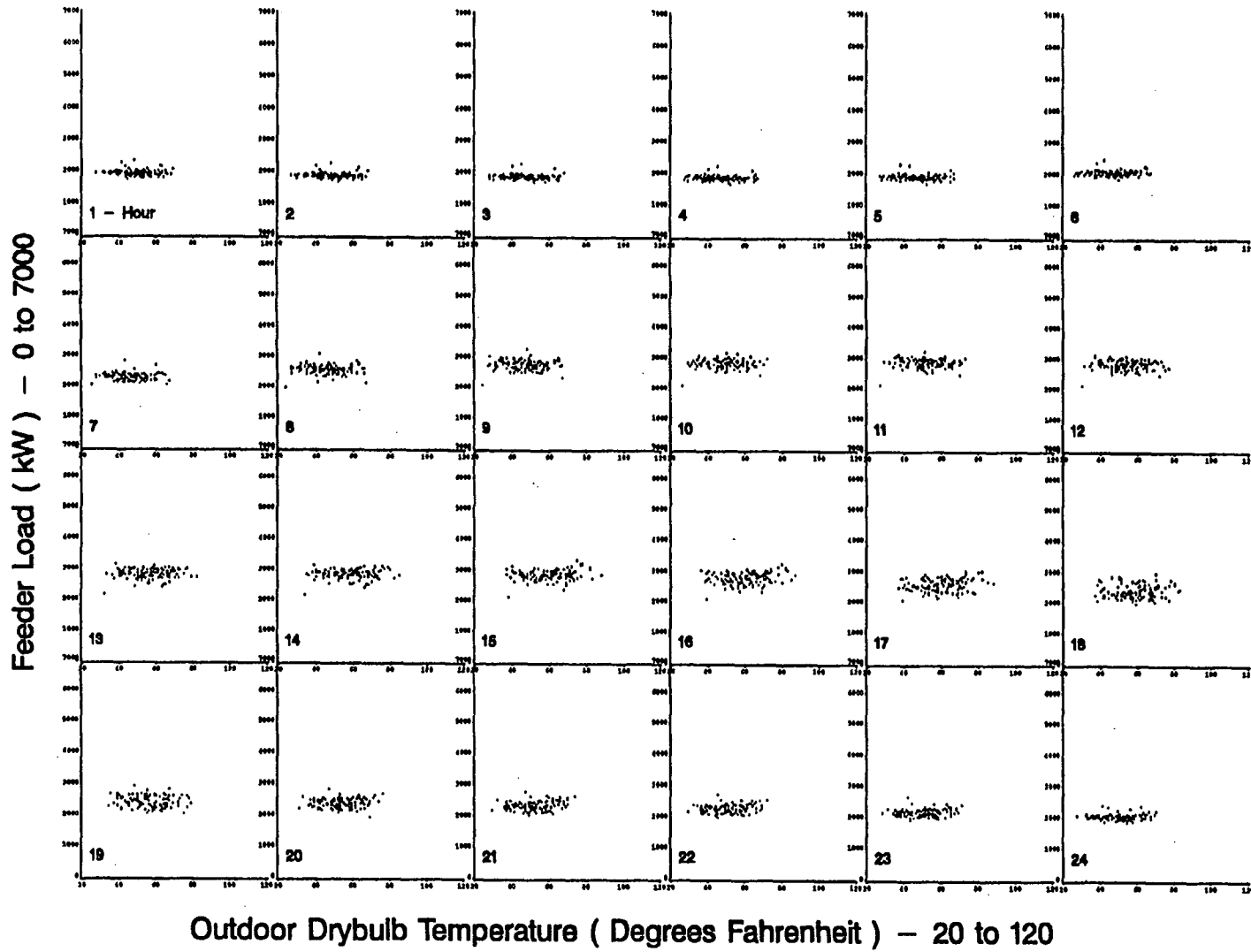
Figure A-27. Scatterplots of Feeder 10 Hourly Load vs. Drybulb Temperature for Standard Winter Days
