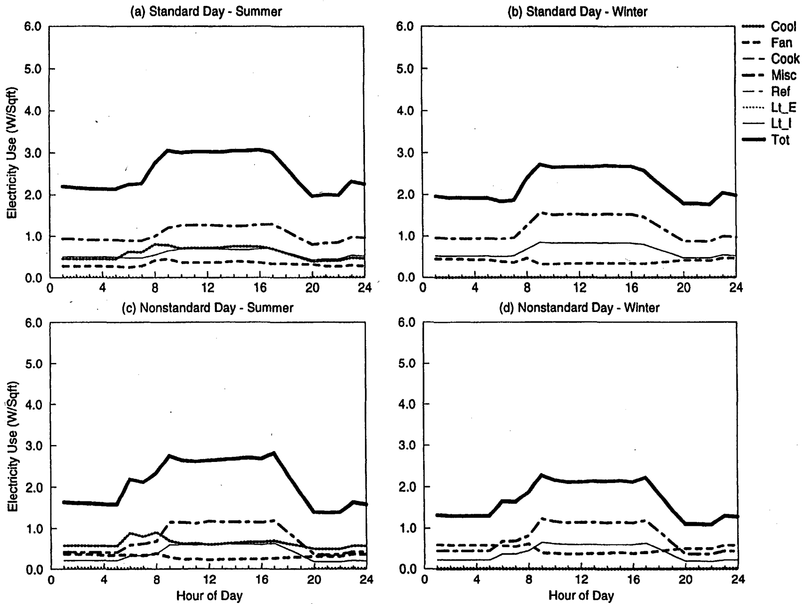
Figure C-21. EDA Reconciled End-use Load Shapes for Large Administration (Feeder 2)
