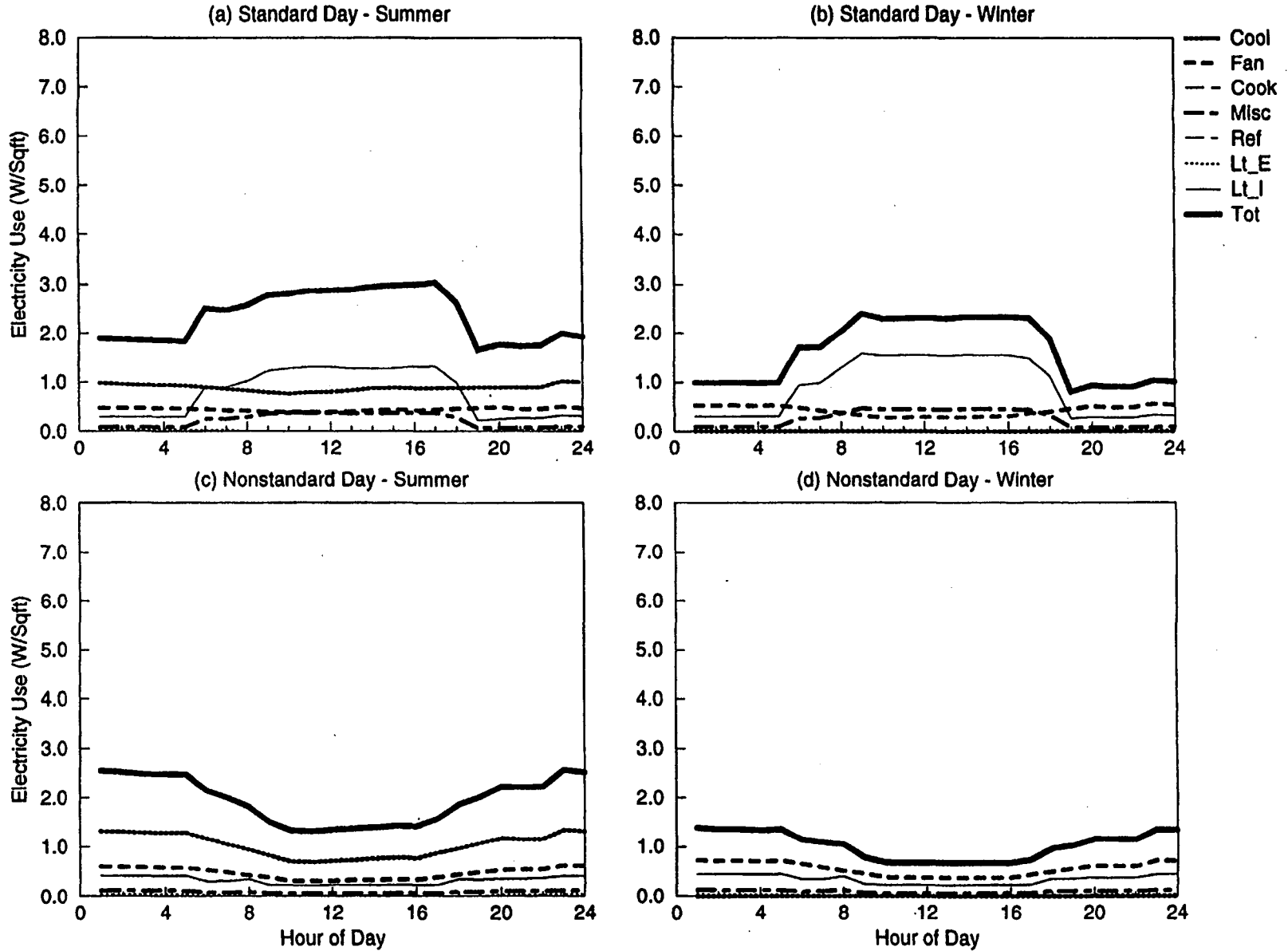
Figure C-36. EDA Reconciled End-use Load Shapes for Small Administration (New w/ Chiller) (Feeder 2)
