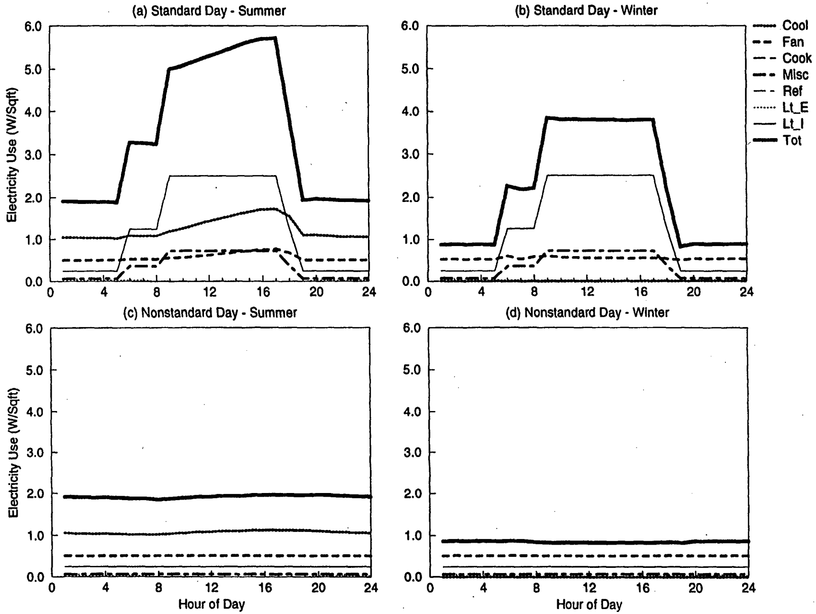
Figure B-9. DOE-2 Simulated End-use Load Shapes for Small Administration (Old w/ Chiller)
