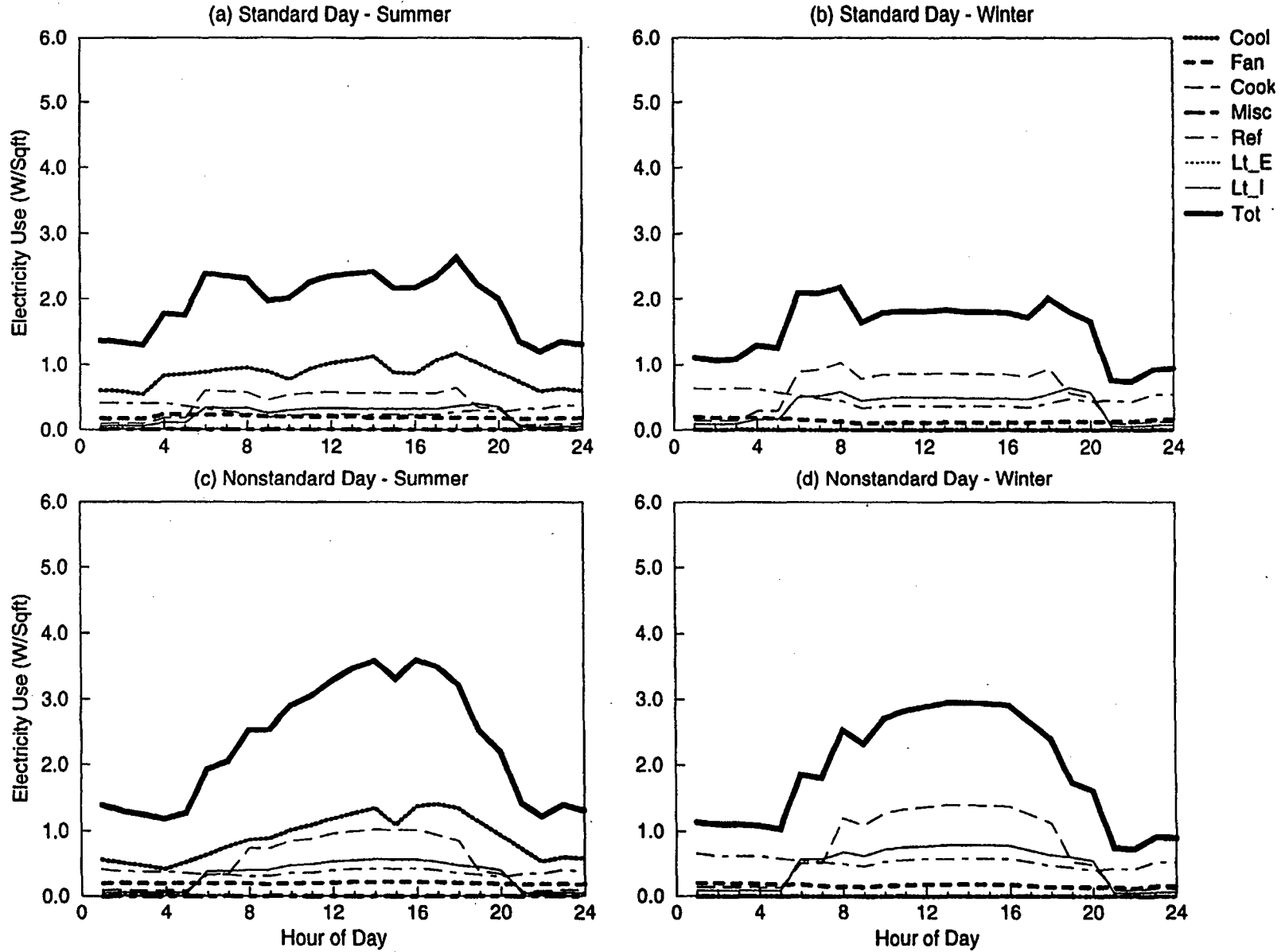
Figure C-14. EDA Reconciled End-use Load Shapes for Dining Hall (Feeder 3)
