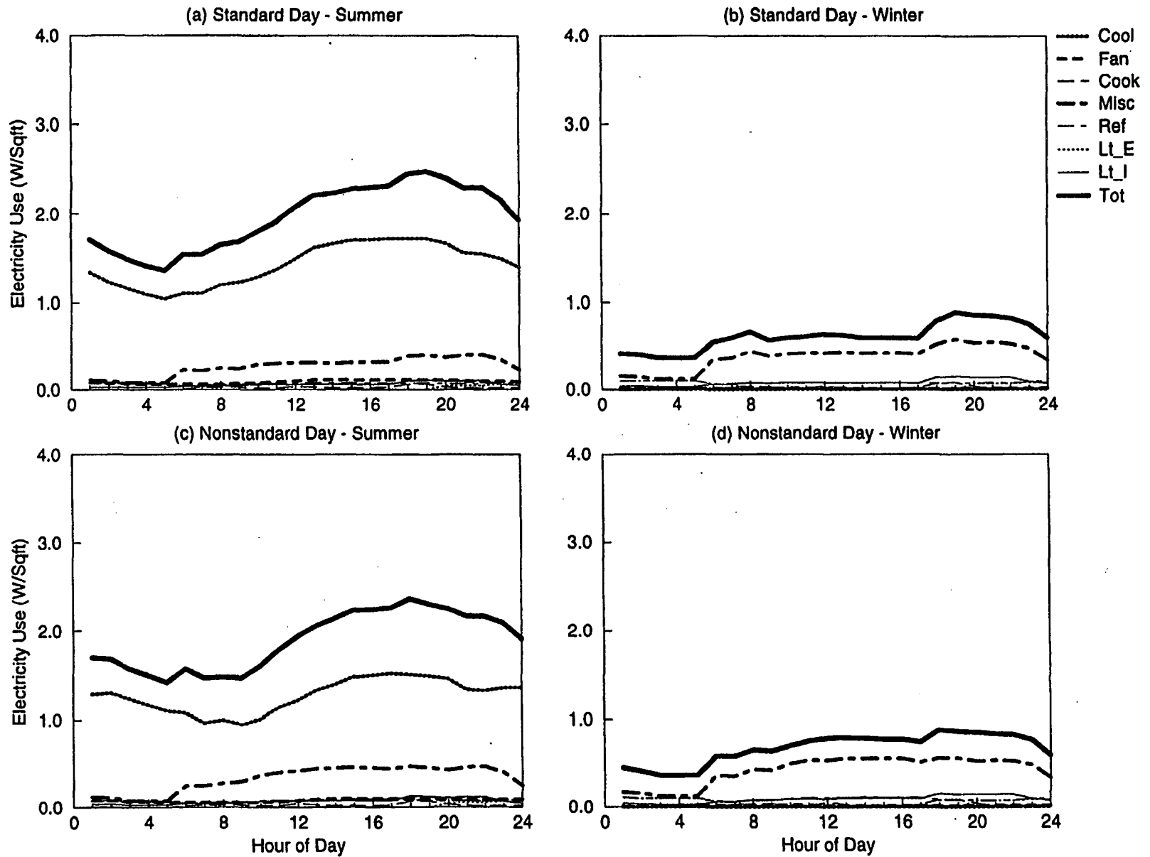
Figure C-61. EDA Reconciled End-use Load Shapes for Four-Plex Residential (Weighted 3,12)
