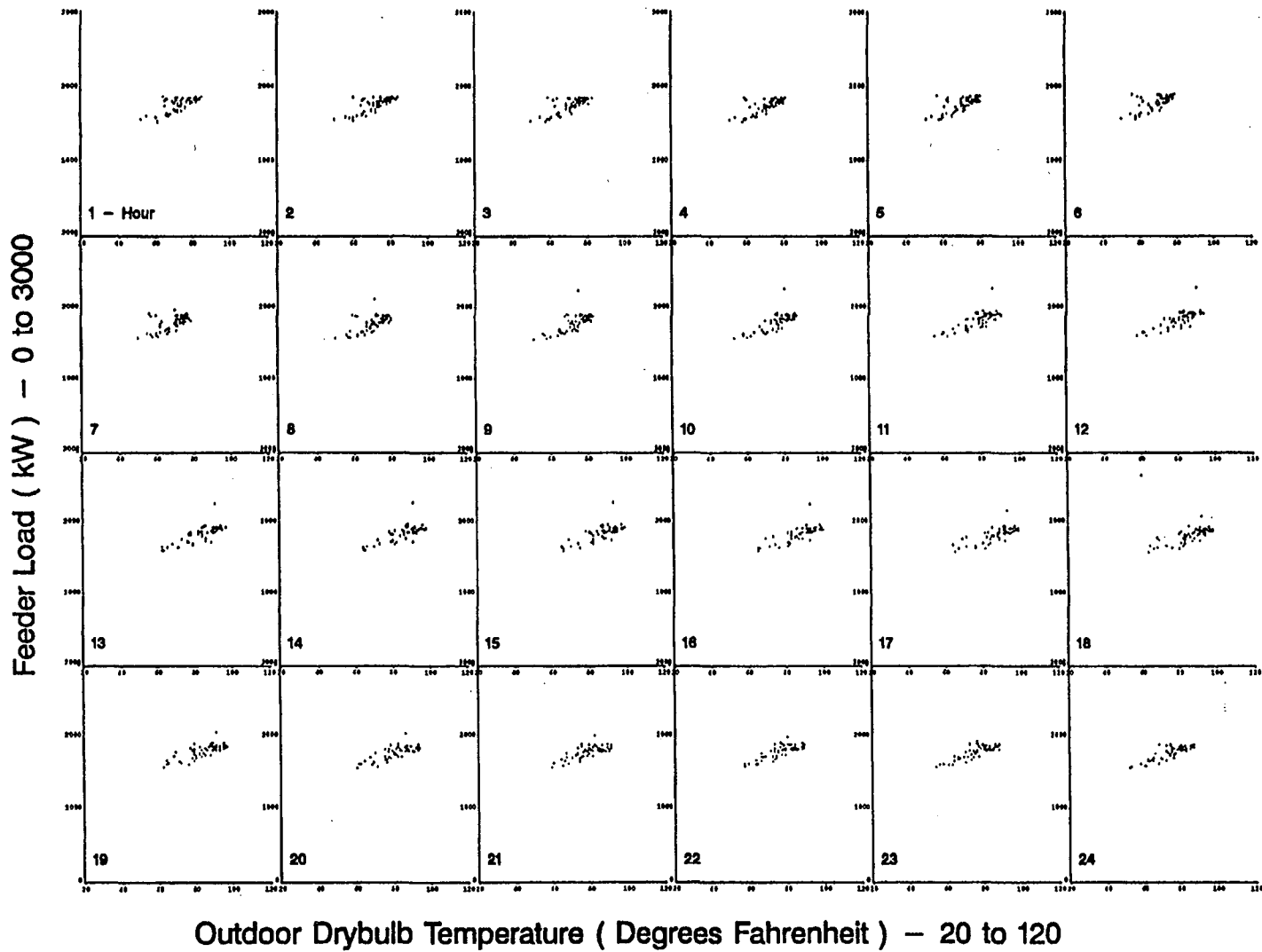
Figure A-25. Scatterplots of Feeder 9 Hourly Load vs. Drybulb Temperature for non-Standard Summer Days
