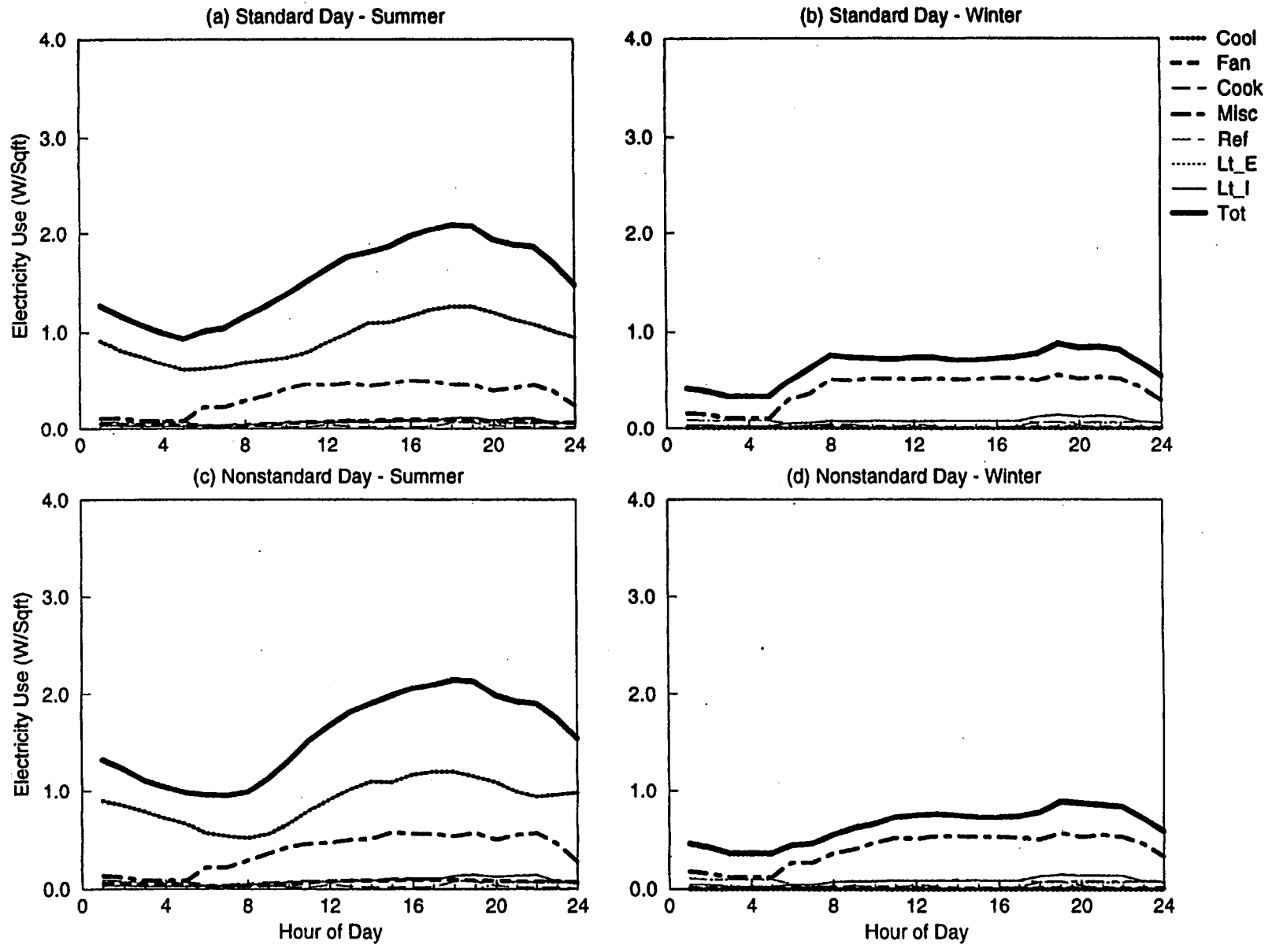
Figure C-56. EDA Reconciled End-use Load Shapes for Two-Plex Residential (Feeder W4)
