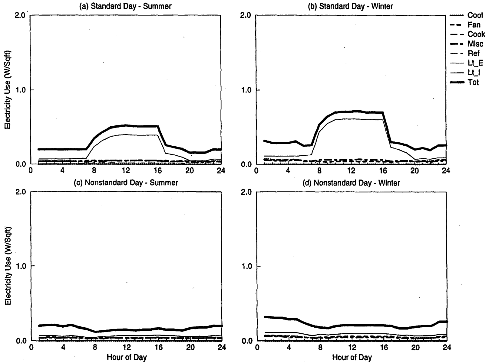
Figure C-38. EDA Reconciled End-use Load Shapes for Small Vehicle Maintenance (No AC) (Feeder 3)
