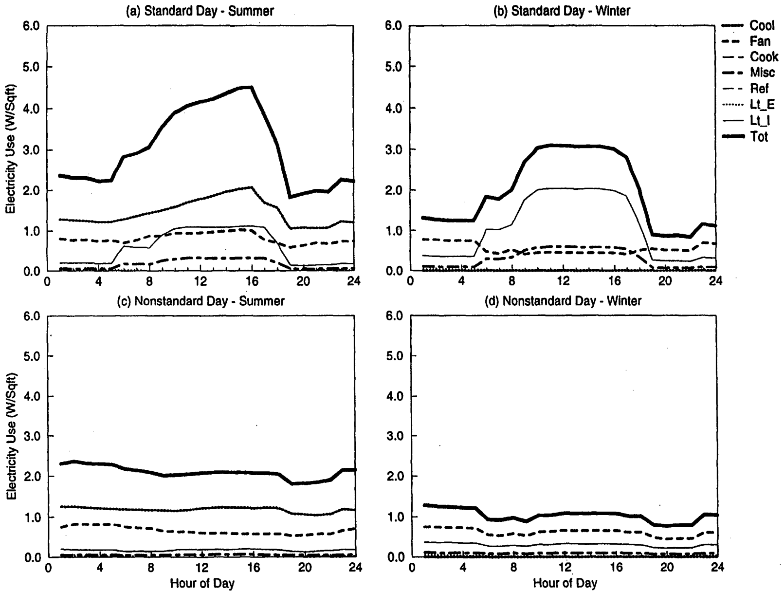
Figure C-31. EDA Reconciled End-use Load Shapes for Small Administration (Old w/ Chiller) (Feeder 15)
