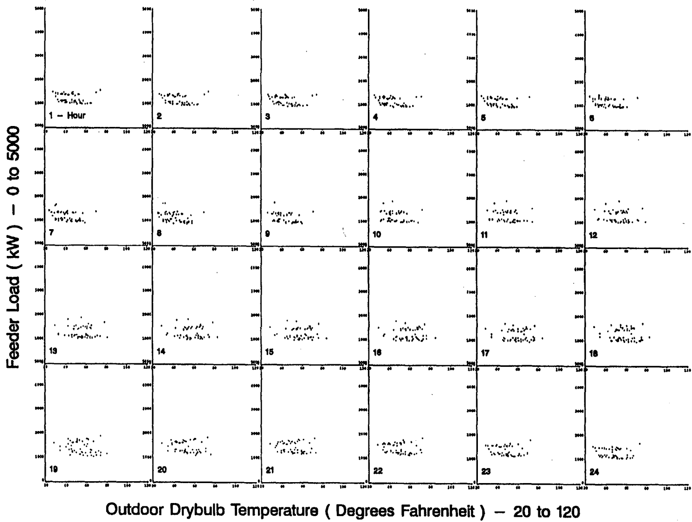
Figure A-8. Scatterplots of Feeder 3 Hourly Load vs. Drybulb Temperature for non-Standard Winter Days
