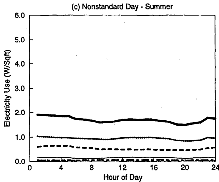
Figure C-32. EDA Reconciled End-use Load Shapes for Small Administration (Old w/ Chiller) (Weighted 3,10,15)
