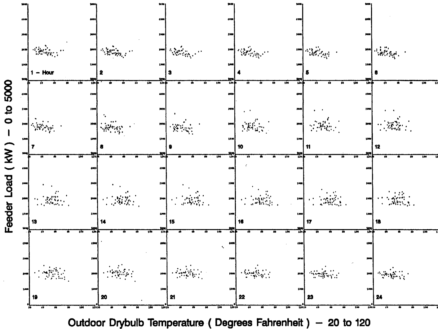
Figure A-38. Scatterplots of Feeder 15 Hourly Load vs. Drybulb Temperature for non-Standard Winter Days
