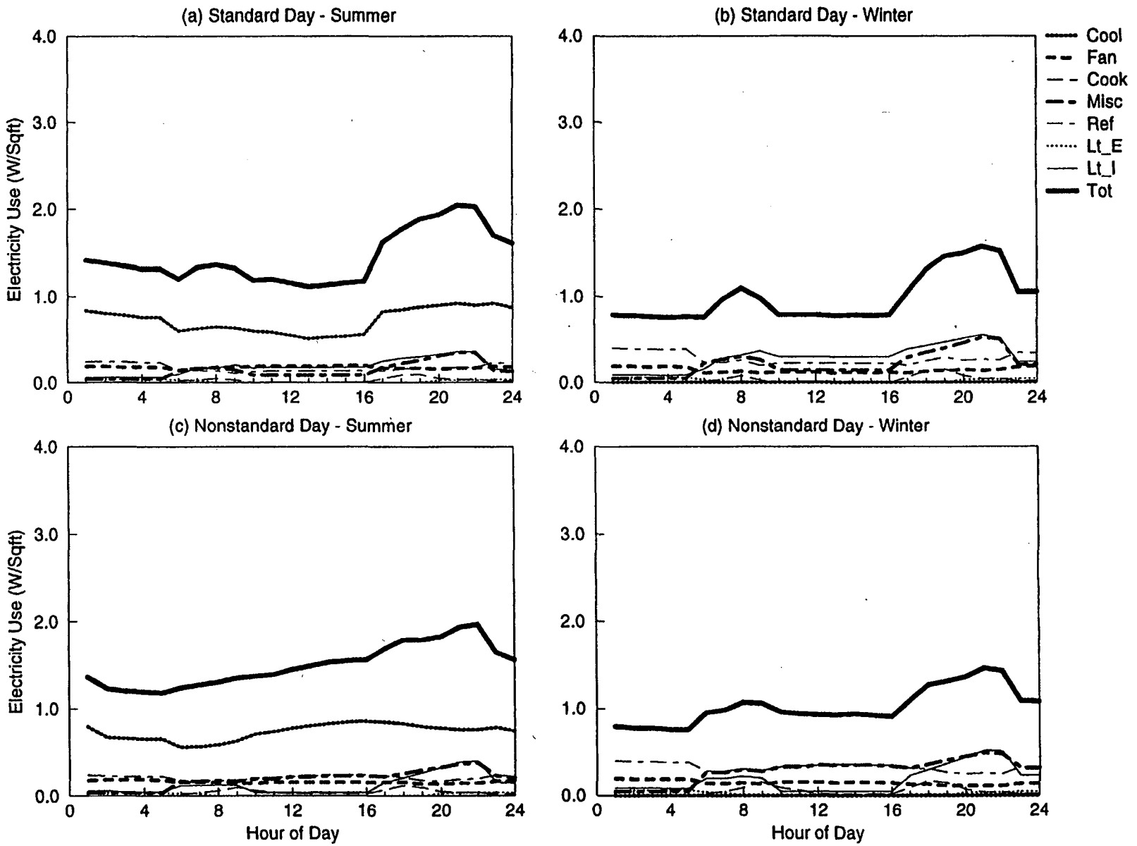
Figure C-4. EDA Reconciled End-use Load Shapes for Hammerhead Barrack (Weighted 3,10,15)
