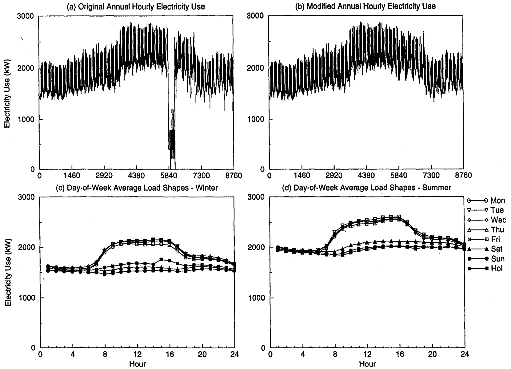
Figure A-1. Feeder 2 Data
