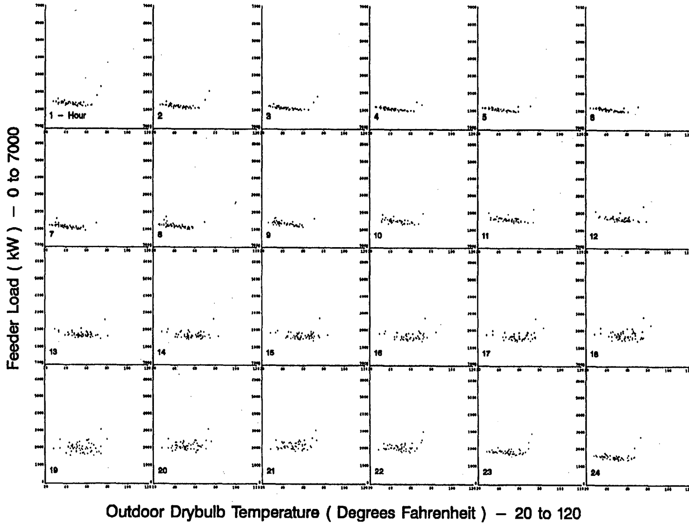
Figure A-43. Scatterplots of Feeder W4 Hourly Load vs. Drybulb Temperature for non-Standard Winter Days
