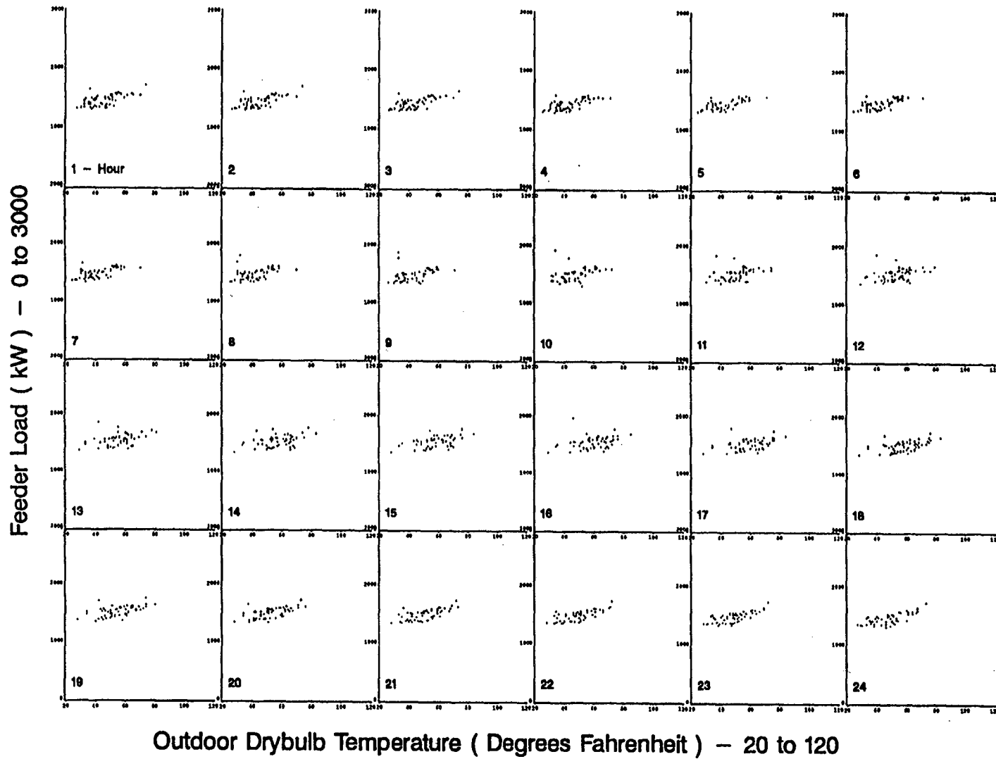
Figure A-23. Scatterplots of Feeder 9 Hourly Load vs. Drybulb Temperature for non-Standard Winter Days
