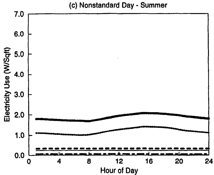
Figure B-8. DOE-2 Simulated End-use Load Shapes for Small Administration (Old w/ Split DX)
