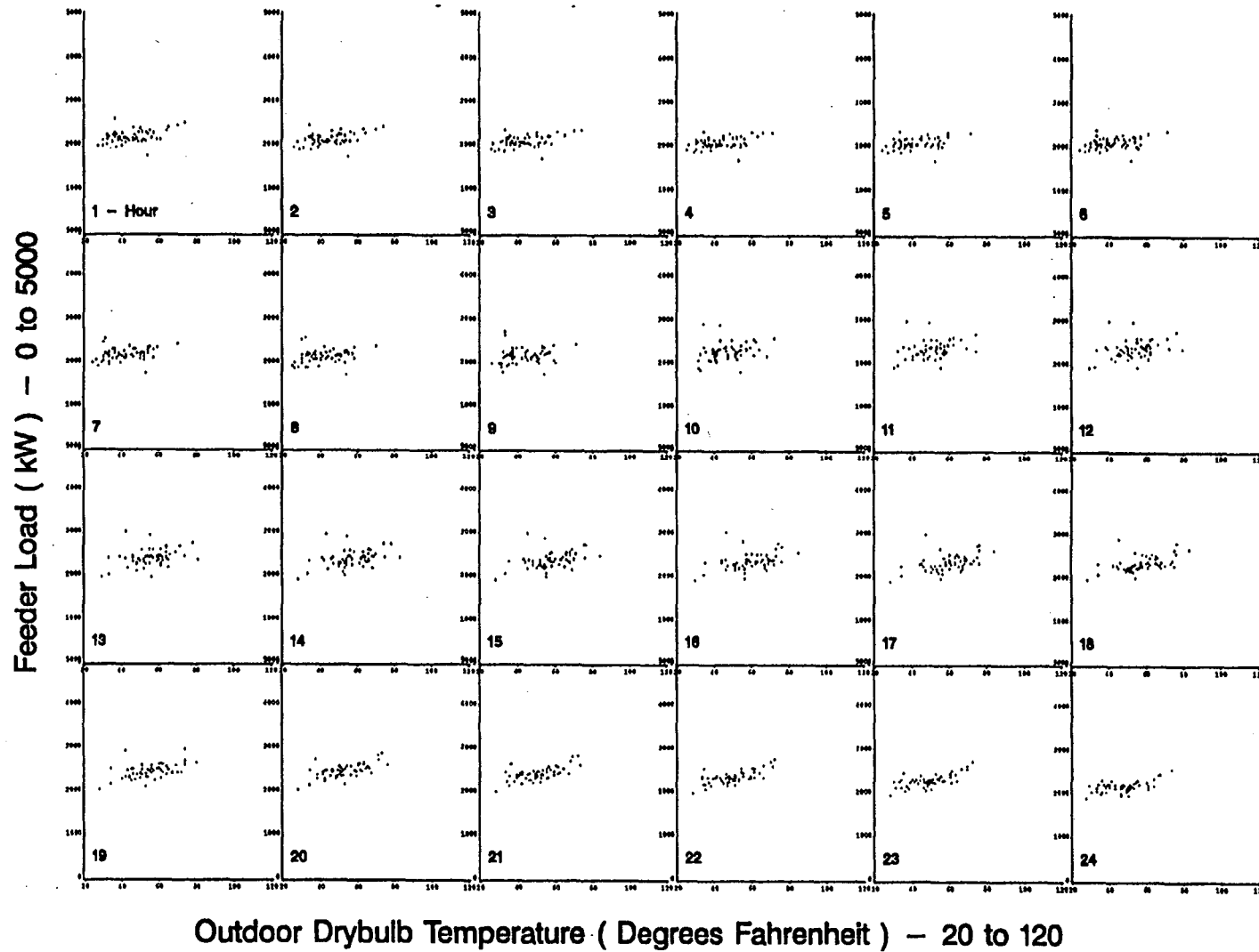
Figure A-48. Scatterplots of Feeder W5 Hourly Load vs. Drybulb Temperature for non-Standard Winter Days
