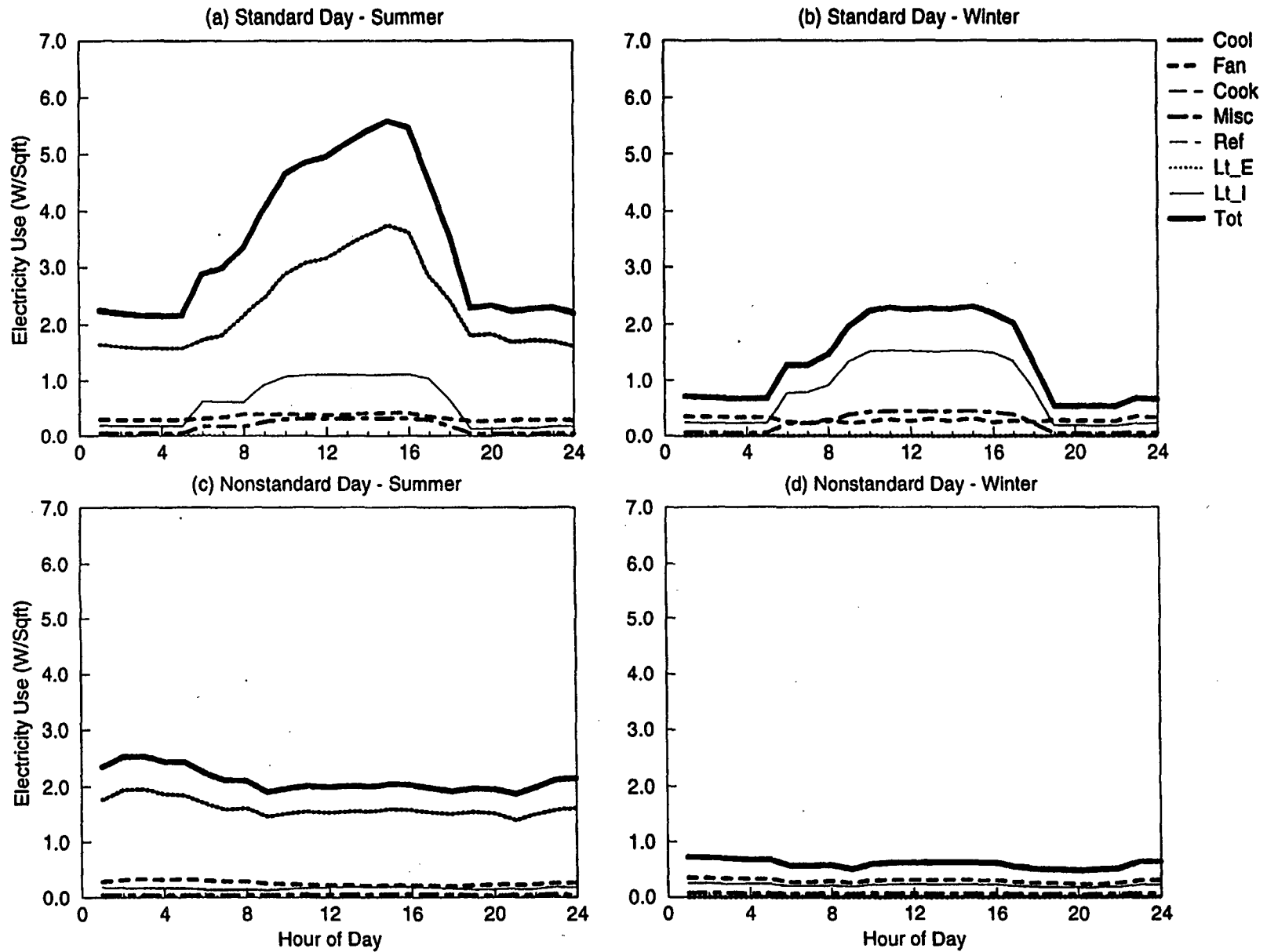
Figure C-25. EDA Reconciled End-use Load Shapes for Small Administration (Old w/ Split DX) (Feeder 10)
