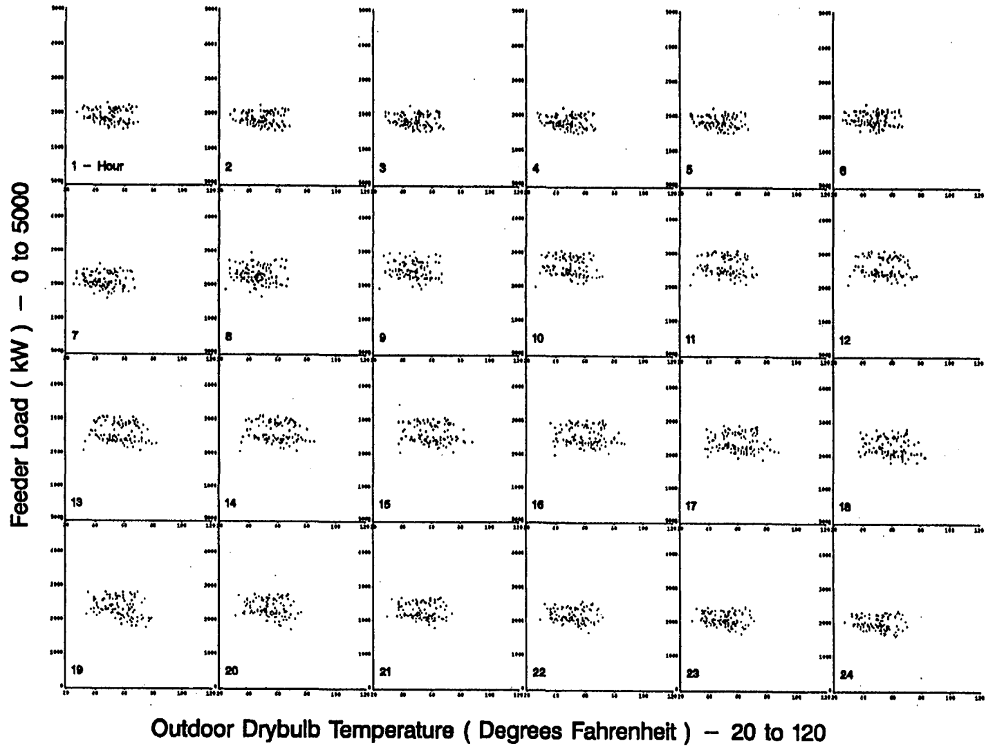
Figure A-37. Scatterplots of Feeder 15 Hourly Load vs. Drybulb Temperature for Standard Winter Days
