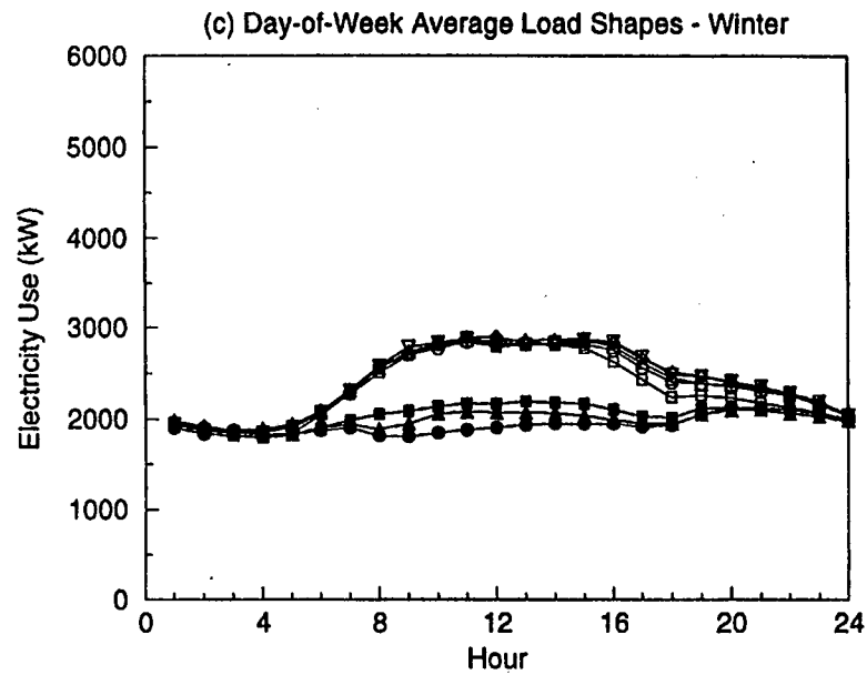
Figure A-26. Feeder 10 Data
