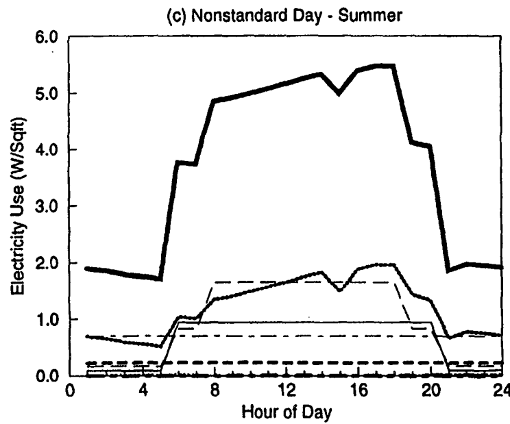
Figure B-5. DOE-2 Simulated End-use Load Shapes for Dining Hall
