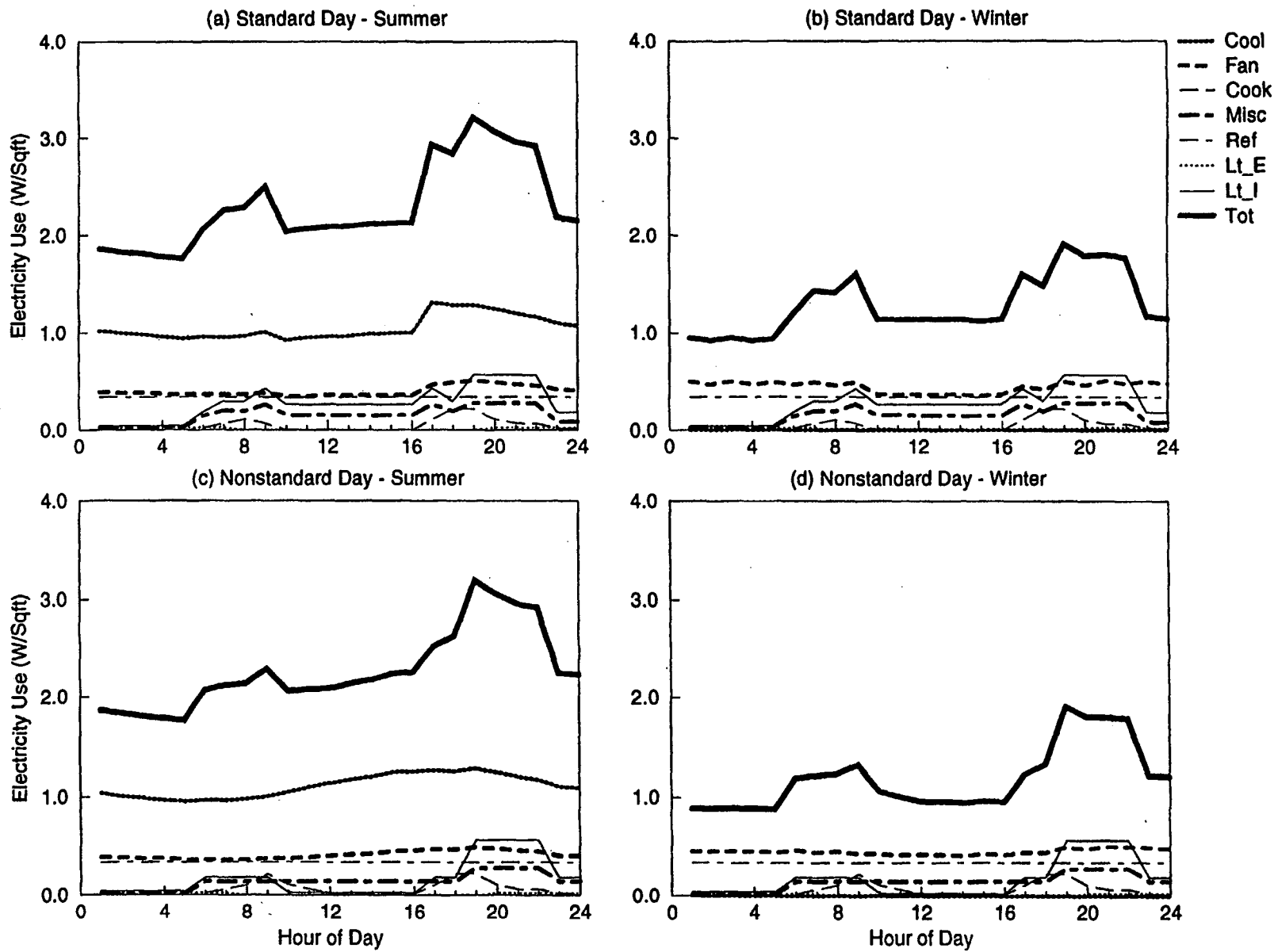
Figure B-2. DOE-2 Simulated End-use Load Shapes for Rolling Pin Barrack
