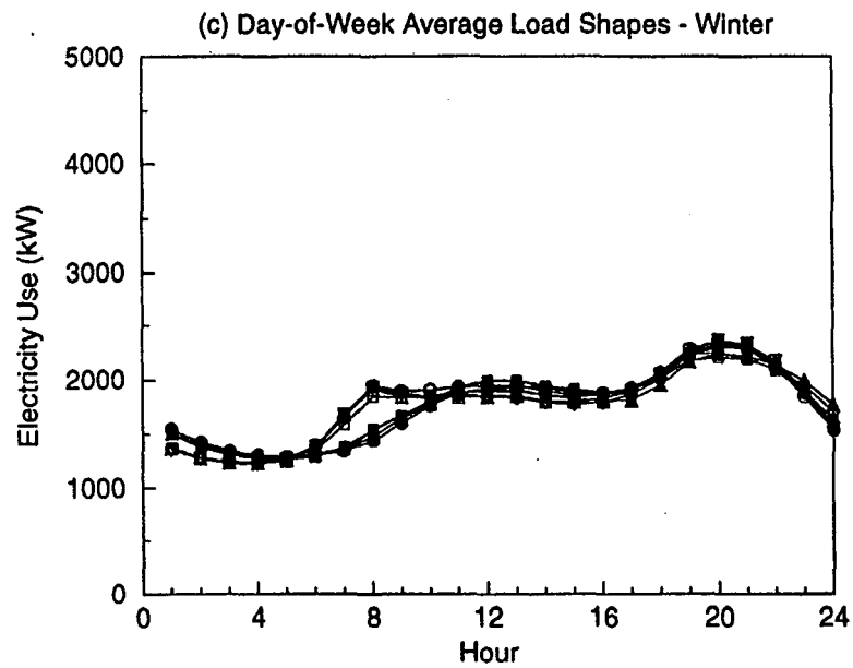
Figure A-16. Feeder 5 Data
