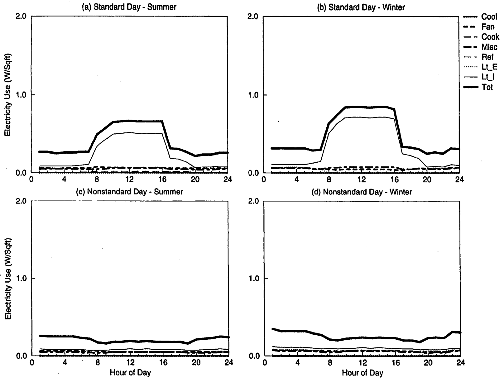
Figure C-39. EDA Reconciled End-use Load Shapes for Small Vehicle Maintenance (No AC) (Feeder 10)
