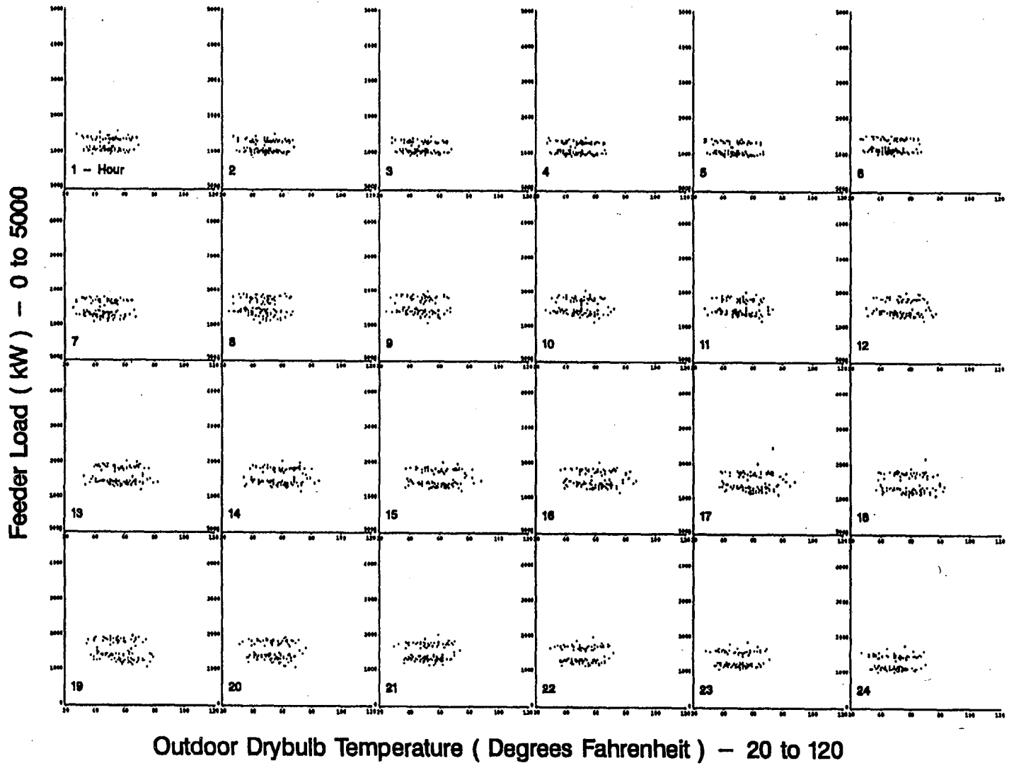
Figure A-7. Scatterplots of Feeder 3 Hourly Load vs. Drybulb Temperature for Standard Winter Days
