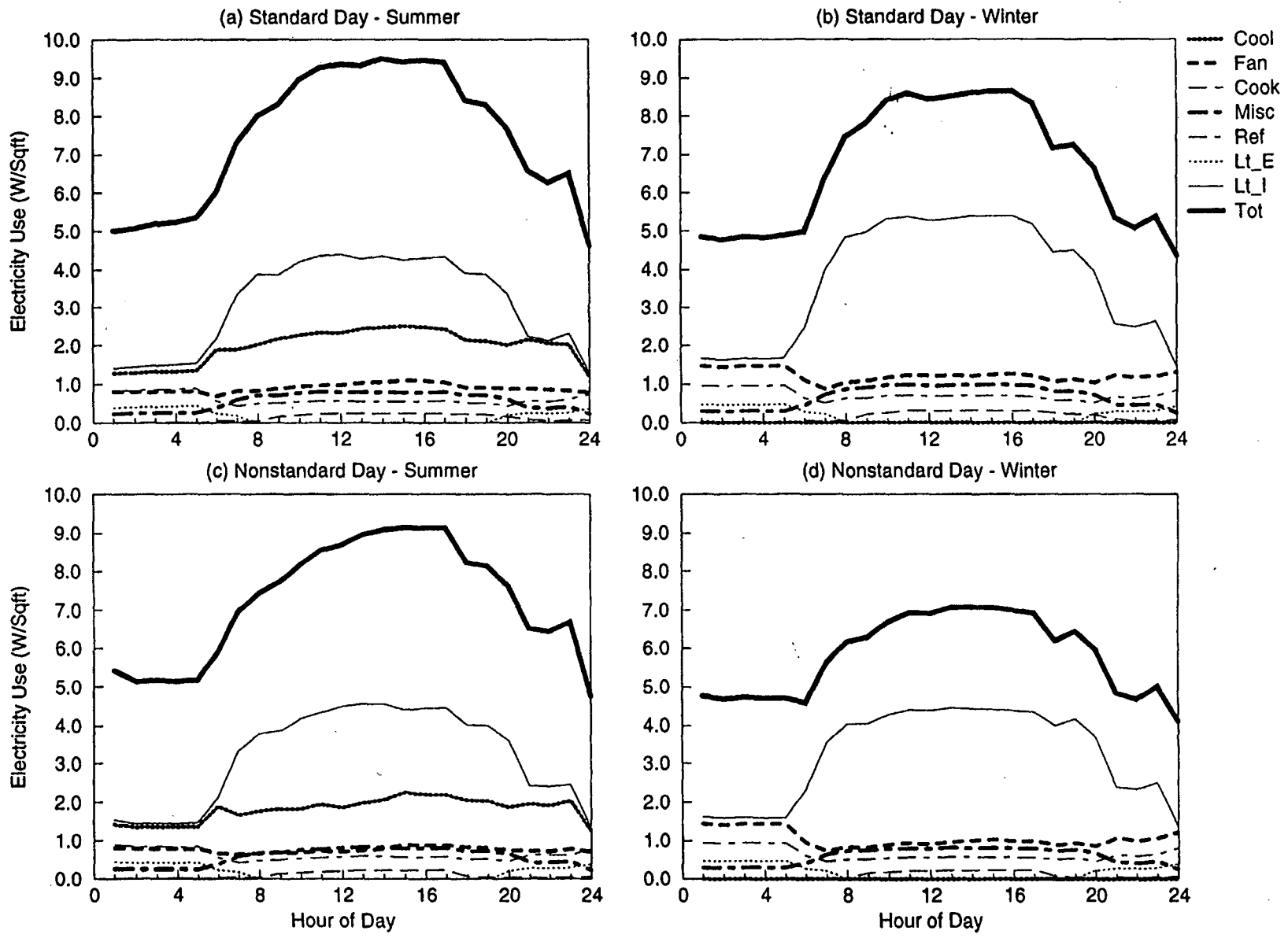
Figure C-62. EDA Reconciled End-use Load Shapes for Large Retail (Feeder W5)
