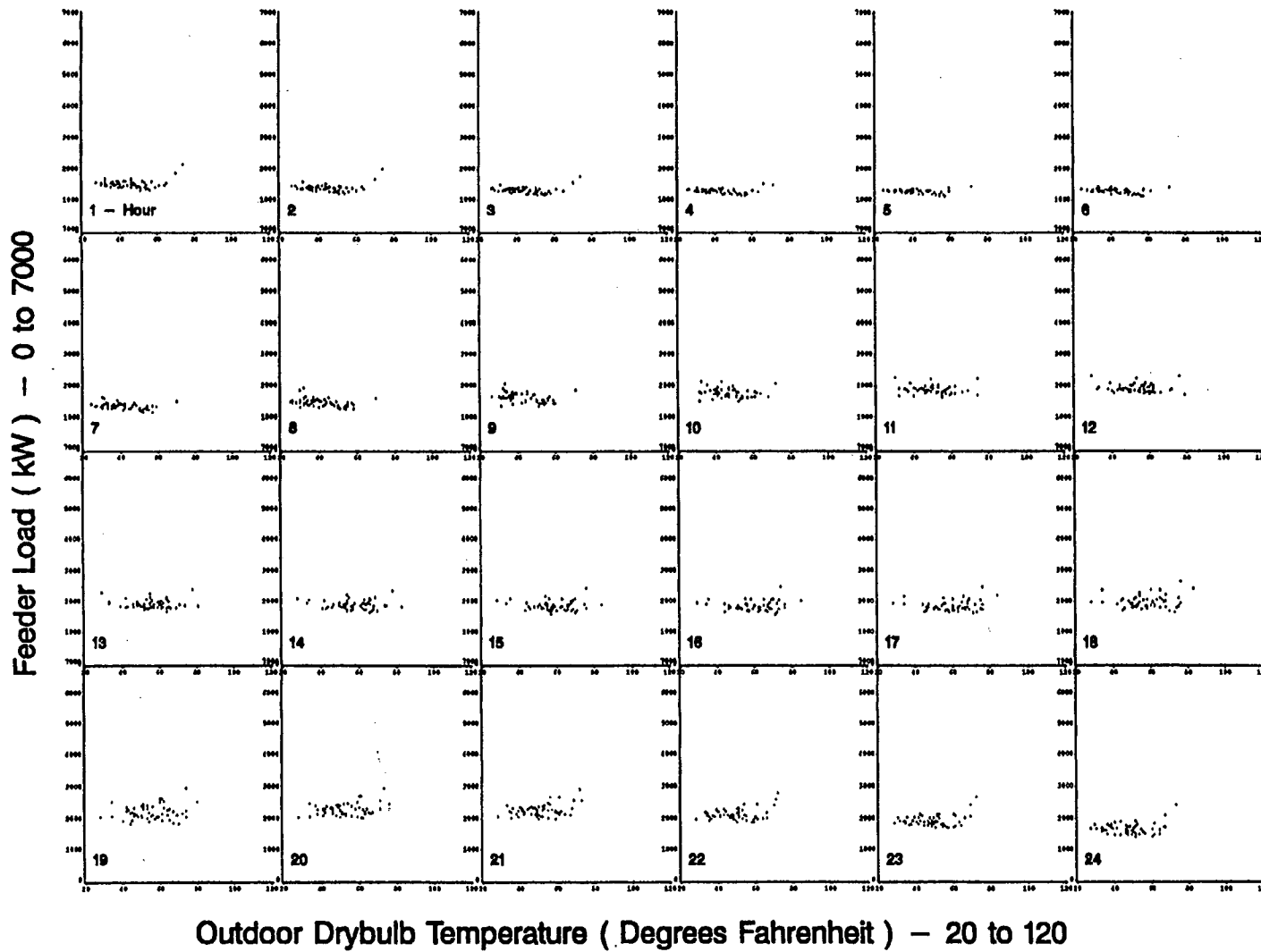
Figure A-18. Scatterplots of Feeder 5 Hourly Load vs. Drybulb Temperature for non-Standard Winter Days
