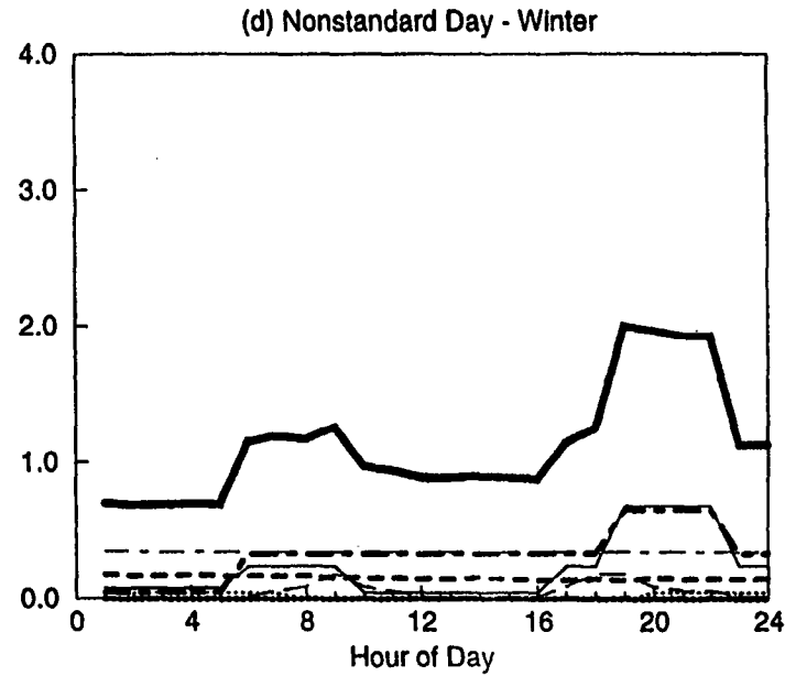
Figure B-1. DOE-2 Simulated End-use Load Shapes for Hammerhead Barrack
