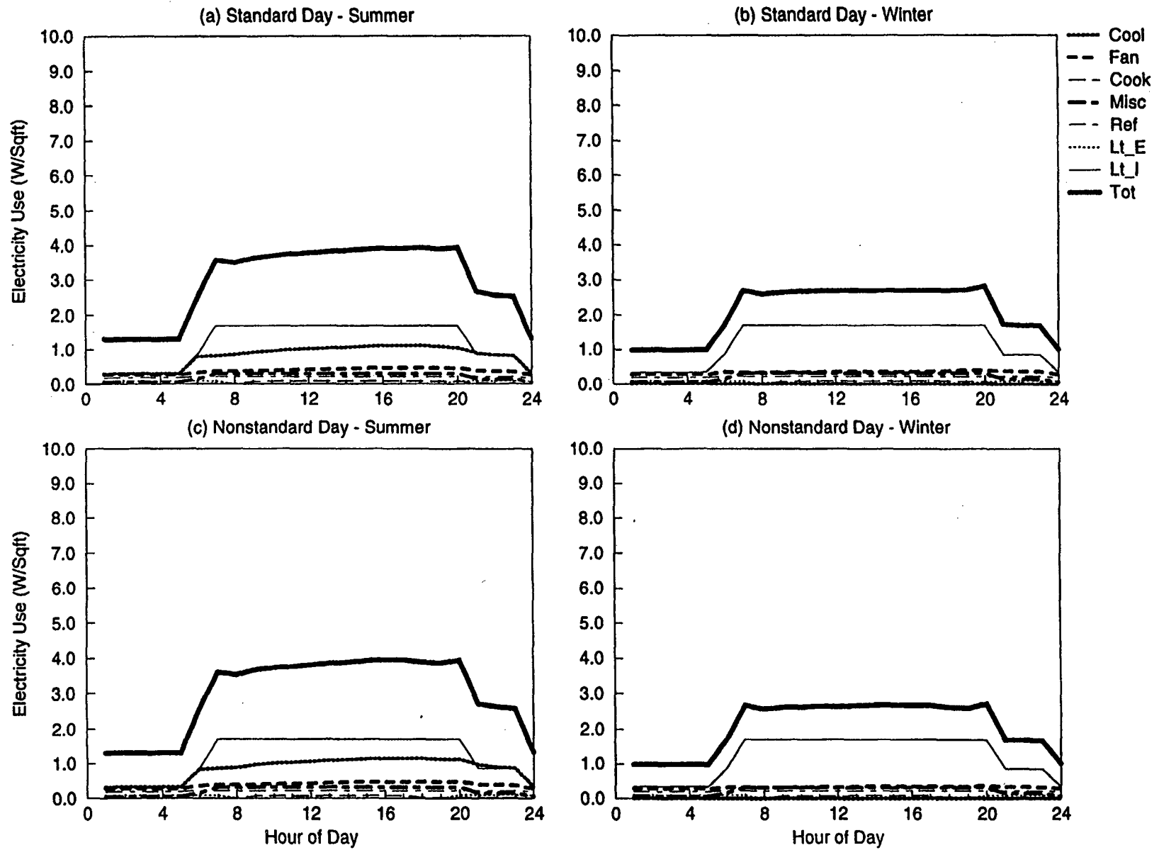
Figure B-20. DOE-2 Simulated End-use Load Shapes for Large Retail
