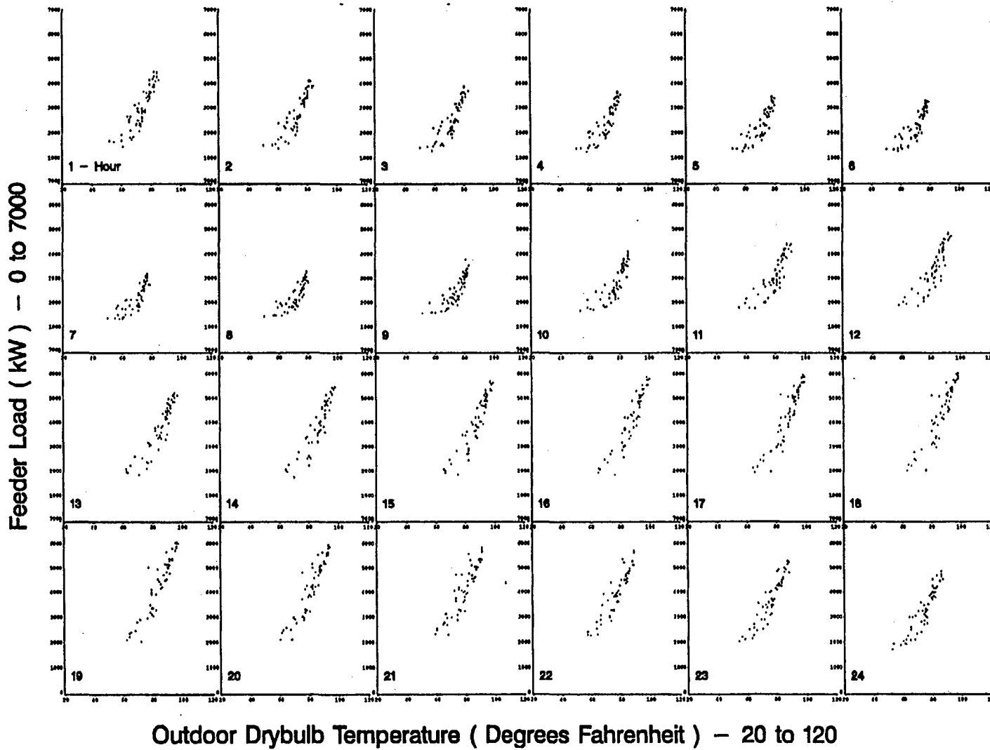
Figure A-20. Scatterplots of Feeder 5 Hourly Load vs. Drybulb Temperature for non-Standard Summer Days
