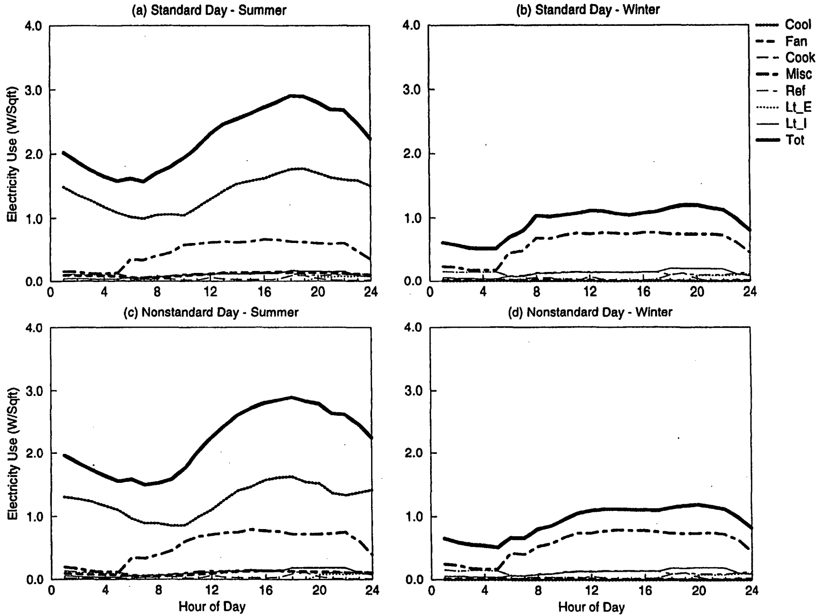
Figure C-51. EDA Reconciled End-use Load Shapes for Detached Residential (Feeder 12)
