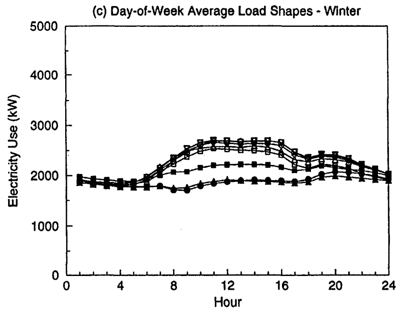
Figure A-36. Feeder 15 Data
