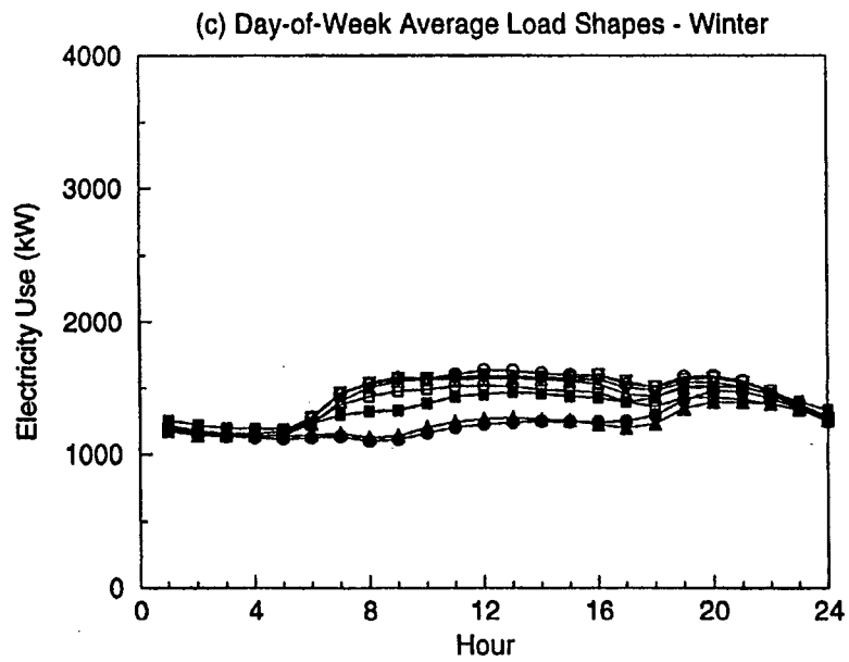
Figure A-6. Feeder 3 Data
