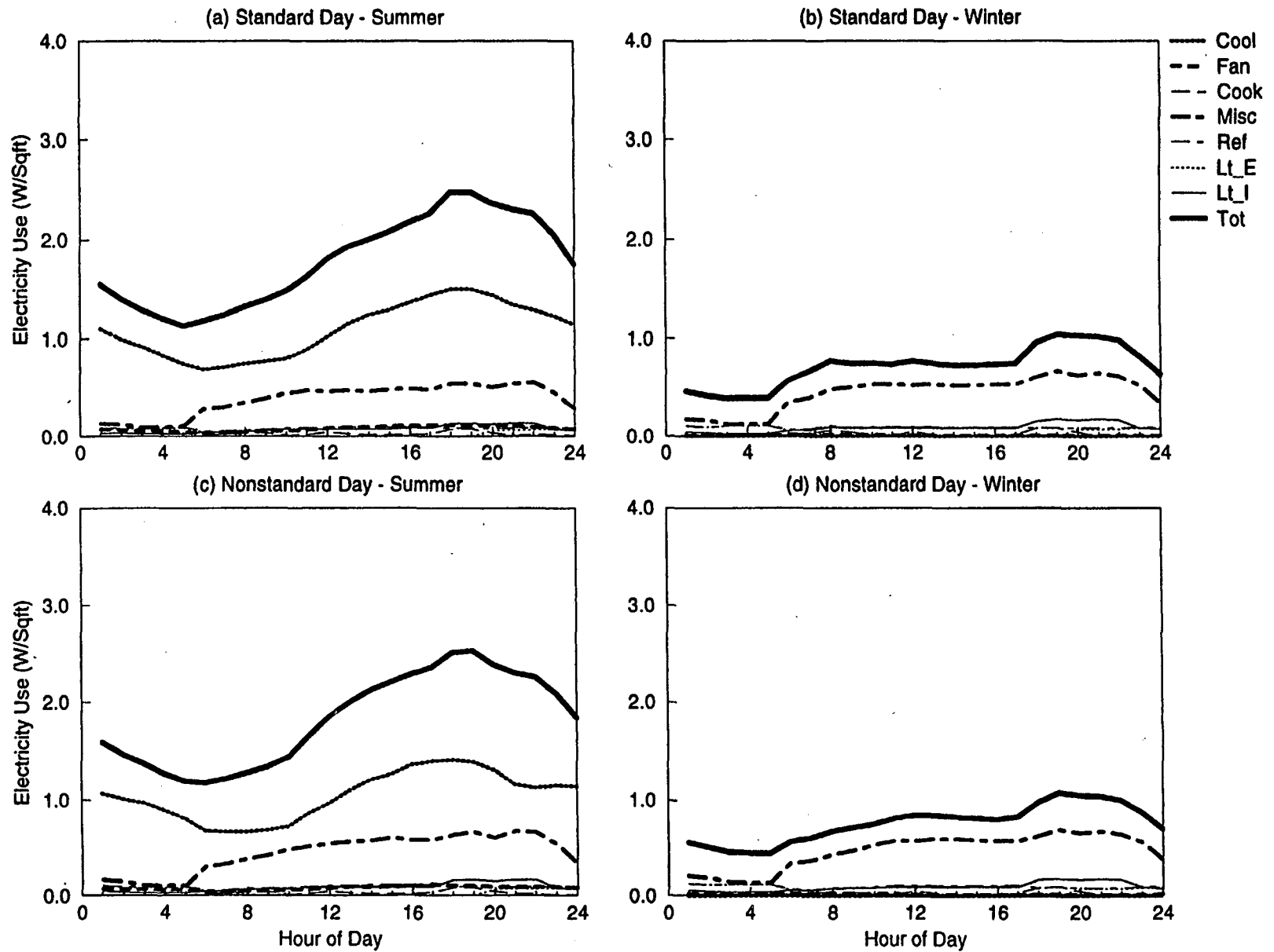
Figure C-53. EDA Reconciled End-use Load Shapes for Detached Residential (Weighted 5,12,W4)
