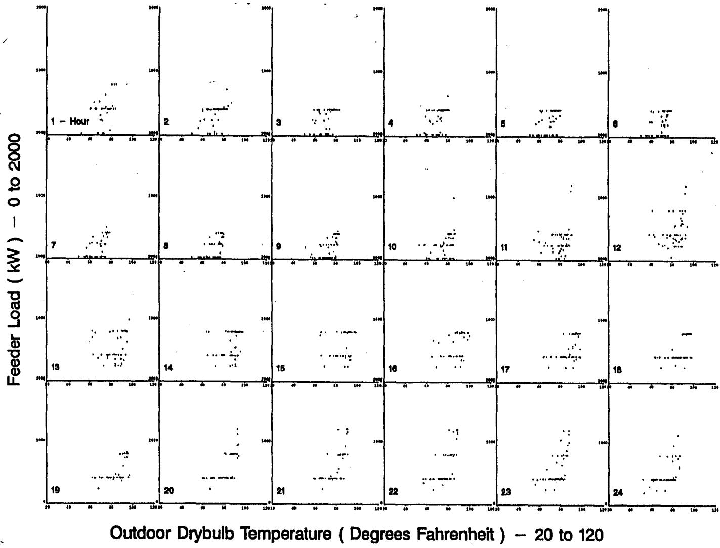
Figure A-15. Scatterplots of Feeder 4 Hourly Load vs. Drybulb Temperature for non-Standard Summer Days
