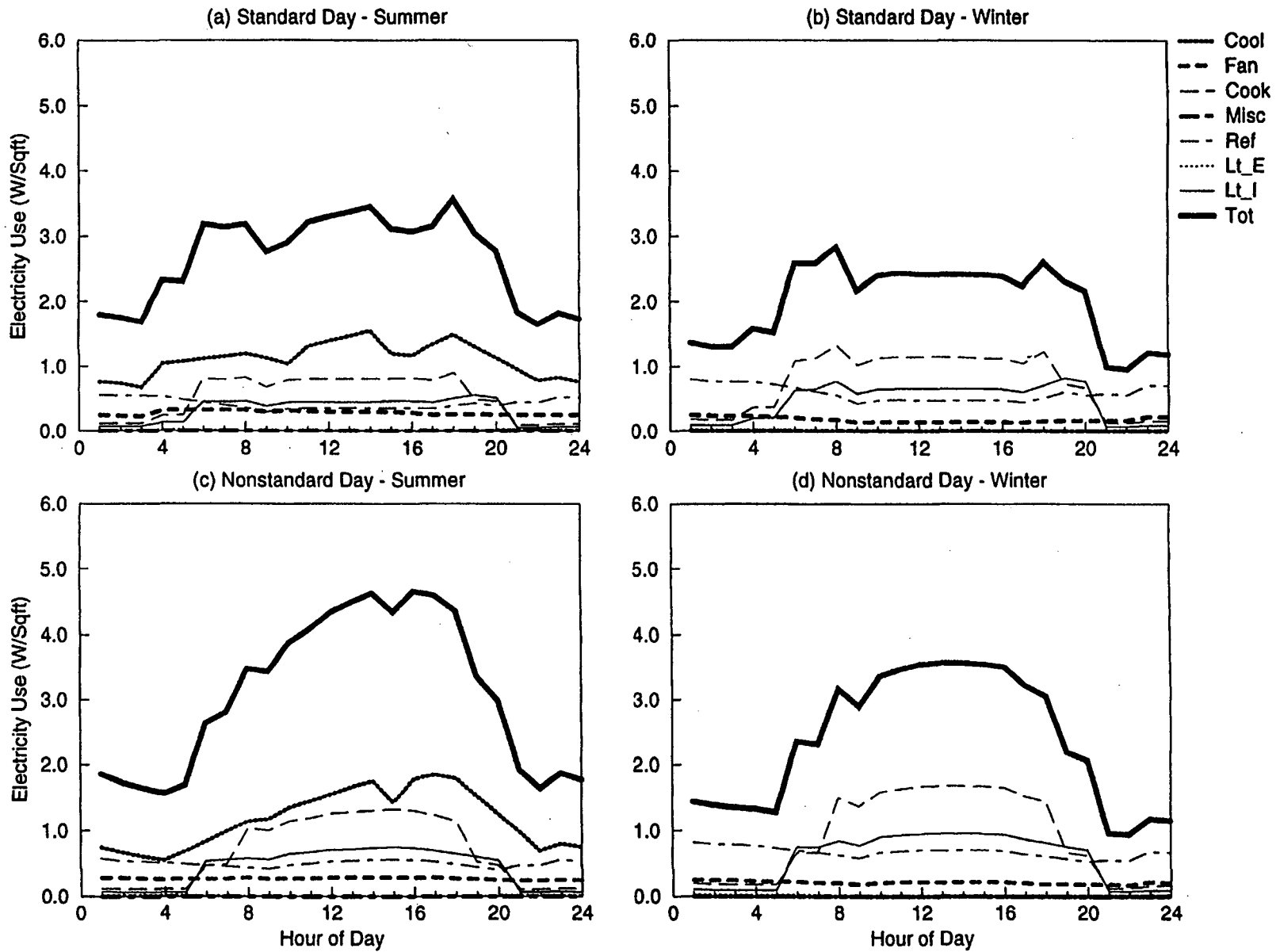
Figure C-18. EDA Reconciled End-use Load Shapes for Dining Hall (Weighted 3,5,10,15)
