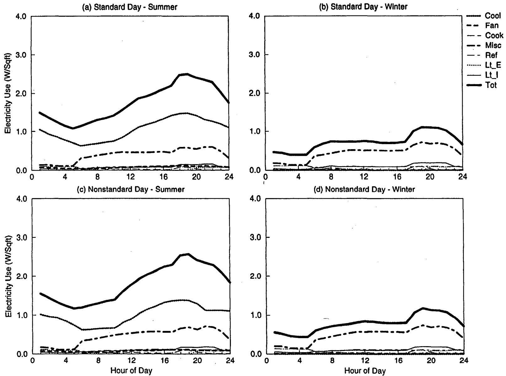
Figure C-54. EDA Reconciled End-use Load Shapes for Two-Plex Residential (Feeder 5)
