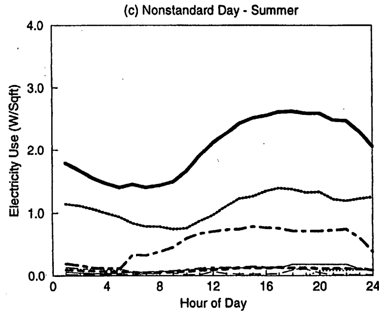
Figure C-60. EDA Reconciled End-use Load Shapes for Four-Plex Residential (Feeder 12)
