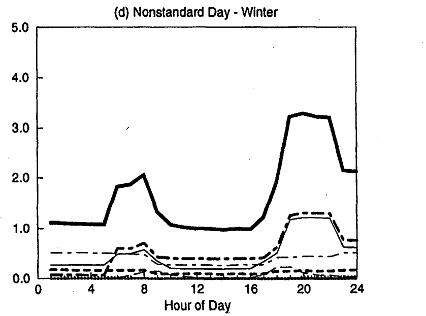
Figure C-8. EDA Reconciled End-use Load Shapes for Modular Barrack (Feeder 2)
