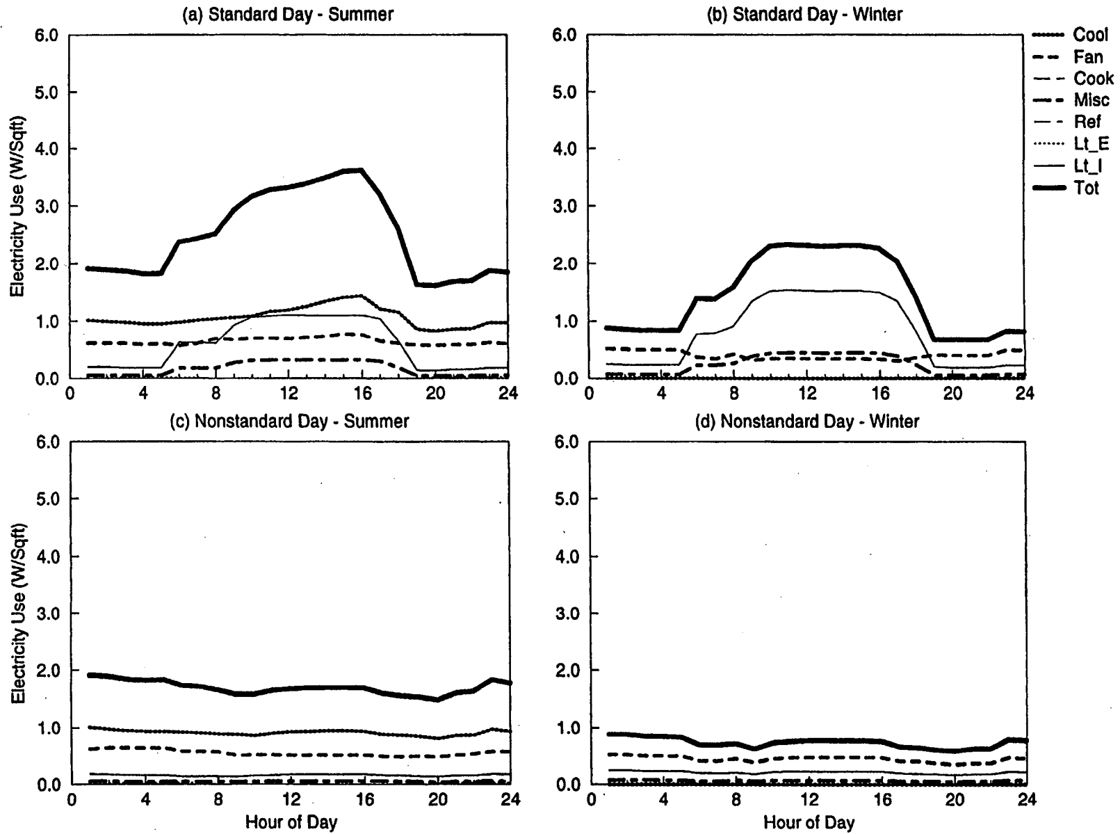
Figure C-30. EDA Reconciled End-use Load Shapes for Small Administration (Old w/ Chiller) (Feeder 10)
