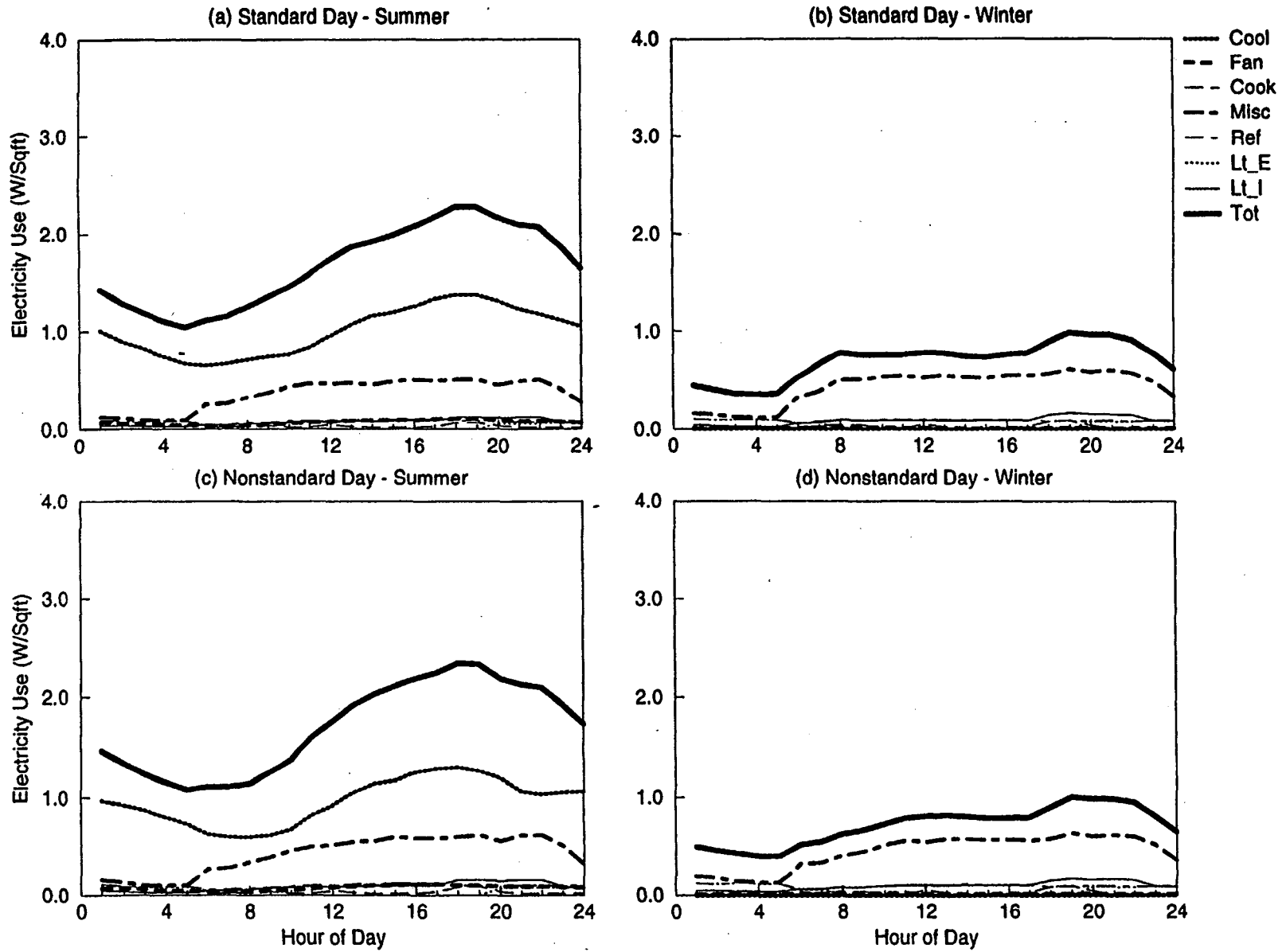
Figure C-58. EDA Reconciled End-use Load Shapes for Two-Plex Residential (Weighted 5,12,W4)
