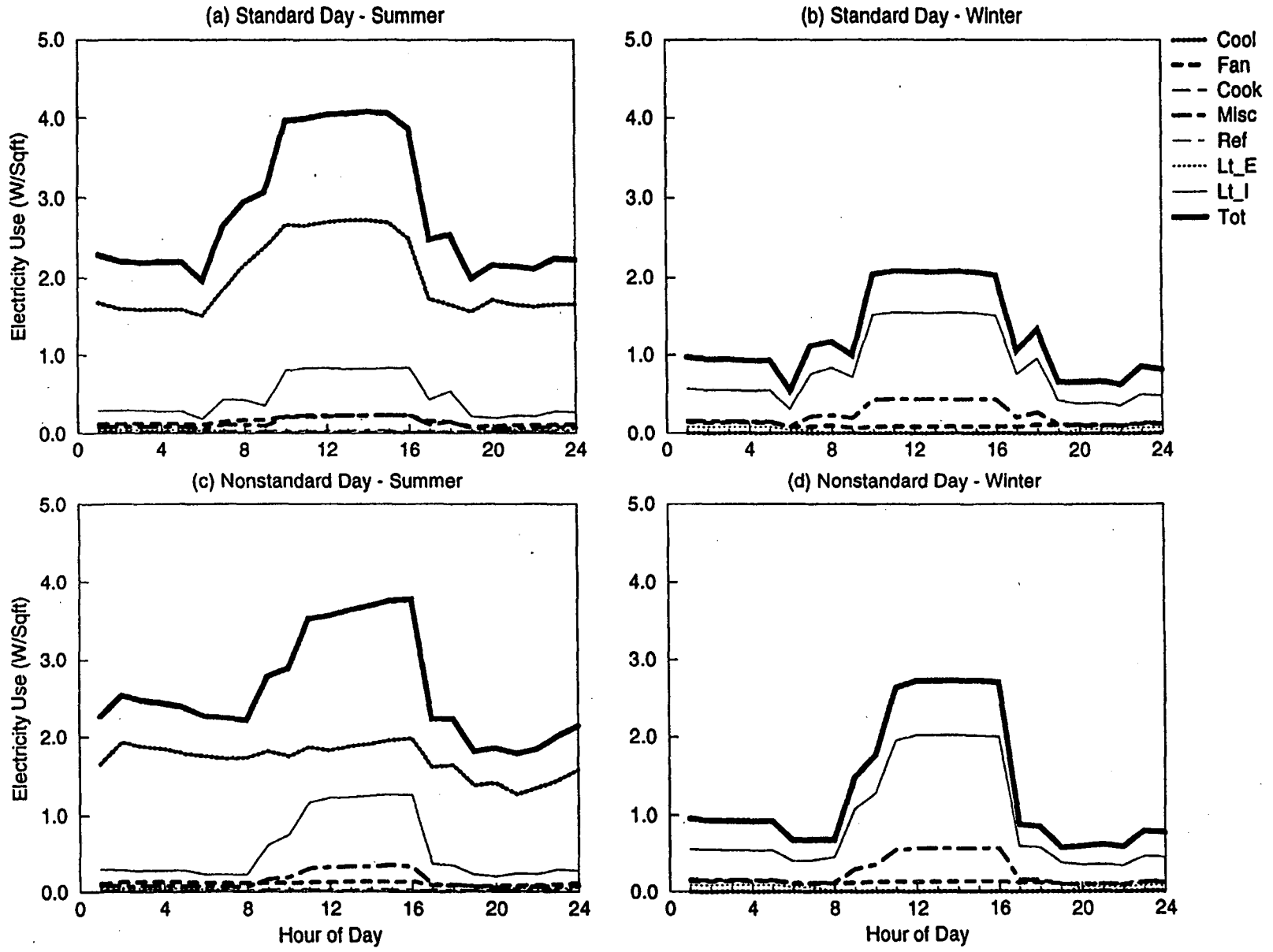
Figure C-69. EDA Reconciled End-use Load Shapes for Miscellaneous (Feeder 15)
