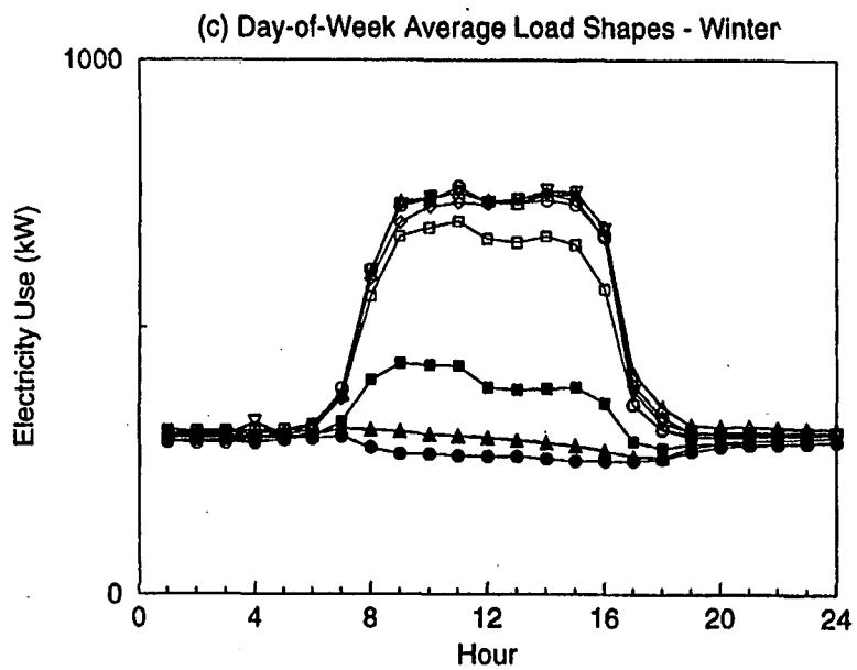
Figure A-51. Feeder W6 Data
