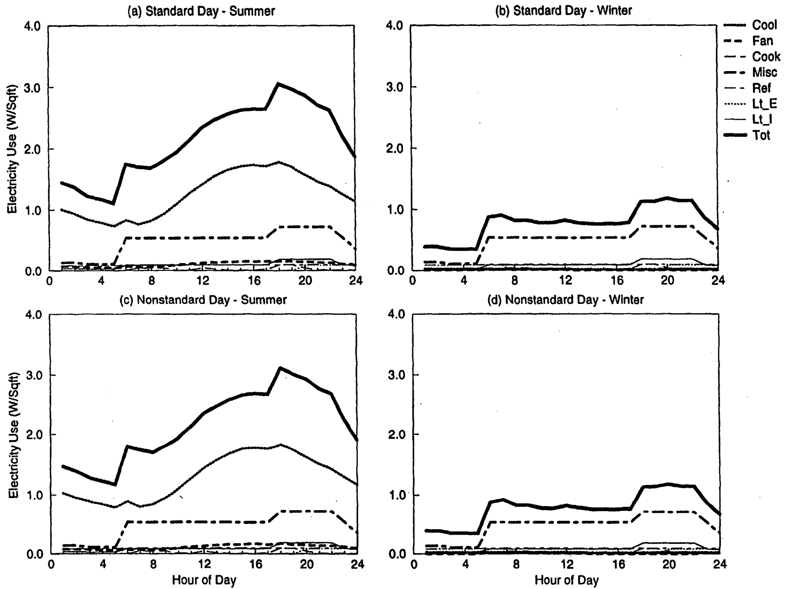
Figure B-19. DOE-2 Simulated End-use Load Shapes for Four-Plex Residential
