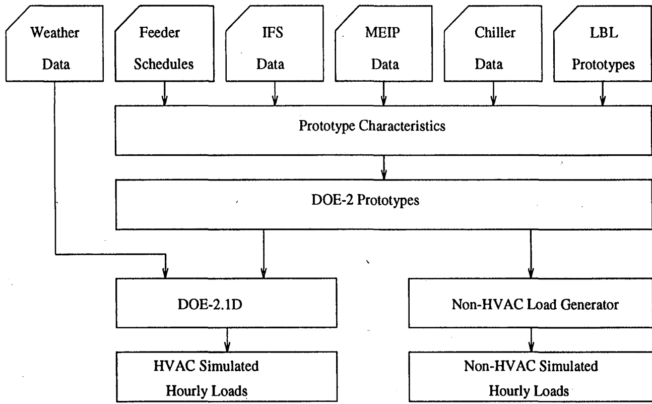
Figure 3-7. Fort Hood End-Use Characterization Methodology - Prototype Development
