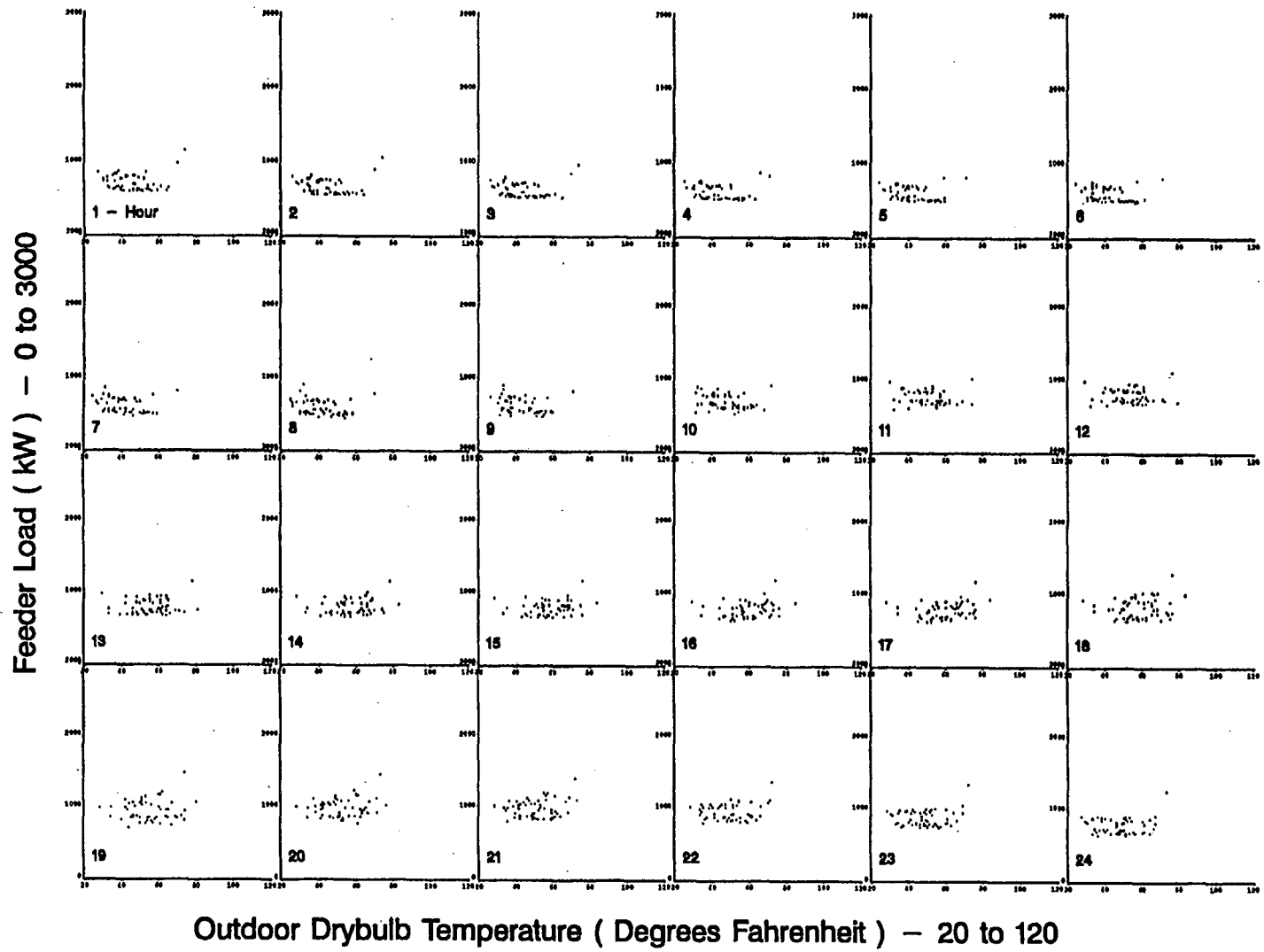
Figure A-33. Scatterplots of Feeder 12 Hourly Load vs. Drybulb Temperature for non-Standard Winter Days
