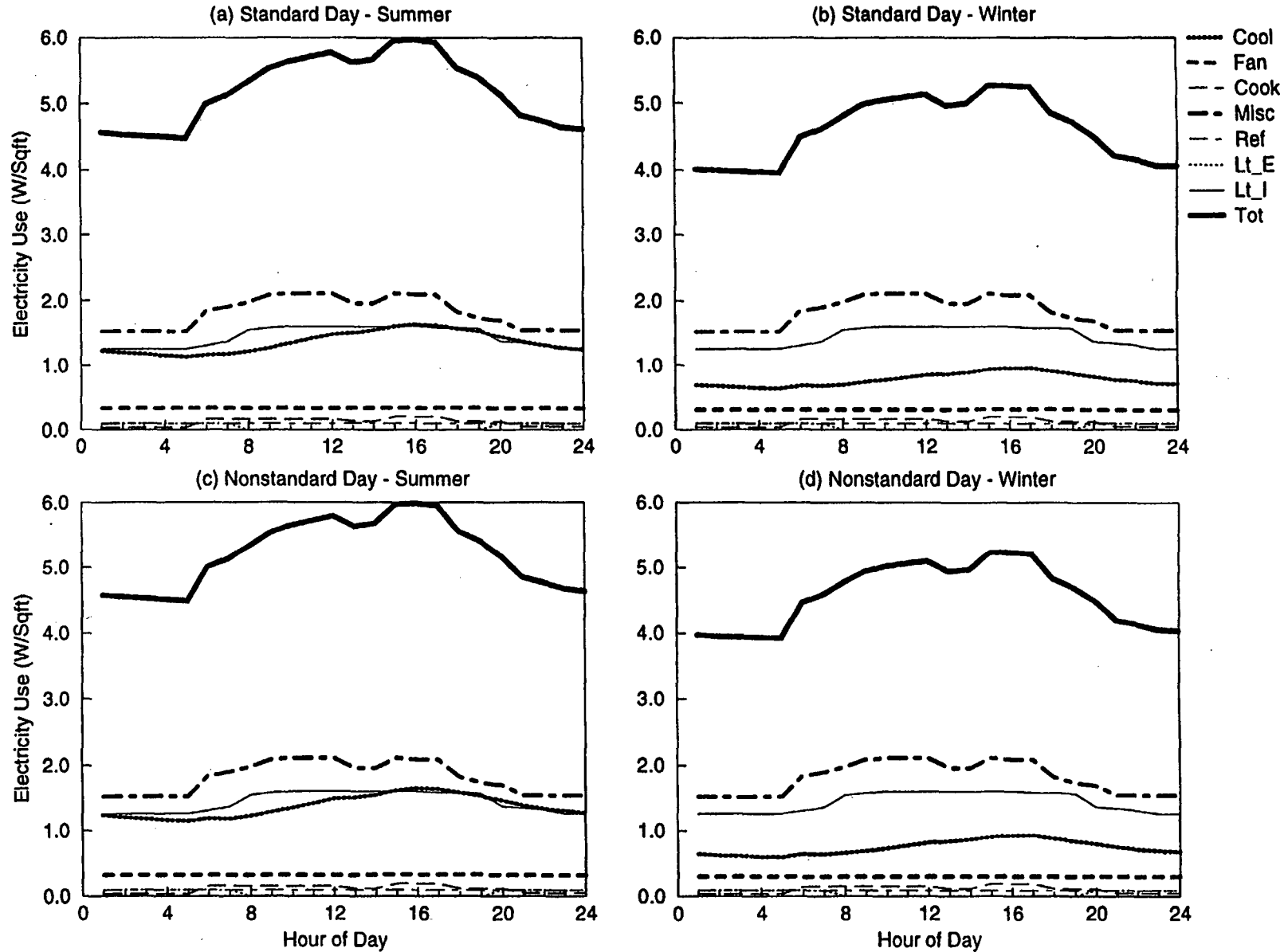
Figure B-16. DOE-2 Simulated End-use Load Shapes for Hospital
