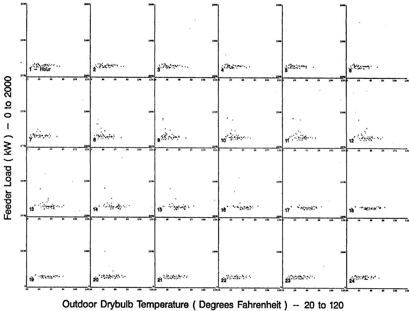
Figure A-53. Scatterplots of Feeder W6 Hourly Load vs. Drybulb Temperature for non-Standard Winter Days
