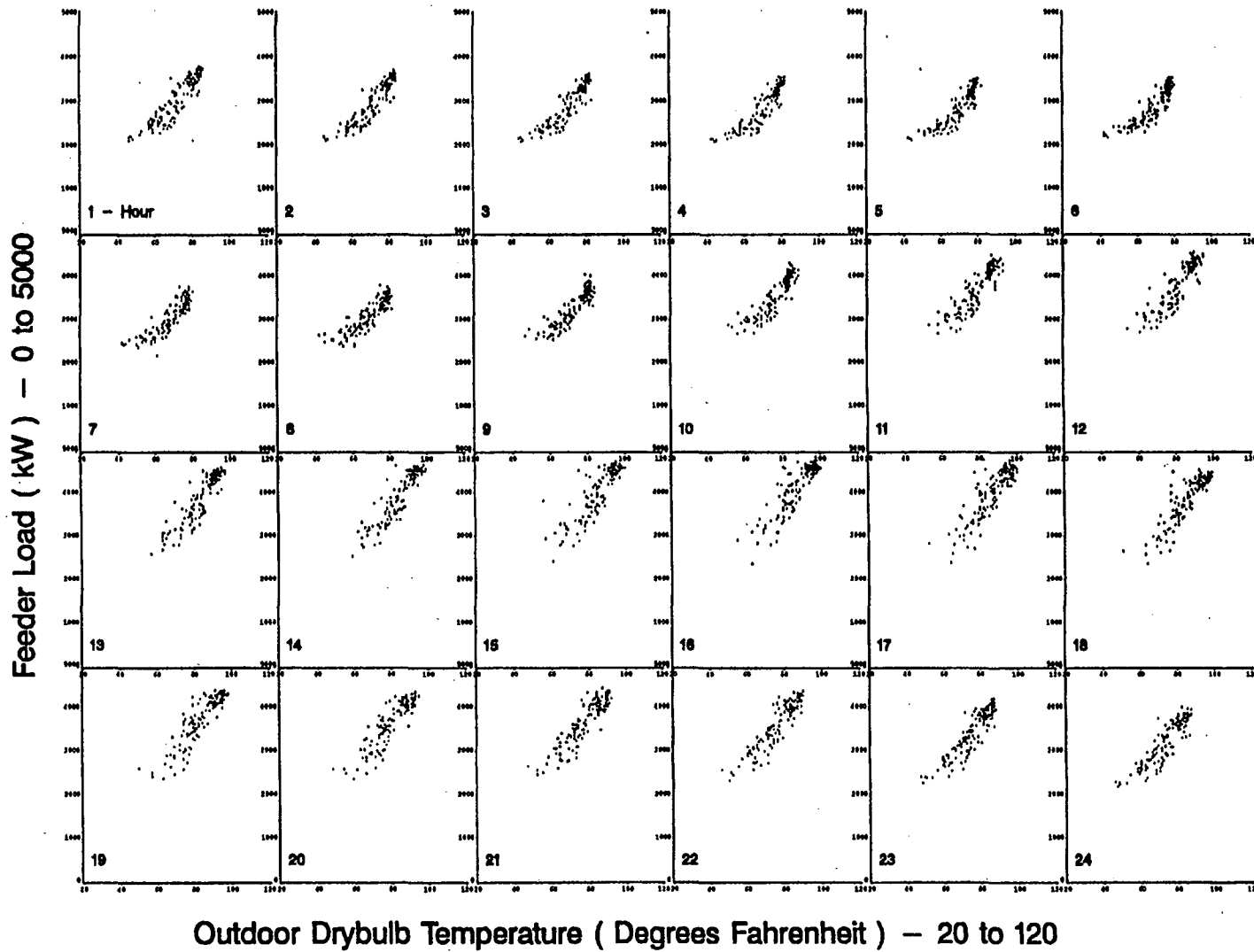
Figure A-49. Scatterplots of Feeder W5 Hourly Load vs. Drybulb Temperature for Standard Summer Days
