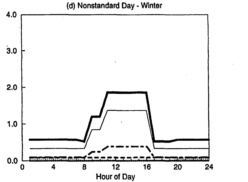
Figure B-30. DOE-2 Simulated End-use Load Shapes for Youth Center
