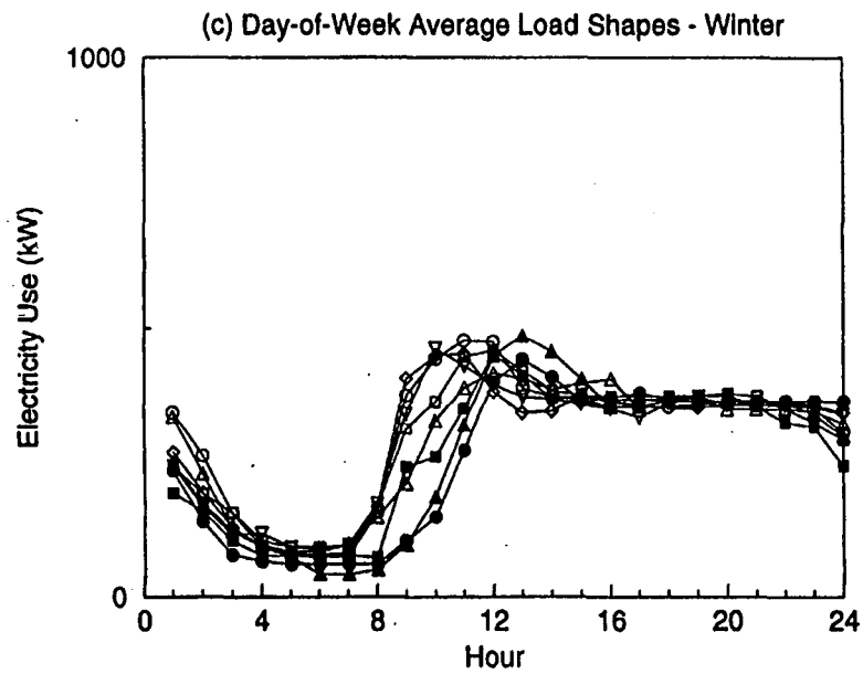
Figure A-11. Feeder 4 Data
