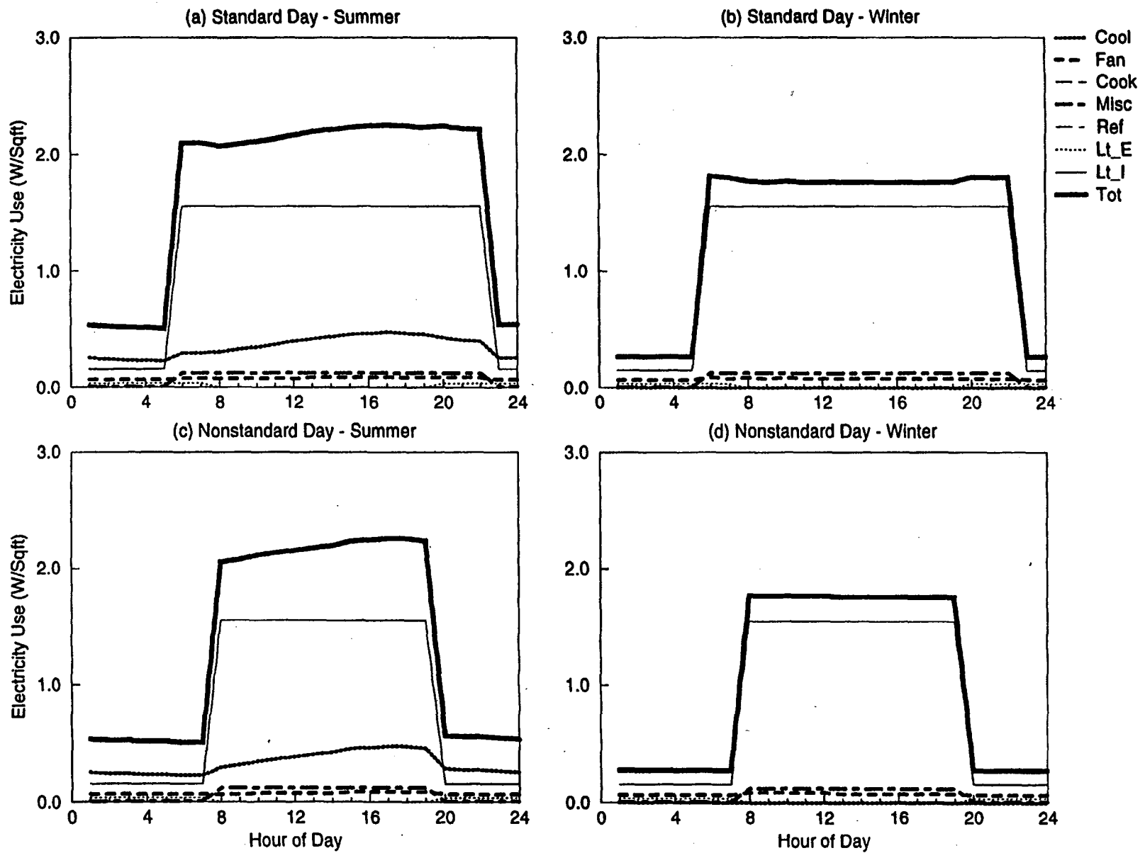
Figure B-6. DOE-2 Simulated End-use Load Shapes for Gymnasium
