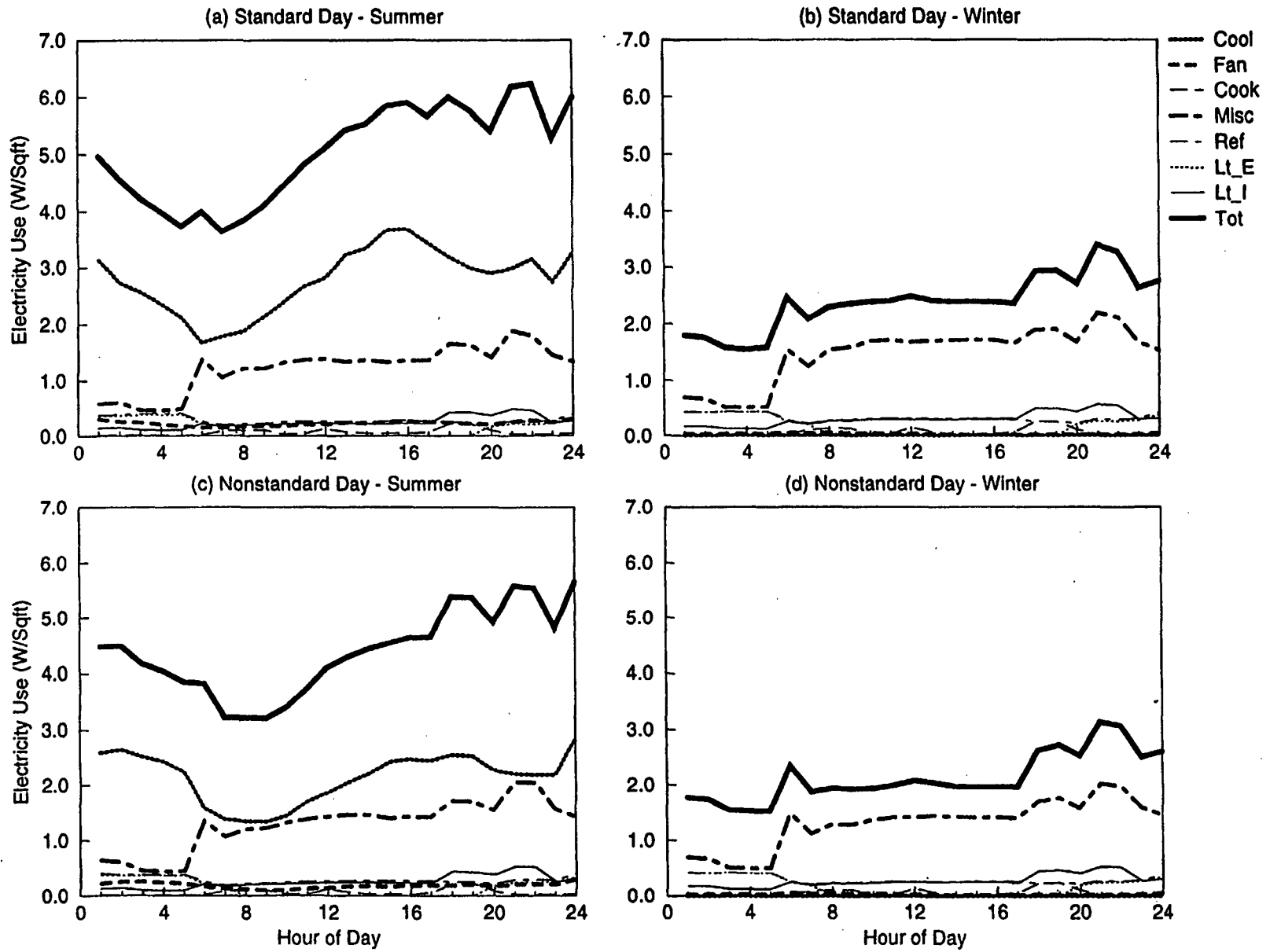
Figure C-57. EDA Reconciled End-use Load Shapes for Two-Plex Residential (Feeder W5)
