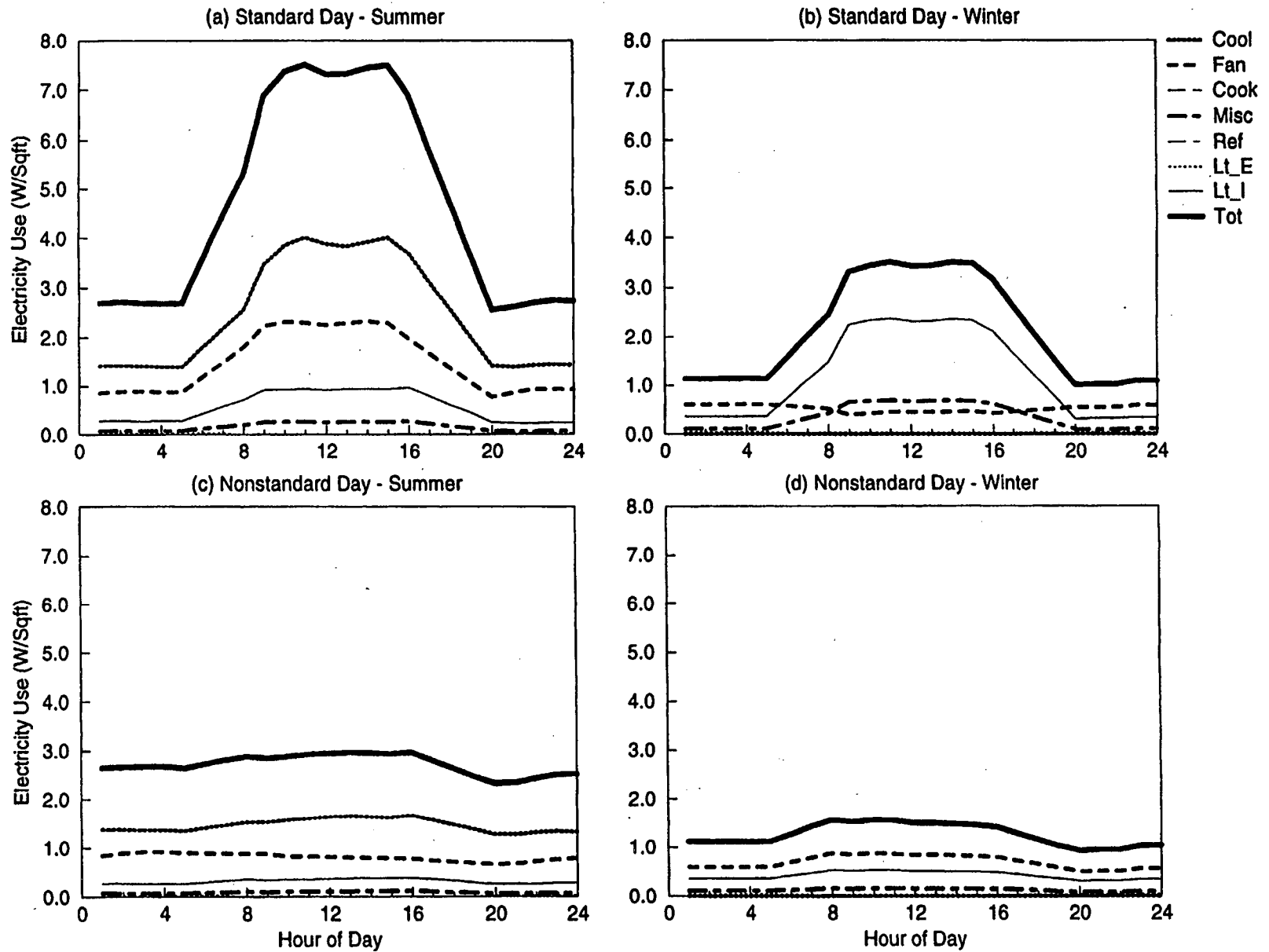
Figure C-37. EDA Reconciled End-use Load Shapes for Small Administration (New w/ Chiller) (Feeder W6)
