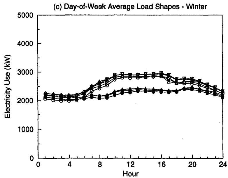
Figure A-46. Feeder W5 Data
