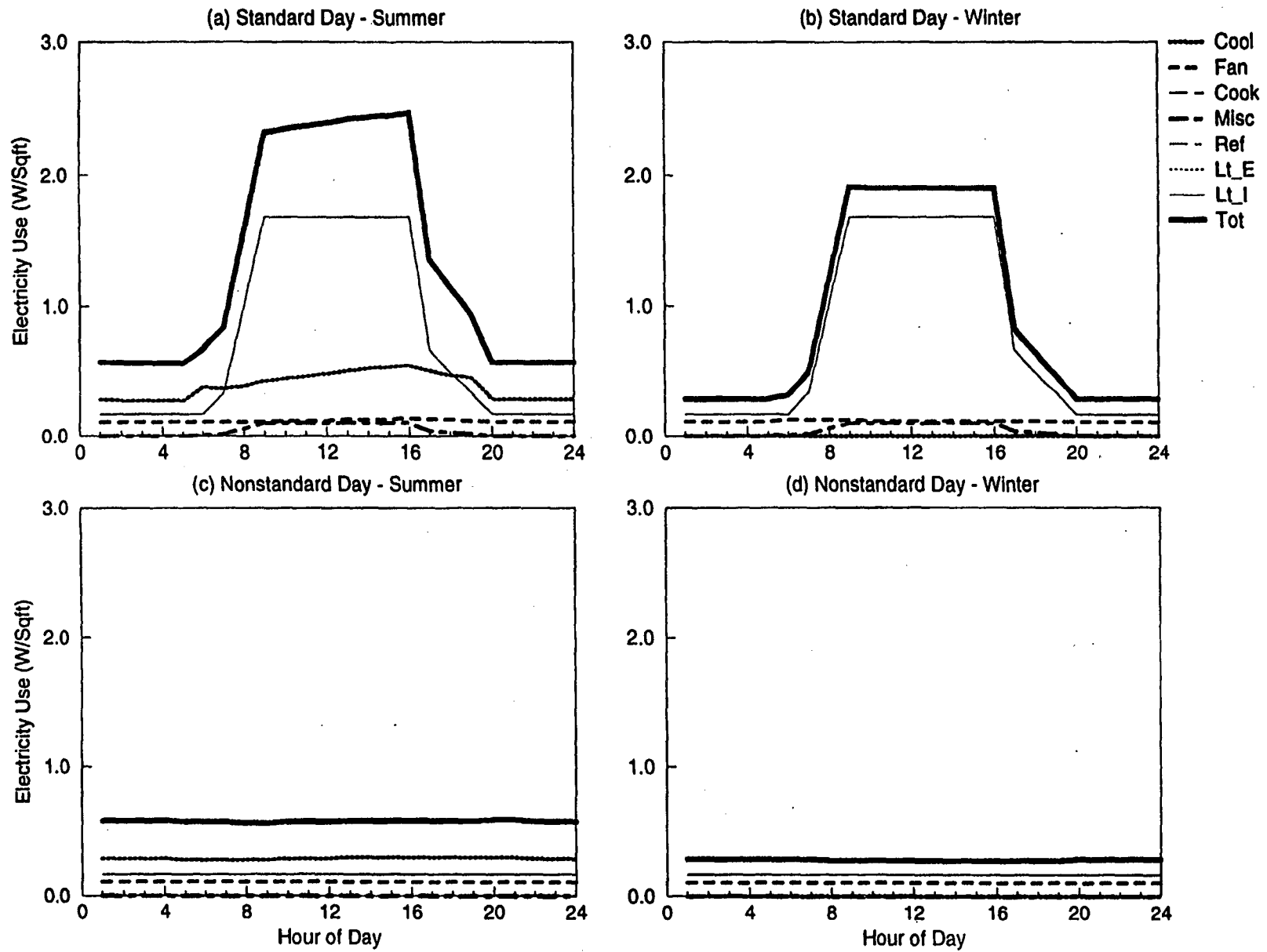
Figure B-15. DOE-2 Simulated End-use Load Shapes for Hangar
