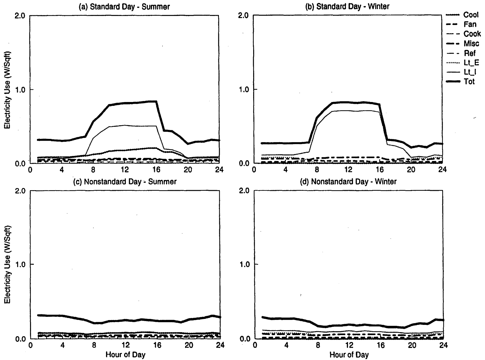
Figure C-42. EDA Reconciled End-use Load Shapes for Large Vehicle Maintenance (Split DX) (Feeder 10)
