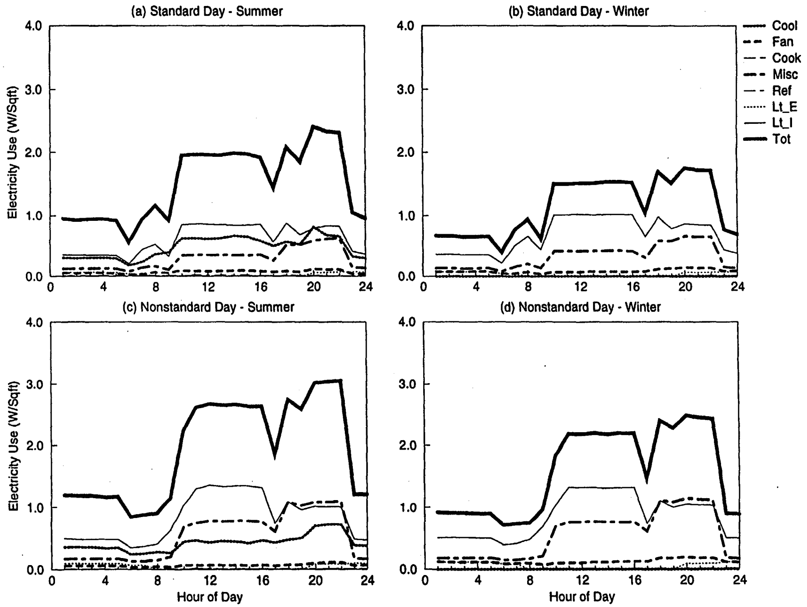
Figure C-65. EDA Reconciled End-use Load Shapes for Miscellaneous (Feeder 2)
