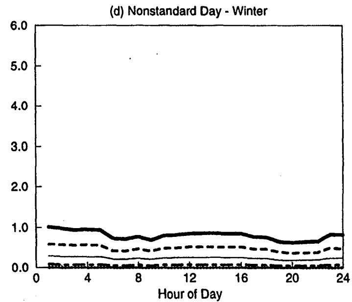
Figure C-32. EDA Reconciled End-use Load Shapes for Small Administration (Old w/ Chiller) (Weighted 3,10,15)
