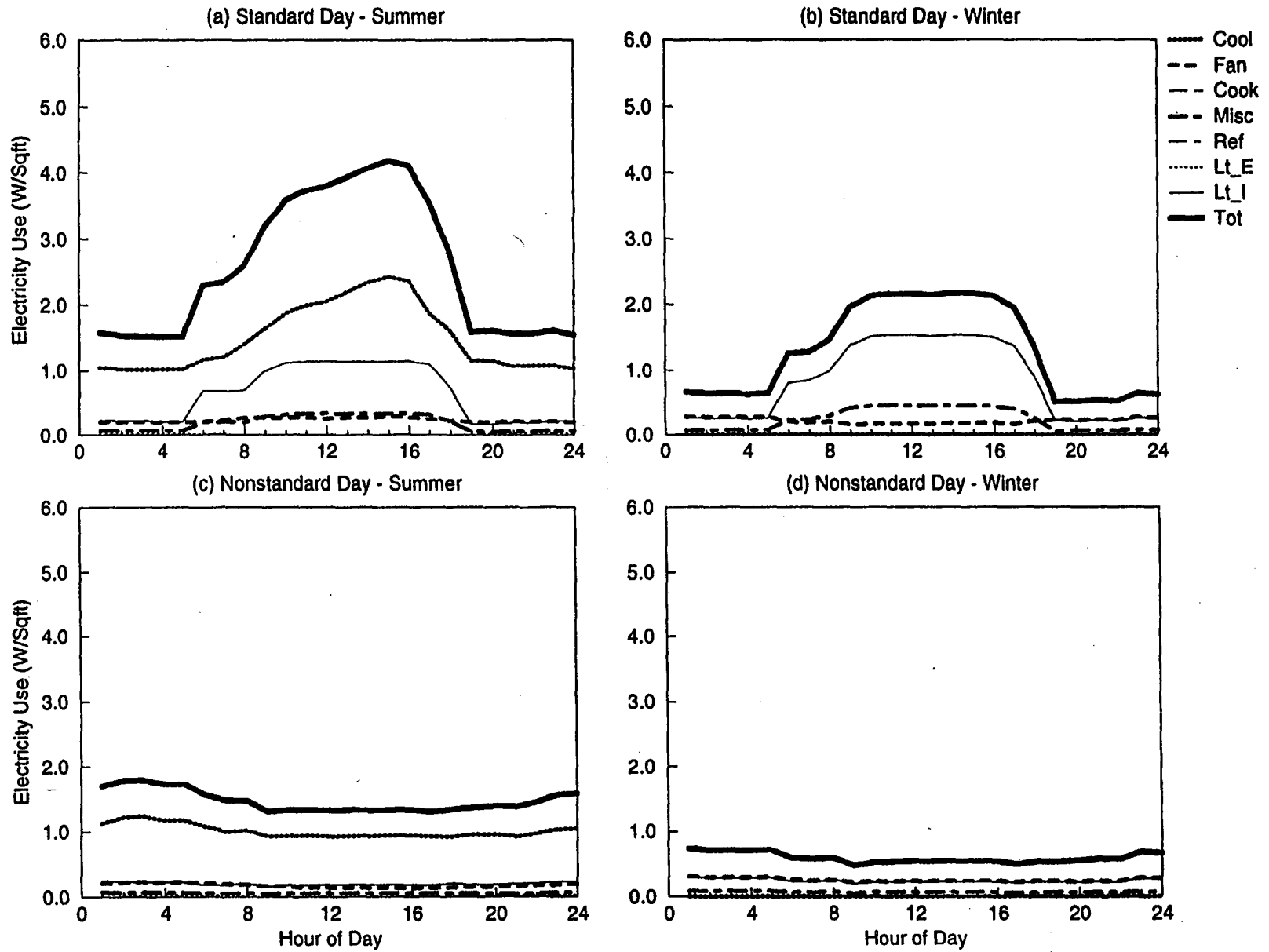
Figure C-35. EDA Reconciled End-use Load Shapes for Small Administration (New w/ Split DX) (Weighted 2,10)
