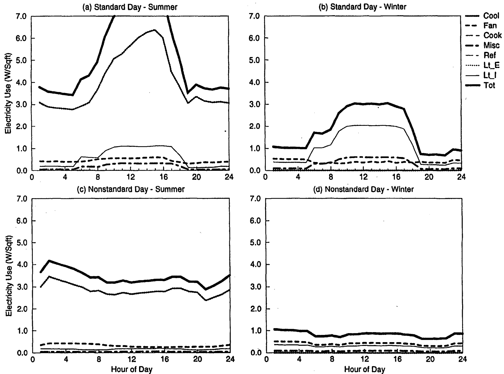
Figure C-26. EDA Reconciled End-use Load Shapes for Small Administration (Old w/ Split DX) (Feeder 15)
