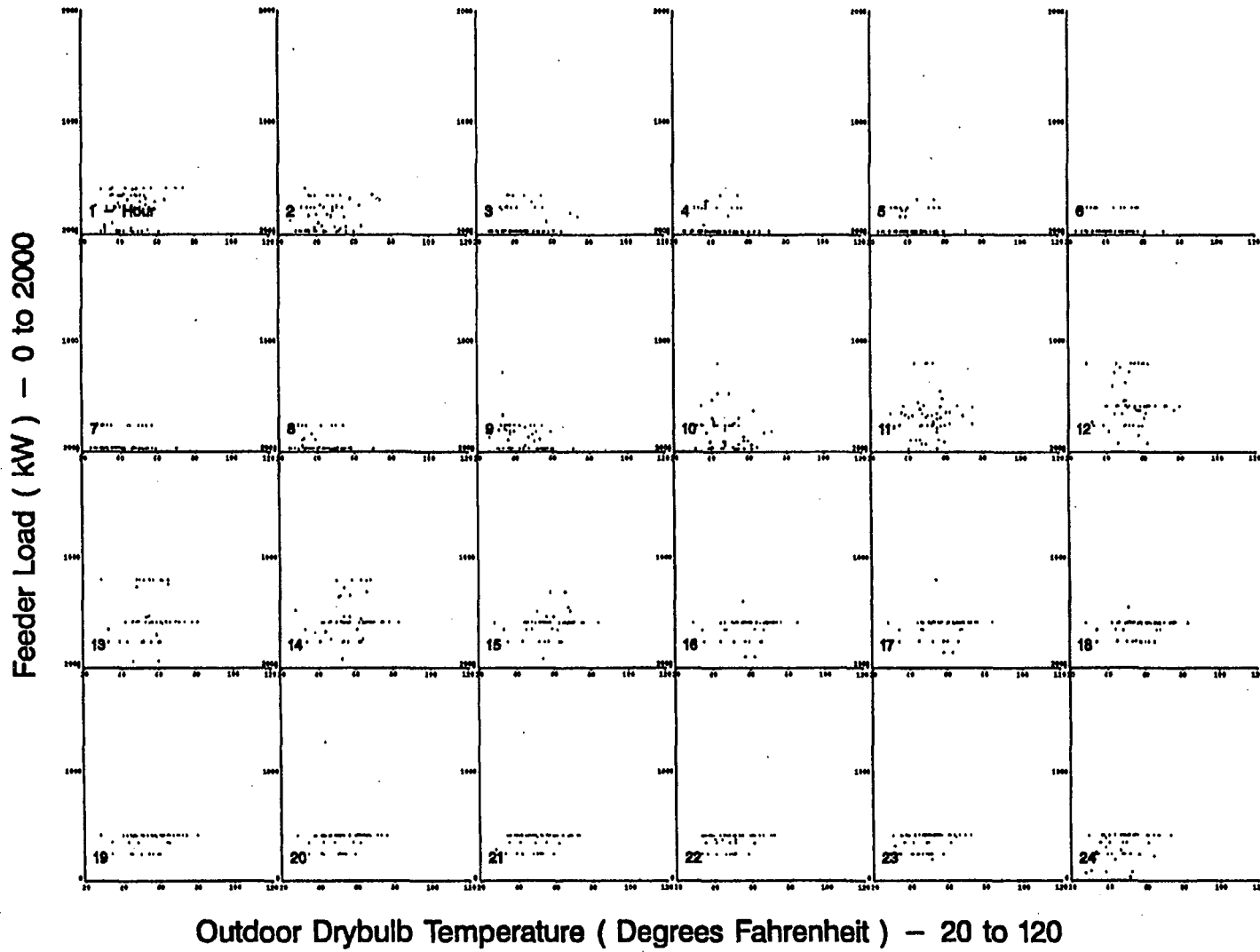
Figure A-13. Scatterplots of Feeder 4 Hourly Load vs. Drybulb Temperature for non-Standard Winter Days
