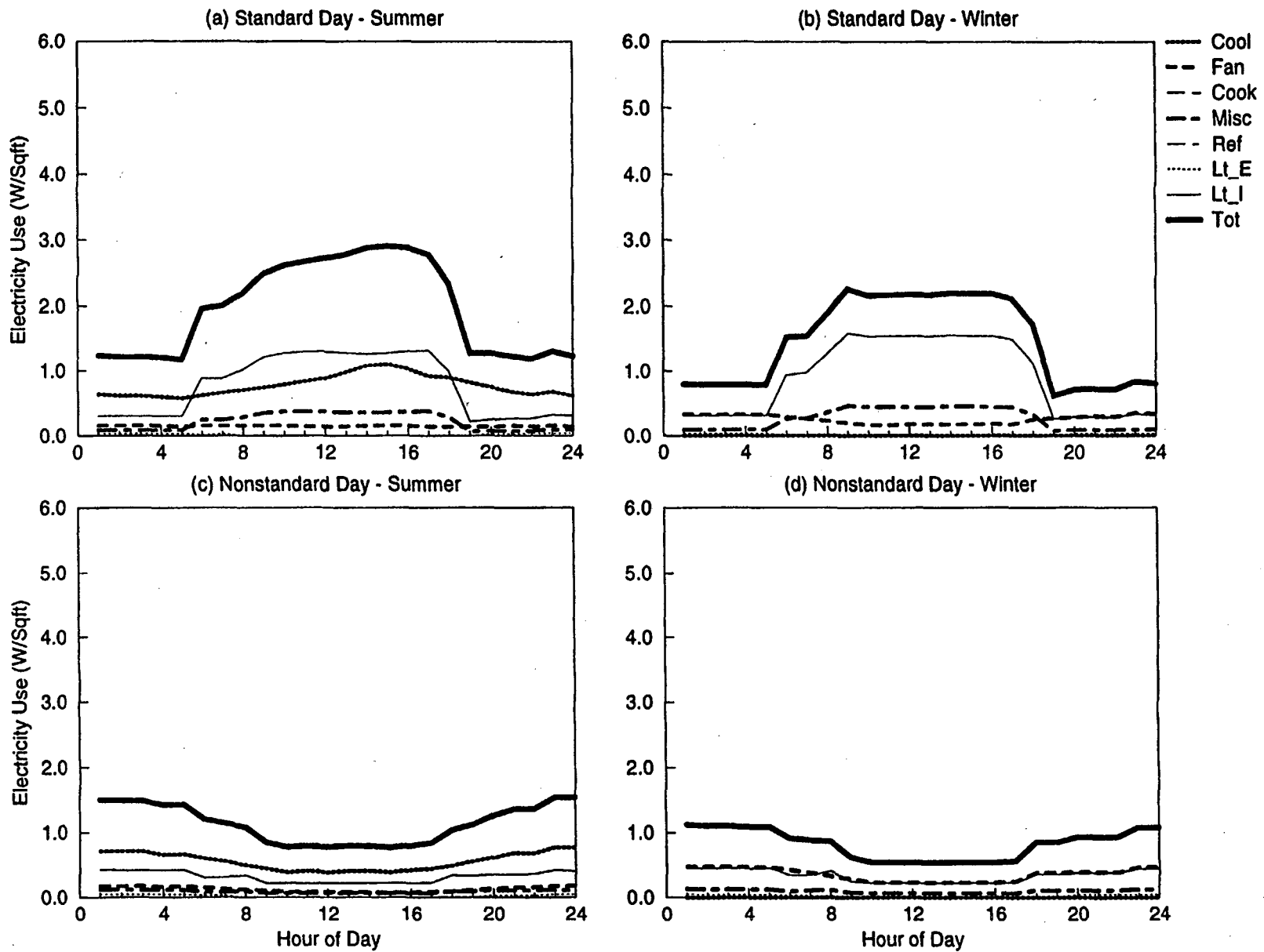
Figure C-33. EDA Reconciled End-use Load Shapes for Small Administration (New w/ Split DX) (Feeder 2)
