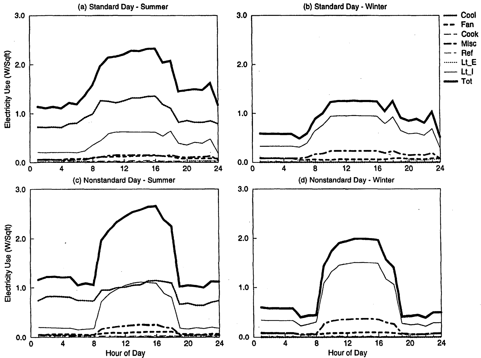
Figure C-66. EDA Reconciled End-use Load Shapes for Miscellaneous (Feeder 3)
