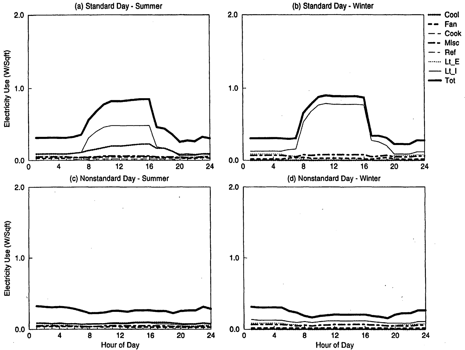
Figure C-45. EDA Reconciled End-use Load Shapes for Large Vehicle Maintenance (Split DX) (Weighted 3,10,15)
