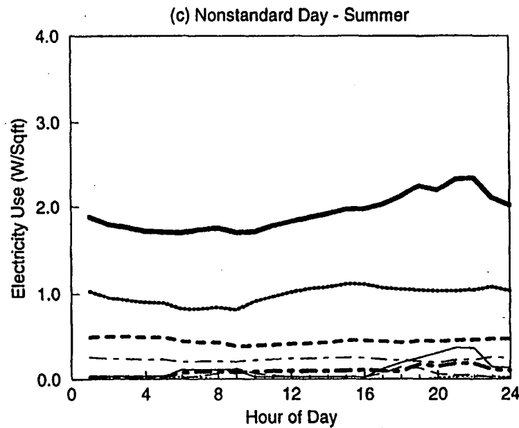
Figure C-7. EDA Reconciled End-use Load Shapes for Rolling Pin Barrack (Weighted 3,10)
