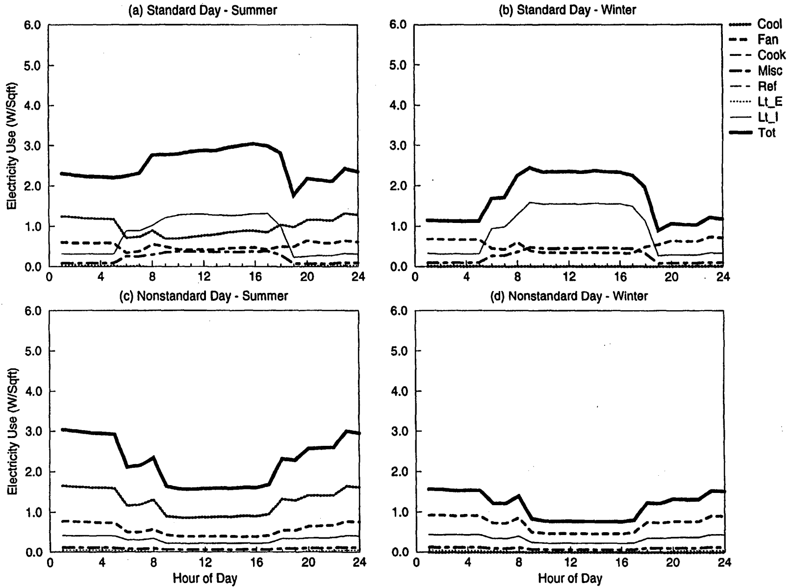
Figure C-28. EDA Reconciled End-use Load Shapes for Small Administration (Old w/ Chiller) (Feeder 2)
