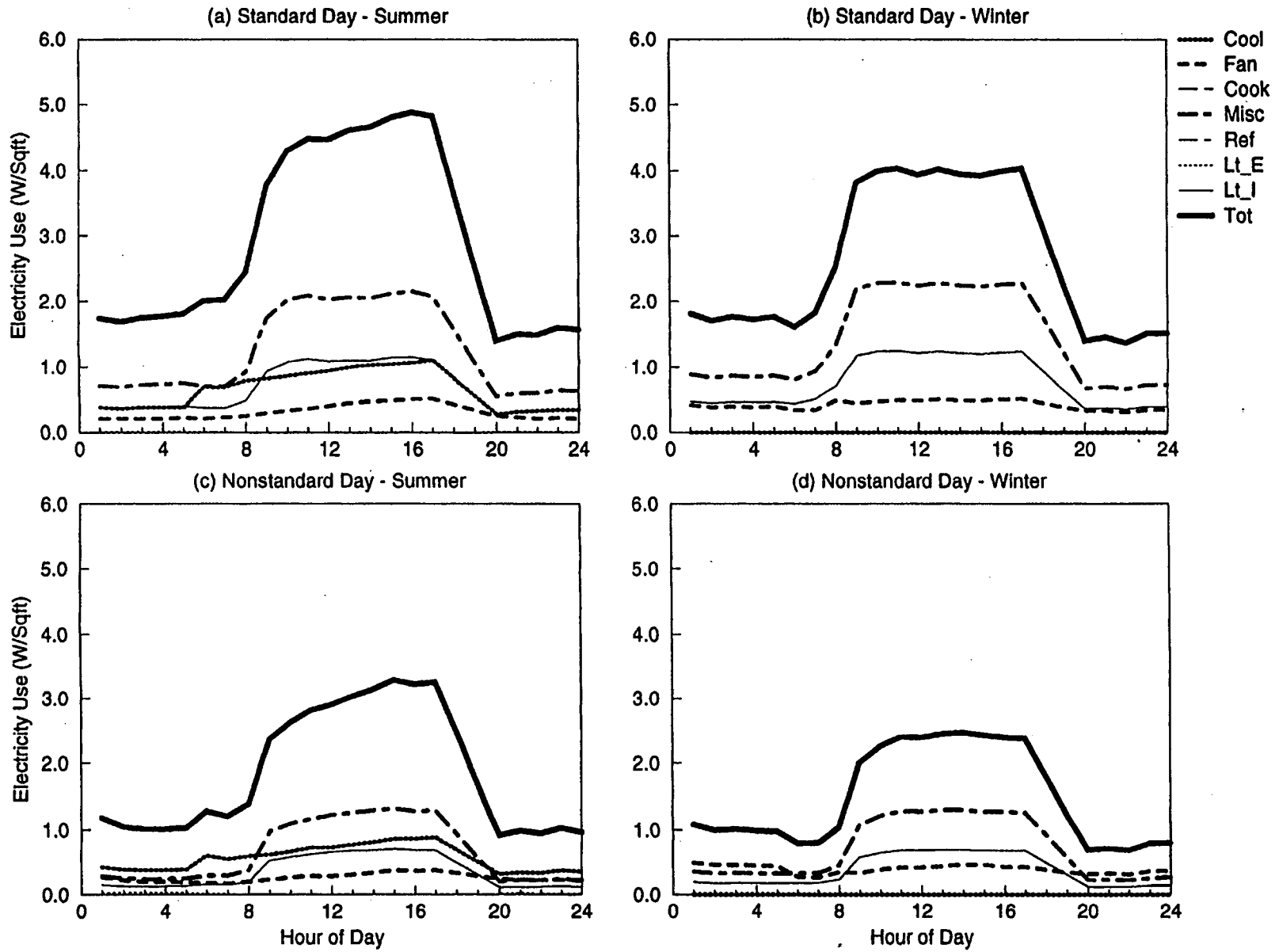
Figure C-22. EDA Reconciled End-use Load Shapes for Large Administration (Feeder 5)
