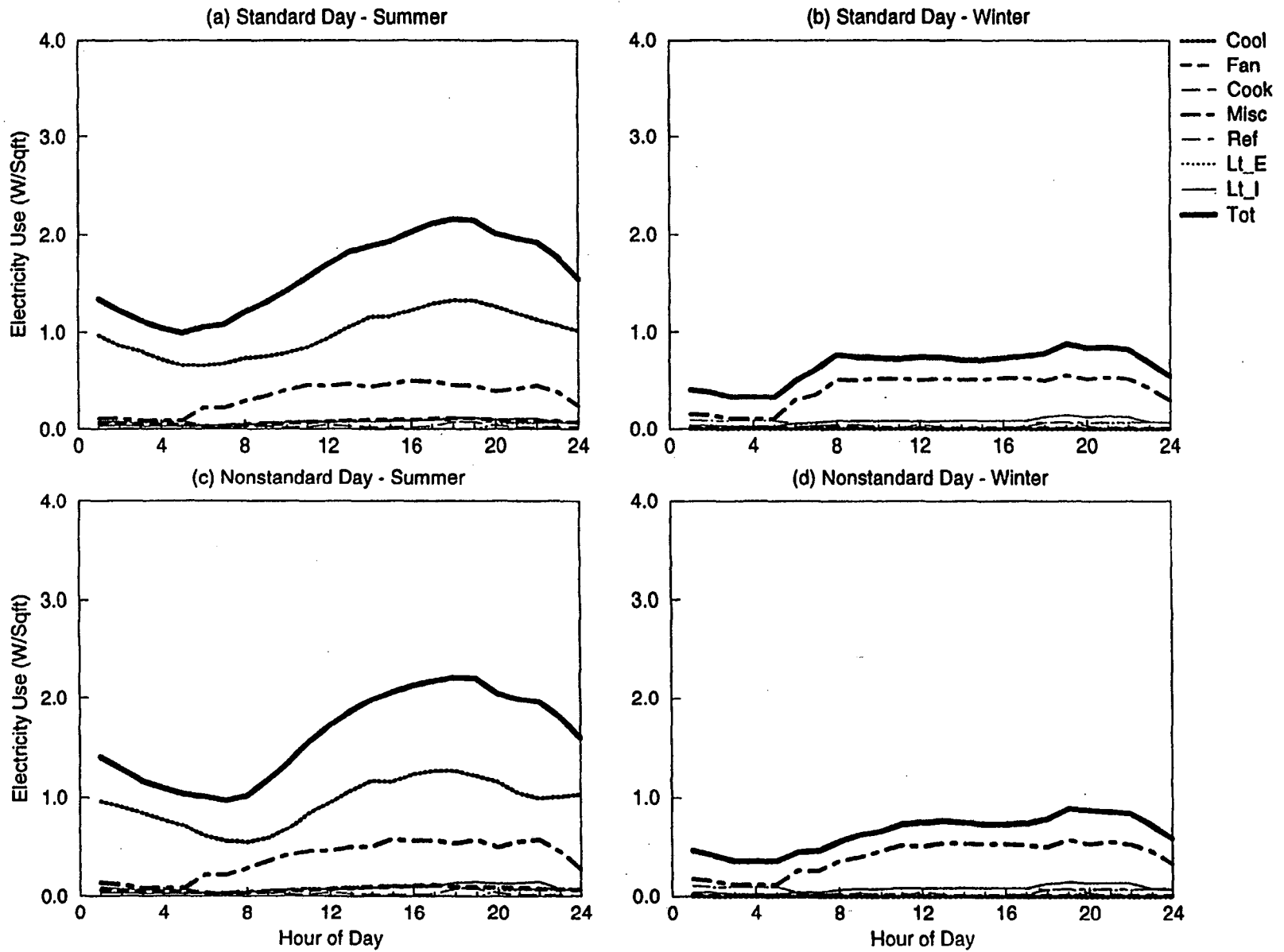
Figure C-52. EDA Reconciled End-use Load Shapes for Detached Residential (Feeder W4)
