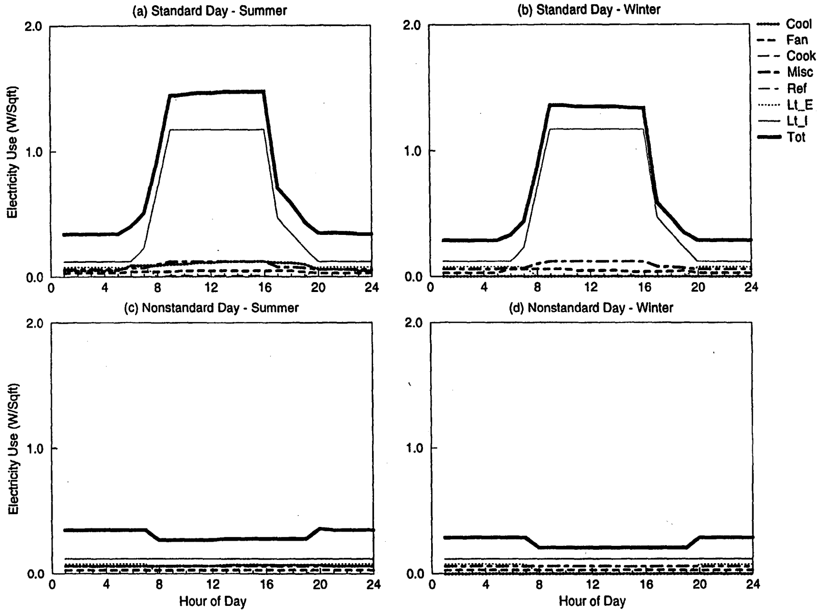
Figure B-14. DOE-2 Simulated End-use Load Shapes for Large Vehicle Maintenance (Chiller)
