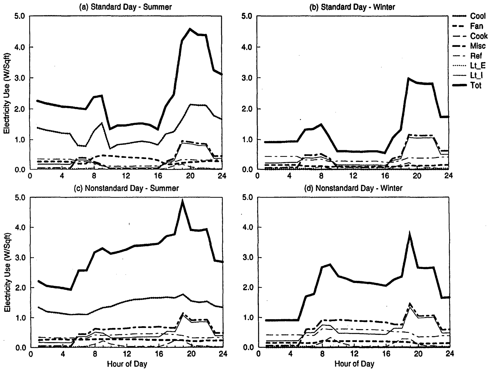
Figure C-11. EDA Reconciled End-use Load Shapes for Modular Barrack (Feeder W6)
