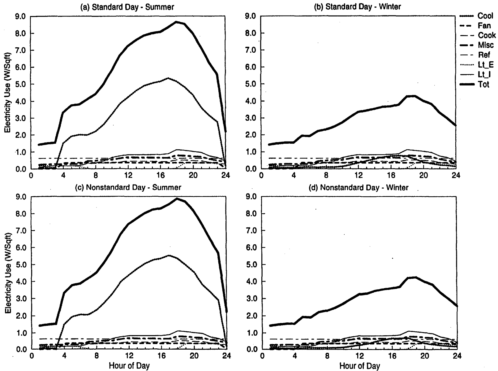
Figure B-28. DOE-2 Simulated End-use Load Shapes for Sitdown Restaurant
