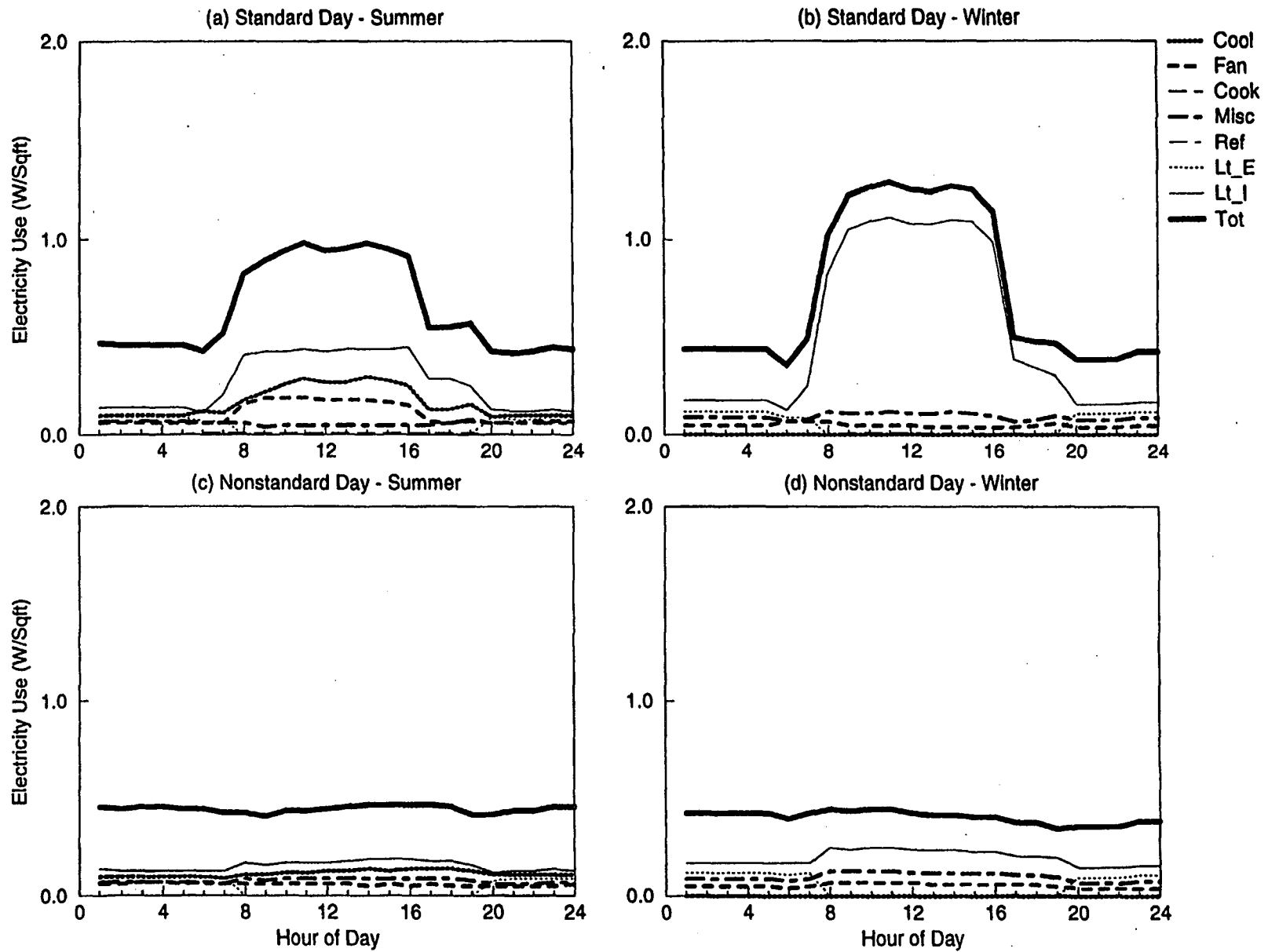
Figure C-47. EDA Reconciled End-use Load Shapes for Large Vehicle Maintenance (Chiller) (Feeder W6)
