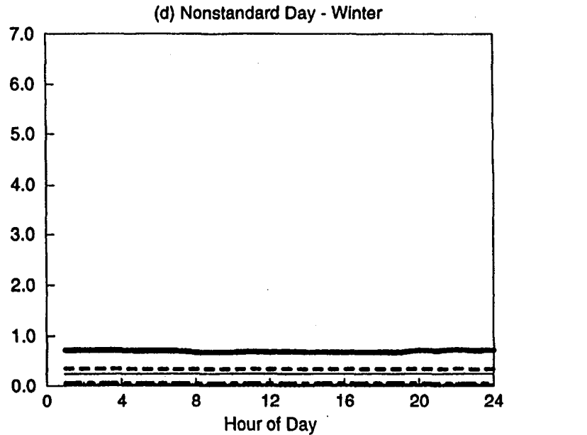
Figure B-8. DOE-2 Simulated End-use Load Shapes for Small Administration (Old w/ Split DX)
