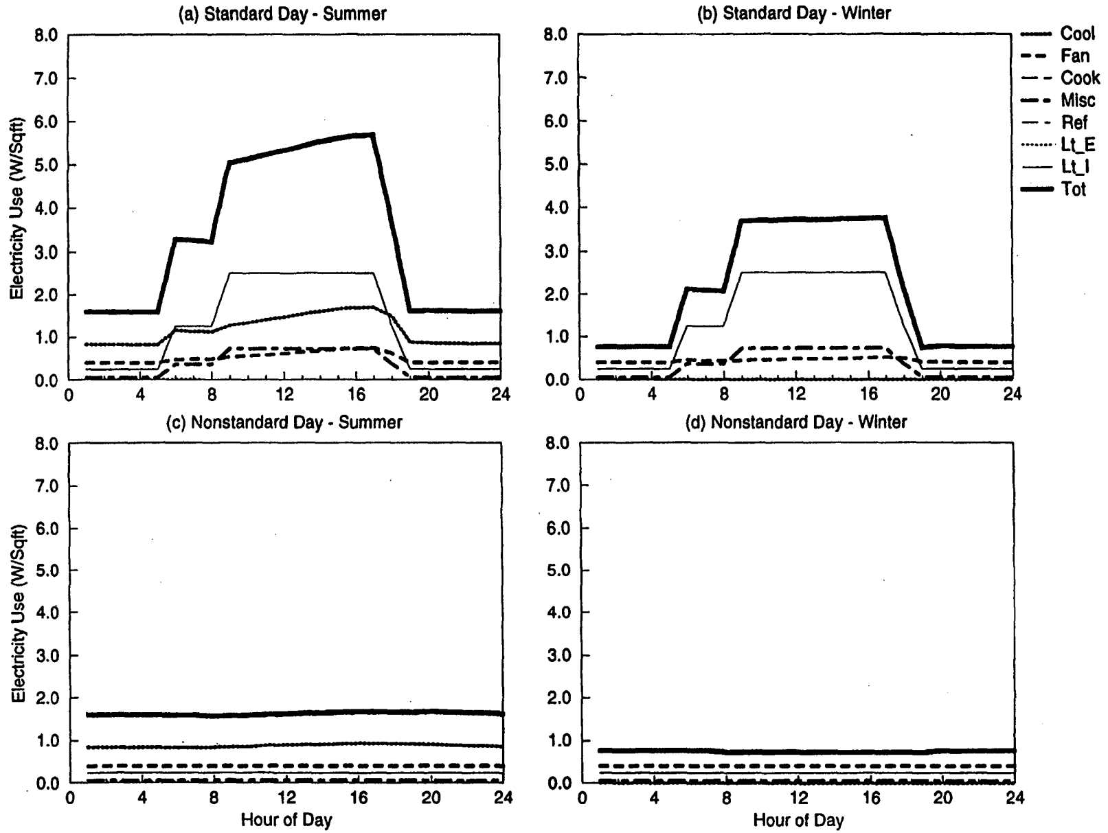
Figure B-11. DOE-2 Simulated End-use Load Shapes for Small Administration (New w/ Chiller)
