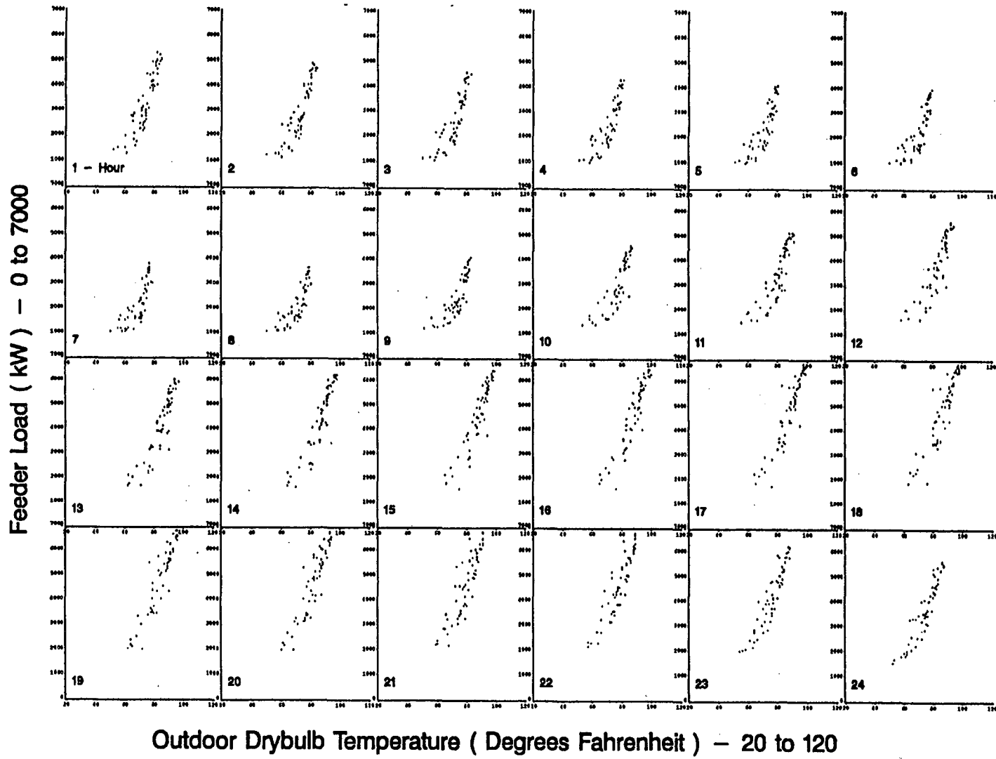
Figure A-45. Scatterplots of Feeder W4 Hourly Load vs. Drybulb Temperature for non-Standard Summer Days
