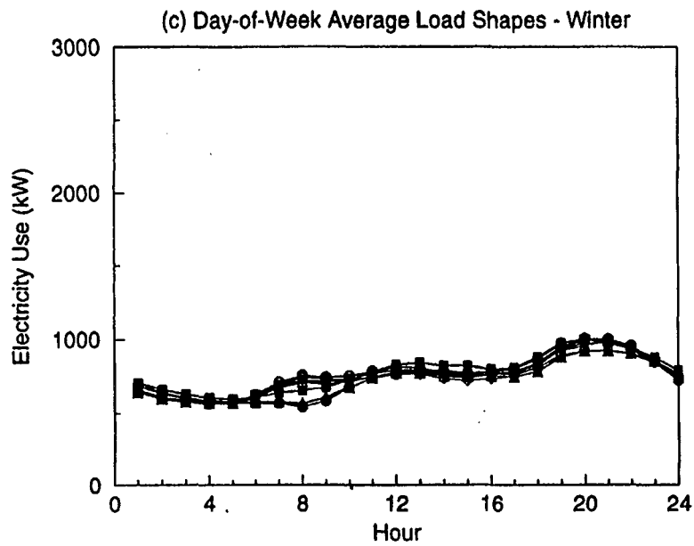
Figure A-31. Feeder 12 Data
