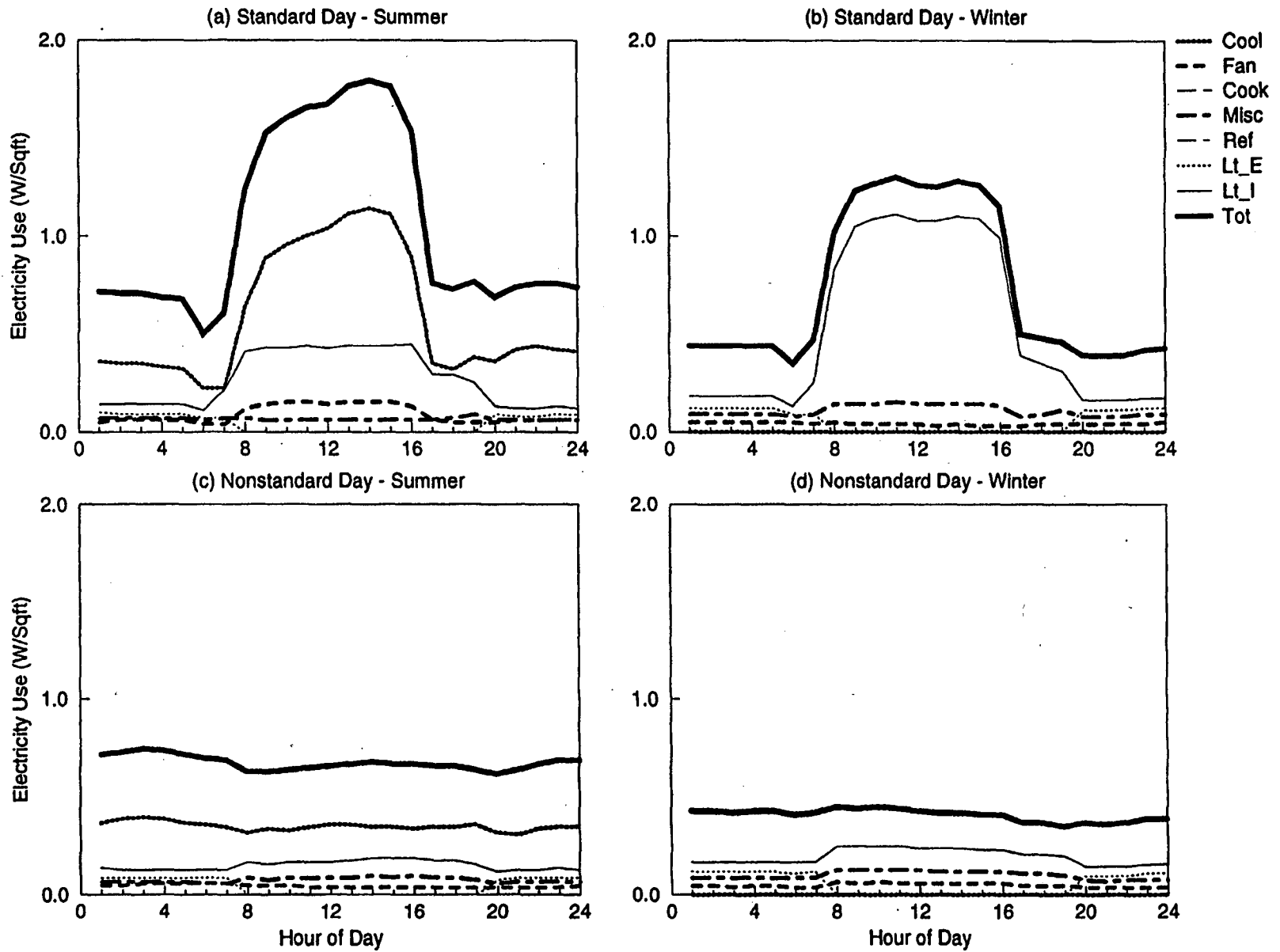
Figure C-64. EDA Reconciled End-use Load Shapes for Warehouse (Split DX) (Feeder W6)
