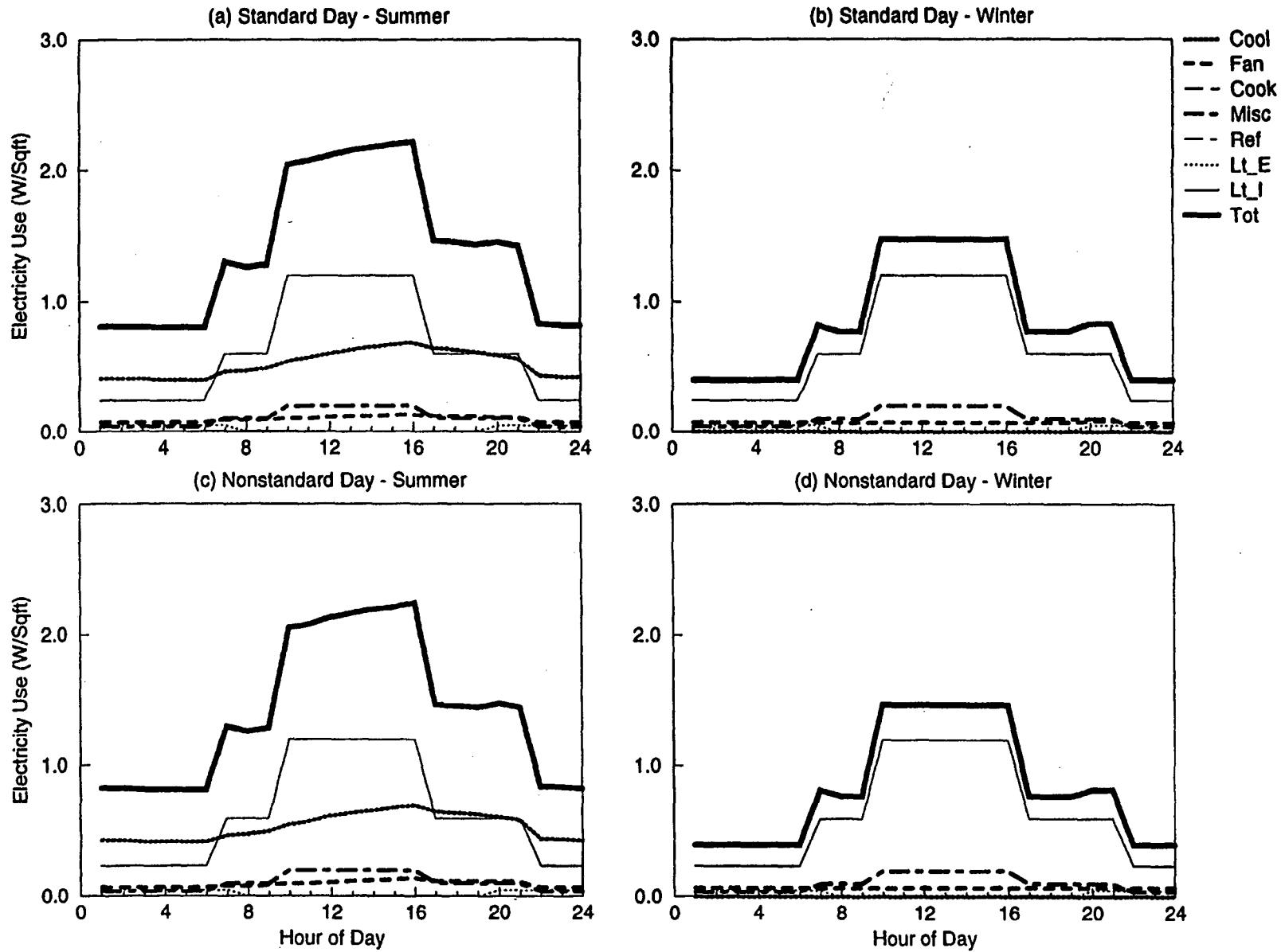
Figure B-24. DOE-2 Simulated End-use Load Shapes for Church
