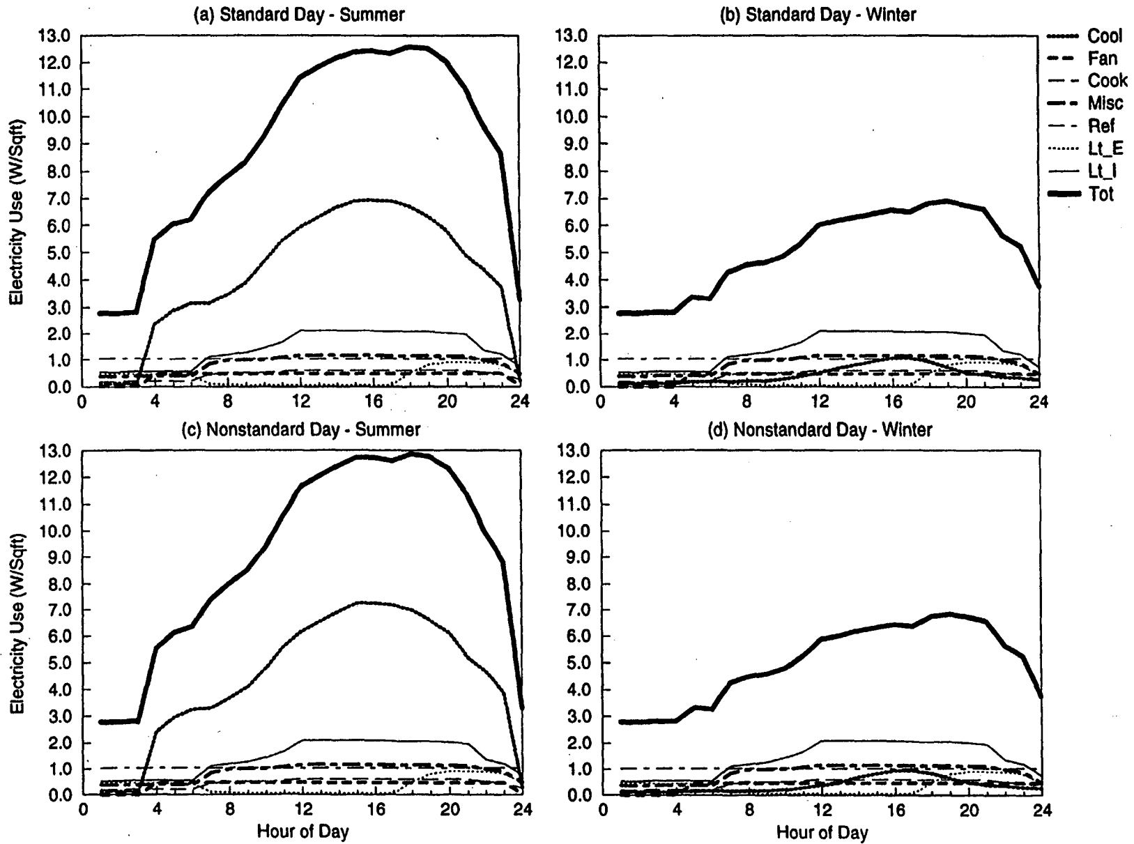
Figure B-27. DOE-2 Simulated End-use Load Shapes for Fastfood Restaurant
