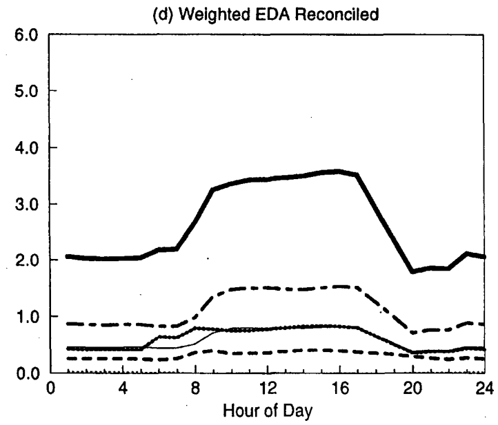
Figure 3-6. Large Administration Load Shapes for Standard Day - Summer.
