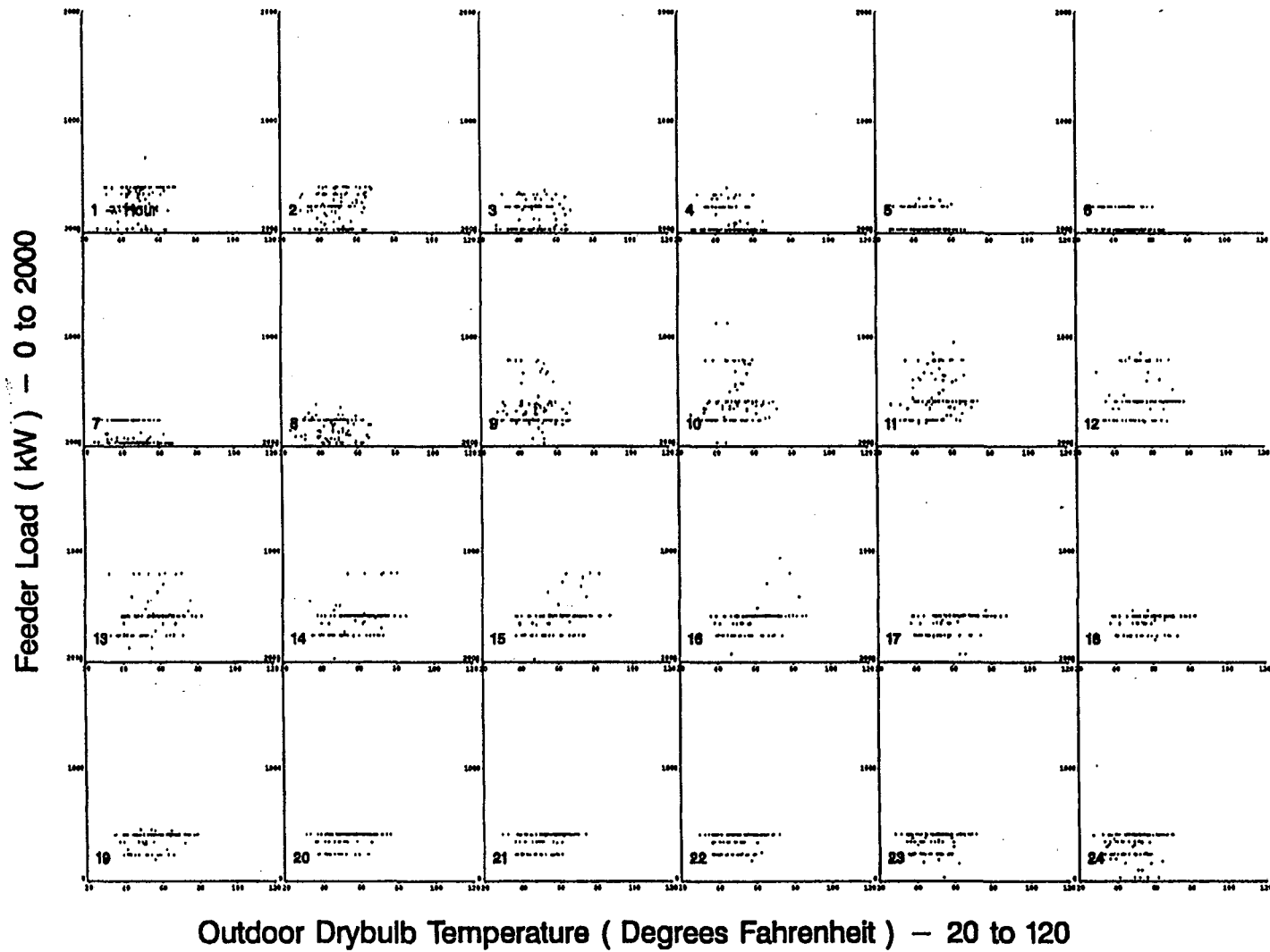
Figure A-12. Scatterplots of Feeder 4 Hourly Load vs. Drybulb Temperature for Standard Winter Days
