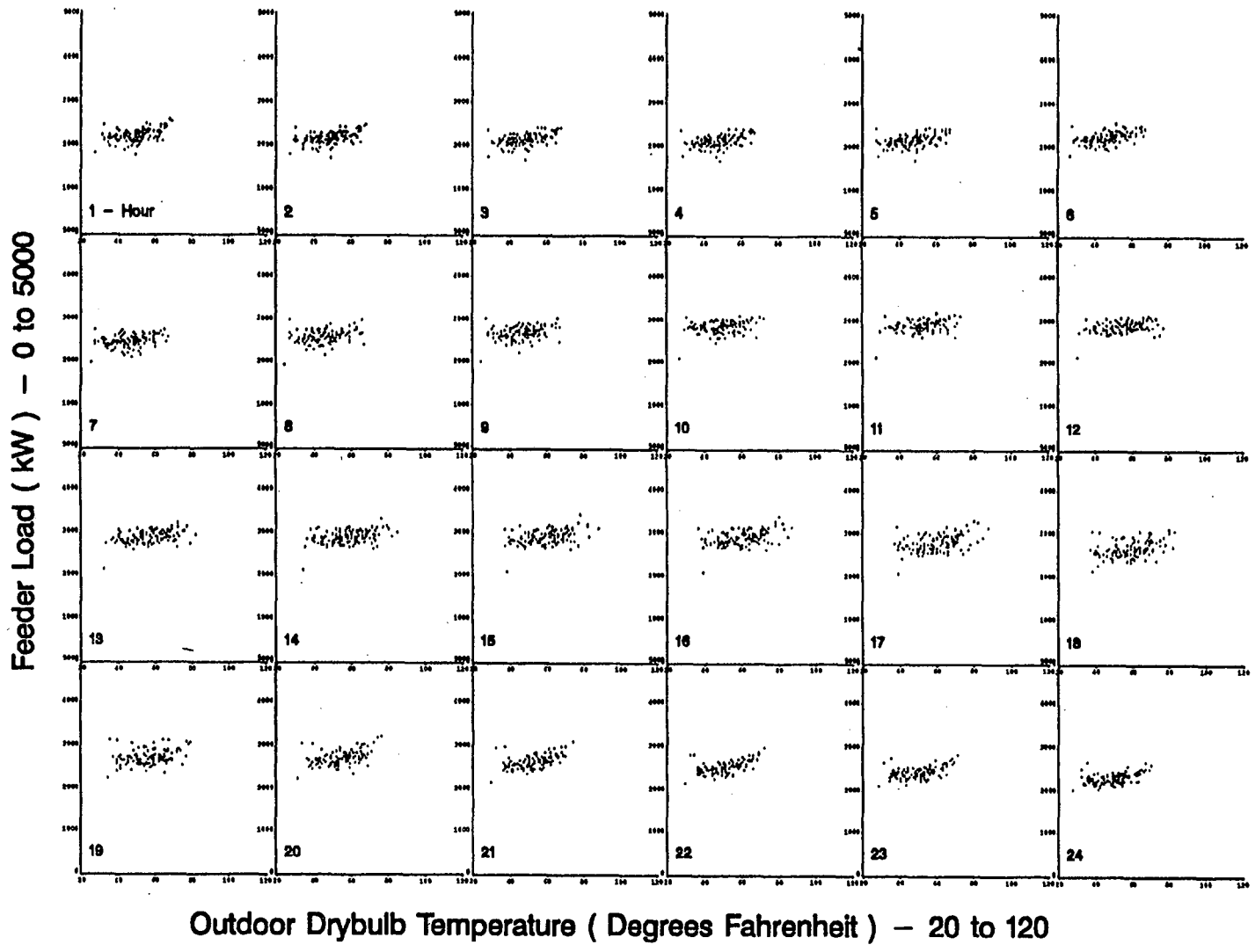
Figure A-47. Scatterplots of Feeder W5 Hourly Load vs. Drybulb Temperature for Standard Winter Days
