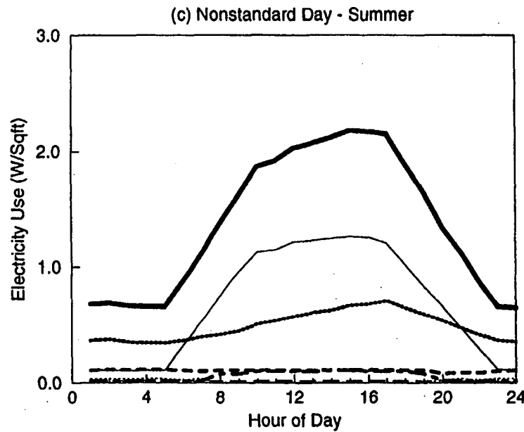
Figure C-20. EDA Reconciled End-use Load Shapes for Gymnasium (Feeder 15)
