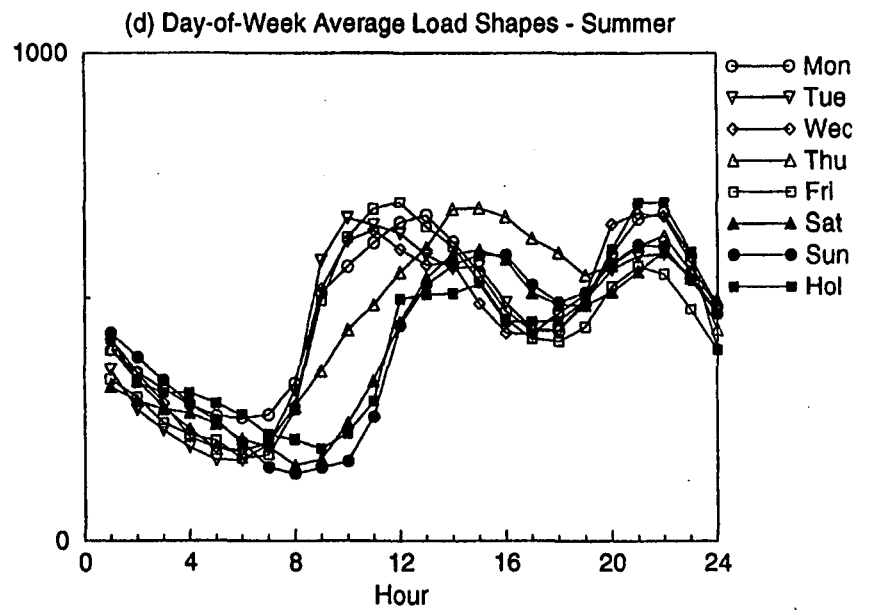
Figure A-11. Feeder 4 Data
