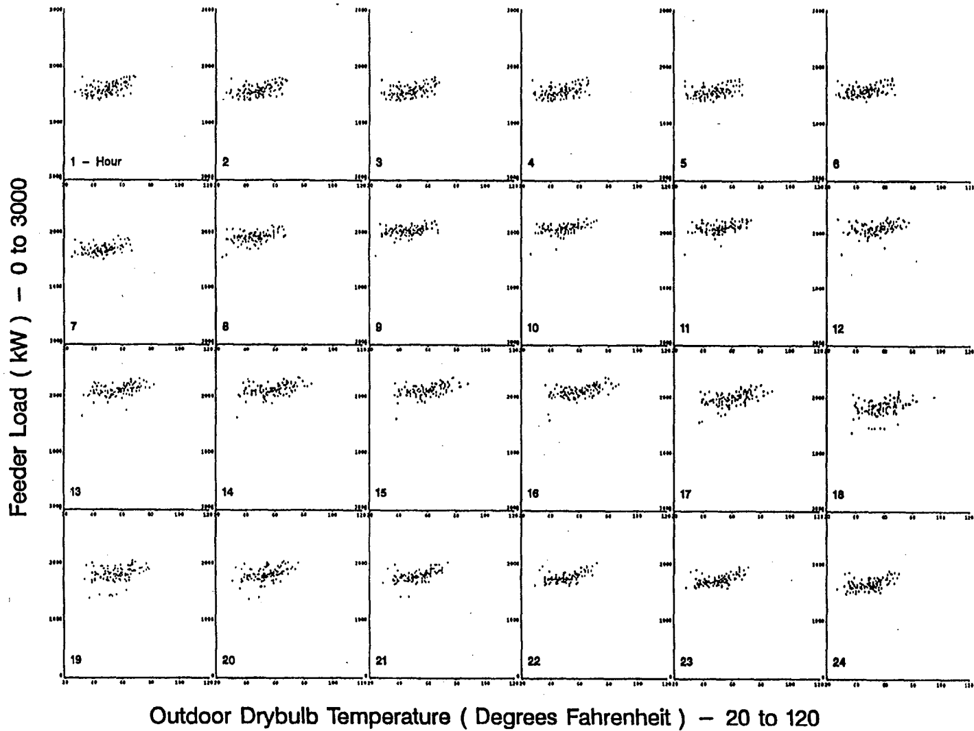
Figure A-2. Scatterplots of Feeder 2 Hourly Load vs. Drybulb Temperature for Standard Winter Days
