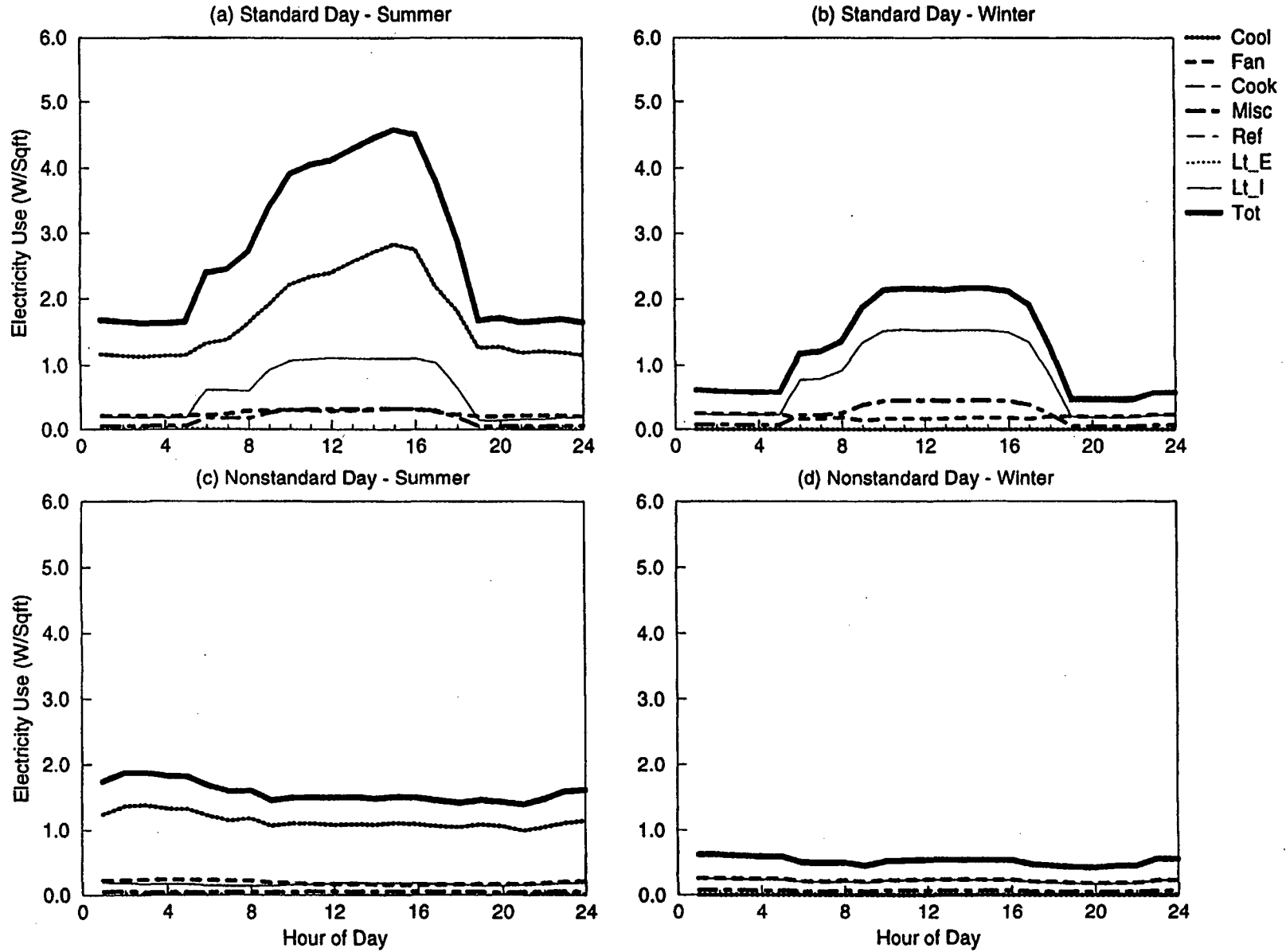
Figure C-34. EDA Reconciled End-use Load Shapes for Small Administration (New w/ Split DX) (Feeder 10)
