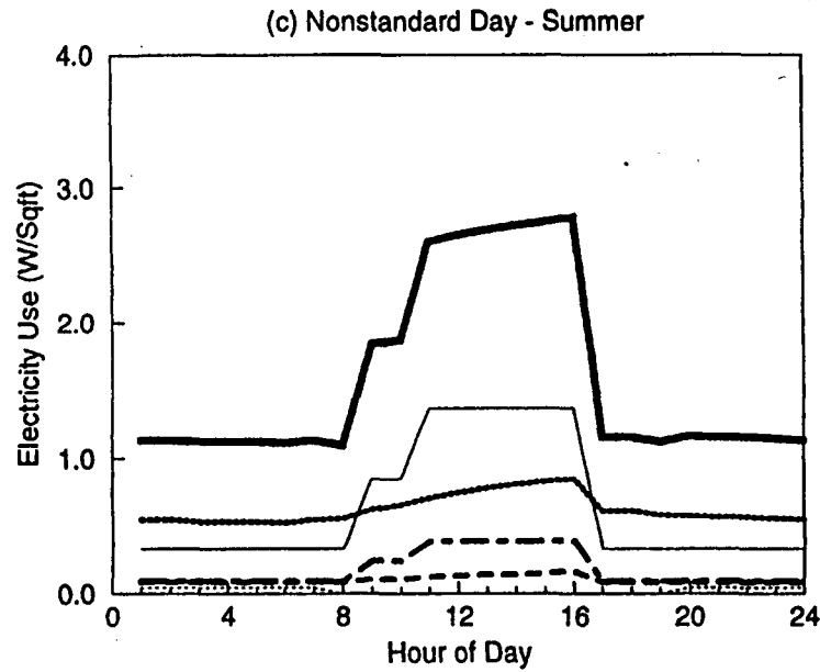
Figure B-30. DOE-2 Simulated End-use Load Shapes for Youth Center
