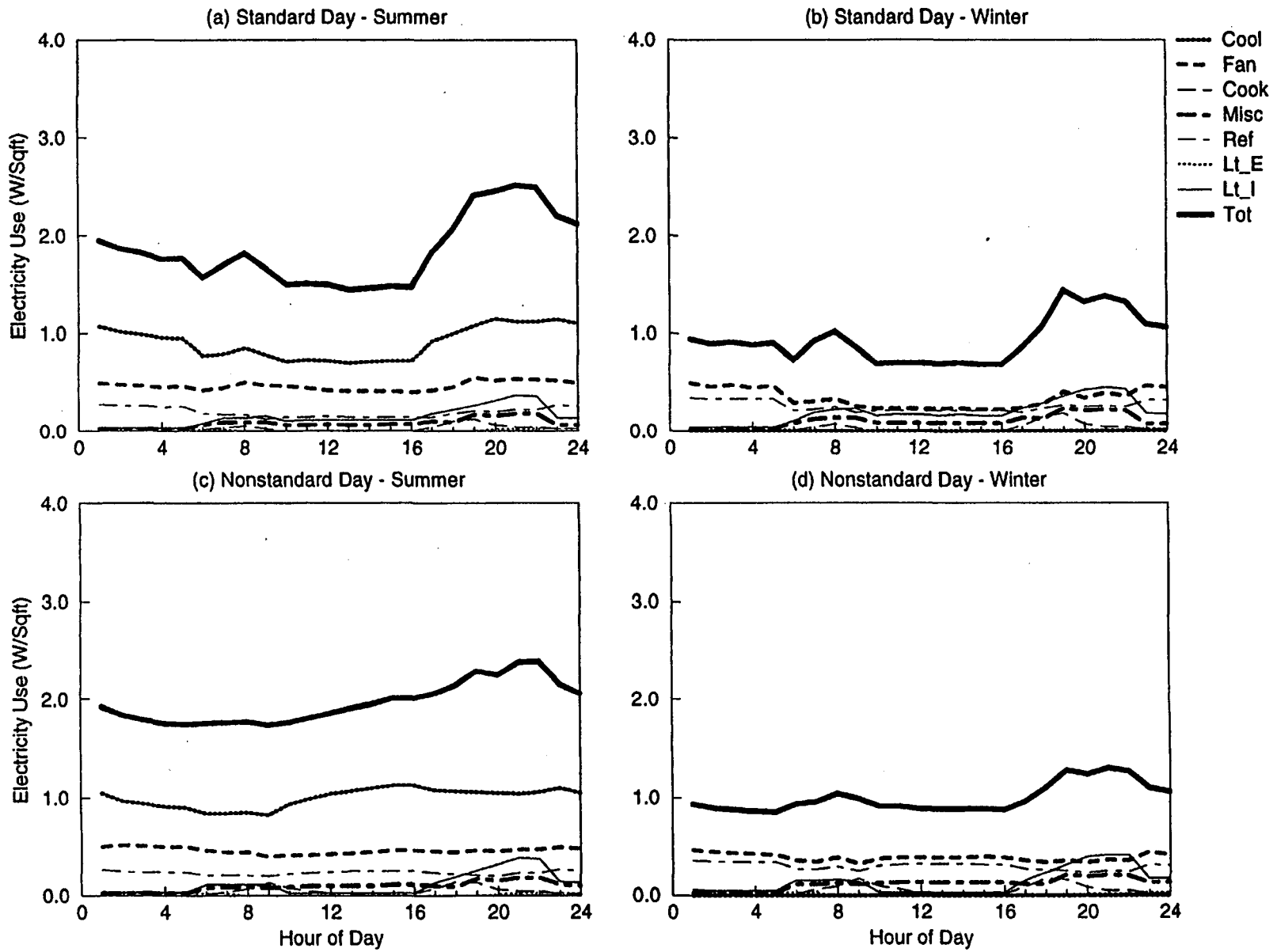
Figure C-6. EDA Reconciled End-use Load Shapes for Rolling Pin Barrack (Feeder 10)
