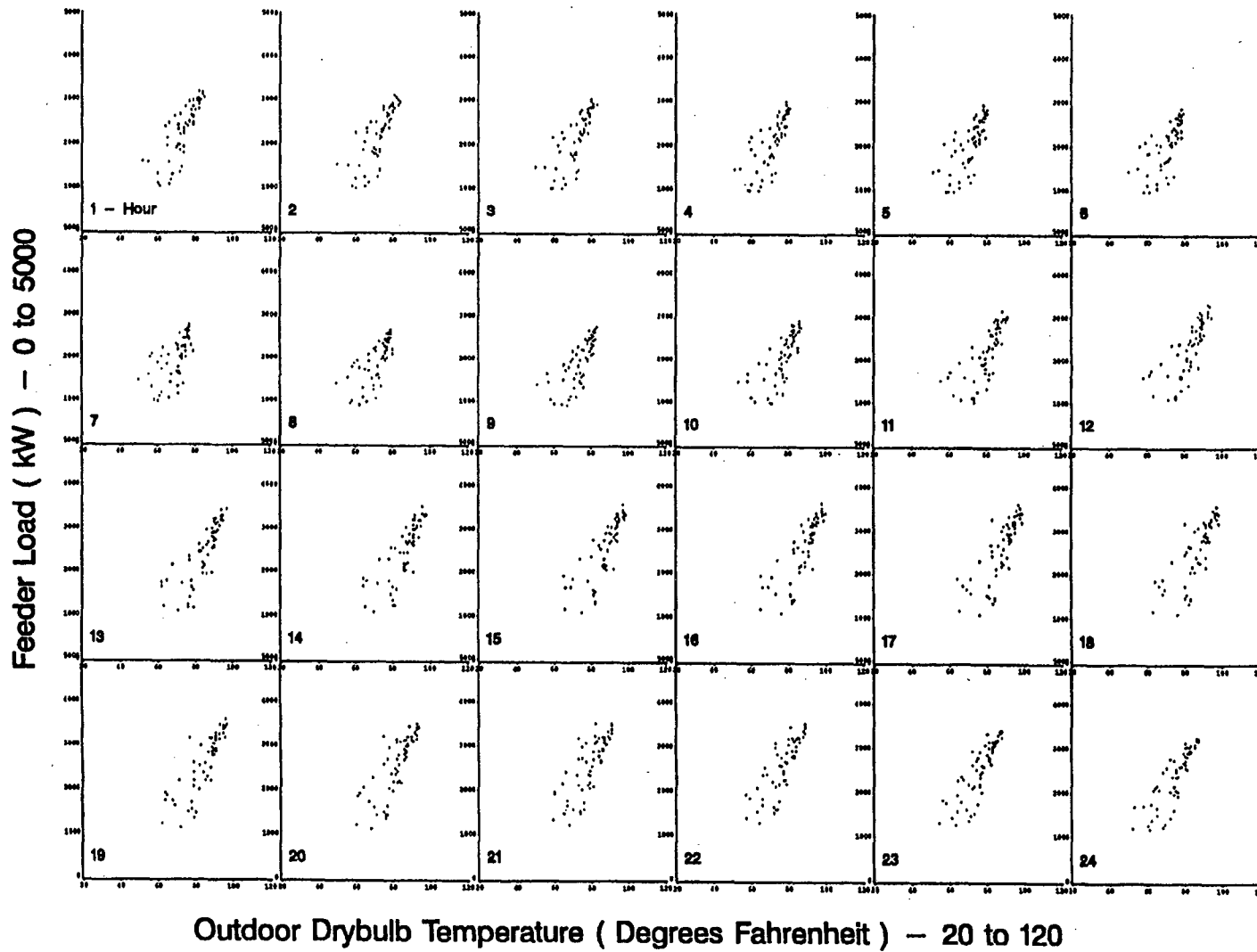
Figure A-10. Scatterplots of Feeder 3 Hourly Load vs. Drybulb Temperature for non-Standard Summer Days
