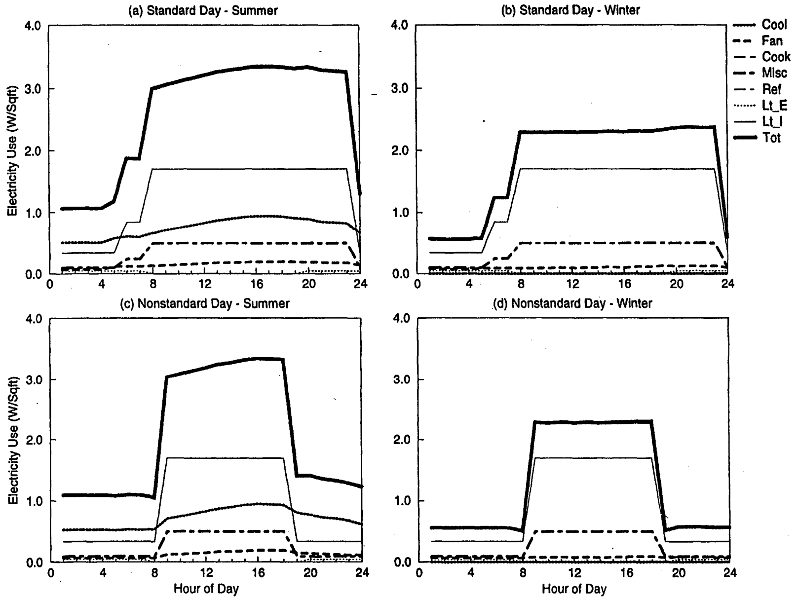
Figure B-25. DOE-2 Simulated End-use Load Shapes for Grocery Store
