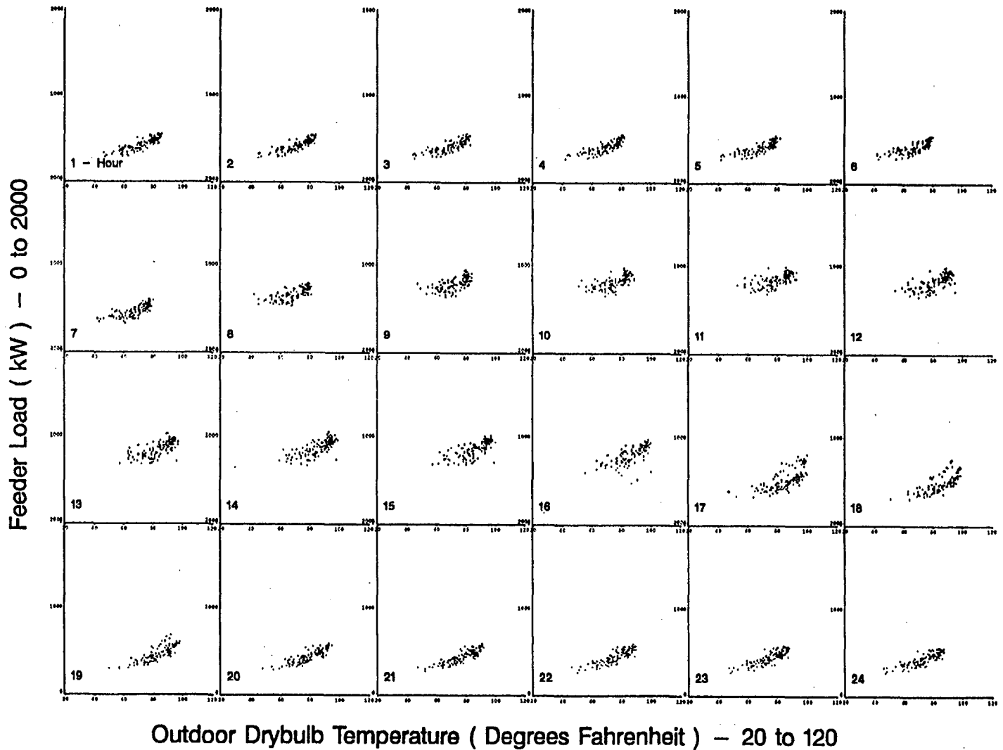
Figure A-54. Scatterplots of Feeder W6 Hourly Load vs. Drybulb Temperature for Standard Summer Days
