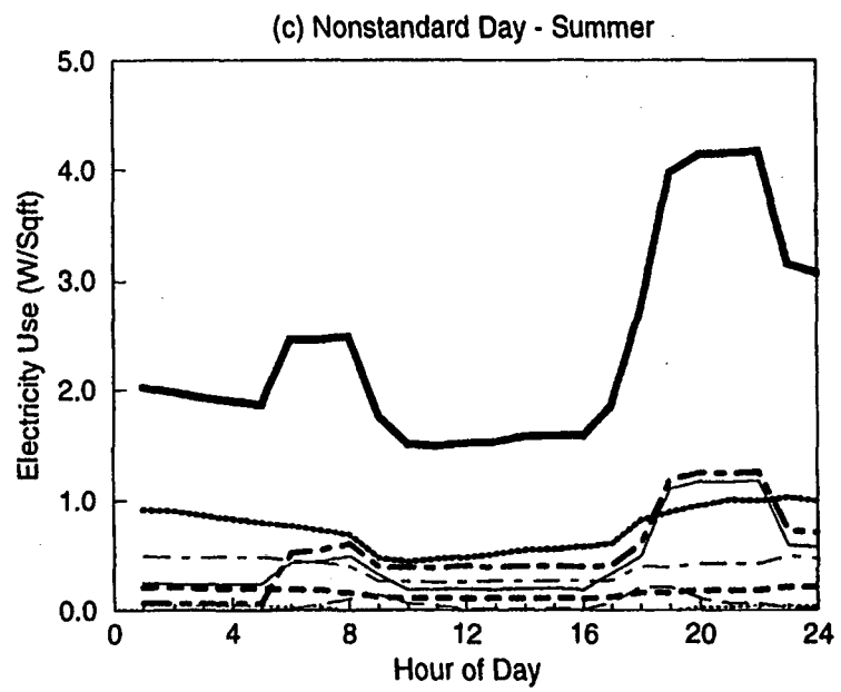
Figure C-8. EDA Reconciled End-use Load Shapes for Modular Barrack (Feeder 2)
