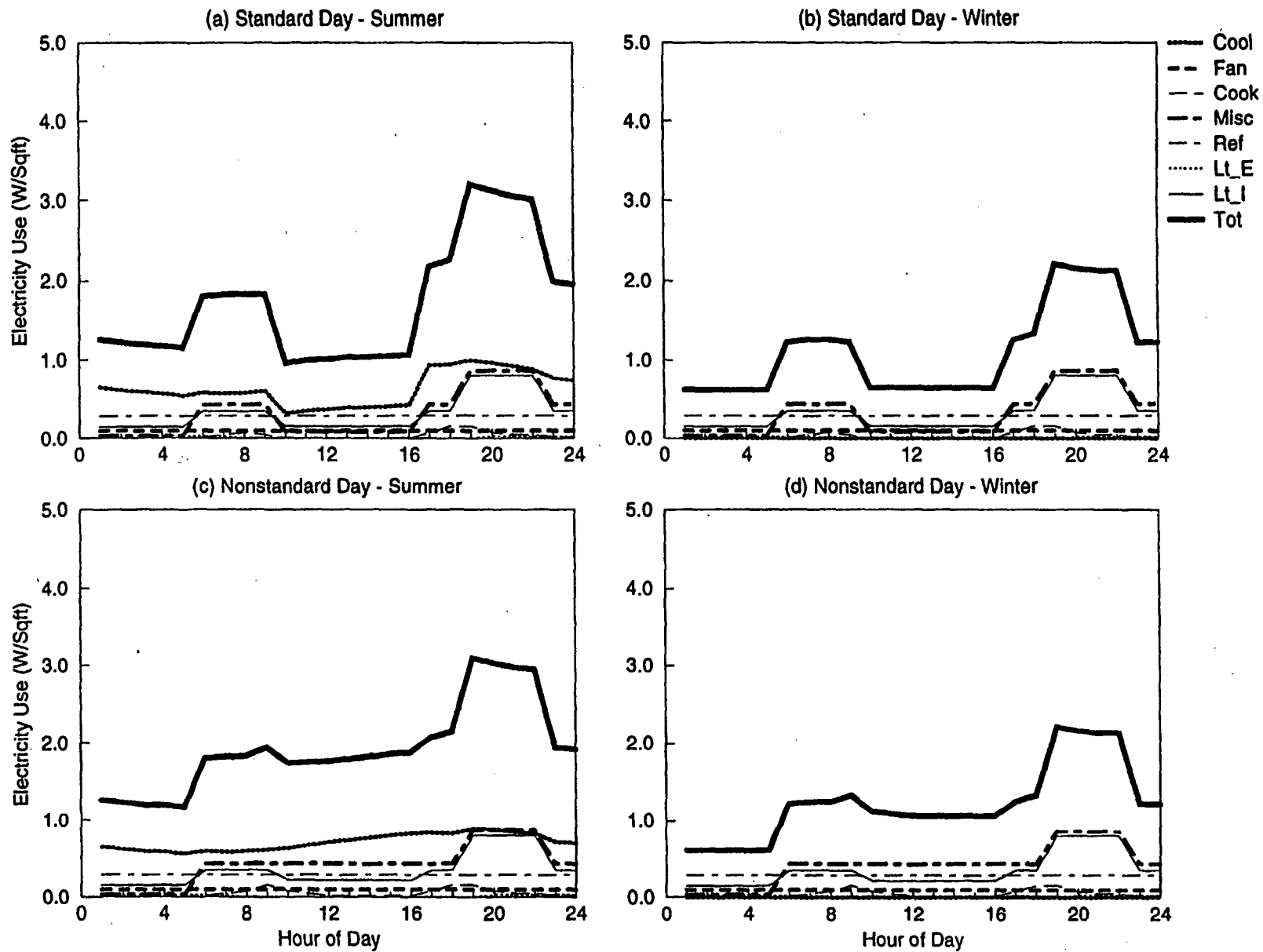
Figure B-3. DOE-2 Simulated End-use Load Shapes for Modular Barrack
