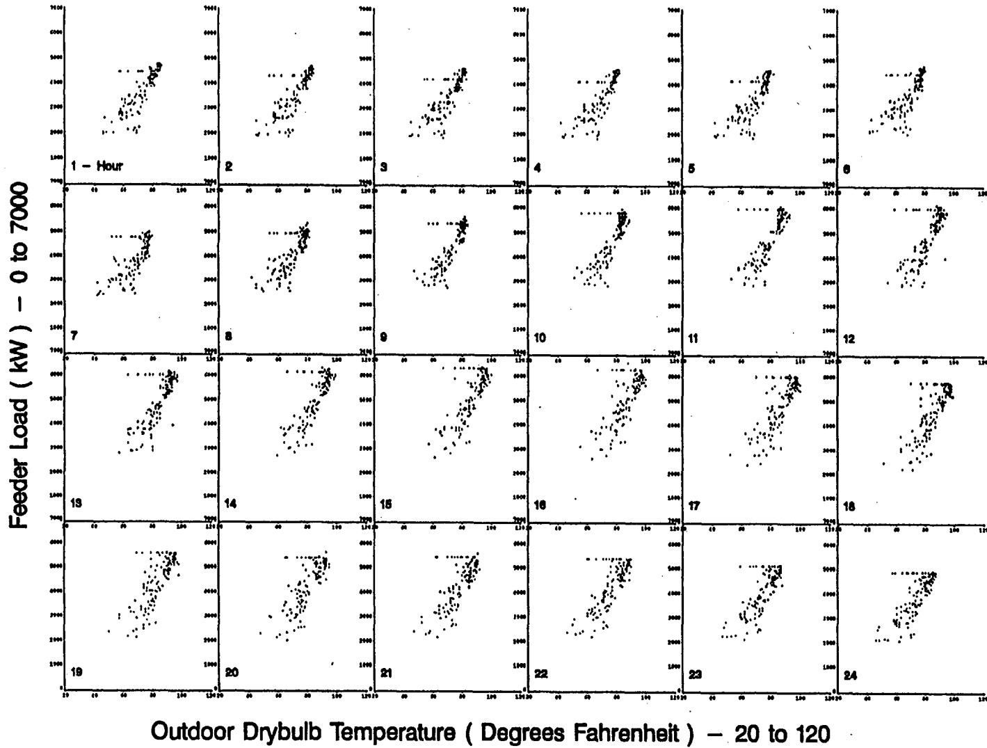
Figure A-29. Scatterplots of Feeder 10 Hourly Load vs. Drybulb Temperature for Standard Summer Days
