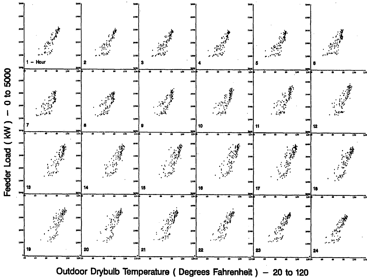
Figure A-9. Scatterplots of Feeder 3 Hourly Load vs. Drybulb Temperature for Standard Summer Days
