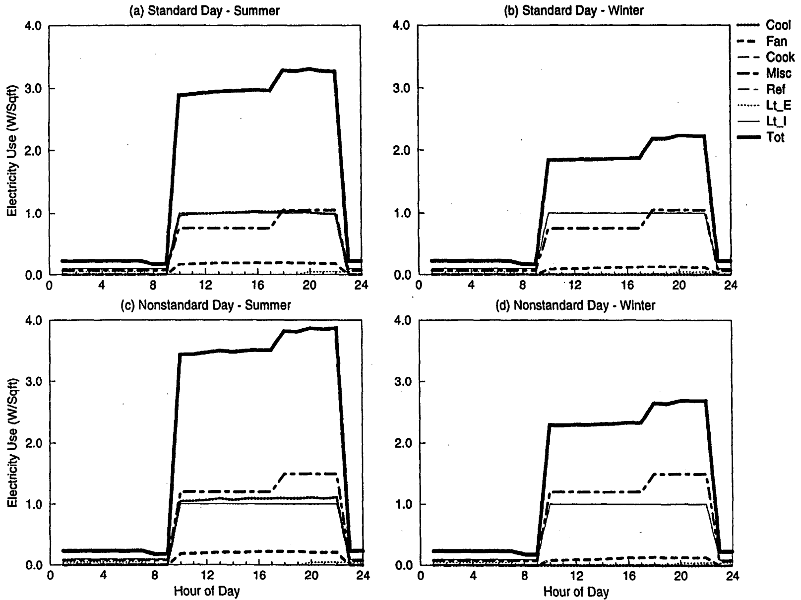
Figure B-23. DOE-2 Simulated End-use Load Shapes for Bowling Center
