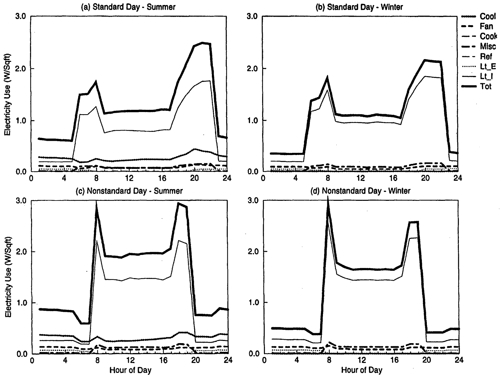
Figure C-19. EDA Reconciled End-use Load Shapes for Gymnasium (Feeder 2)
