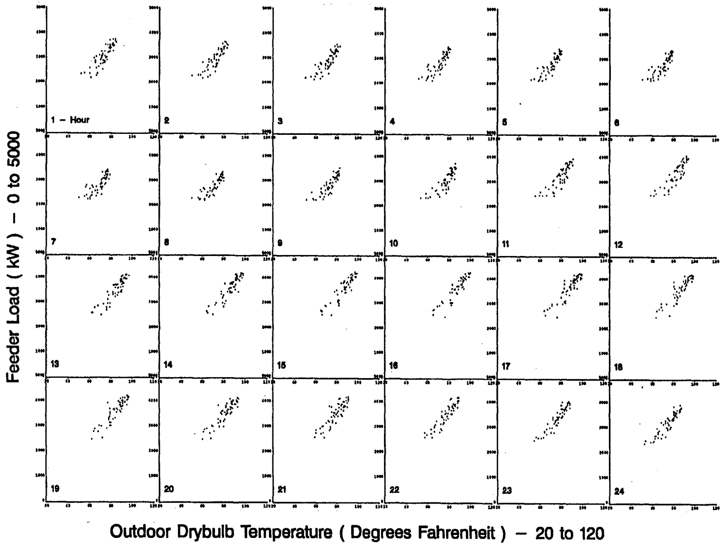
Figure A-50. Scatterplots of Feeder W5 Hourly Load vs. Drybulb Temperature for non-Standard Summer Days
