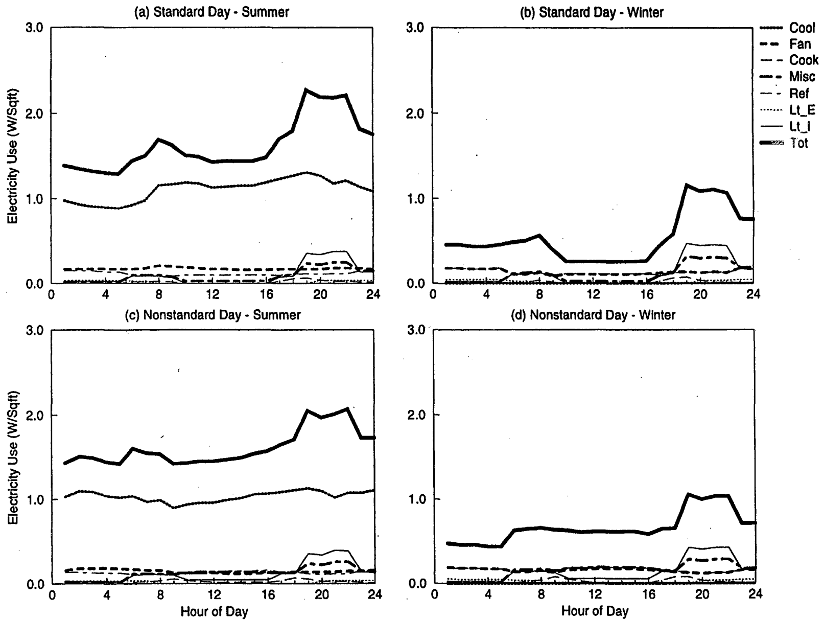
Figure C-13. EDA Reconciled End-use Load Shapes for Small Barrack (Feeder 10)
