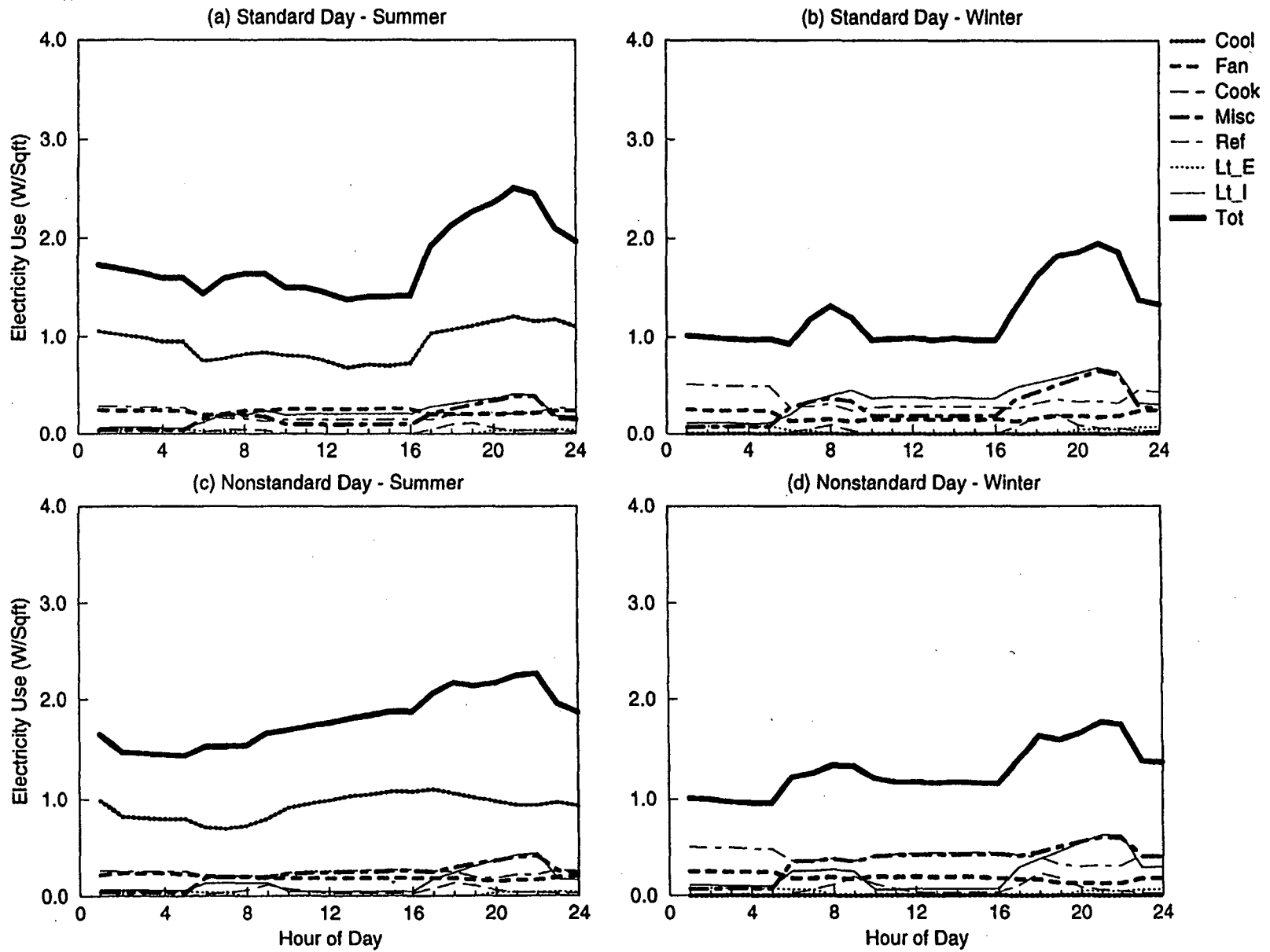
Figure C-3. EDA Reconciled End-use Load Shapes for Hammerhead Barrack (Feeder 15)
