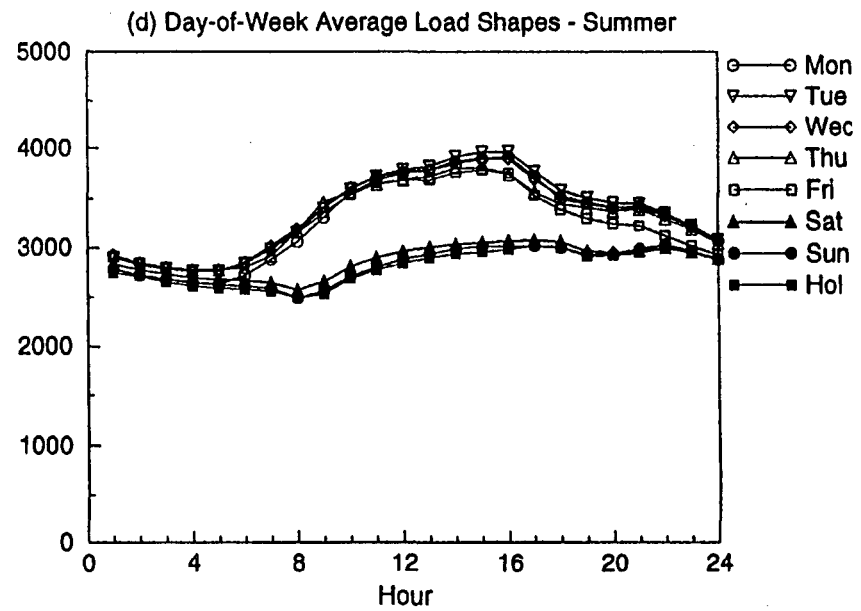
Figure A-36. Feeder 15 Data
