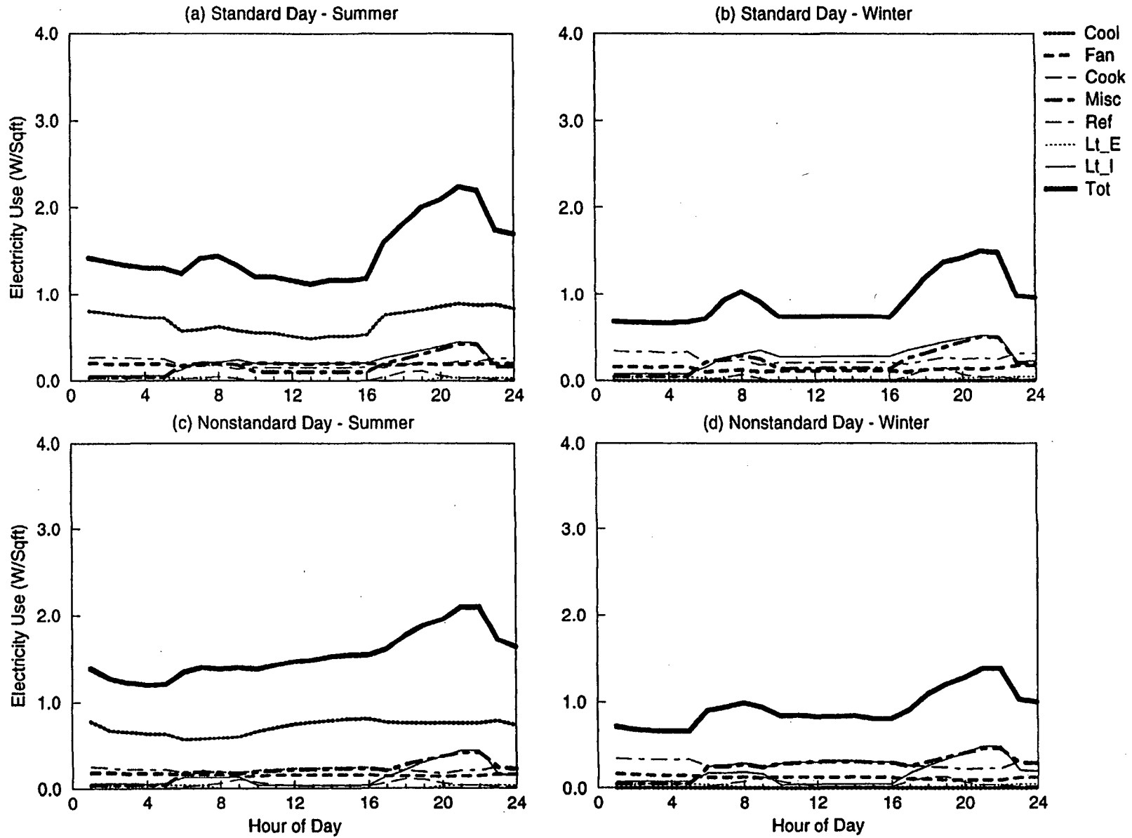
Figure C-2. EDA Reconciled End-use Load Shapes for Hammerhead Barrack (Feeder 10)
