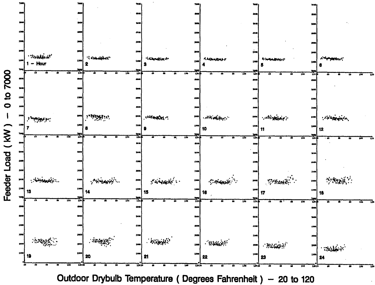
Figure A-17. Scatterplots of Feeder 5 Hourly Load vs. Drybulb Temperature for Standard Winter Days
