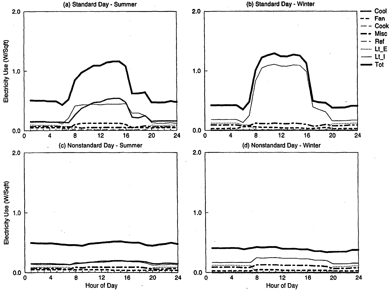
Figure C-44. EDA Reconciled End-use Load Shapes for Large Vehicle Maintenance (Split DX) (Feeder W6)
