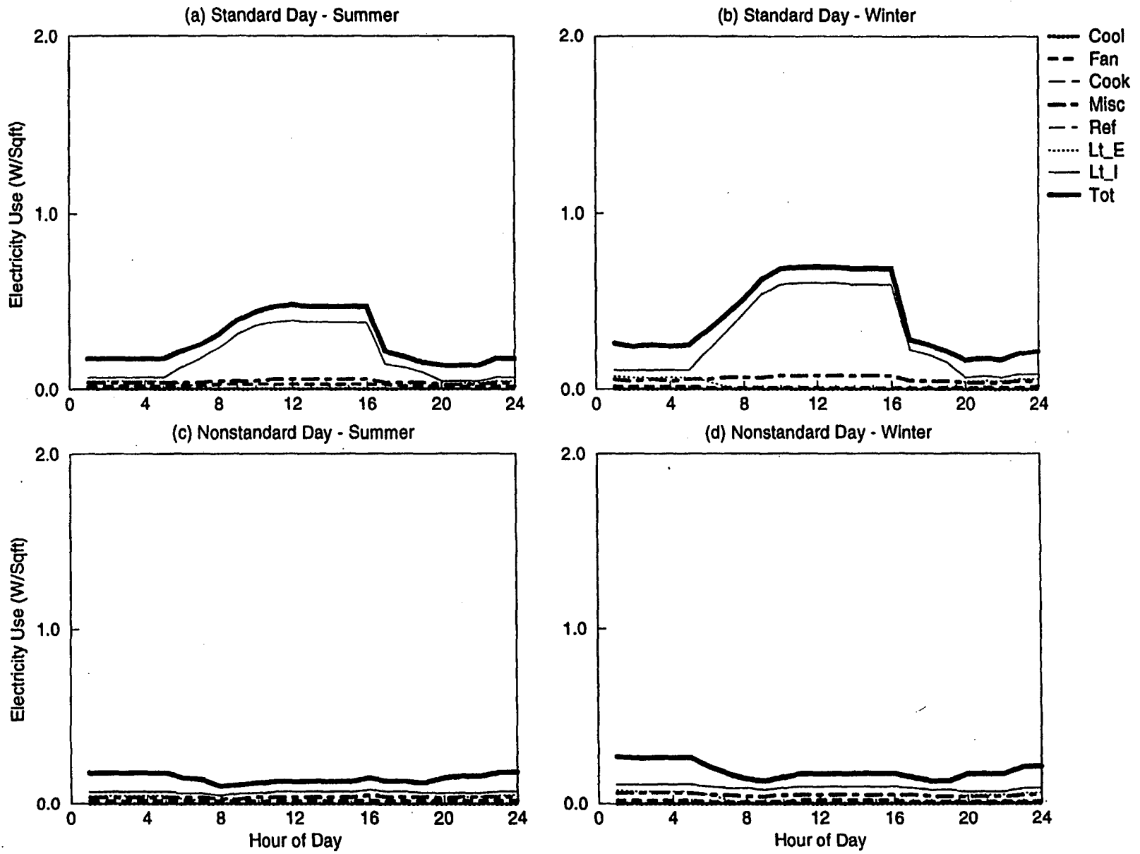
Figure C-63. EDA Reconciled End-use Load Shapes for Warehouse (No AC) (Feeder 3)
