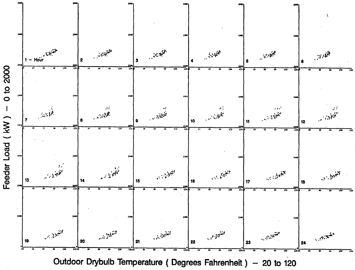
Figure A-55. Scatterplots of Feeder W6 Hourly Load vs. Drybulb Temperature for non-Standard Summer Days
