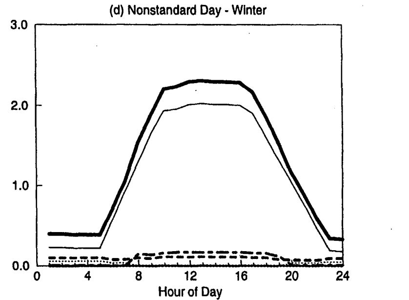
Figure C-20. EDA Reconciled End-use Load Shapes for Gymnasium (Feeder 15)
