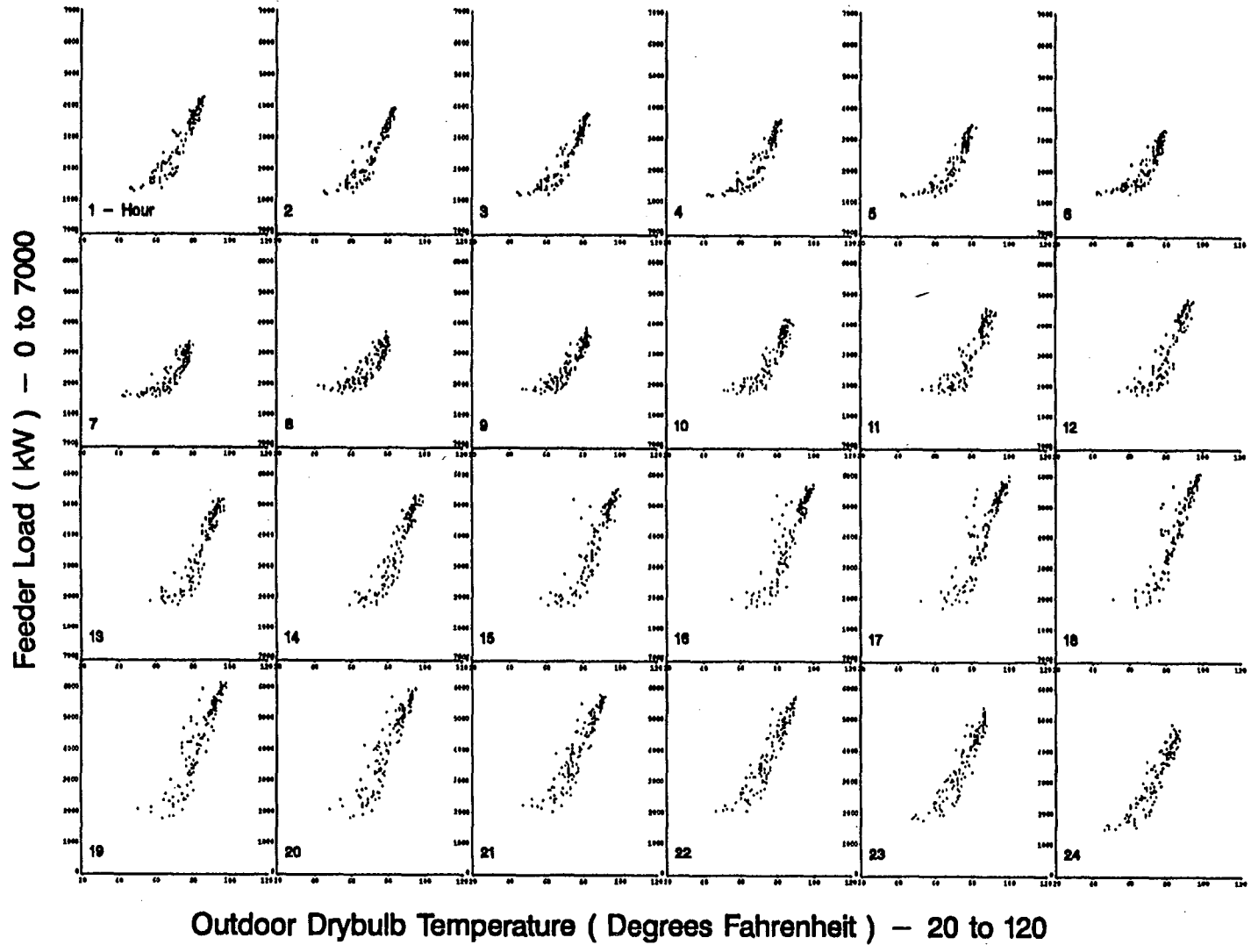
Figure A-19. Scatterplots of Feeder 5 Hourly Load vs. Drybulb Temperature for Standard Summer Days
