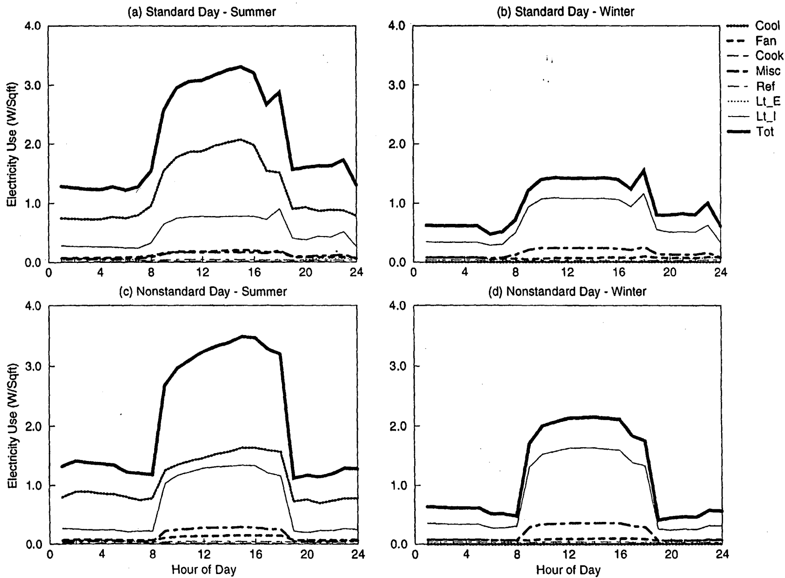
Figure C-68. EDA Reconciled End-use Load Shapes for Miscellaneous (Feeder 10)
