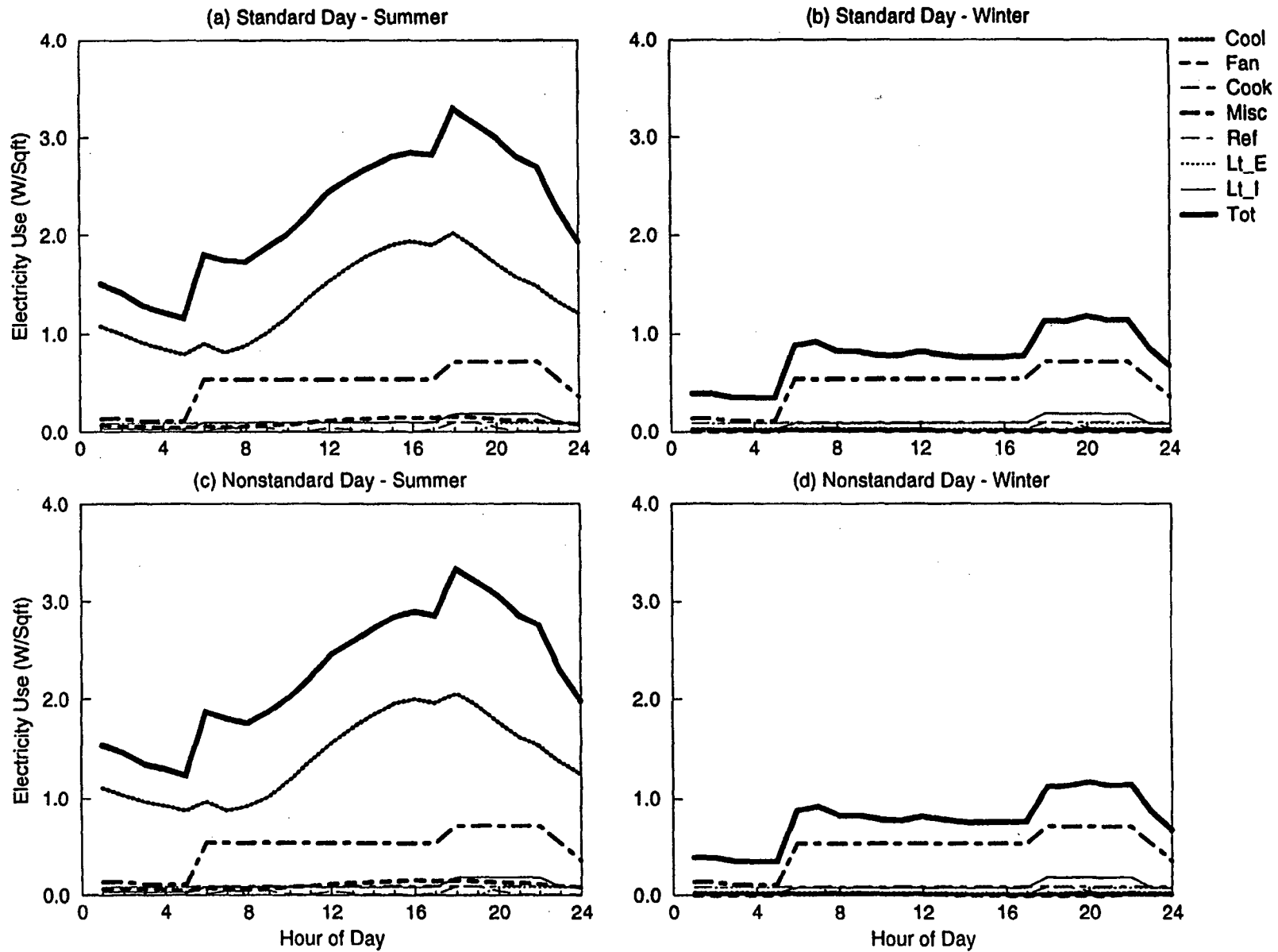
Figure B-18. DOE-2 Simulated End-use Load Shapes for Two-Plex Residential
