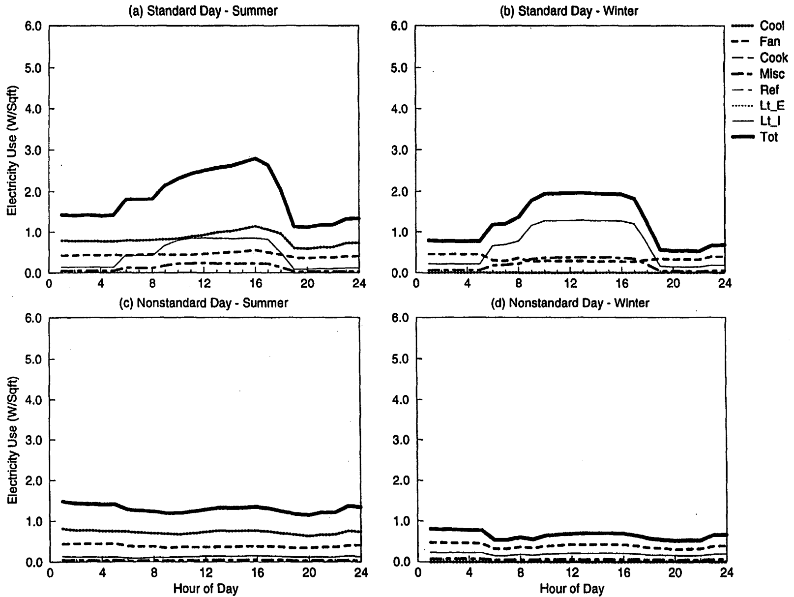
Figure C-29. EDA Reconciled End-use Load Shapes for Small Administration (Old w/ Chiller) (Feeder 3)
