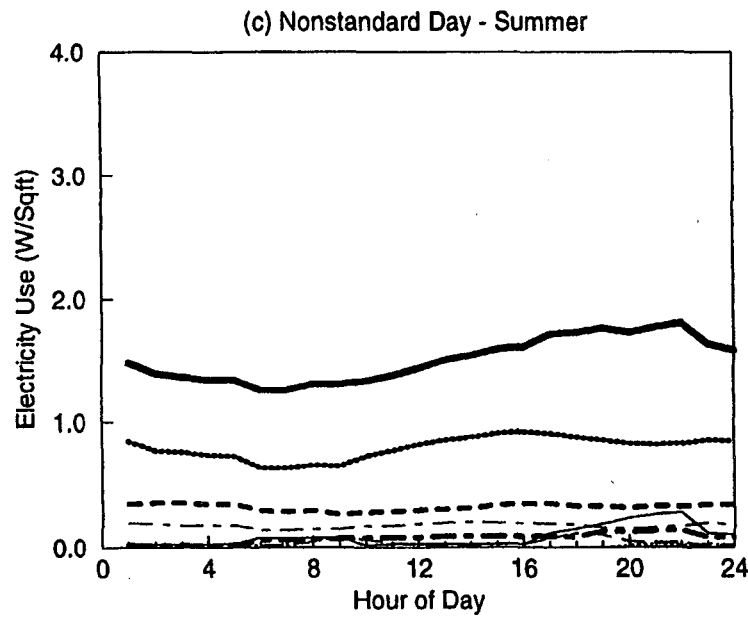
Figure C-5. EDA Reconciled End-use Load Shapes for Rolling Pin Barrack (Feeder 3)
