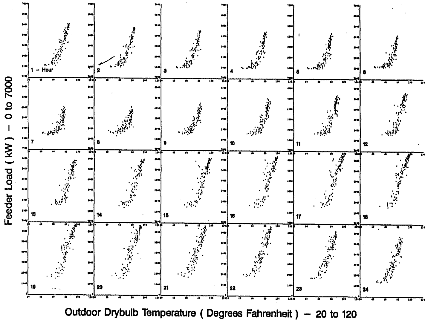
Figure A-44. Scatterplots of Feeder W4 Hourly Load vs. Drybulb Temperature for Standard Summer Days
