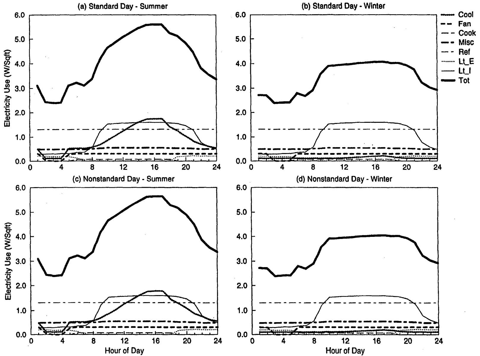
Figure B-26. DOE-2 Simulated End-use Load Shapes for Library
