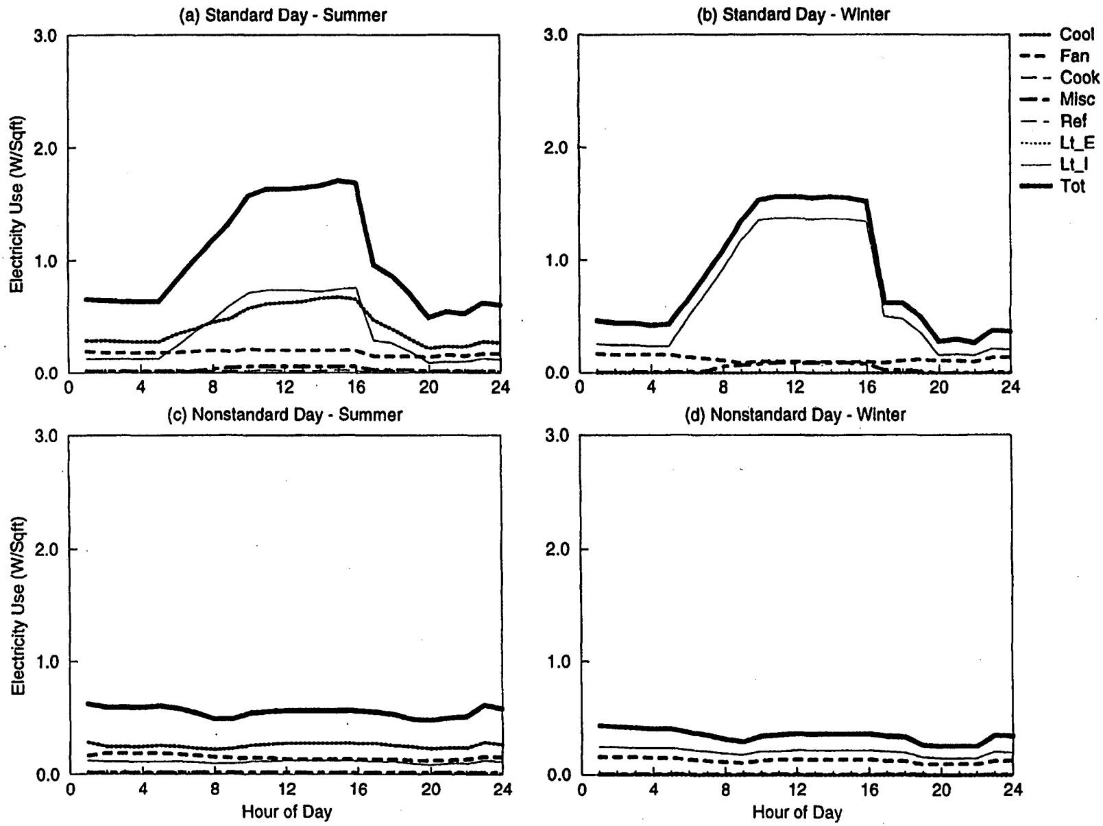
Figure C-48. EDA Reconciled End-use Load Shapes for Hangar (Feeder 15)
