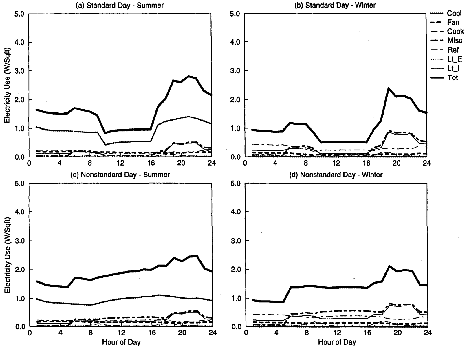
Figure C-10. EDA Reconciled End-use Load Shapes for Modular Barrack (Feeder 15)
