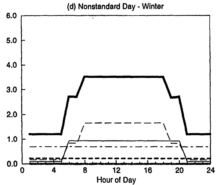
Figure B-5. DOE-2 Simulated End-use Load Shapes for Dining Hall
