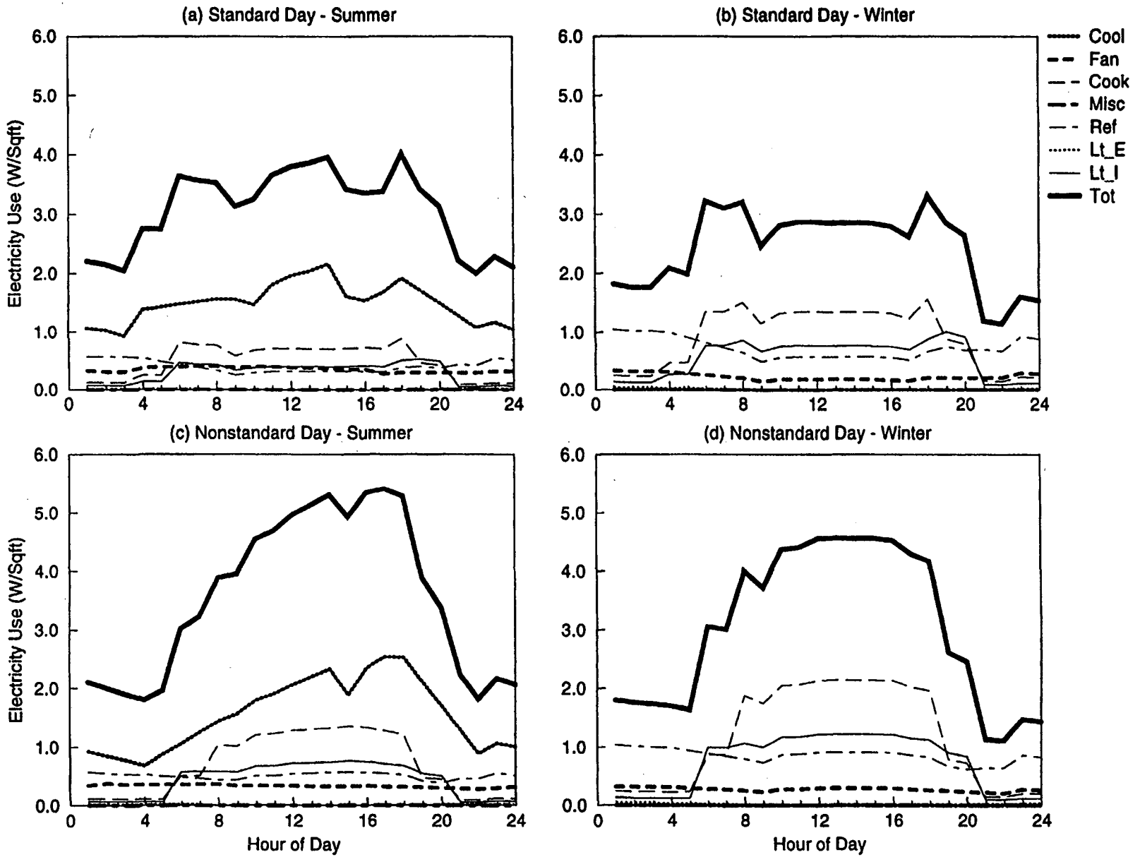
Figure C-17. EDA Reconciled End-use Load Shapes for Dining Hall (Feeder 15)
