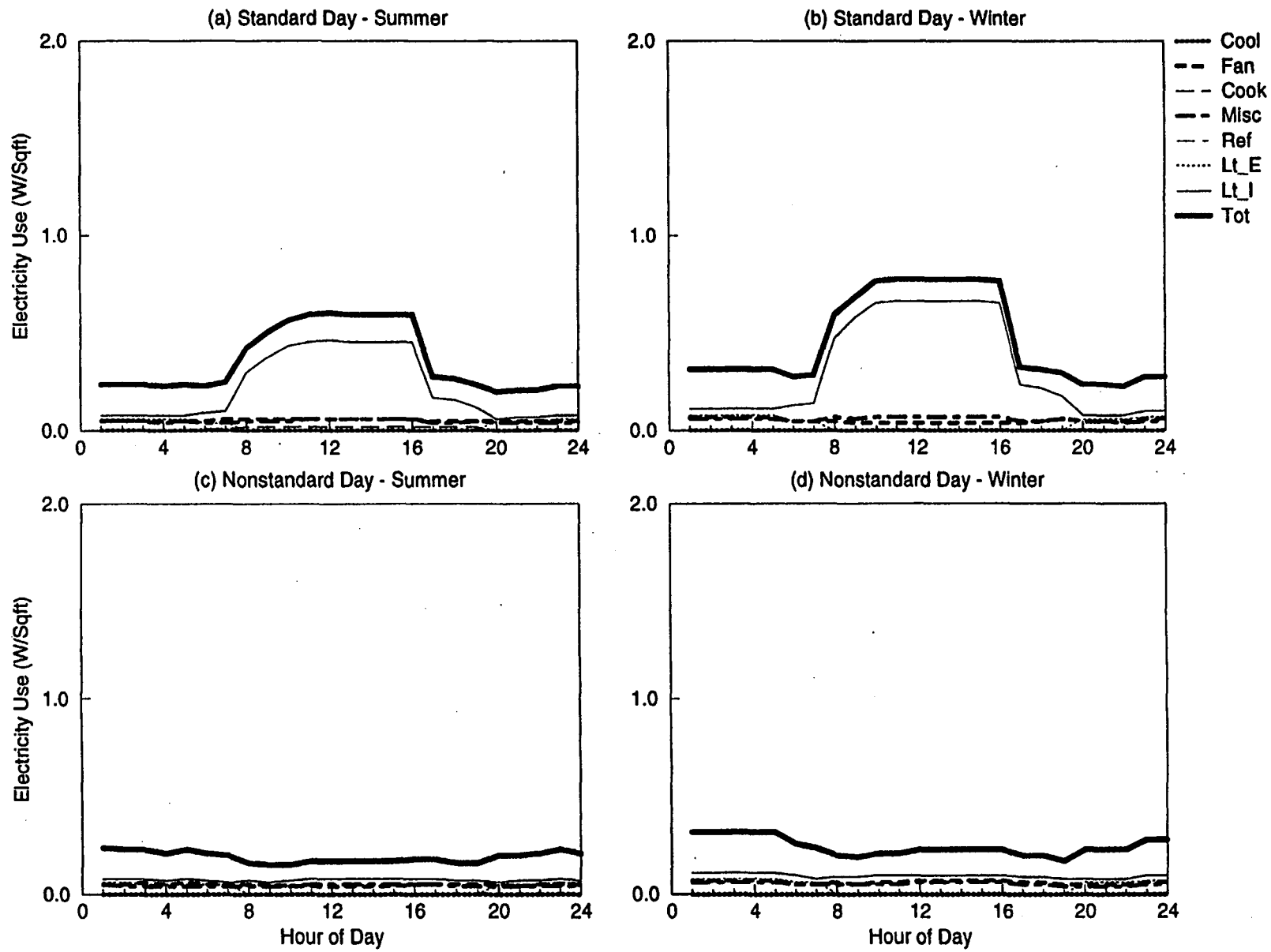
Figure C-40. EDA Reconciled End-use Load Shapes for Small Vehicle Maintenance (No AC) (Weighted 3,10)
