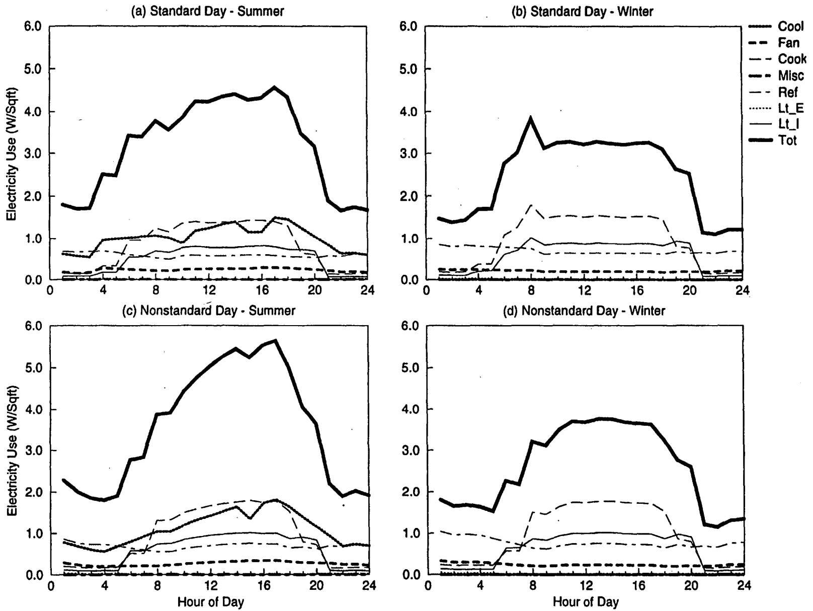
Figure C-15. EDA Reconciled End-use Load Shapes for Dining Hall (Feeder 5)
