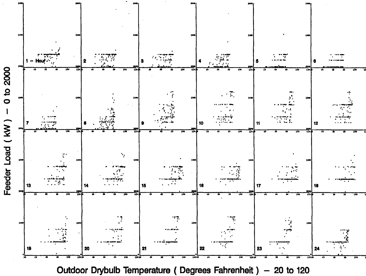
Figure A-14. Scatterplots of Feeder 4 Hourly Load vs. Drybulb Temperature for Standard Summer Days
