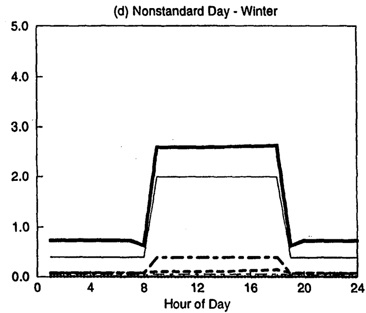
Figure B-29. DOE-2 Simulated End-use Load Shapes for Small Retail
