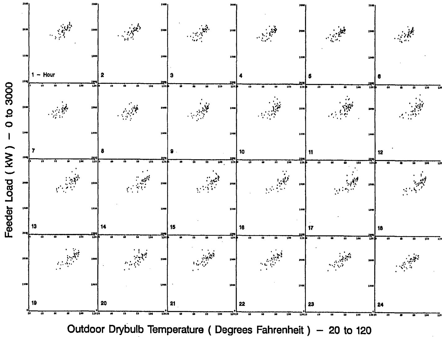
Figure A-5. Scatterplots of Feeder 2 Hourly Load vs. Drybulb Temperature for non-Standard Summer Days
