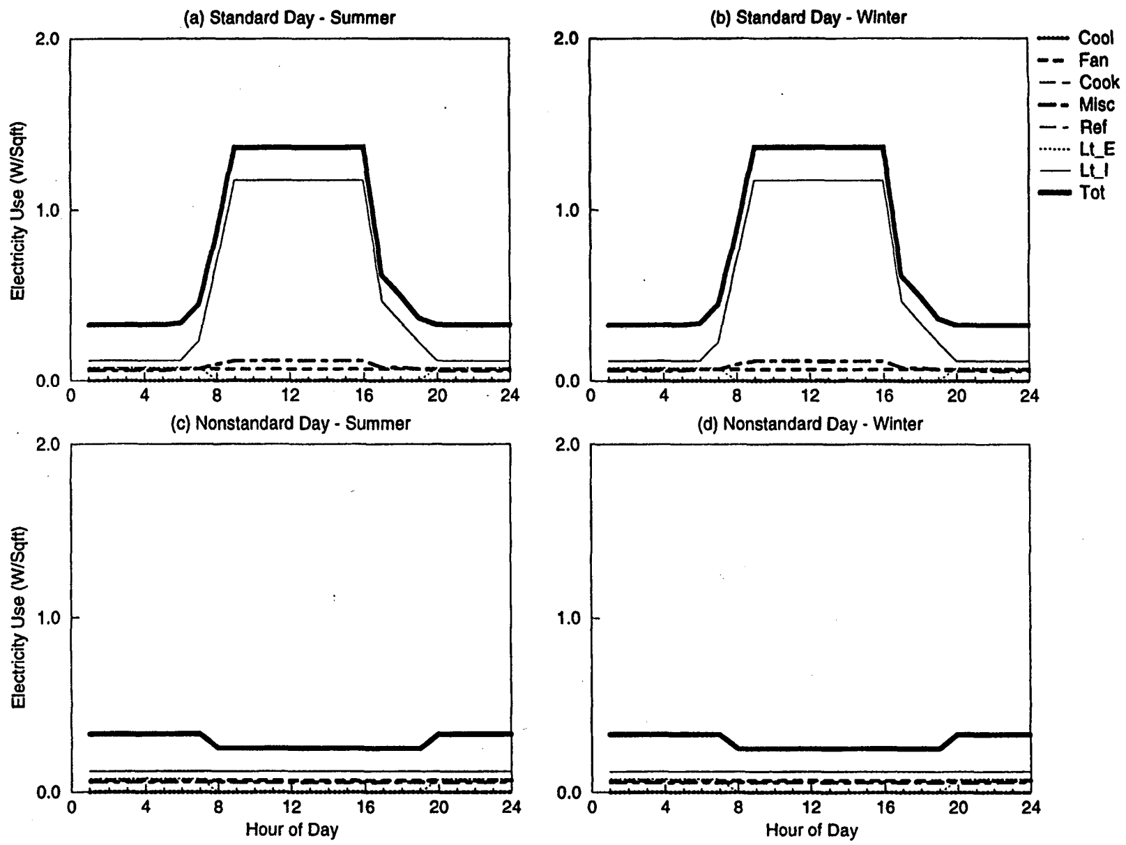
Figure B-12. DOE-2 Simulated End-use Load Shapes for Small Vehicle Maintenance (No AC)
