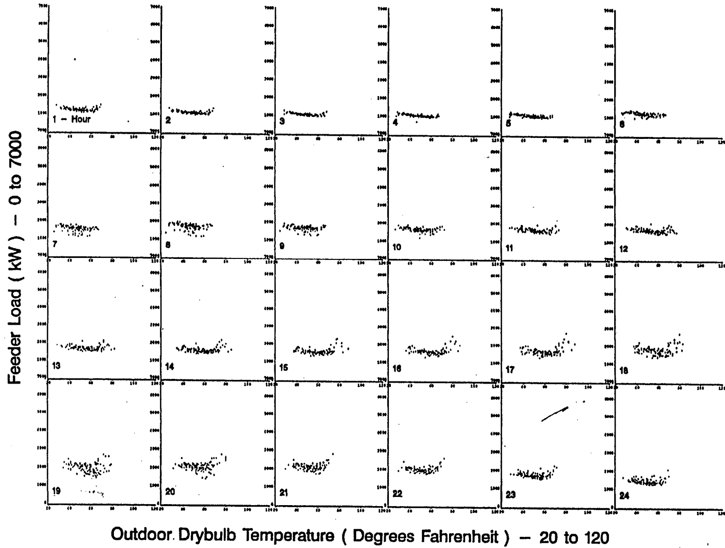
Figure A-42. Scatterplots of Feeder W4 Hourly Load vs. Drybulb Temperature for Standard Winter Days
