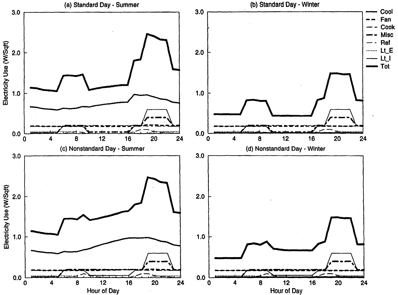
Figure B-4. DOE-2 Simulated End-use Load Shapes for Small Barrack
