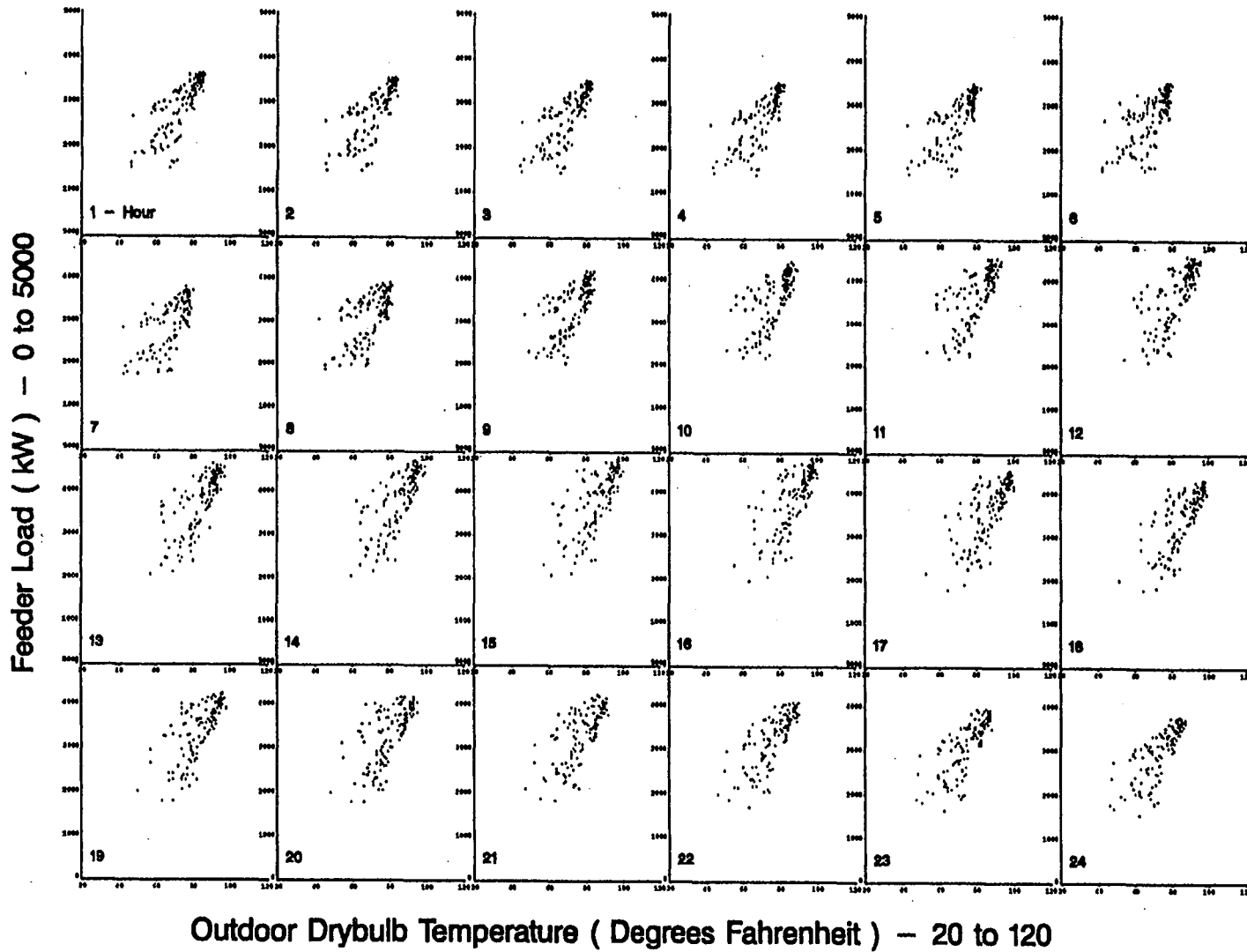
Figure A-39. Scatterplots of Feeder 15 Hourly Load vs. Drybulb Temperature for Standard Summer Days
