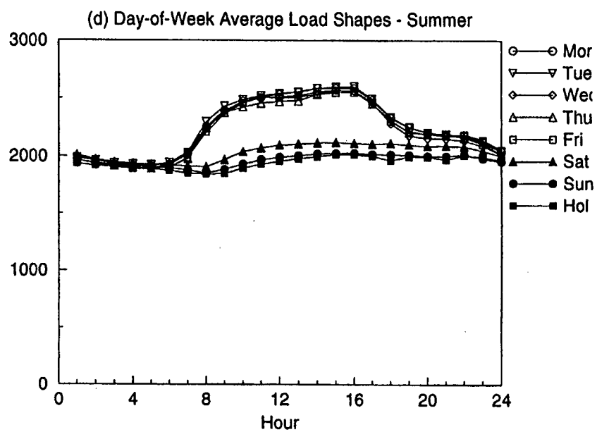
Figure 3-3. Feeder 2 Data
