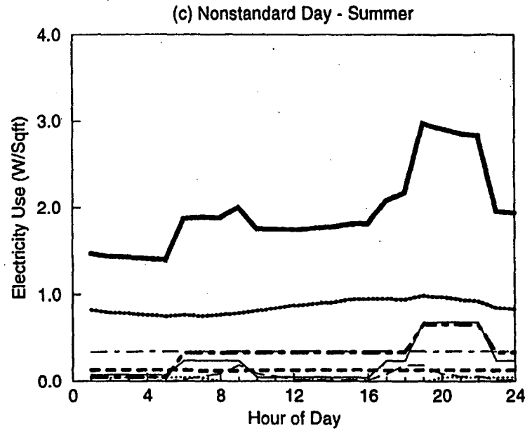
Figure B-1. DOE-2 Simulated End-use Load Shapes for Hammerhead Barrack
