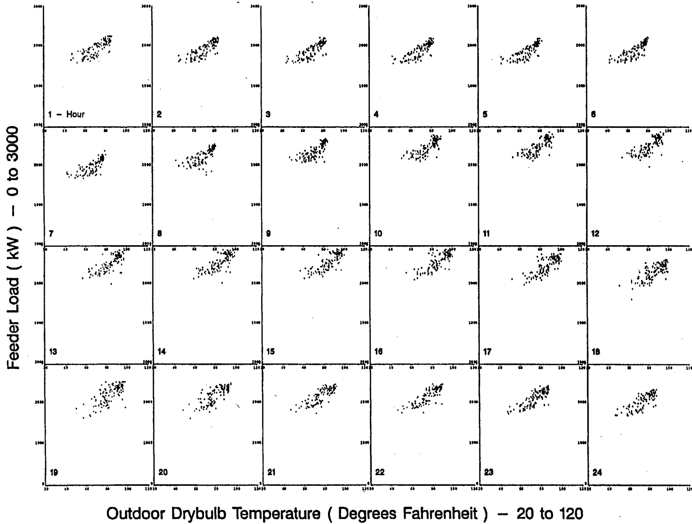
Figure A-4. Scatterplots of Feeder 2 Hourly Load vs. Drybulb Temperature for Standard Summer Days
