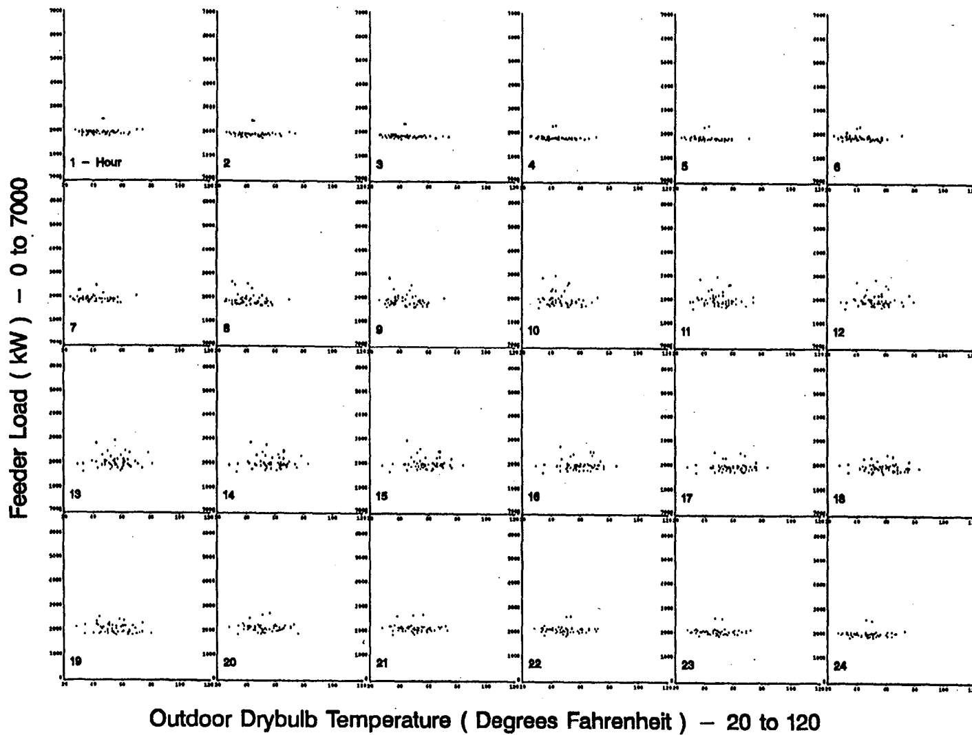
Figure A-28. Scatterplots of Feeder 10 Hourly Load vs. Drybulb Temperature for non-Standard Winter Days
