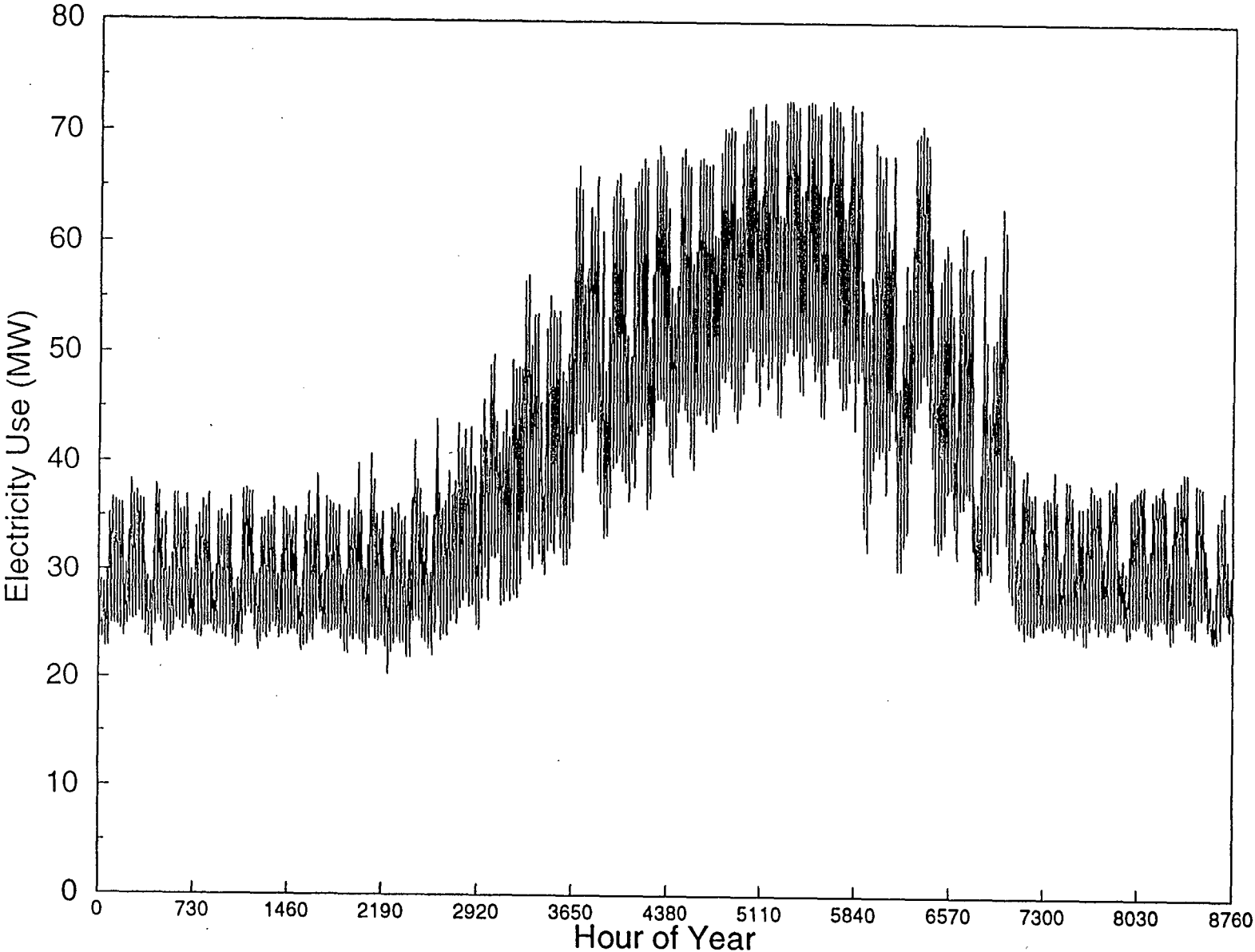
Figure 2-1. Texas Utility Annual Hourly Electricity Use
