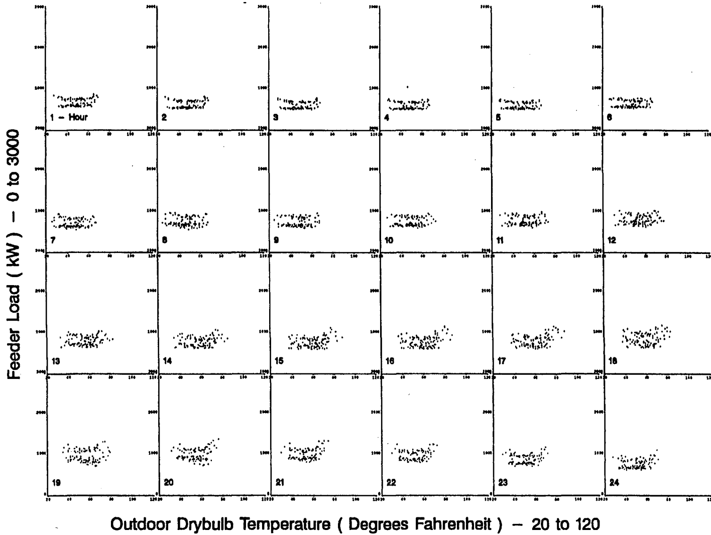
Figure A-32. Scatterplots of Feeder 12 Hourly Load vs. Drybulb Temperature for Standard Winter Days
