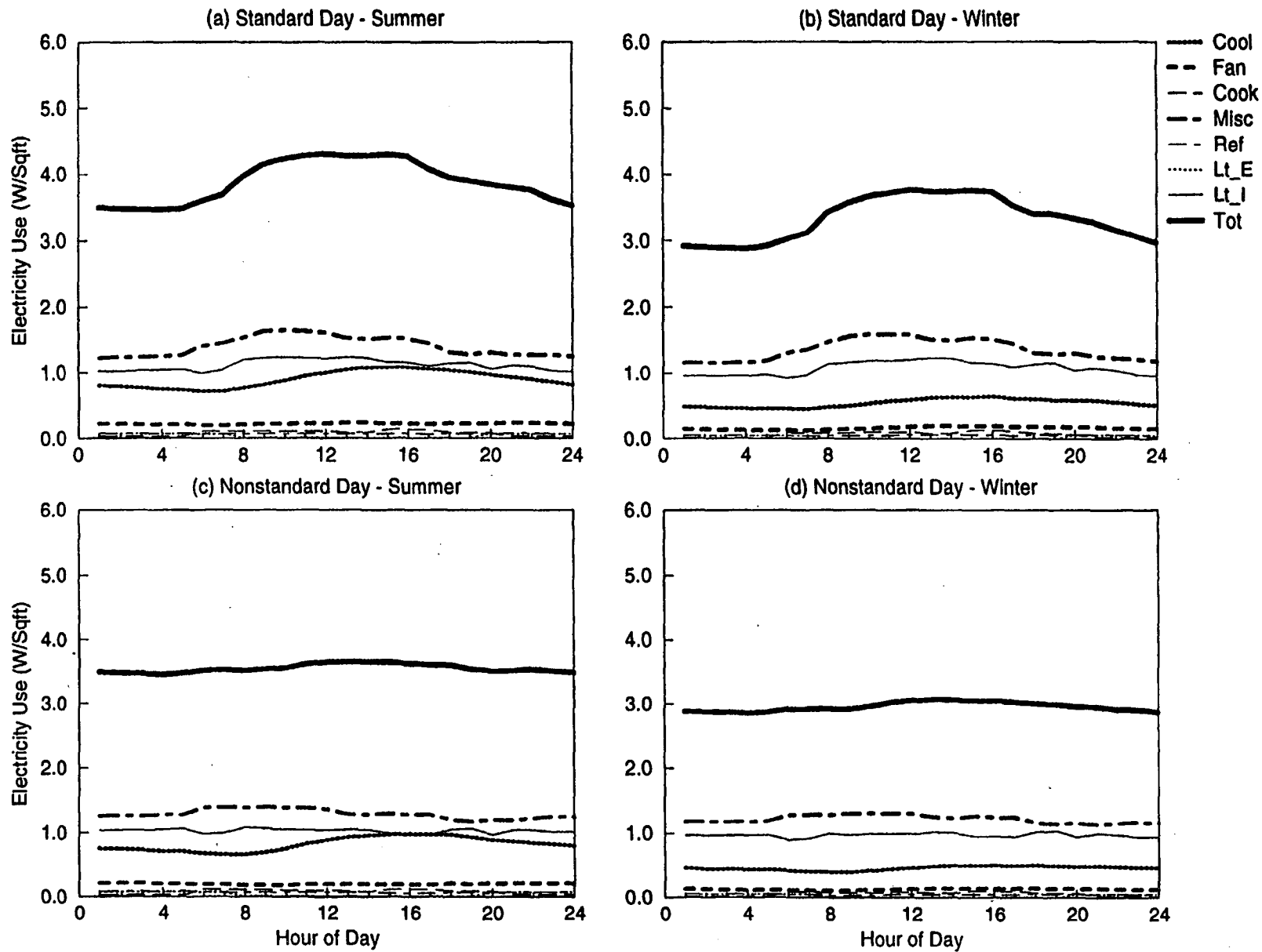
Figure C-49. EDA Reconciled End-use Load Shapes for Hospital (Feeder 9)
