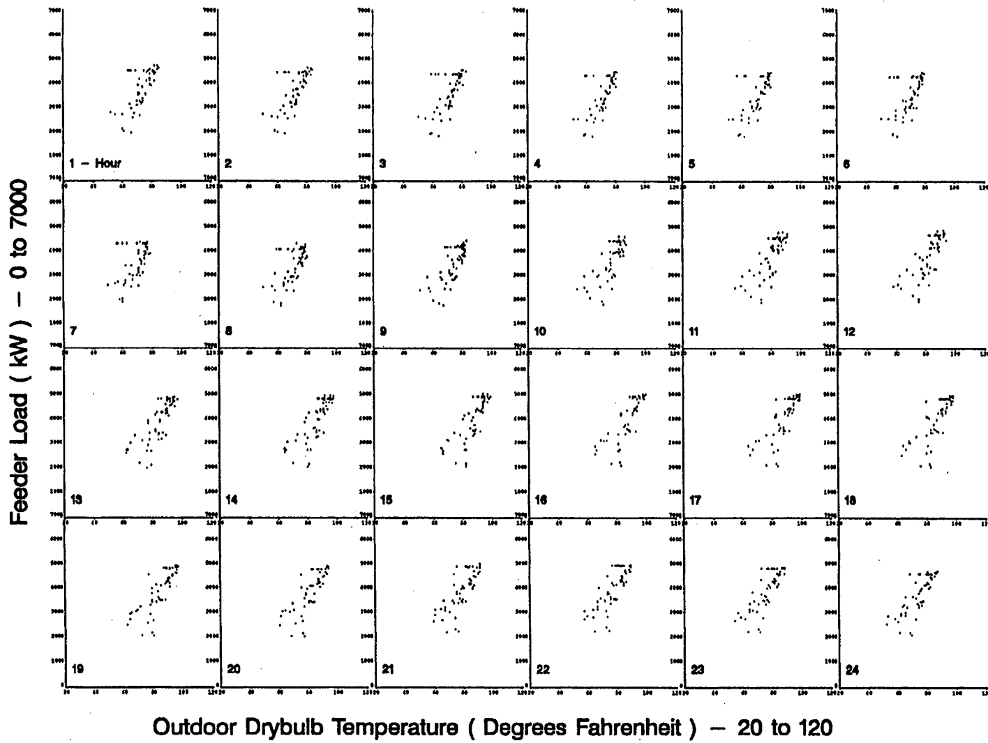
Figure A-30. Scatterplots of Feeder 10 Hourly Load vs. Drybulb Temperature for non-Standard Summer Days
