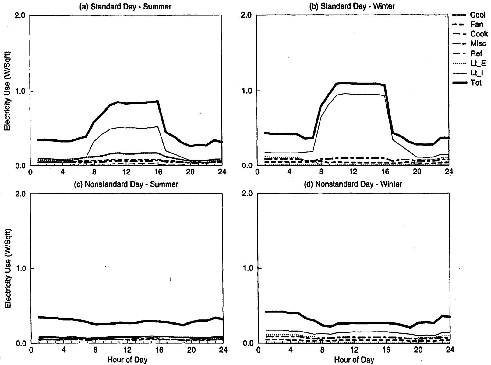
Figure C-46. EDA Reconciled End-use Load Shapes for Large Vehicle Maintenance (Chiller) (Feeder 15)
