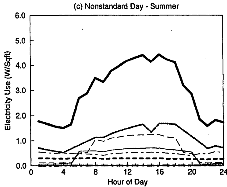
Figure C-16. EDA Reconciled End-use Load Shapes for Dining Hall (Feeder 10)
