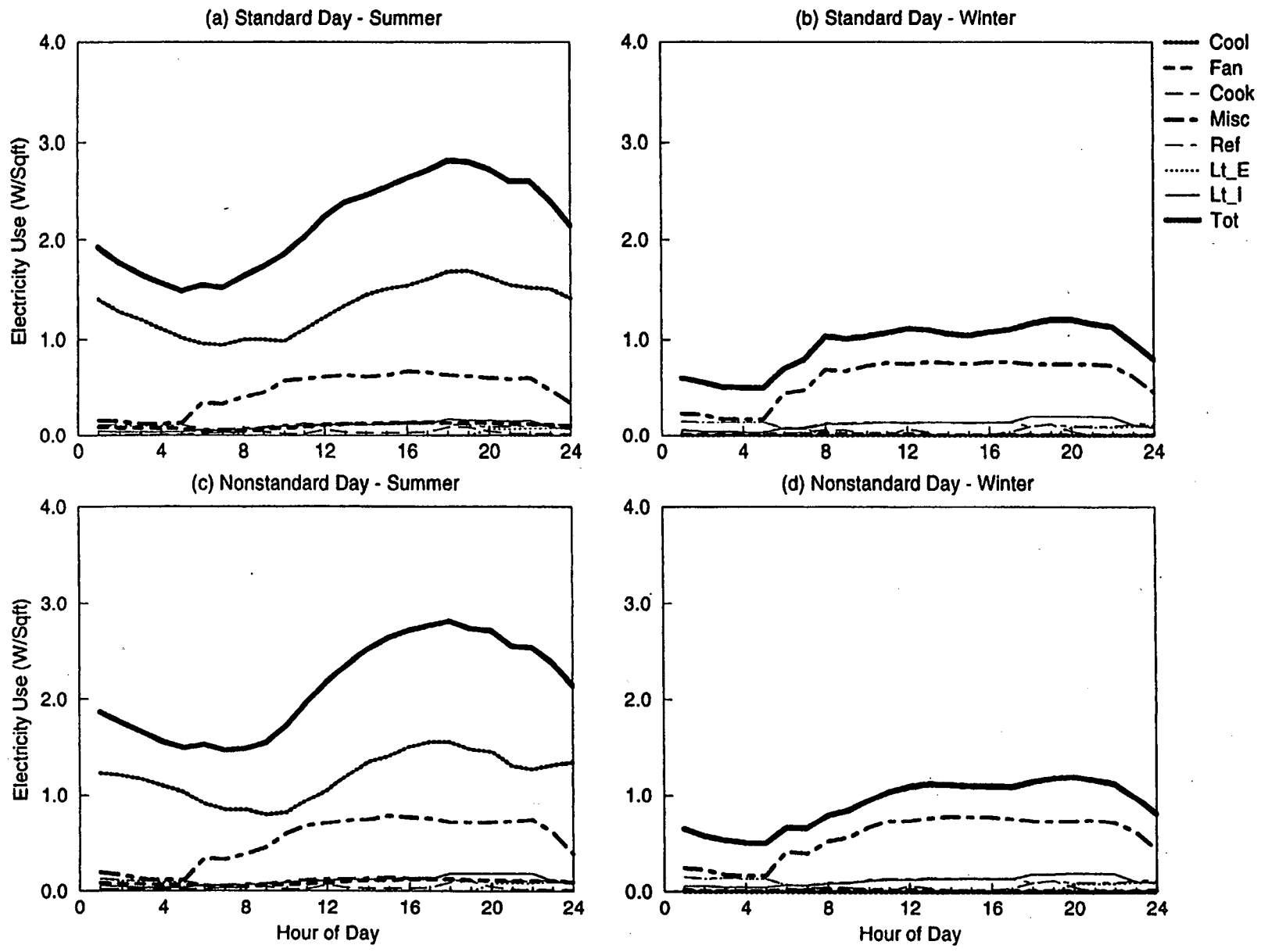
Figure C-55. EDA Reconciled End-use Load Shapes for Two-Plex Residential (Feeder 12)
