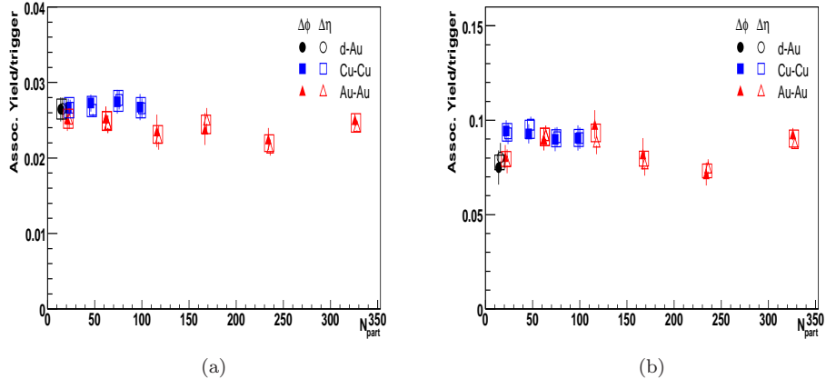
Figure 2: N_{part} dependence of the the near-side associated-particle yield for two trigger p_T ranges: (a) 4 \text{ GeV}/c < p_T^{trig} < 6 \text{ GeV}/c , (b) 6 \text{ GeV}/c < p_T^{trig} < 10 \text{ GeV}/c . For both panels 3 \text{ GeV}/c < p_T^{assoc} < p_T^{trig} . The hollow symbols are horizontally offset for clarity.
