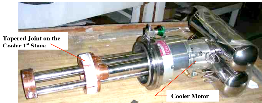
Figure 2. The Cryomech PT415 cooler (To the left is the cooler second stage with its condenser. The white part is the tapered drop-in part of the cooler first stage. To the right are the cooler rotary valve, the valve motor and the ballast tanks for the two cooler stages.)
