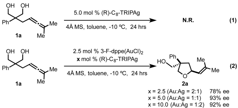
Scheme 2. Control experiments.
