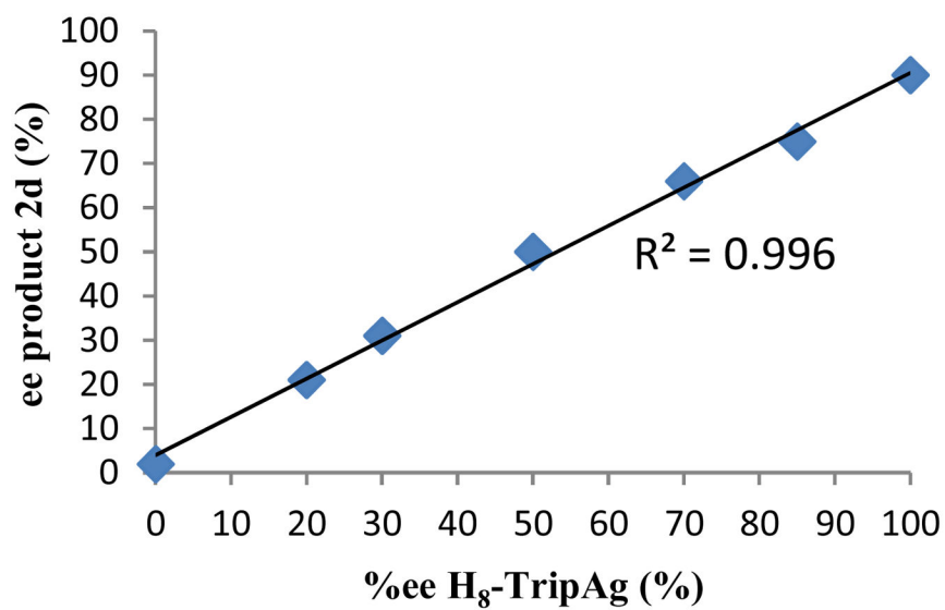
Figure 3. Relationship between the optical purity of product 2d and catalyst using 3-F-dppe(AuCl) 2 /H 8 -TripAg in toluene.
