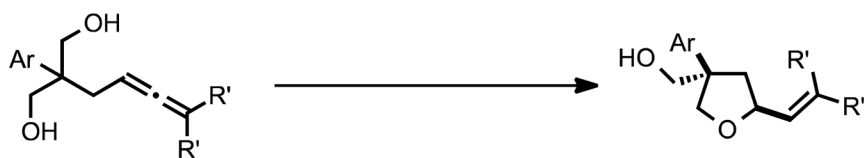
Figure 1. Strategies for enantioselective intramolecular desymmetrization of 1,3-diols
