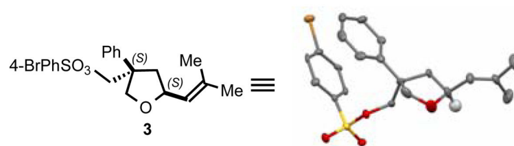
Figure 2. Absolute stereochemistry of 3 determined by X-ray crystallography.
