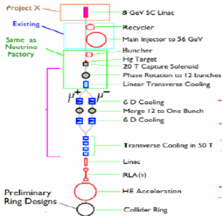
Figure 8: Muon Collider schematic. After the initial cooling section, the beam is split, cooled longitudinally, and then recombined for more transverse cooling. The final cooling stage makes use of extremely high field solenoids, up to 50 T.
