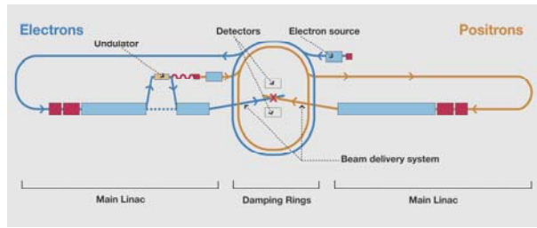
Figure 4: Layout of ILC facility. Its footprint is 31 km in length.
