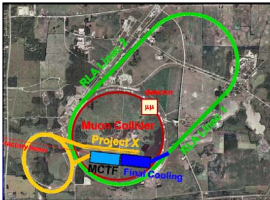
Figure 2: Schematic layout of 1.5–4 TeV Muon Collider on the Fermilab site.
