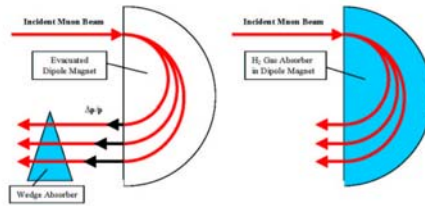
Figure 9: Schematic approaches to longitudinal cooling. On the left, a magnet creates dispersion so there is a correlation between horizontal position and momentum. The beam then passes through a wedge-shaped absorber such that low-energy particles have reduced energy loss compared with high-energy ones. On the right, the magnet is filled with a gaseous absorbing medium. Higher energy particles have a longer path length and hence experience more energy loss than do low-energy particles.
