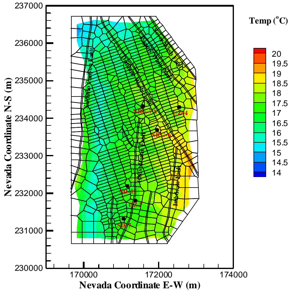
Figure 14b. Temperature distributions estimated at the Yucca Mountain surface
