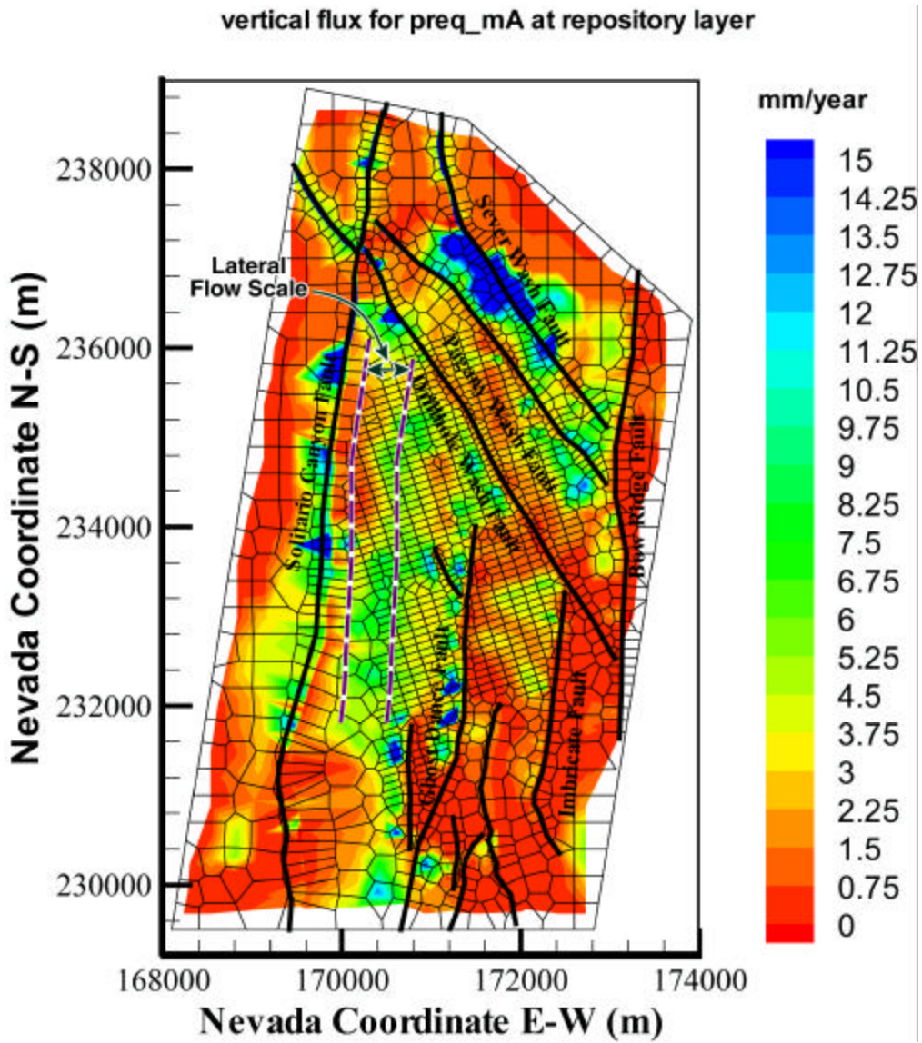
Figure 8. Simulated percolation fluxes at the repository horizon, using the present-day, mean infiltration scenario, base-case model results (preq_mA) (modified from Wu et al. , 2004)
