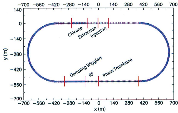
FIG. 1. Layout of DTC04 lattice.
