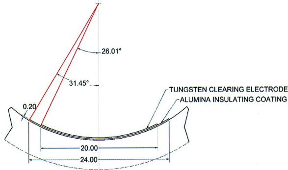
FIG. 7. Dimensions of the clearing electrode designed for cloud suppression in the wiggler magnets.
