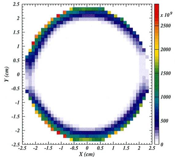
FIG. 14. Effect of a 40\text{-G} solenoidal magnetic field on the simulated EC density profile in a fieldfree region of the ring.
