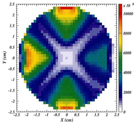
FIG. 11. Simulated EC density profile on a 41 \times 41 grid in a quadrupole magnet in an arc region of the ILC CR averaged over the 2.2 \mu\text{s} simulation time. Cloud electron escape zones are observed along the diagonal regions connecting magnet poles, as are several regions of trapped cloud.
