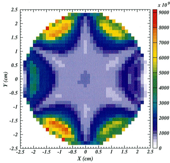
FIG. 12. Simulated EC density profile averaged over the 2.2 \mu\text{s} simulation time in an ILC DR sextupole magnet.
