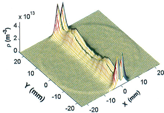
FIG. 15. Simulated EC distribution in transverse plane at the position of maximum vertical magnetic field component in the wiggler for the case of no clearing voltage.
