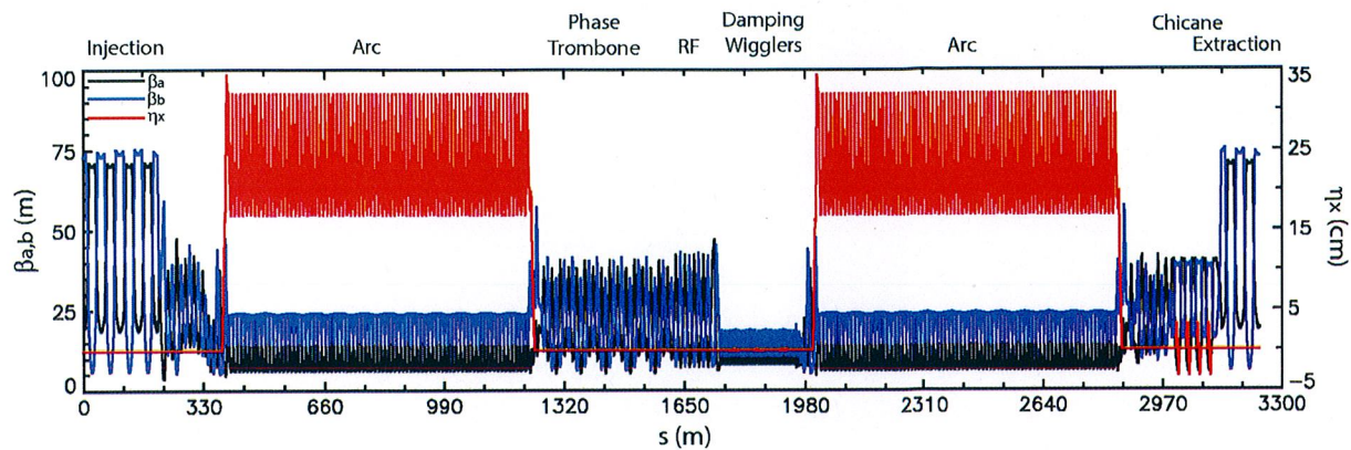
FIG. 3. Horizontal and vertical beta functions \beta_a and \beta_b , and the horizontal dispersion function \eta_x for the entire DTC04 lattice.
