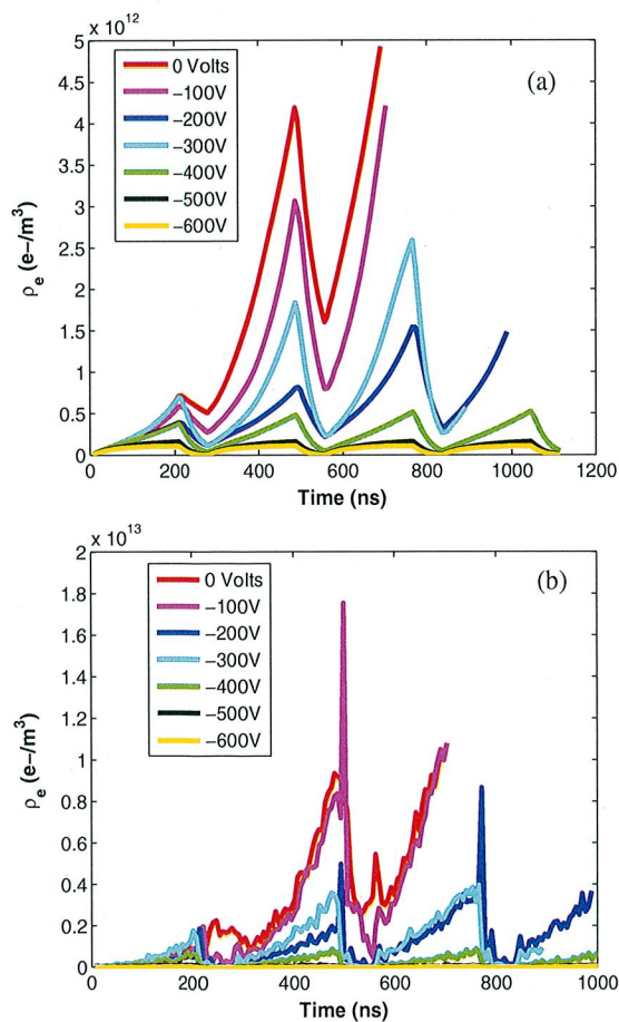
FIG. 18. Simulated buildup of the EC at the center of a wiggler pole with a negative clearing voltage applied: (a) cloud density averaged over the vacuum chamber, (b) central cloud density.
