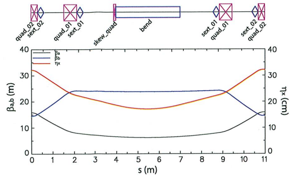
FIG. 2. Horizontal and vertical beta functions \beta_a and \beta_b , and the horizontal dispersion function \eta_x in the DTC04 arc cell.
