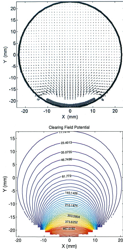
FIG. 16. The clearing electrode electric field in the simulated wiggler vacuum chamber for an electrode voltage of 500 V. The top plot shows the field vectors. The bottom plot shows equipotential lines labeled in units of volts.
