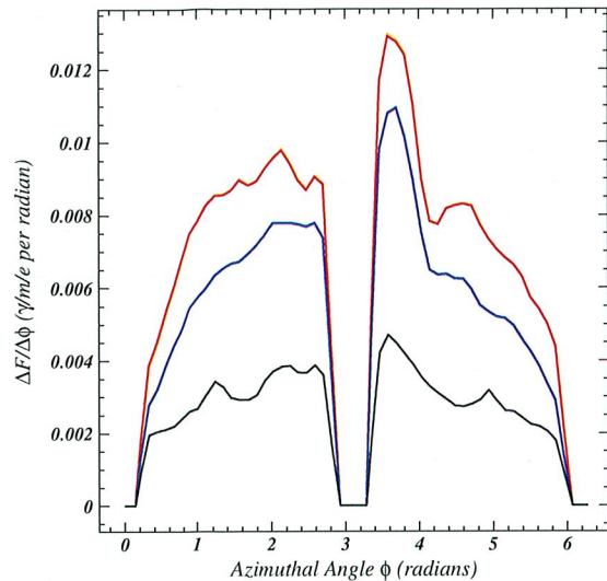
FIG. 8. Absorbed photon rate per radian \frac{\Delta F}{\Delta\phi}(\phi) versus azimuthal angle \phi in Arc 1 of the DR, averaged over the regions corresponding to three types of magnetic environment: (i) quadrupole fields (red), (ii) fieldfree regions (blue), and (iii) dipole fields (black). The azimuthal angle \phi is defined to be zero where the vacuum chamber intersects the bend plane on the outside of the ring. The angle \pi/2 corresponds to the top of the vacuum chamber. The low photon rates at zero and \pi radians are due to the absorption in the antechambers.
