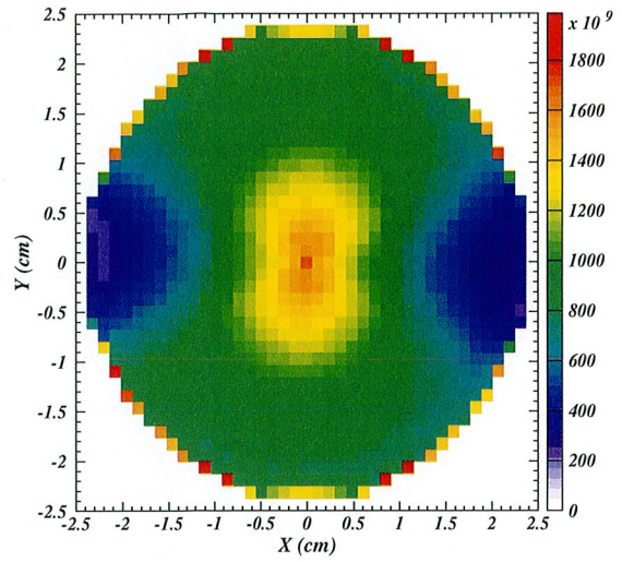
FIG. 13. Simulated EC density profile averaged over the 4.5 \mu\text{s} simulation time in a fieldfree region of arc region 1 without application of the solenoidal magnetic field mitigation technique.
