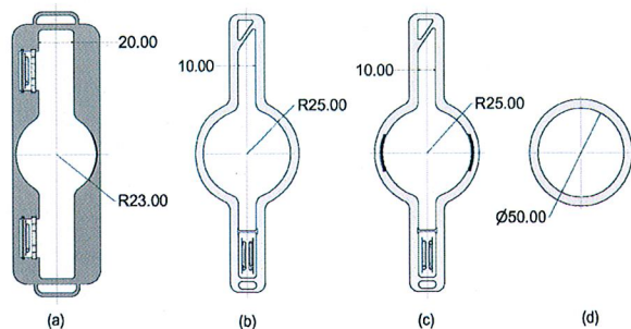
FIG. 4. Vacuum chamber profiles for the (a) wiggler magnets, (b) arc sections, (c) dipole magnets, and (d) fieldfree regions of the damping ring. Note the positions of the NEG strips, the grooves in the dipole vacuum chambers and the angled rear walls of the antechambers.
