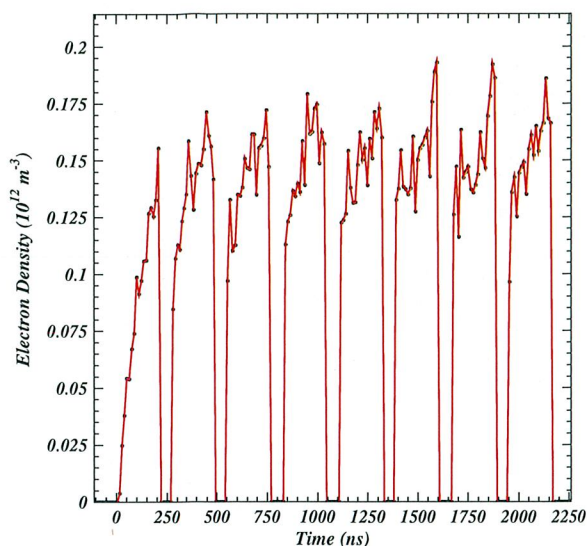
FIG. 10. 20\sigma cloud densities on a beam axis just prior to the passage of each of the 34 bunches in 8 trains in a quadrupole magnet in an arc region of the ILC DR. Cloud trapping effects build up over many train passages, but the maximum central density along a train stabilizes at a value less than 2 \times 10^{11} \text{ m}^{-3} after two trains.
