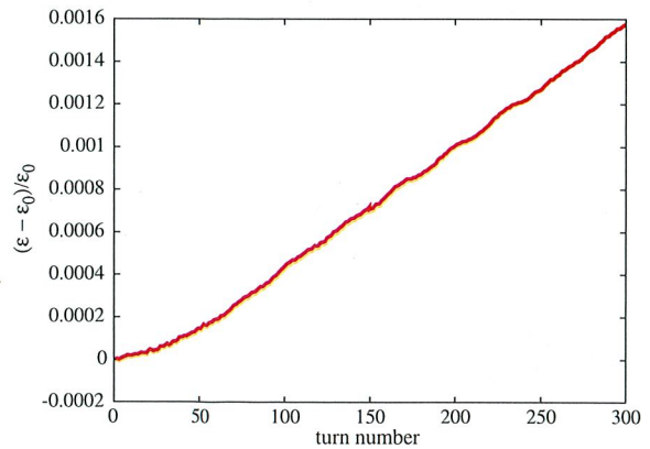
FIG. 21. Estimate of the emittance growth using the full lattice in the model with specified cloud densities in each element of the lattice.
