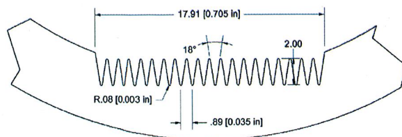
FIG. 5. Schematic cross section of bottom wall showing the dimensions of the grooves used to suppress EC buildup in the dipole magnets.
