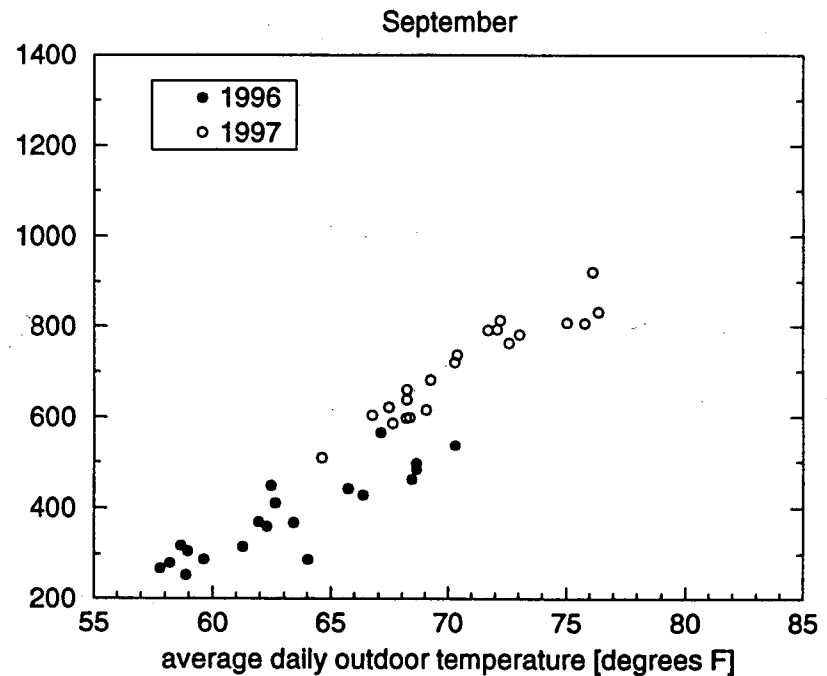
Figure 3.10b. Gilroy monitored daily air-conditioning electricity use vs daily average outdoor air temperature for standard weekdays.
