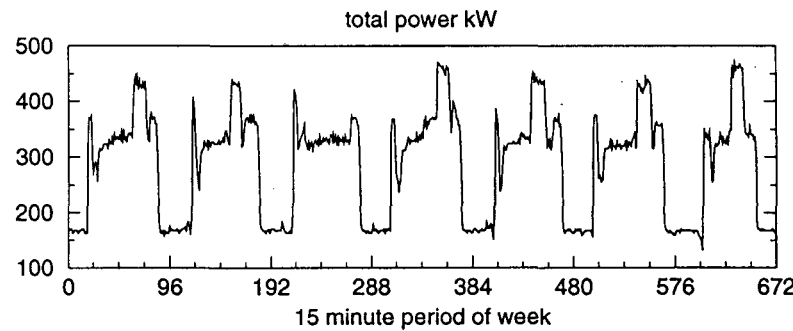
Figure 2.14. San Jose monitored 15 minute data for the week of August 18 - 24, 1997.
