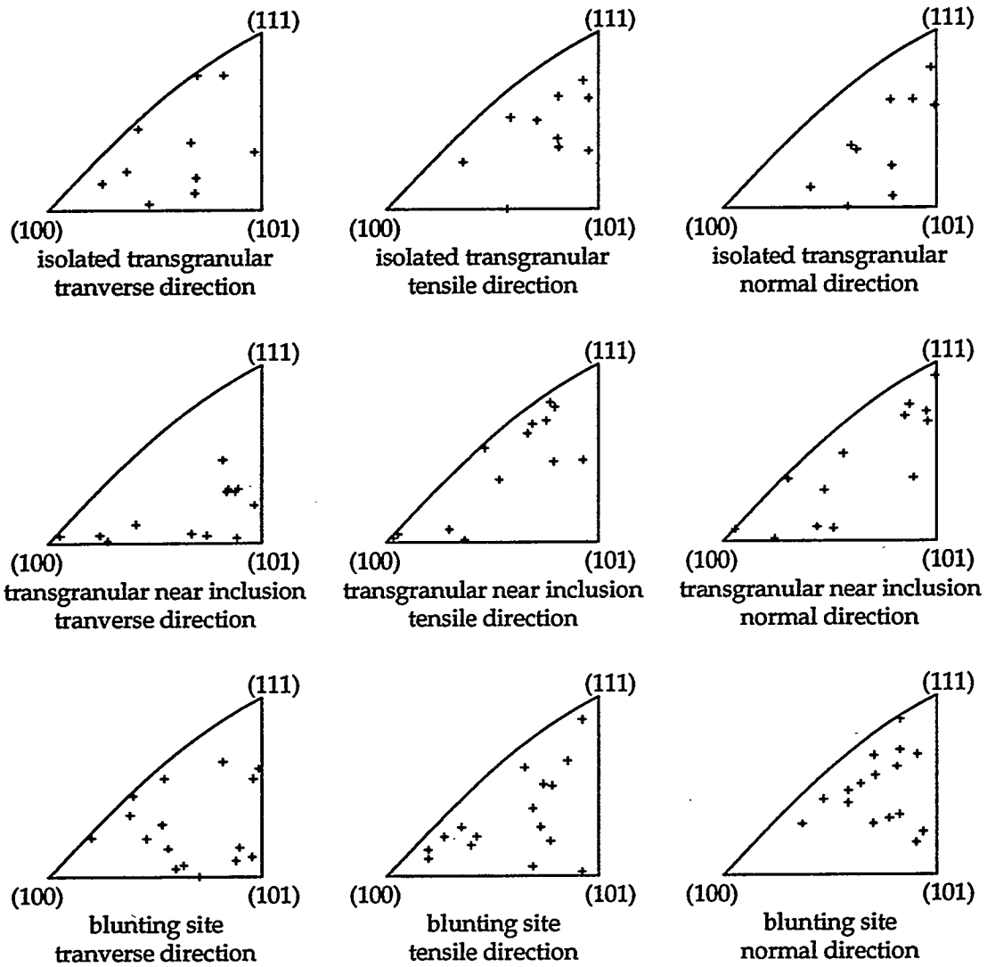
Figure 10: Inverse pole figures for initiation and blunting sites in A-286.
