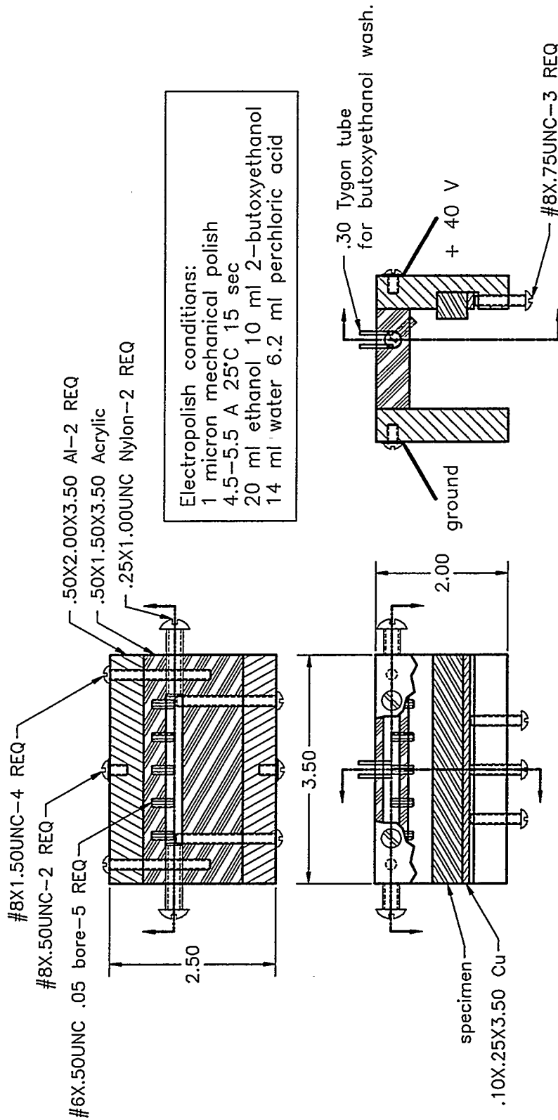
Figure 1: Design of electropolisher for large area specimens.
