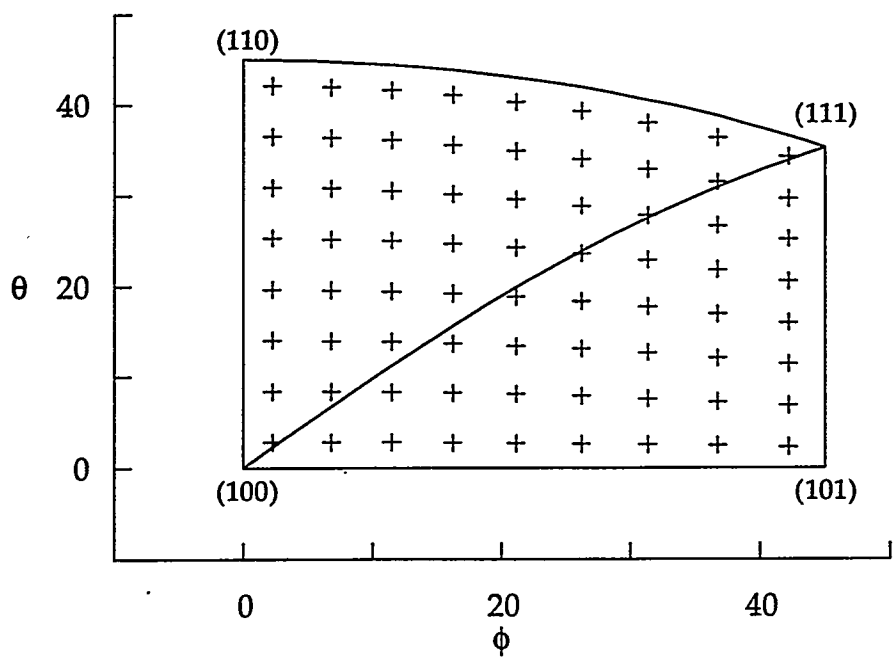
Figure 4: Plot of orientations of "random" grains within two unit crystallographic triangles.
