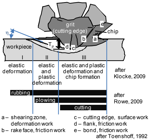
Figure 4. The three phases of ductile chip formation [1] including the different contact types rubbing, plowing, and cutting (after [28]) and the sources of heat generation (after [31]).
