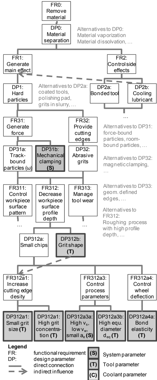
Figure 3. Tree for the functional requirement of decreasing workpiece surface profile depth.
