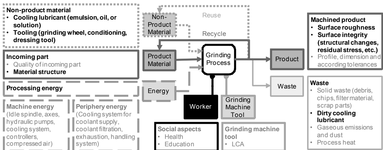
Figure 1. Scope of the grinding process inventory analysis after [18]; This paper focuses on those items in bold black.
