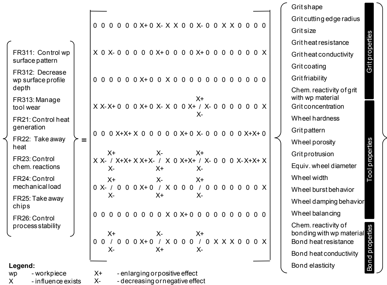
Figure 5. Matrix for grinding tool properties.
