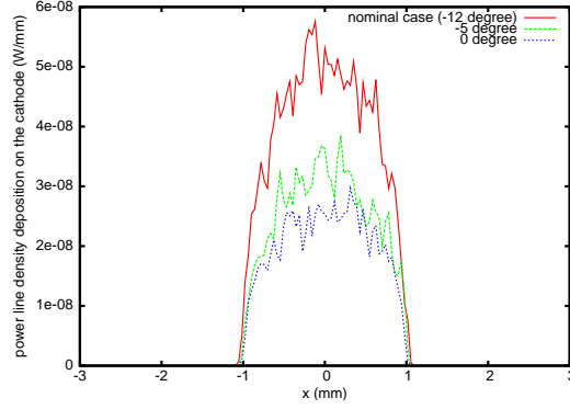
FIG. 9: Pulse averaged H_2^+ ion power line density distribution on the photocathode with 0 degree (blue), -5 degree (green), and -12 degree (red) initial RF phases.
