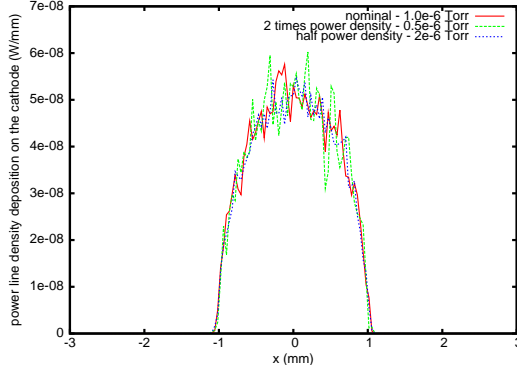
FIG. 3: Pulse averaged H_2^+ power line density distribution on the photocathode with nominal pressure, half of the nominal pressure, and twice of the nominal pressure.
