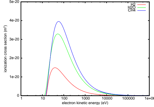
FIG. 1: Electron impact ionization cross section of H_2 (red), H_2O (green), and CH_4 (blue) as a function electron kinetic energy.
