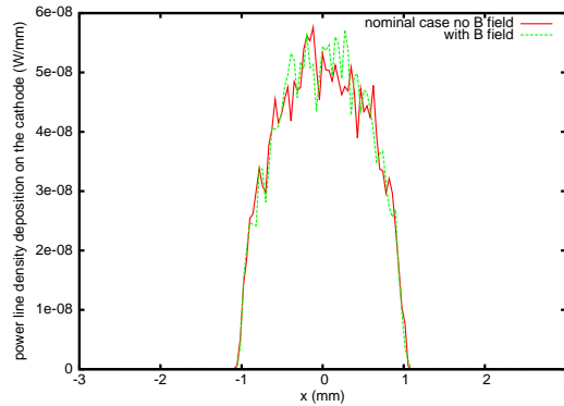
FIG. 16: Pulse averaged H_2^+ ion power line density distribution on the photocathode without external magnetic field (red) and with magnetic field (green).
