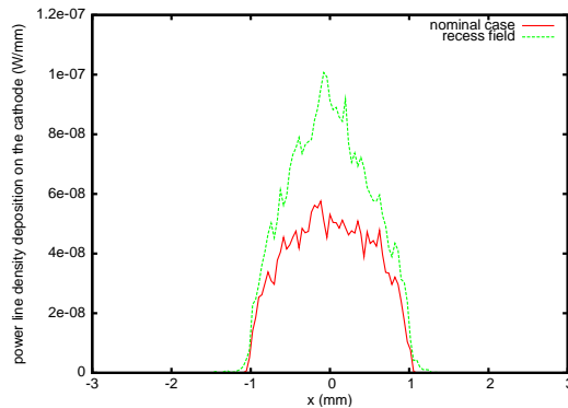
FIG. 12: Pulse averaged H_2^+ ion power line density distribution on the photocathode with peak electric field on the cathode (red) and recessed electric field on the cathode (green).
