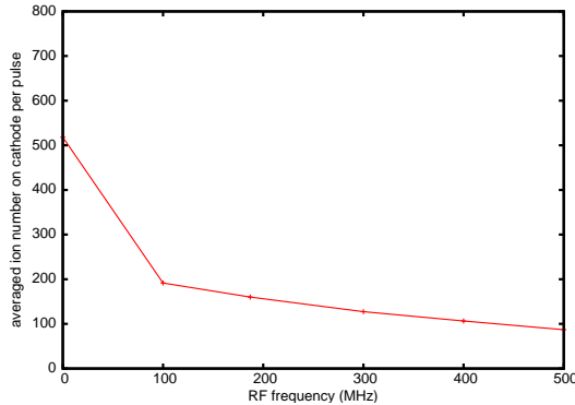
FIG. 4: The pulse averaged total H_2^+ ion particle number on the cathode as a function of RF frequency.
