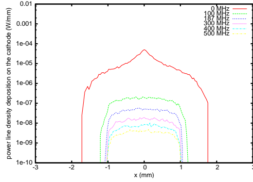
FIG. 7: Pulse averaged H_2^+ ion power line density distribution on the photocathode with 0 (red), 100 MHz (green), 187 MHz (blue), 300 MHz (pink), 400 MHz (light blue), and 500 MHz (yellow) RF frequencies inside the gun.
