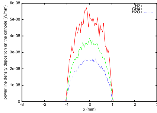
FIG. 18: Pulse averaged H_2^+ ion power line density distribution on the photocathode for H_2^+ (red), CH_4^+ (green) and H_2O^+ (blue) ions.
