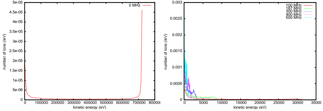
FIG. 6: Pulse averaged H_2^+ kinetic energy distribution on the photocathode with 0 frequency (top), and with 100 MHz (red), 187 MHz (green), 300 MHz (blue), 400 MHz (pink), and 500 MHz (light blue) RF frequencies inside the gun.
