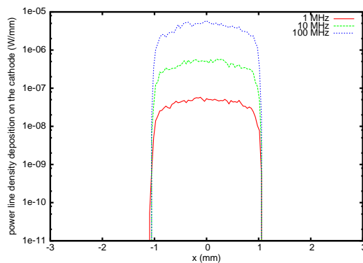
FIG. 14: Pulse averaged H_2^+ ion power line density distribution on the photocathode with 1 MHz (red), 10 MHz, and 100 MHz repetition rate.
