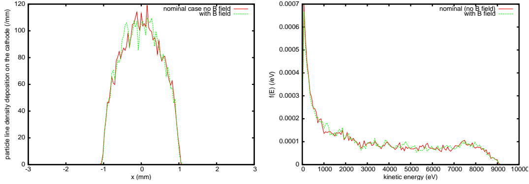
FIG. 15: Pulse averaged H_2^+ ion particle line density distribution (top) and the kinetic energy distribution (bottom) on the photocathode without external magnetic field (red) and with magnetic field (green).
