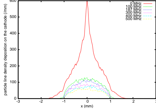
FIG. 5: Pulse averaged H_2^+ ion particle line density distribution on the photocathode with 0 (red), 100 MHz (green), 187 MHz (blue), 300 MHz (pink), 400 MHz (light blue), and 500 MHz (yellow) RF frequencies inside the gun.
