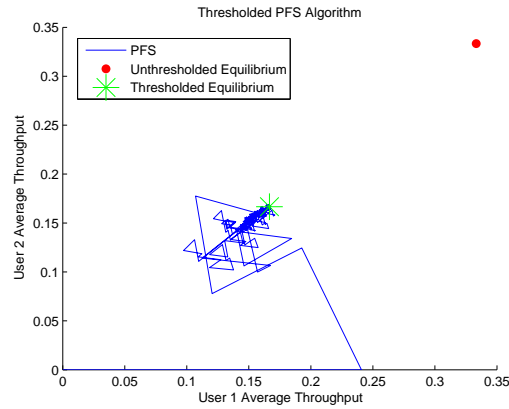
Figure 4.5: Threshold for N = 2 , R_{loss} = \frac{1}{3}
