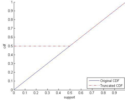
Figure 3.2: Uniform Distribution Truncated at x_{threshold} = 0.5
