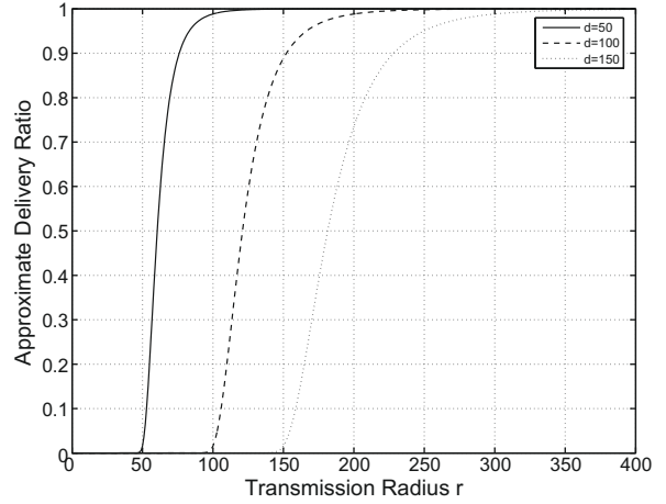
Fig. 9. A sample of approximate delivery ratio.
