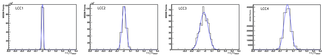
Figure 3: Probability distribution of predictions for the neutralino relic density \Omega_\chi h^2 based on expected measurements at the LHC and at the ILC, in the four supersymmetry models presented in Table I.
