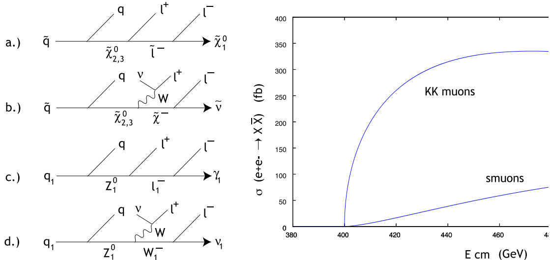
Figure 2: Left: Four possible physics models for missing-energy events at the LHC; Right, discrimination of the models (a) and (c) by a total cross section measurement at the ILC.
