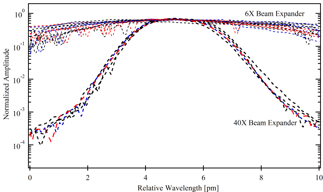
Figure 3.6: Spectral distribution for 5 narrowband (40X) and 15 broadband (6X) laser pulses relative to the peak amplitude of a pulse. Individual pulses are very similar in shape, but the 10 pm window limit of the wavemeter makes it difficult to analyze the shape of the wings of the broad bandwidth laser pulses. All pulses were measured by the WS-7 in fine mode.
