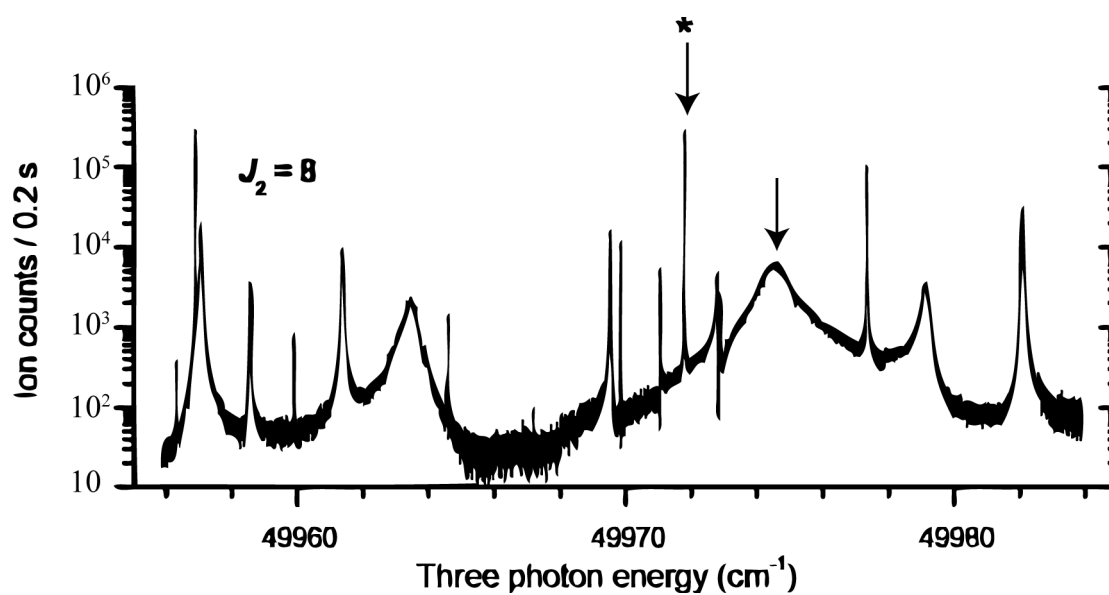
Figure 2.7: Ionization rate of ^{238}\text{U} as a function of wave number just above the ionization limit for excitation from a highly excited bound state with angular momentum J_2 = 8 . Note the presence of very strong, narrow resonances and compare their peak amplitudes to the region near 49,966\text{ cm}^{-1} . The arrows indicate the autoionizing states explored in the present work. The narrow resonance marked with an asterisk is described in the text. (Reproduced from Schumann, et al. [51])
