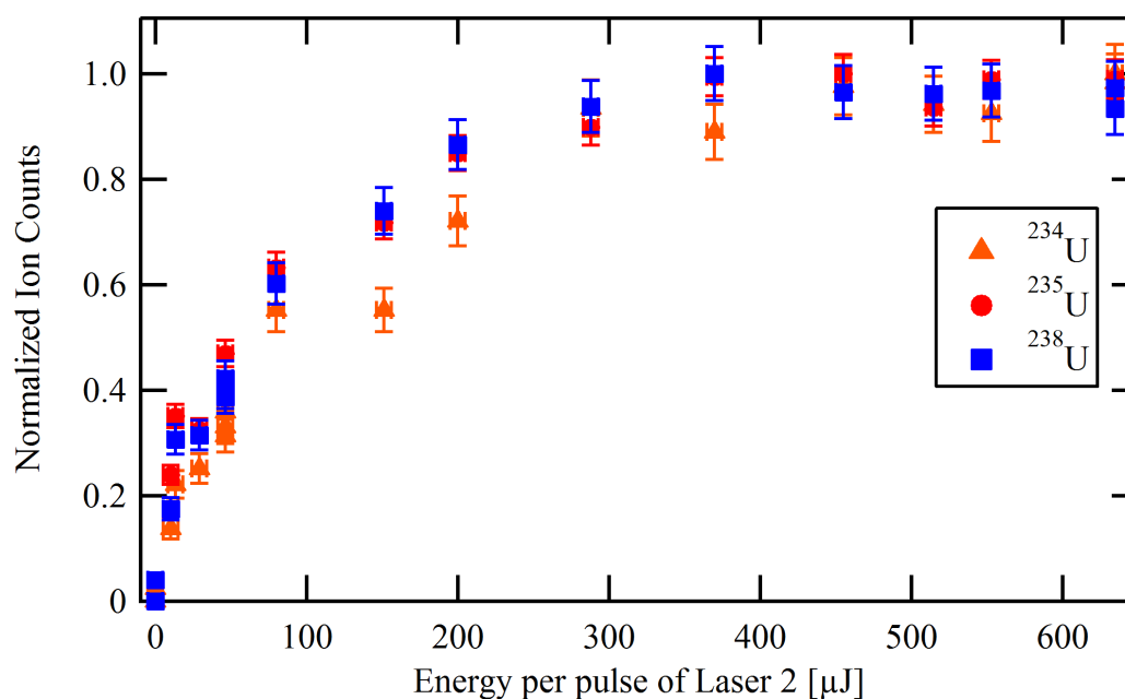
Figure 4.26: The normalized ion signal as a function of energy per pulse of the second resonance laser beam with the bandwidth of the first and second laser cavities broadened to \sim 5 pm and \sim 6 pm, respectively. The total counts are normalized so that the ^{234}\text{U} can be compared with the major isotopes. The transition of all three isotopes appear to be saturated above energies of 400 \mu\text{J}/\text{pulse} in the second laser beam. Uncertainty estimates include changes in sputter yield. Measurement performed on CRM U500.
