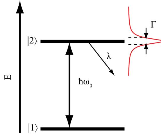
Figure 2.1: Two-state atomic model.
