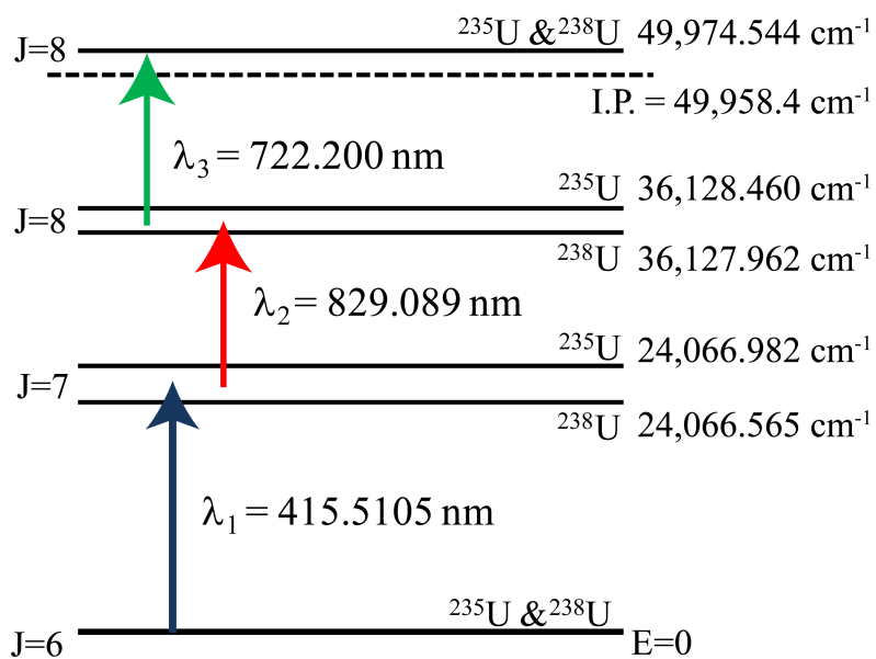
Figure 3.22: A 3-color, 3-photon U ionization scheme. This partial energy diagram shows the isotope shift between the levels of ^{235}\text{U} and ^{238}\text{U} used in this scheme and the wavelengths of the lasers used to excited these transitions between the levels. On the left are the total electron angular momenta of the levels.
