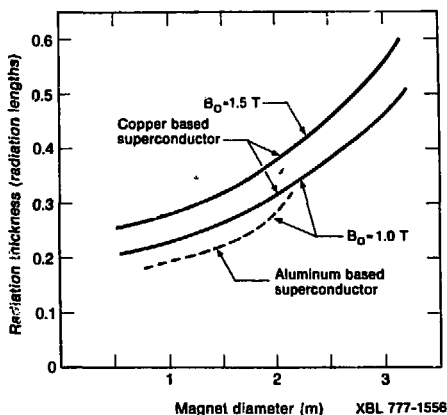
Figure 15. The projected radiation thickness of thin solenoids using the LBL technique as a function of magnet diameter, superconductor type and central induction B_0 .
