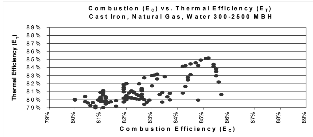
Figure 2: Example of a scatter plot E_C vs. E_T (HI 1999)
