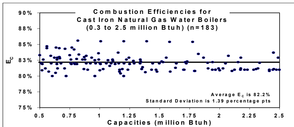
Figure 3: Standard Deviation for Cast Iron, Natural Gas Boilers (HI 1999)
