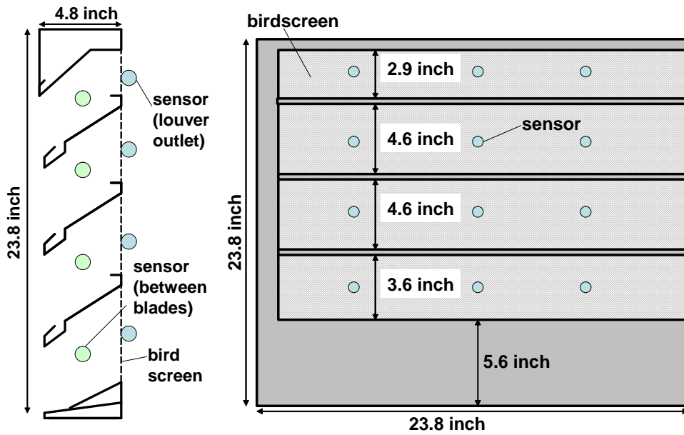
Figure 2. Side view cross section and outlet view of Arrow EA 64 louver with sensor locations.
