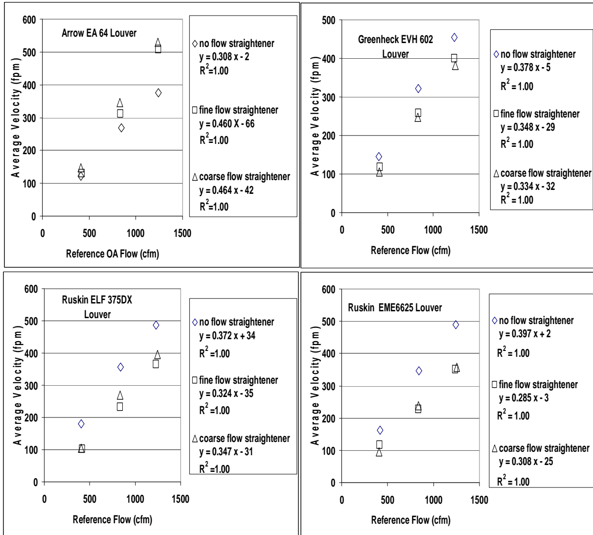
Figure 11. Average air velocity, using data from nine velocity sensors, versus reference flow from tests with airflow straighteners.
