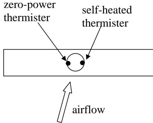
Figure 6. Schematic illustration of a velocity probe containing one velocity sensor.
