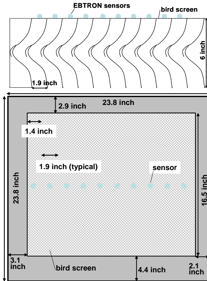
Figure 3. Top cross section and outlet view of Greenheck EVH602 louver with sensor locations.
