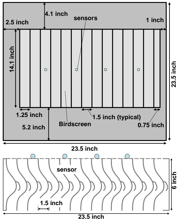
Figure 5. Outlet view and top cross section of Ruskin EME6625 louver with sensor locations.
