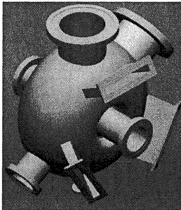
Figure 1. Low-Power test prototype of PEP-II RF cavity. The damping waveguides are attached to the three rectangular ports emerging from the cavity body. The large circular ports at the top of the cavity are the two alternative locations being considered for the main RF drive coupler.
