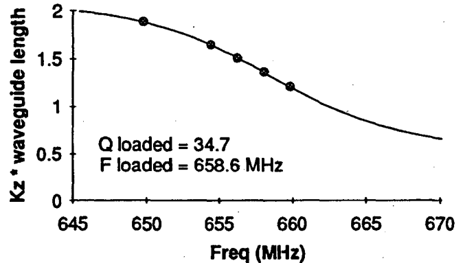
Figure 2. Phase vs Frequency plot showing theoretical curve and ARGUS data used to find loaded Q for the TE111 mode by Kroll-Yu method.
