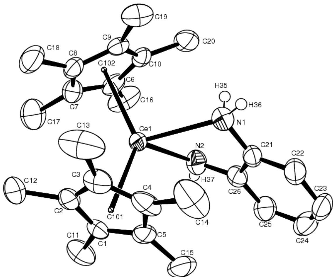
Figure 1.3.7: ORTEP diagram of \text{Cp}^*_2\text{Ce}(1\text{-amido-2-aminobenzene}) (50% probability ellipsoids). All non-hydrogen atoms are refined anisotropically. Hydrogen atoms other than the N-H hydrogens, which are found in the Fourier difference map and refined isotropically, are not shown. Selected bond distances and angles are given in Tables 1.3.5 and 1.3.6 respectively.
