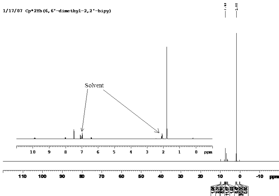
Figure 4.4.8: Room temperature ^1\text{H} NMR spectrum of \text{Cp}^*_2\text{Yb}(6,6' -dimethyl-bipy) in toluene- \text{d}_8 .
