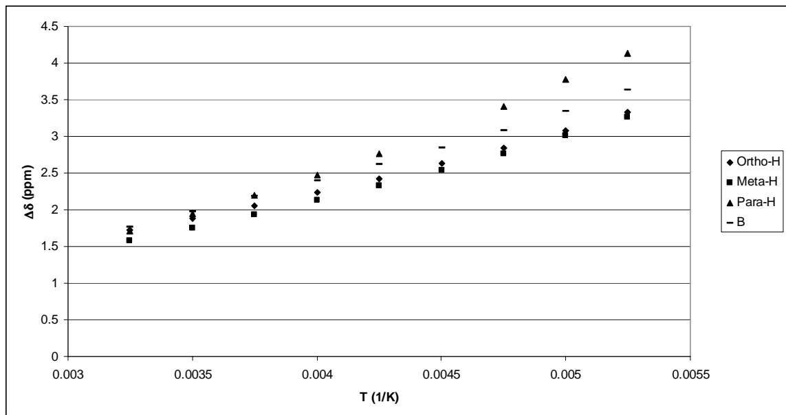
Figure 2.4.11: Variable Temperature of the isotropic values of the ^1\text{H} and ^{11}\text{B} NMR shifts represented as a \delta vs. 1/T plot of [\text{BPh}_4] in [\text{Cp}^*_2\text{Yb}(\text{N,N}'\text{-bis}(\text{p-anisyl})\text{-2,3-dimethyl-1,4-diazadienyl})][\text{BPh}_4] in \text{CD}_2\text{Cl}_2 . The isotropic shift, \Delta\delta = \delta^{\text{dia}} - \delta^{\text{para}} , where \delta^{\text{dia}} is taken from the ^1\text{H} and ^{11}\text{B} NMR spectra of [\text{Cp}^*_2\text{Lu}(\text{bipy})][\text{BPh}_4] in \text{CD}_2\text{Cl}_2 . In the ^1\text{H} NMR spectrum of [\text{Cp}^*_2\text{Lu}(\text{bipy})][\text{BPh}_4] the ortho-H is at 7.43 ppm and the meta-H is at 7.05 ppm, and they are easily distinguishable by their coupling pattern. In [\text{Cp}^*_2\text{Yb}(\text{p-tolyl-dad})][\text{BPh}_4] there is no coupling on the [\text{BPh}_4] resonances, and therefore it is difficult to assign which peak is which. We assume that the peak that is further downfield is the ortho-H just as in the case of [\text{Cp}^*_2\text{Lu}(\text{bipy})][\text{BPh}_4] . The para-H is easily identified by its relative integral.
