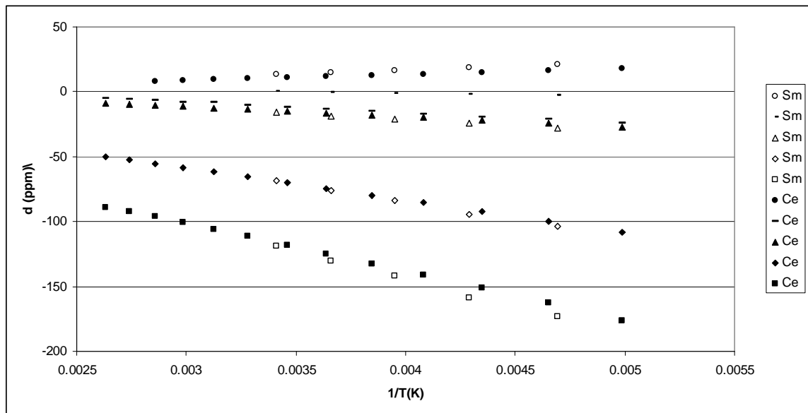
Figure 3.4.13: Variable Temperature ^1\text{H} NMR spectra represented as a \delta vs. 1/T plot of \text{Cp}^*_2\text{Sm}(2,2',6',2'') -terpyridine) and the corresponding peaks in \text{Cp}^*_2\text{Ce}(2,2',6',2'') -terpyridine) in toluene- d_8 . The peak between -200 and -500 ppm is shown in the next figure. The \text{Cp}^* peaks have been omitted for clarity; they do not overlap.
