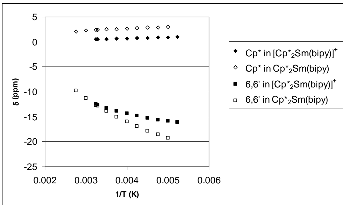
Figure 3.4.8: Comparison of the Cp* and the 6 position in the bipy in the variable temperature ^1\text{H} NMR spectrum of \text{Cp}^*_2\text{Sm}(\text{bipy}) (in toluene- d_8 ) and [\text{Cp}^*_2\text{Sm}(\text{bipy})][\text{BPh}_4] (in \text{CD}_2\text{Cl}_2 )
