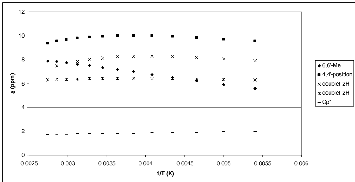
Figure 4.4.9: Variable Temperature ^1\text{H} NMR spectra represented as a \delta vs. 1/T plot of \text{Cp}^*_2\text{Yb}(6,6'\text{-dmb}) in toluene- d_8 .
