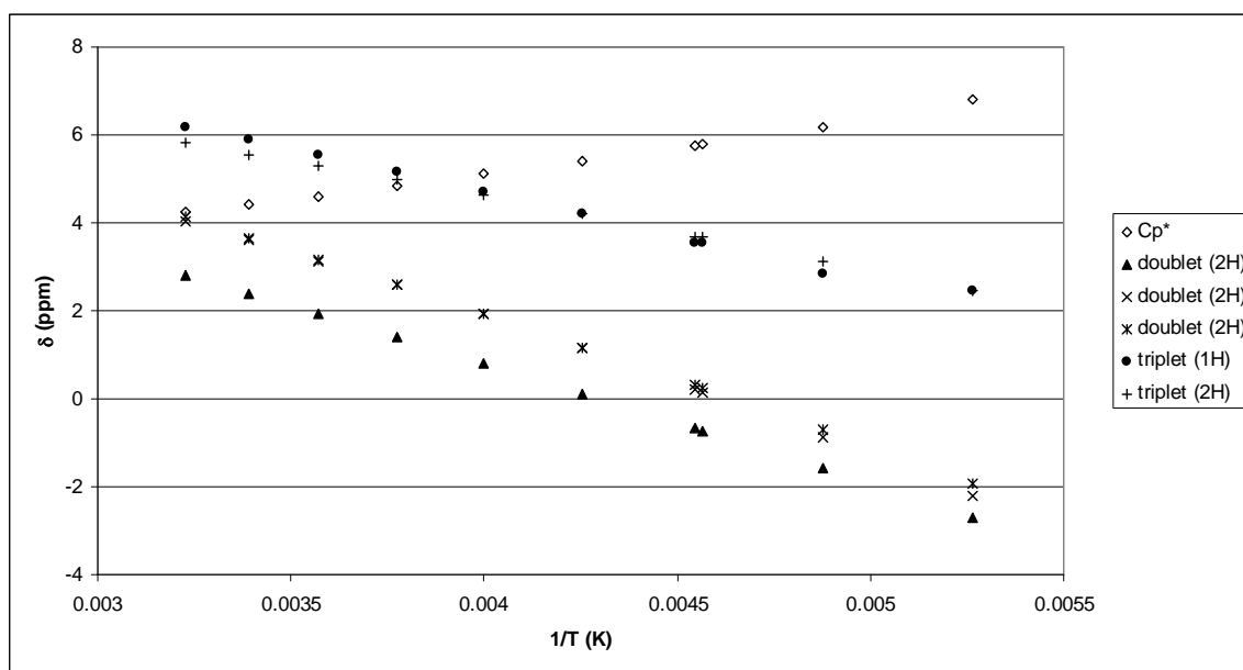
Figure 2.3.1: Variable temperature ^1\text{H} NMR spectra, represented as a \delta vs. 1/T plot, of [\text{Cp}^*_2\text{Ce}(\text{terpy})][\text{OTf}] in \text{CD}_2\text{Cl}_2 . For clarity's sake the area 2 singlet, which goes from -42.51 ppm at 190K to -16.02 ppm at 310K is not shown; it also obeys Curie law.
