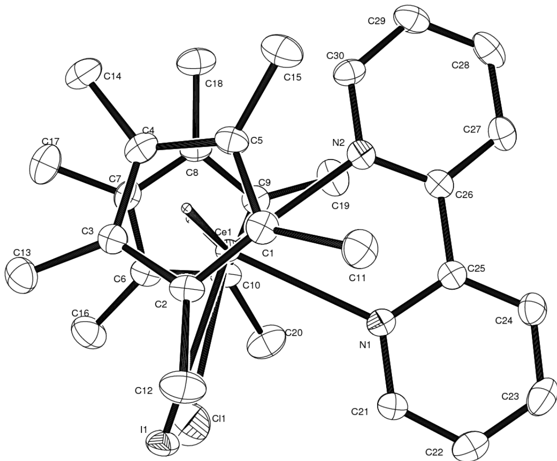
Figure 2.2.13: ORTEP diagram of \text{Cp}^*_2\text{Ce}(\text{bipy})(\text{X}) (where X is partially occupied by I/Cl where the site is modeled with a 93% occupancy of I and 7% occupancy of Cl (50% probability ellipsoids). All non-hydrogen atoms except for Cl are refined anisotropically; Cl is refined isotropically. Hydrogen atoms are placed and not refined and are not shown. Selected Bond Distances and Angles are given in Tables 2.2.5 and 2.2.6, respectively. The \text{N1-C25-C26-N2} torsion angle is 13.8(5)^\circ . I1 is 0.52 \text{ \AA} out of the least-squares plane defined by the atoms in the bipyridine ring. 7
