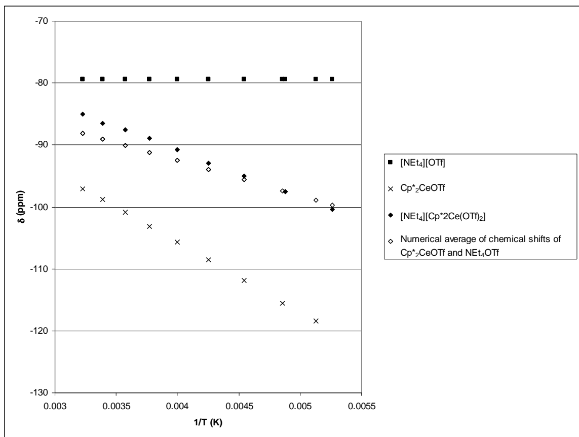
Figure 1.5.3: Variable-temperature ^{19}\text{F} NMR chemical shifts as a \delta vs. 1/T plot of \text{NEt}_4\text{OTf} , \text{Cp}^*_2\text{Ce}(\text{OTf}) , and [\text{NEt}_4][\text{Cp}^*_2\text{Ce}(\text{OTf})_2] in \text{CD}_2\text{Cl}_2 . The chemical shift of diamagnetic [\text{NEt}_4][\text{OTf}] is presumed to be temperature independent. The numerical average of the chemical shifts of \text{Cp}^*_2\text{Ce}(\text{OTf}) and [\text{NEt}_4][\text{OTf}] is also shown.
