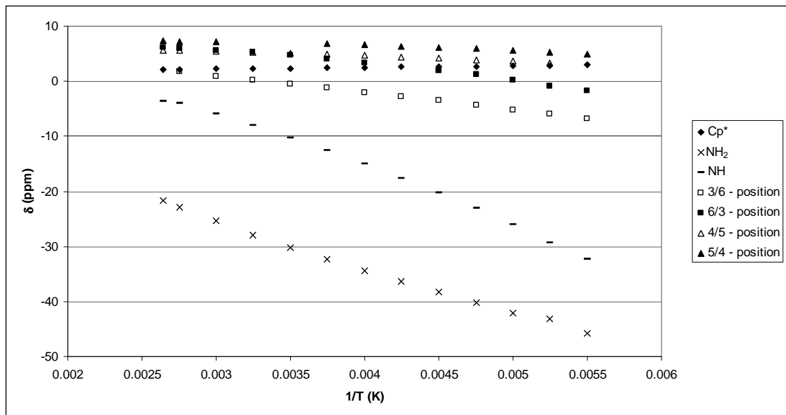
Figure 1.3.8: Variable-temperature ^1\text{H} NMR spectra represented as a \delta vs. 1/T plot of \text{Cp}^*_2\text{Ce}(\text{1-amido-2-aminobenzene}) in \text{toluene-d}_8 . The peak labeled 5/4 is hidden by the solvent peak between 280 and 310 K.
