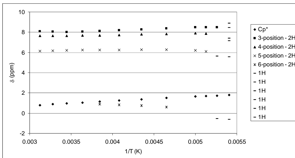
Figure 2.4.2: Variable Temperature ^1\text{H} NMR spectra represented as a \delta vs. 1/T plot of \text{Cp}^*_2\text{Sm}(\text{bipy})(\text{OTf}) in \text{CD}_2\text{Cl}_2 . Two of the area one resonances are not found.
