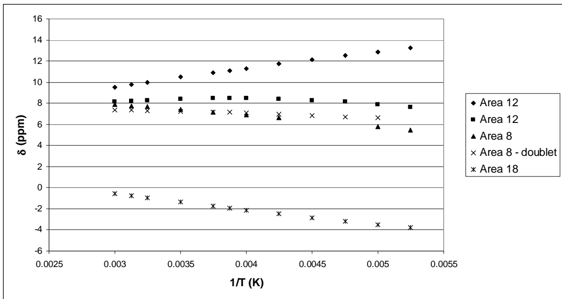
Figure 5.3.2: Variable Temperature 1 H NMR spectra represented as a \delta vs. 1/T plot of [(\text{MeC}_5\text{H}_4)_3\text{Ce}]_2(4,4'\text{-bipyridine}) in \text{thf-d}_8 .
