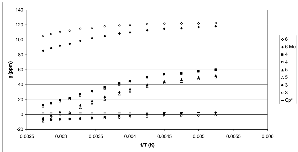
Figure 4.4.6: Variable Temperature ^1\text{H} NMR spectra represented as a \delta vs. 1/T plot of \text{Cp}^*_2\text{Yb}(\text{6-methyl-bipy}) in toluene- d_8 .
