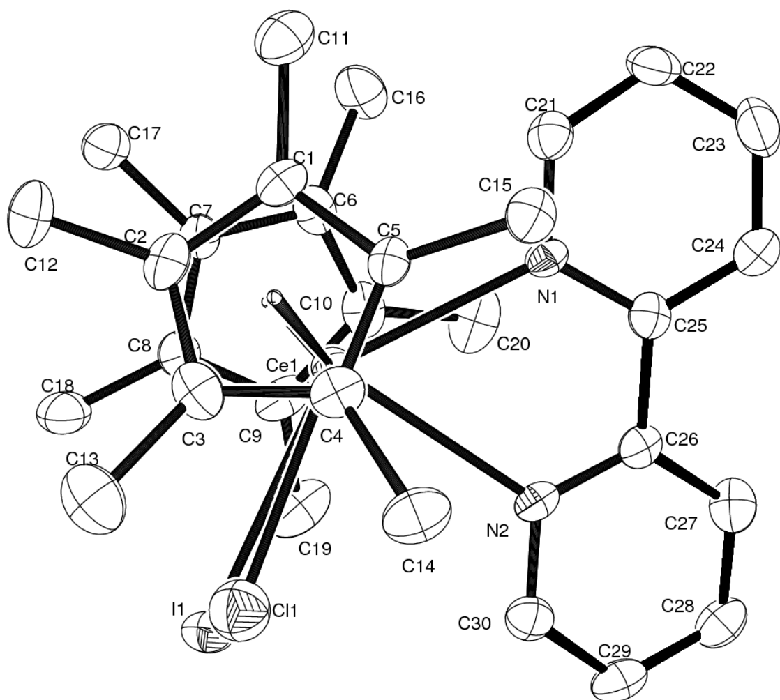
Figure 2.2.14: ORTEP diagram of Cp* 2 Ce(bipy)(X) (where X is partially occupied by I/Cl where the site is modeled with a 73% occupancy of I and 27% occupancy of Cl (50% probability ellipsoids). All non-hydrogen atoms except for Cl are refined anisotropically; Cl is refined isotropically. Hydrogen atoms are placed and not refined and are not shown. Selected Bond Distances and Angles are given in Tables 2.2.7 and 2.2.8, respectively. The N1-C25-C26-N2 torsion angle is 8.5(7)°. I1 is 0.031 Å out of the least-squares plane defined by the atoms in the bipyridine ring. 7
