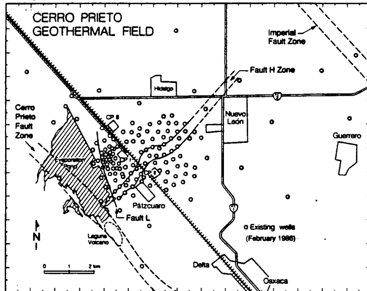
Figure 1 Location of geothermal wells and faults at Cerro Prieto. Fault H zone is shown at the beta reservoir level; Fault L is subvertical (after Halfman et al. , 1986).
