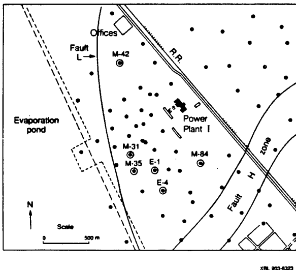
Figure 2 Location of Cerro Prieto I wells mentioned in the paper.
