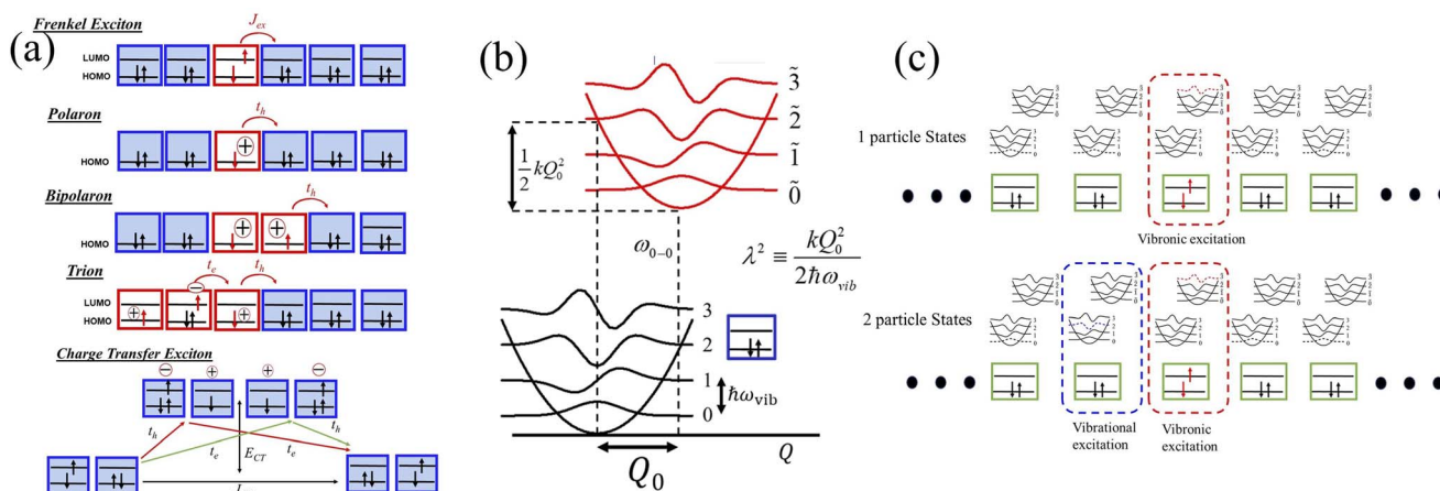
Fig. 1 (a) Simplified view of various forms of neutral and charged excitations. (b) Nuclear potential well corresponding to the aromatic to quinoidal stretching mode, Q , in the ground and excited electronic states for each isolated molecular unit. \omega_{\text{vib}} refers to the vibrational energy and the nuclear relaxation energy is denoted by \lambda^2 \omega_{\text{vib}} . (c) Schematic showing one-particle states, i.e. , vibronic excitations (top panel) and two-particle states, i.e. , vibronic/vibrational exciton pair.
