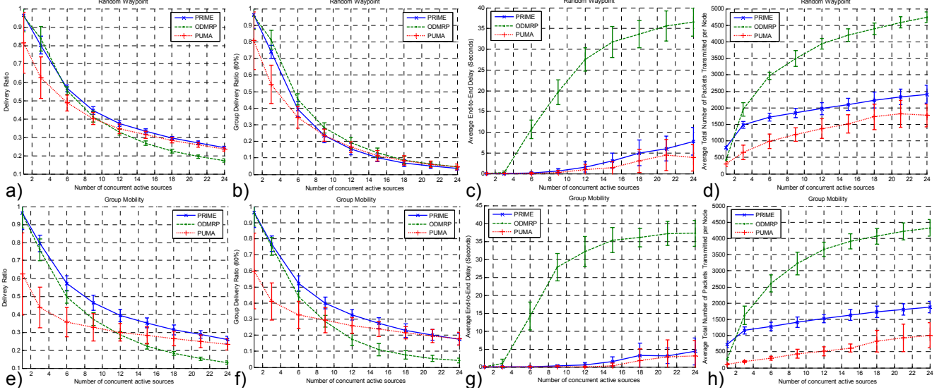
Fig. 5. Performance with increasing number of MCBR sources. (a-d) Random waypoint mobility model. (e-h) Group mobility model. (a and e) Delivery ratio. (b and f) Group delivery ratio. (c and g) End-to-End delay. (d and h) Average total number of packets transmitted per node.
