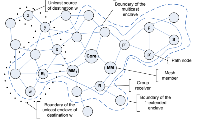
Fig. 3. Examples of a multicast enclave, its associated 1-extended enclave, and of the enclave of a unicast flow.
