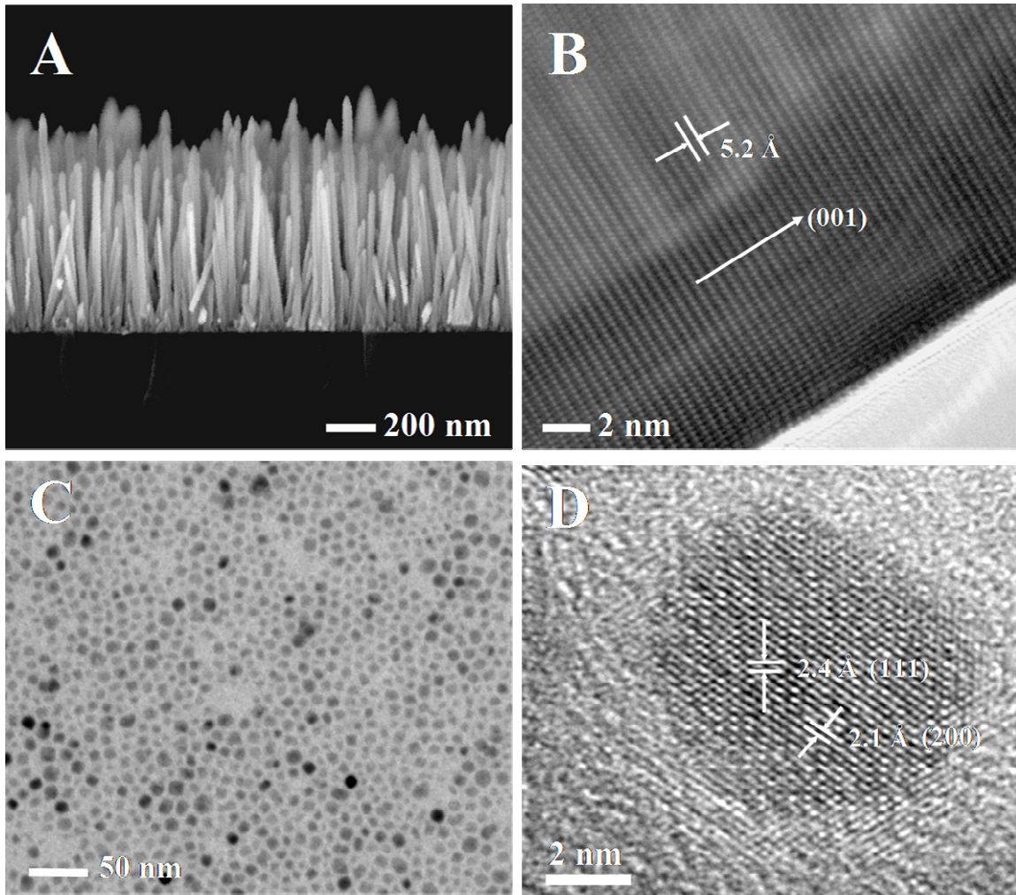
Figure 1. A) Cross-sectional SEM image of ZnO nanowire array used in solar cells, prior to Cu 2 O addition. B) High-resolution TEM image of an individual ZnO nanowire. C) Low r
