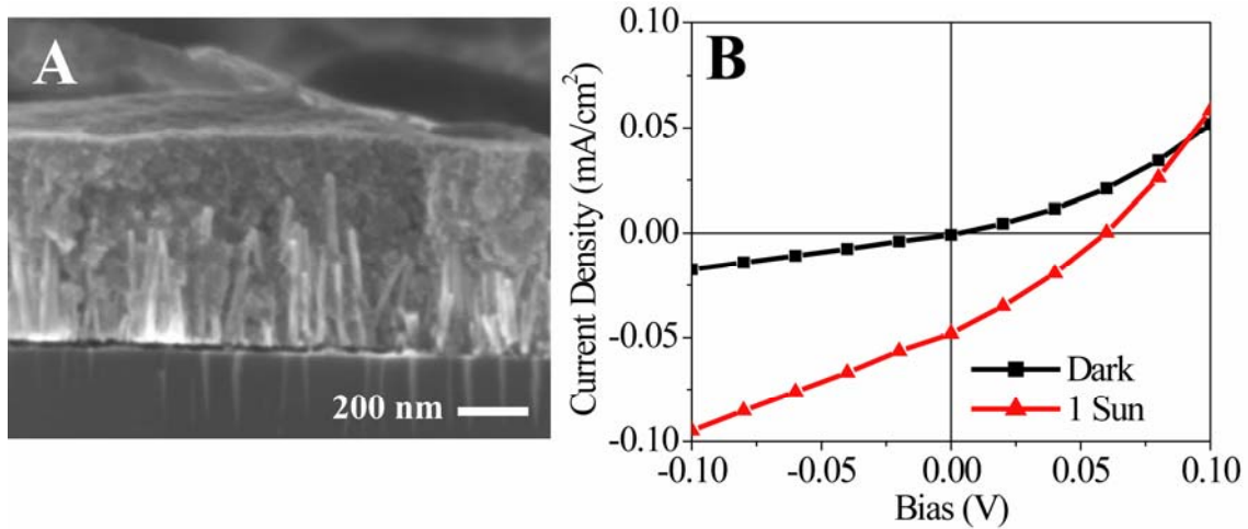
Figure 4. A) Cross-section SEM of a completed ZnO/Cu 2 O solar cell, with the cell annealed at 200°C after each application of Cu 2 O NPs. B) The corresponding J-V curve in darkness and under AM 1.5 and 1 Sun illumination.
