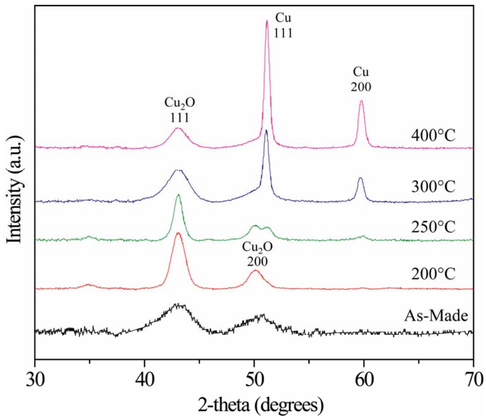
Figure 3. XRD patterns of \text{Cu}_2\text{O} NPs films on glass, annealed at the noted temperatures under Argon. The patterns are vertically offset for clarity.
