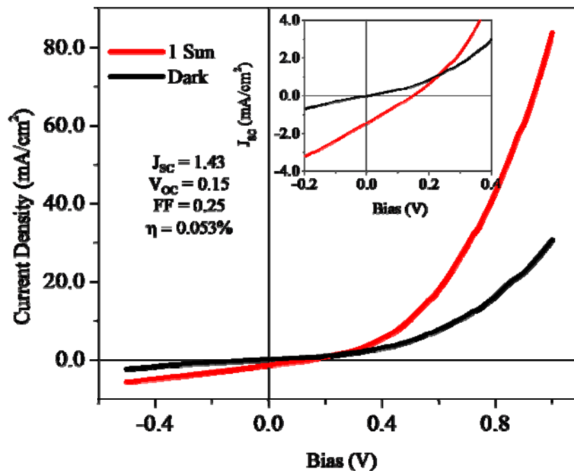
Figure 7. J-V curves of a ZnO/TiO 2 /Cu 2 O solar cell in darkness and under 1 Sun illumination. The Cu 2 O film was annealed at 300°C under 500 mTorr oxygen. The ZnO NWs are 500 nm in length, the TiO 2 coating layer is 10 nm thick, and the Cu 2 O film thickness is 800 nm.
