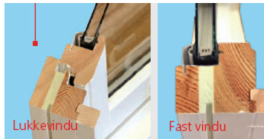
Figure 30. Example of a wood window frame with a relatively low U-value - N-Tech Lavenergi Superspacer by NorDan AS. Wood frame with PUR. The frame U-value is not stated, whereas the total window U-value is reported to be U_w = 1.2 \text{ W/m}^2\text{K} . Note that a two-layer window pane is employed in this case (not three-layer). From http://www.nordan.no .
