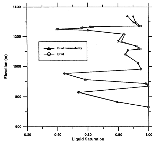
Figure 1. Steady-state liquid saturation profiles for fractures and matrix, obtained using the ECM and the dual-permeability models.
