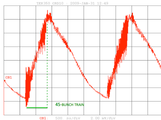
Figure 7. Example of direct phase measurement in the resonant BPM configuration.
