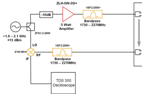
Figure 3. RF mixing circuit used for direct measurements of the phase delay.
