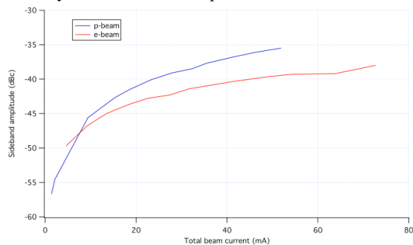
Figure 6. First sideband amplitude measured with the resonant BPM with positron and electron beam.
