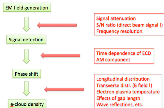
Figure 1. Block diagram of a TE wave measurement procedure, with its sources of error/uncertainty.
