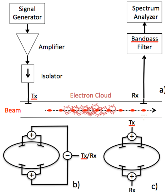
Figure 2. a) Instrumentation setup b) Button arrangement for transmission measurements c) Button arrangement for "resonant BPM" scheme.
