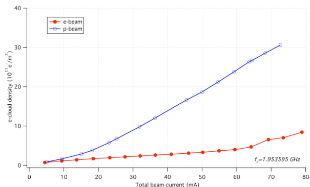
Figure 4. Transmission measurements in the dipole region. 45-bunch train positron and electron beam.
