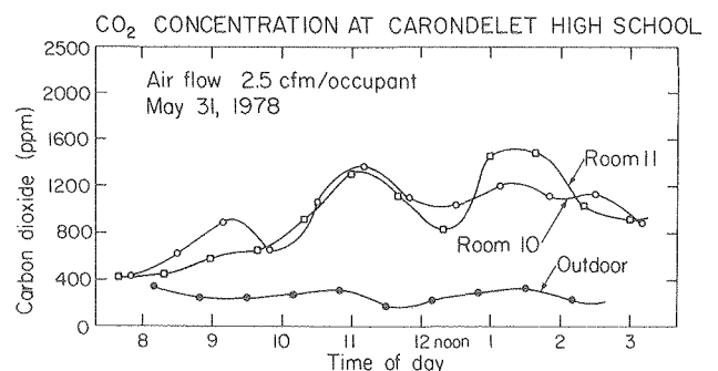
Fig. 2. CO 2 concentrations at Carondelet High School in Rooms 10 and 11 and outside. Total air flow is 3700 cfm. May 31, 1978. (XBL 791-250A)
