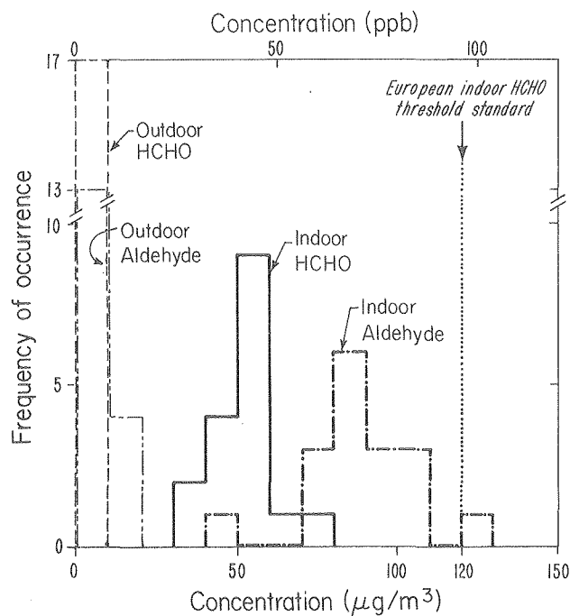
Fig. 10. Indoor/outdoor formaldehyde/aldehyde concentrations. Iowa State University Energy Research House, December 1978.
