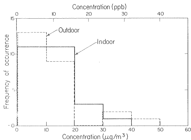
Fig. 11. Indoor/outdoor aldehyde concentration. Naval Regional Medical Center, Long Beach, California, October 1978.
