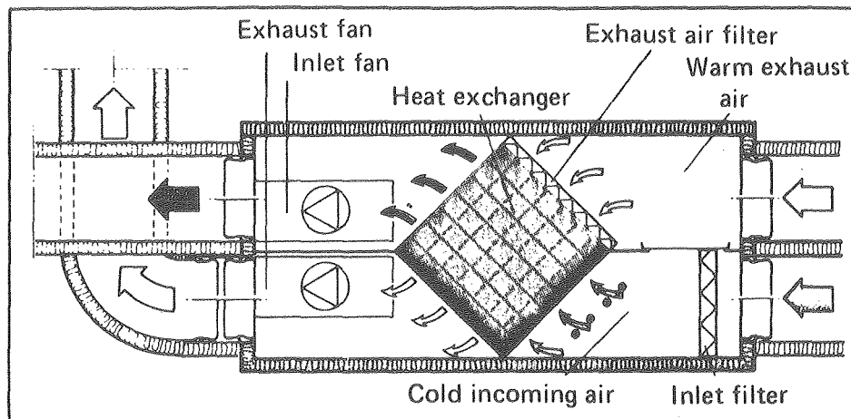
Fig. 13. Principle of operation of heat exchanger.
