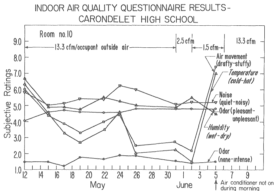
Fig. 3. Six indoor air quality parameters plotted as a function of day of month and ventilation rate. Data taken from questionnaire. The subjective rating ranged from 1 to 9 with lower numbers corresponding to the first adjective in parentheses. (XBL 791-251A)
