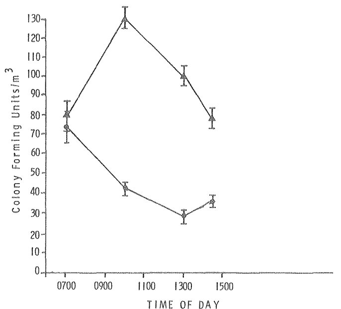
"RESPIRABLE BURDEN" (PARTICLES 5 \mu m IN DIAMETER OR LESS) AT CARONDELET HIGH SCHOOL (●) AND TOTAL NUMBERS (▲).
