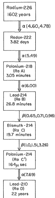
Fig. 6. Decay chain, radium-226 to lead-210 ( \alpha, \beta energies in MeV). (XBL 7212-4903B)
