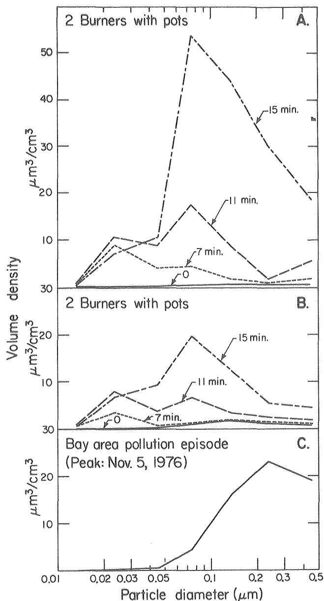
Fig. 2. Volume density and distribution of particulate emissions less than 0.5 \mu\text{m} in diameter. Figures 2A and 2B illustrate gas stove particulate emissions for two experiments under similar conditions in which two top burners were operated with water-filled cooking pots. The size distribution at 7, 11 and 15 minutes after turning on the burners is shown. Figure 2A shows the case where carbon accounts for 35% of the total emitted mass. Figure 2B shows the case where carbon accounts for 90% of the total emitted mass. In both cases, the absolute amount of carbon emitted is the same. Figure 2C shows the peak volume concentration distribution for a San Francisco Bay Area air pollution episode. (XBL 791-235A)
