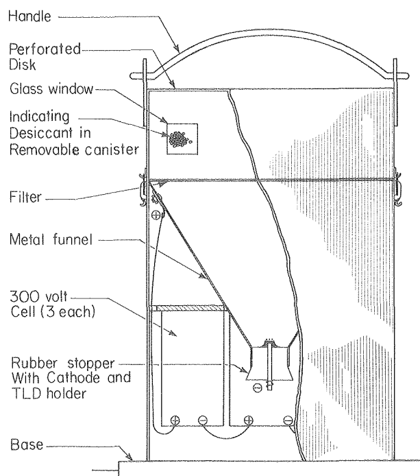
Fig. 7. Schematic drawing of Passive Radon Monitor. (XBL 791-252)
