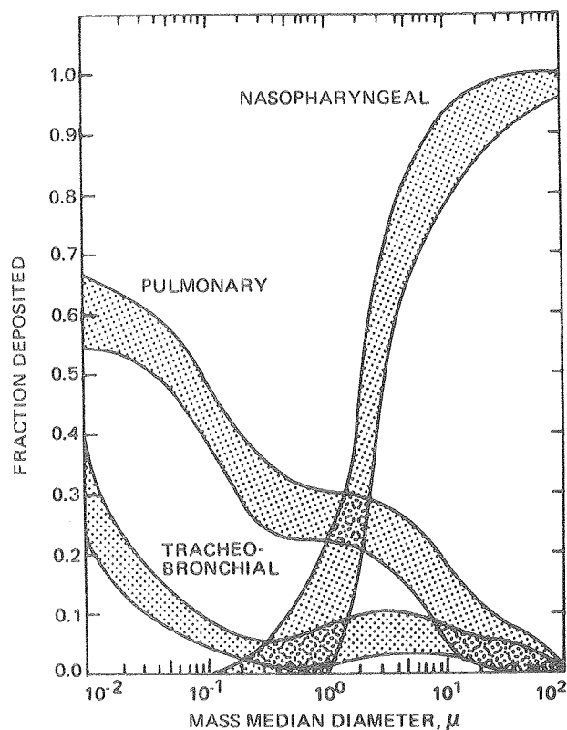
Fig. 1. Fraction of particles deposited in the three respiratory tract compartments as a function of particle diameter. 31 (XBL 771-7190)
