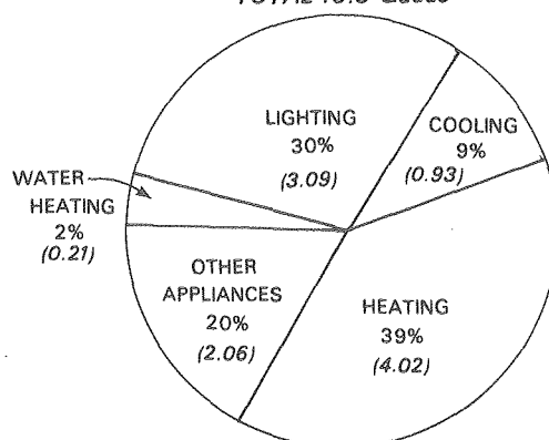
Fig. 1. Primary energy consumed in the U. S. by residential and commercial buildings. Numbers in parentheses are in units of quads or 10^{15} Btu. Source: Department of Energy, Office of Conservation, Buildings and Community Systems, Five Year Program Plan. (XBL 785-903)
