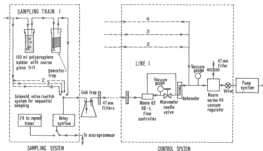
Fig. 8. Formaldehyde/aliphatic aldehydes grab sampling system. (XBL 791-257A)
