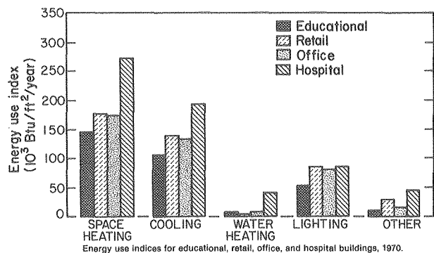
Fig. 1. Energy use indices for educational, retail, office, and hospital buildings, 1970. 1 Energy use in primary units. (XBL 7810-11637)
