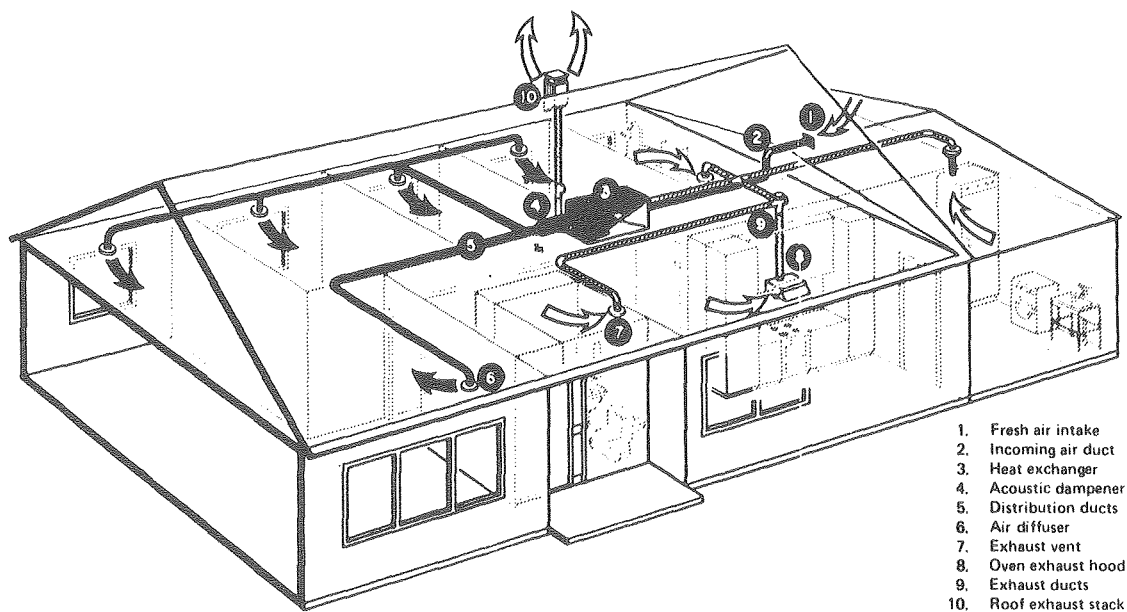
Fig. 12. Residential heat exchanger system.
