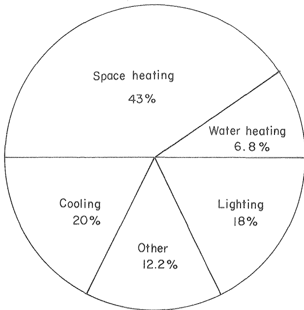
Fig. 2. Hospital energy use in 1975. 1 Energy use calculated in resource or primary units. To account for conversion losses, the primary energy for electricity has been calculated in terms of 10,383 Btu/KWhr (the average heat rate estimated by the Edison Electric Institute for 1975). In addition, 9% electrical transmission-distribution losses have been assumed. (XBL 792-439)
