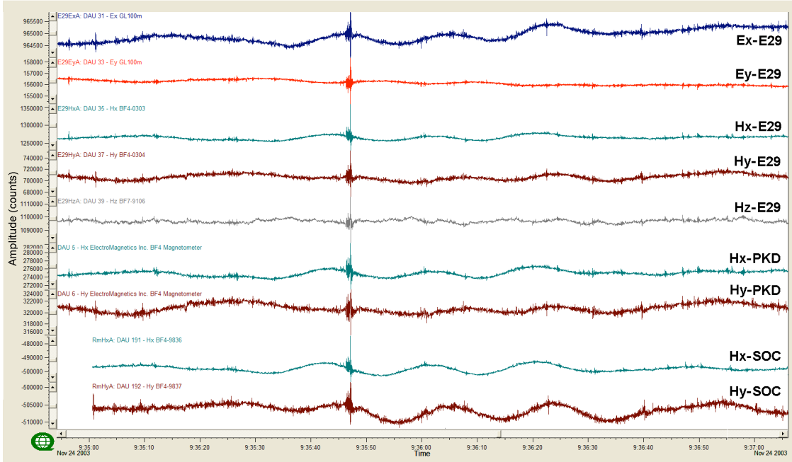
Figure 8. Comparison of all five channels of MT time series at site E29 with the two horizontal magnetic fields used as references at PKD and at SOC.
