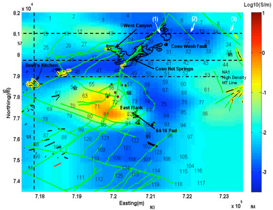
Figure 20. Horizontal slice through 3D conductivity model at a depth of 500m below sea-level based upon 2003 and 2005 data sets; 100 to 0.1 Hz. Color represent \text{log}_{10} of conductivity. The surface elevation averages 1200m above sea-level. Mapped surface expression of faulting are green liniments. The 125 MT stations are numbered. Micro-earthquake seismometer locations (S1, S2, S4, S5, S6, S7 and N1) from Lees and Wu (2000) are shown. Straight dashed lines are location of depth sections shown in Figures 21, 22, 23 and 24. Location of the NA1 high-density MT line (Figure 10) is shown as the dot-dash horizontal black line near Northing 79,000 m.
