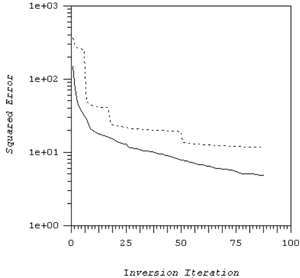
Figure 17. Plot of the convergence of the 3D inversion iteration for the 100 to 1 Hz data. The dashed curve is a plot of the convergence of the error functional with regularization constraint. The solid curve is a plot of the weighted squared error, the data misfit without regularization.
