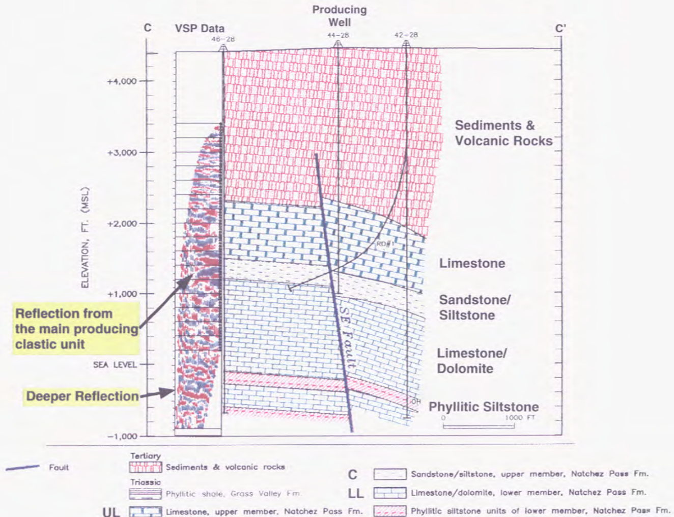
Vertical geologic section, C-C', Rye Patch, Nevada
