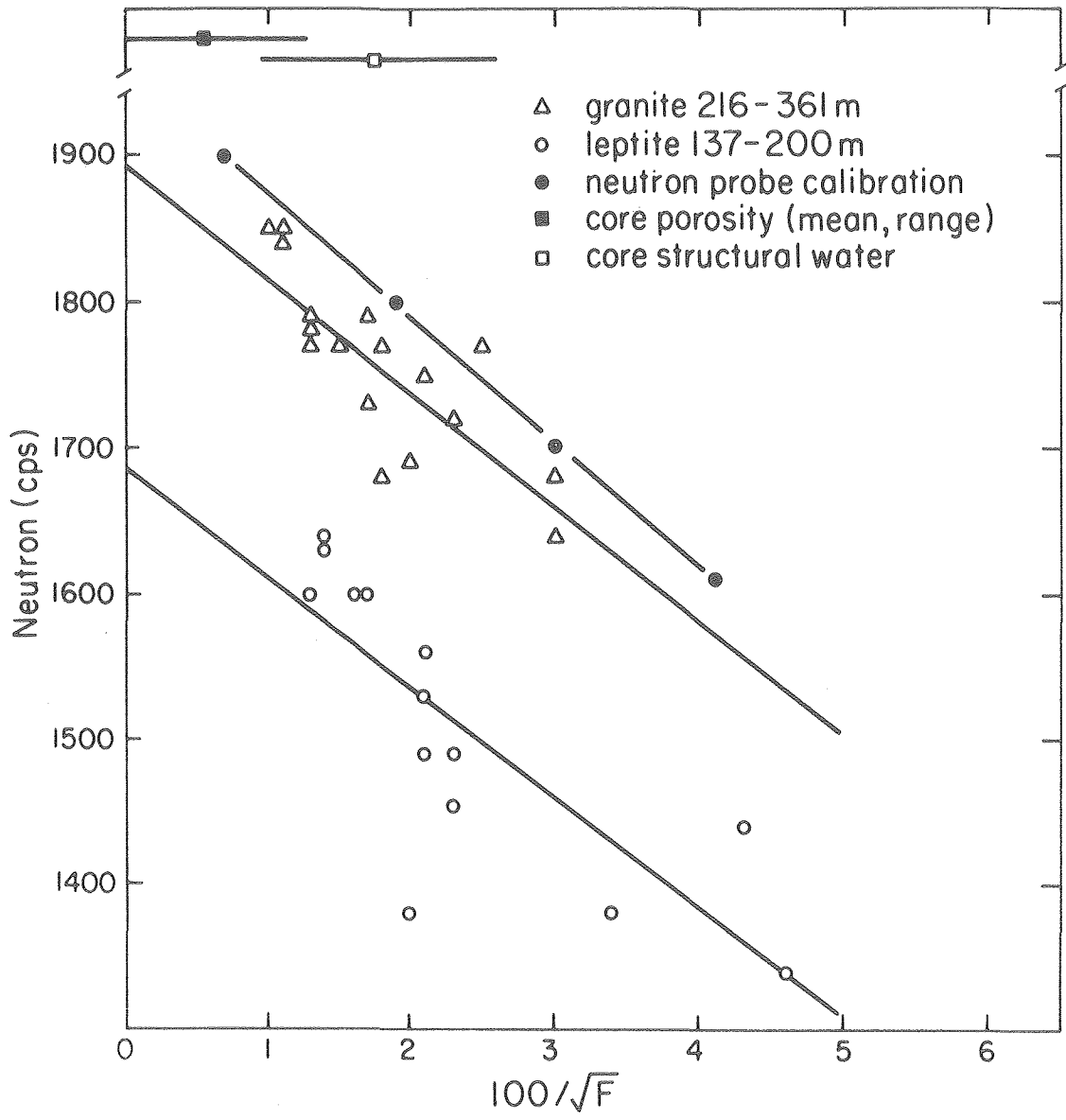
Fig. 6. Neutron-resistivity cross-plot for SBH-1. Conversion of apparent resistivity values to formation factor F is described in the text. Bottom scale is equivalent to volume percent porosity. Standard deviation of neutron count rate is equivalent to the size of the symbols. Straight lines represent least-squares fits to the probe calibration, the granite data, and the leptite data. Mean values and range of core porosity and structural water measurements are given at top of figure.
