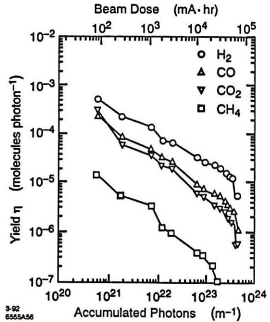
Fig. 3. Desorption coefficients for C10100 sample.
